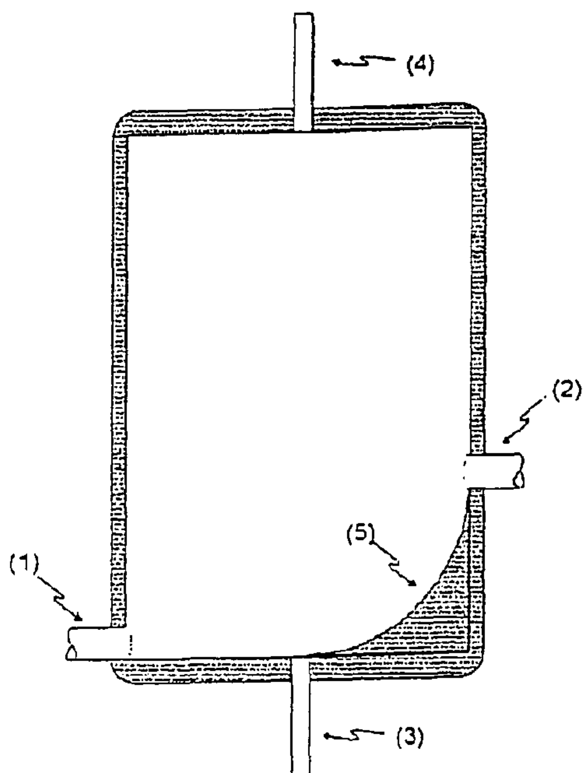
Figure 6. Reservoir design 6.
