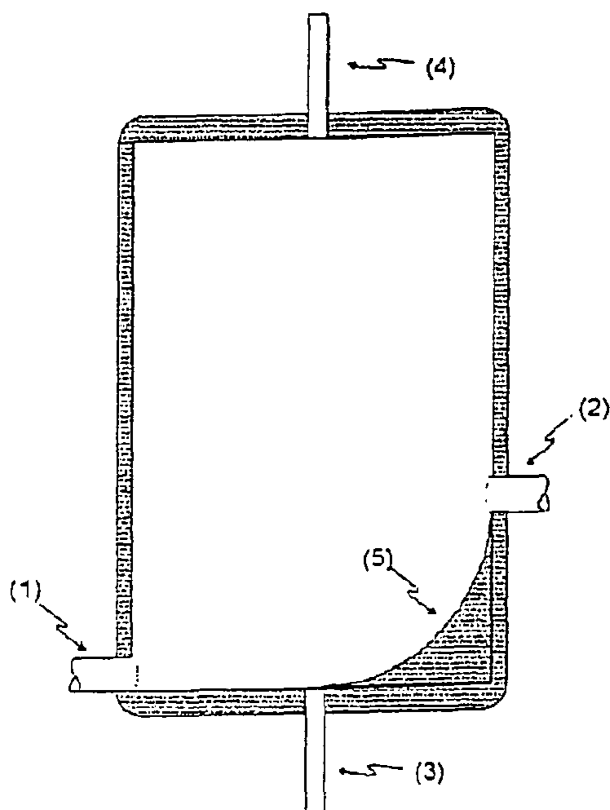
Figure 6. Reservoir design 6.
