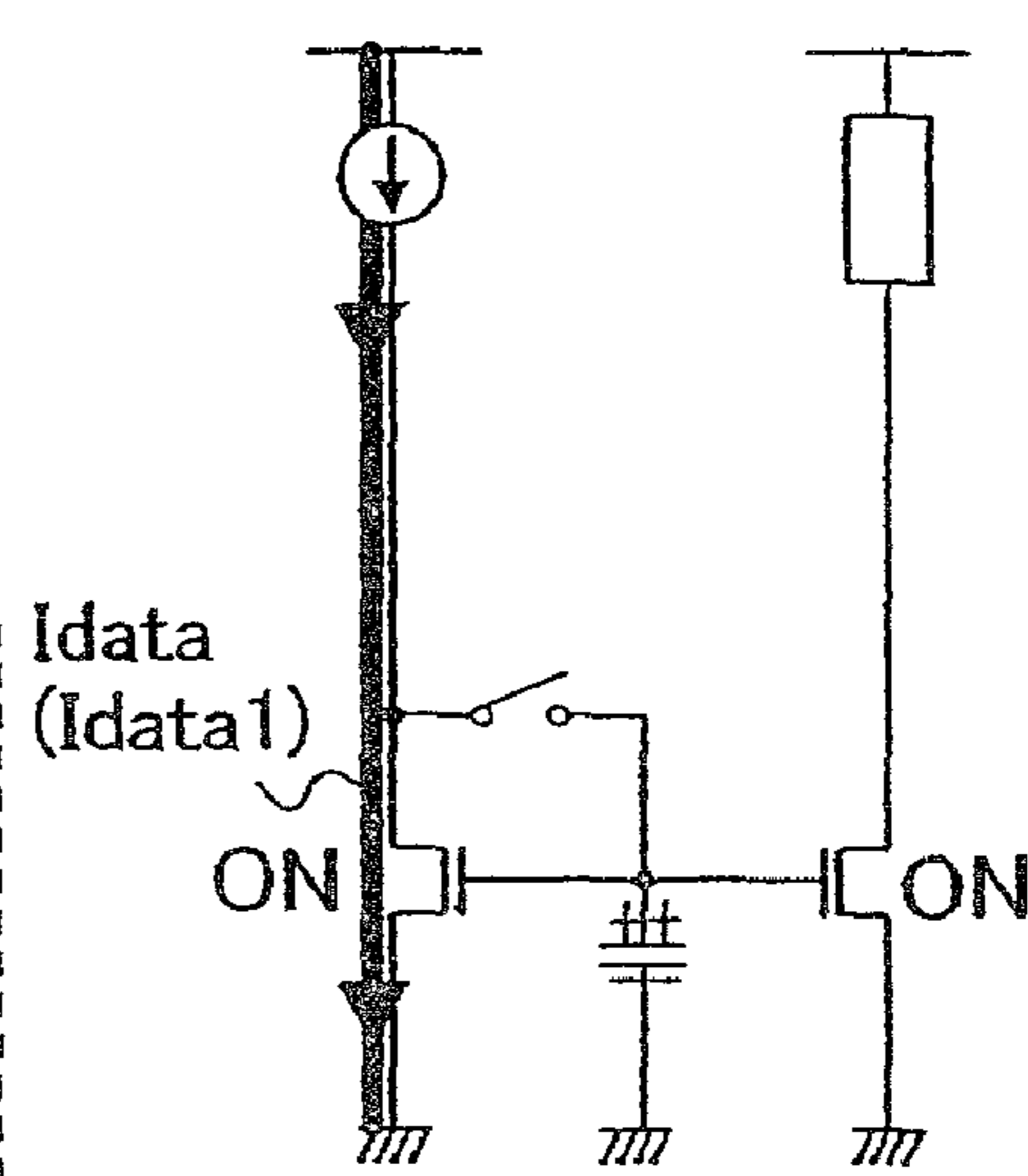
Fig. 20B signal input complete time
