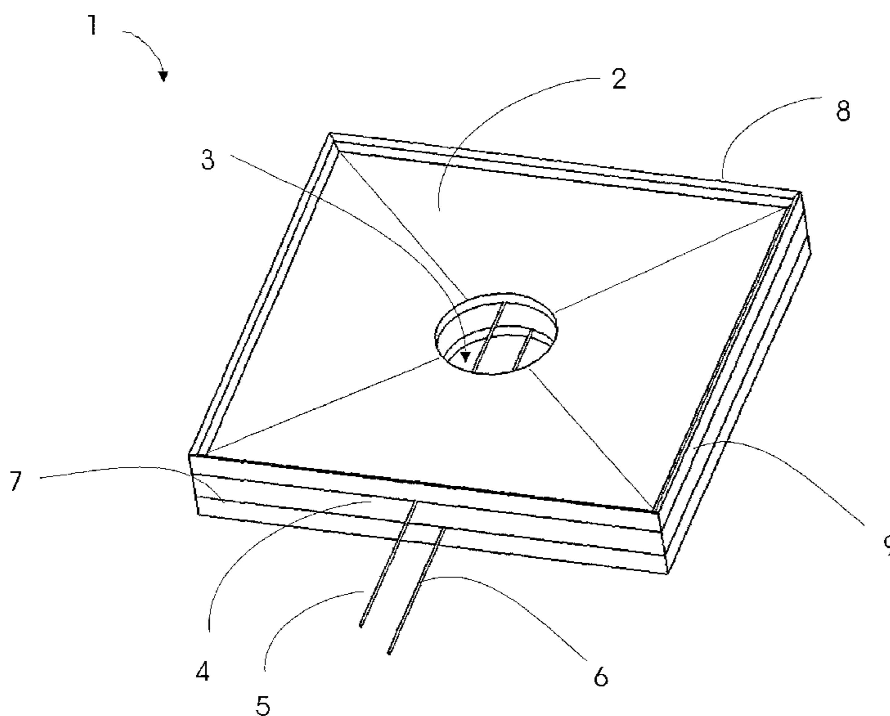
Water Sensing Cell Assembly
