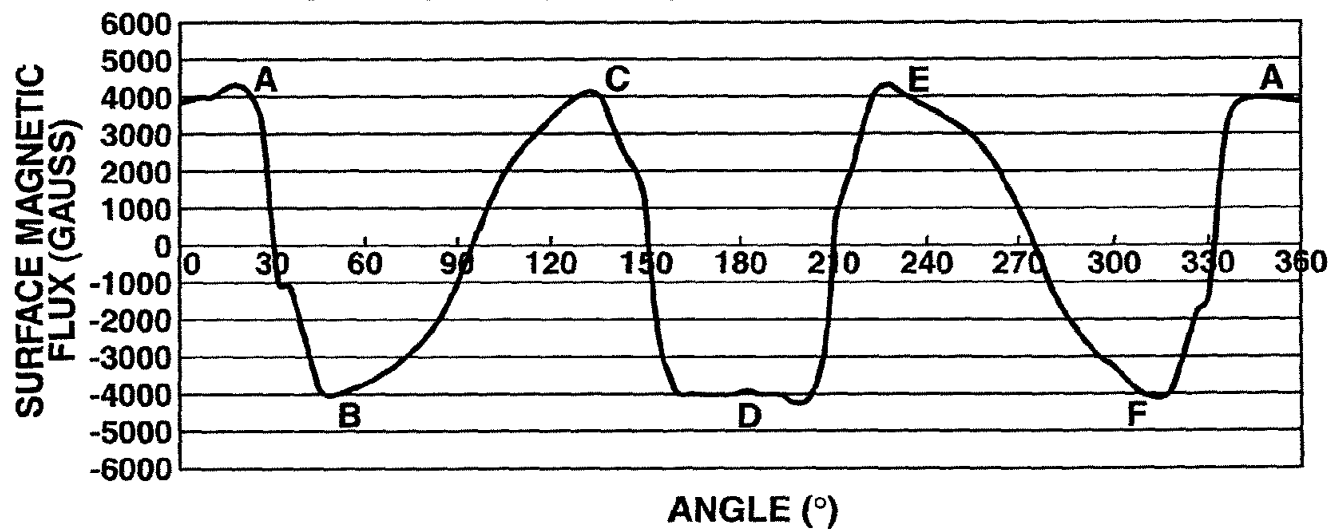
INVENTIVE SIX-POLAR MAGNETIZED PRODUCT FROM DIAMETRICALLY ORIENTED CYLINDRICAL MAGNET
