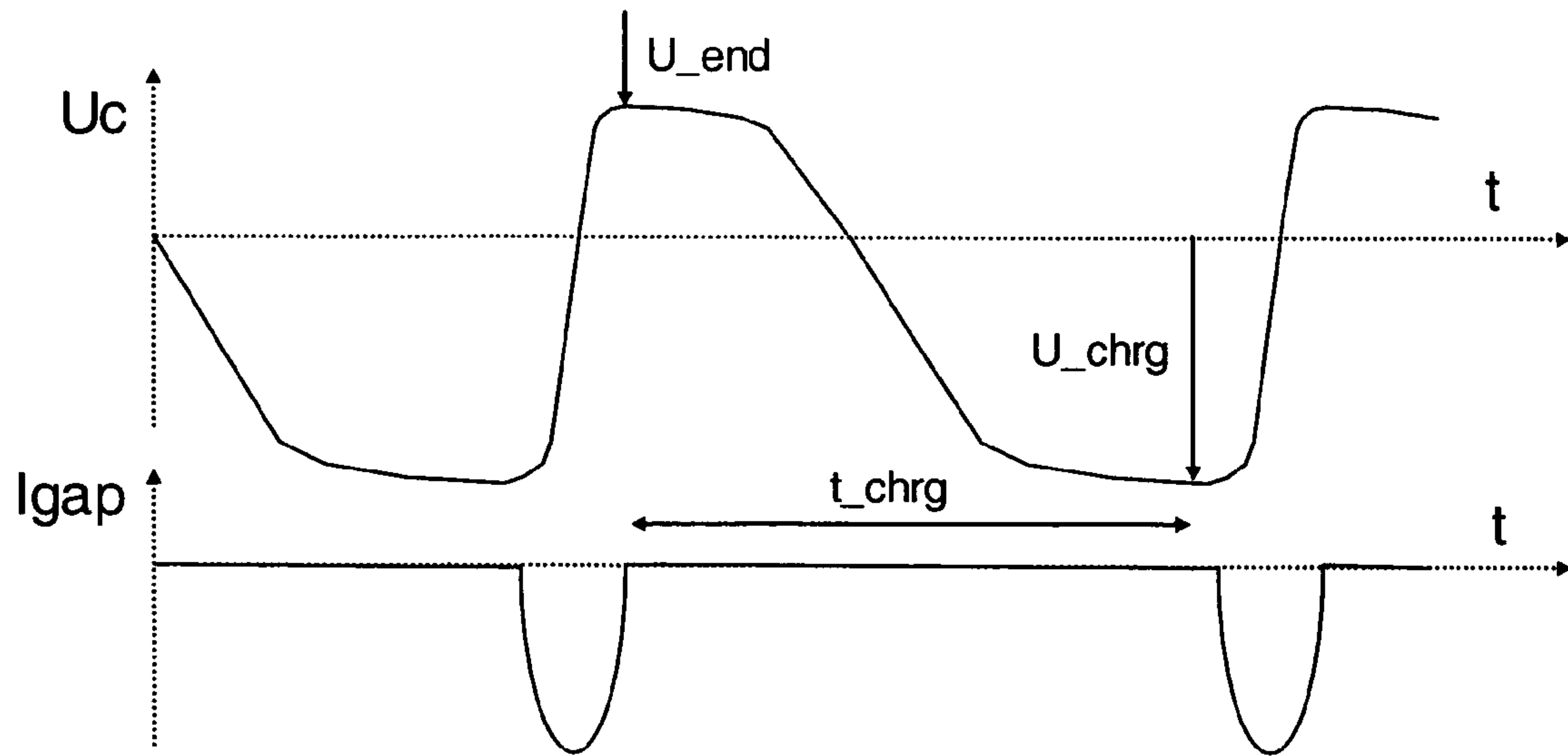
Fig 5 Prior Art
