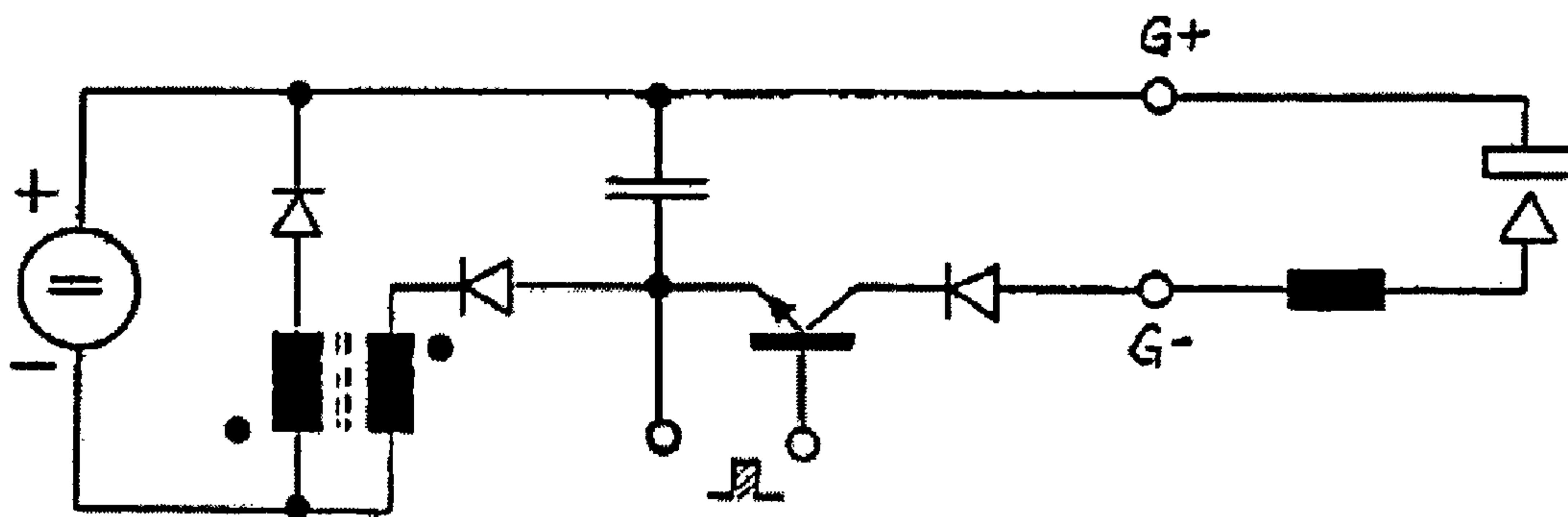
Fig 4 Prior Art
