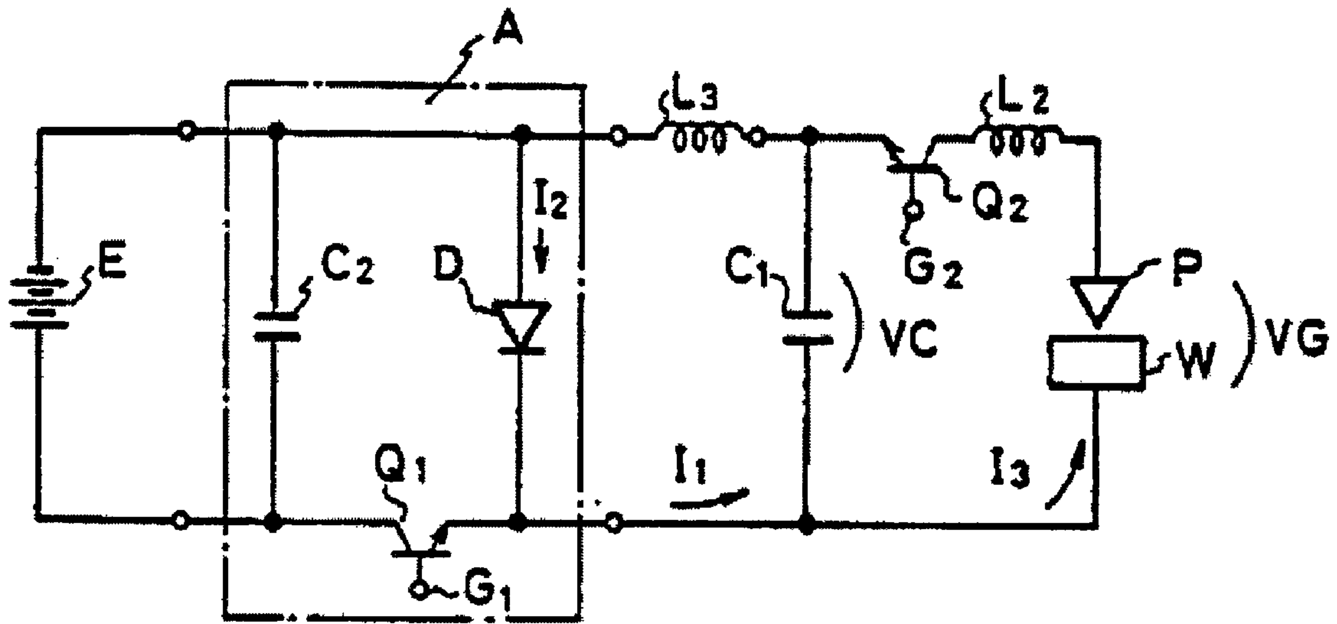
Fig 3 Prior Art
