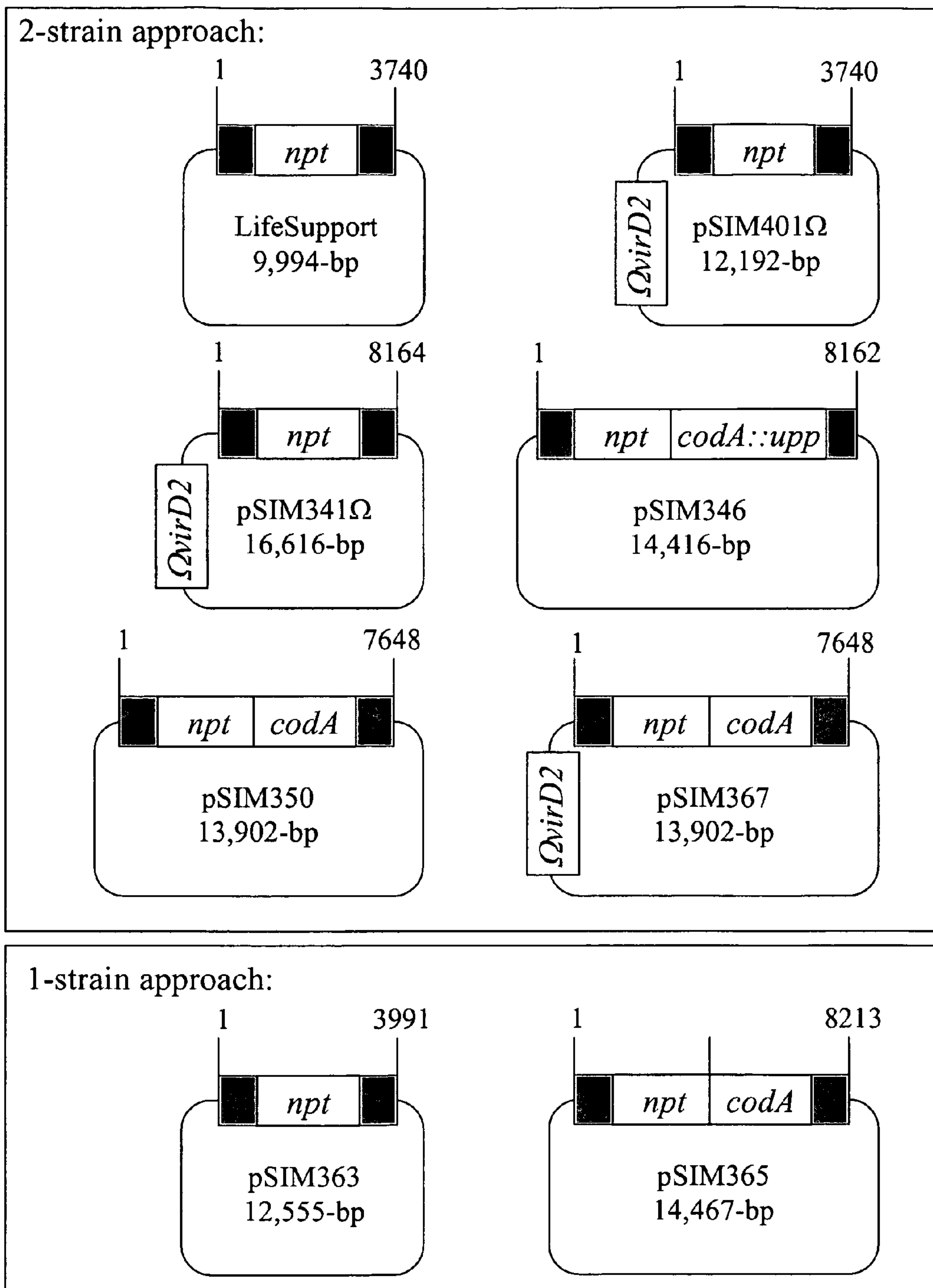
Figure 5. Diagrams for some LifeSupport vectors
