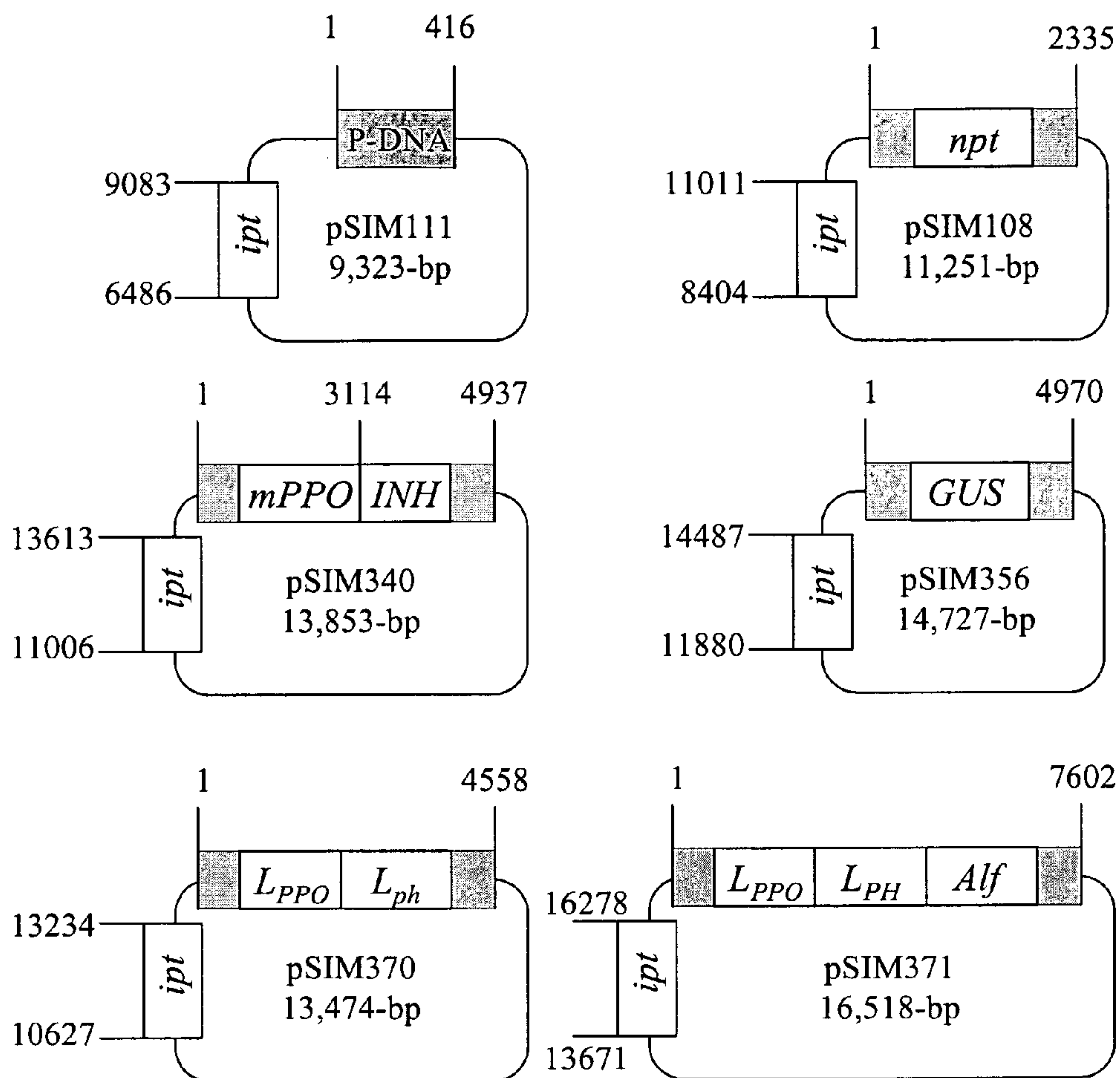
Figure 1. Diagrams for some P-DNA vectors
