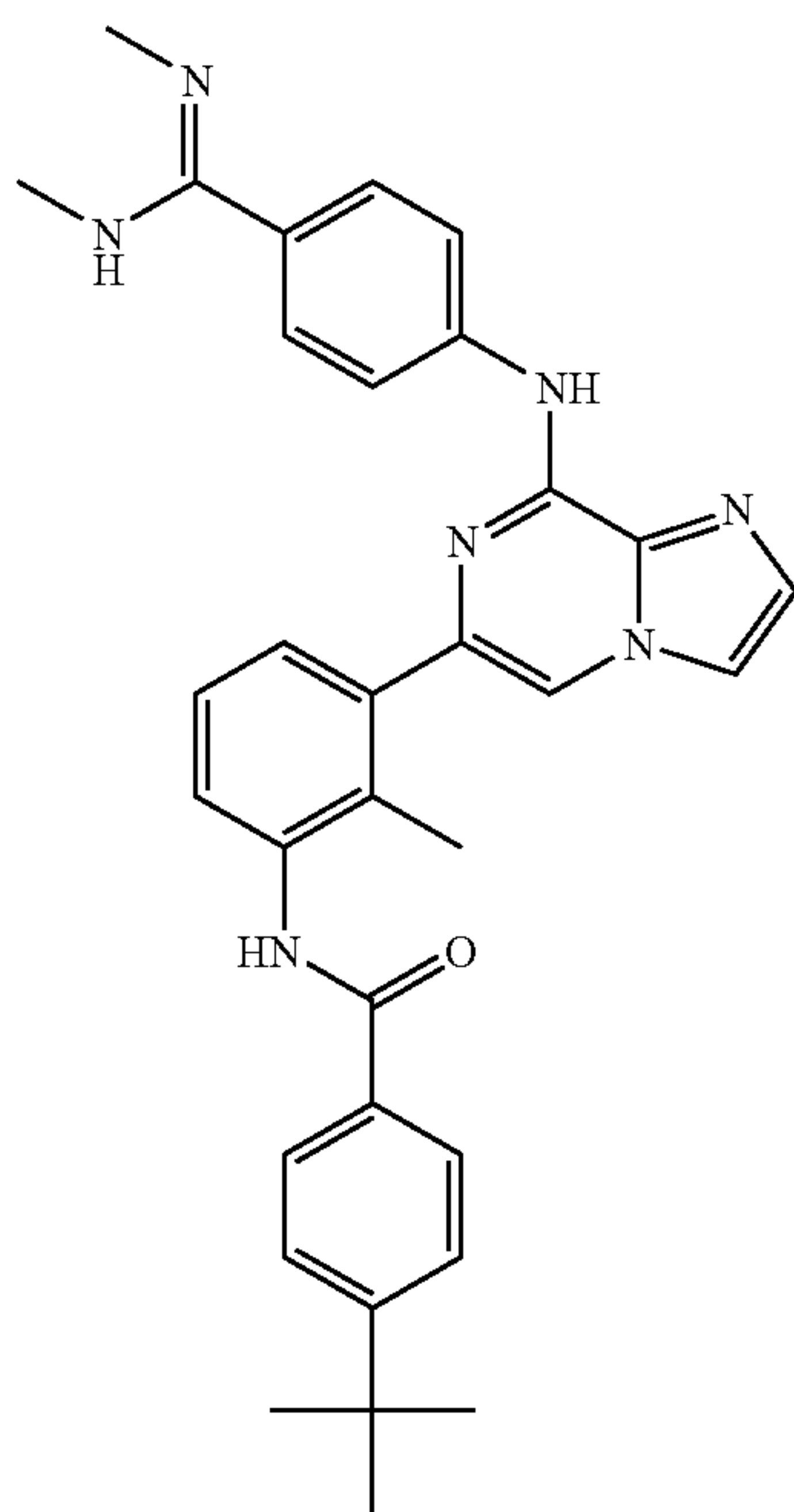
4-tert-Butyl-N-(3-{8-[4-(N,N'-dimethyl-carbamimidoyl)-phenylamino]-imidazo[1,2-a]pyrazin-6-yl}-2-methyl-phenyl)-benzamide
