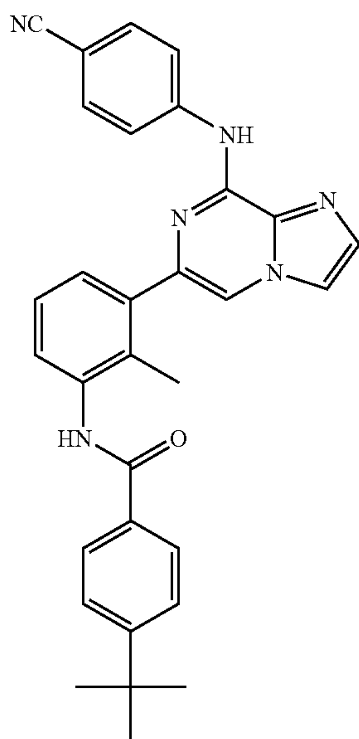
4-tert-Butyl-N-{3-[8-(4-cyano-phenylamino)-imidazo[1,2-a]pyrazin-6-yl]-2-methyl-phenyl}-benzamide
