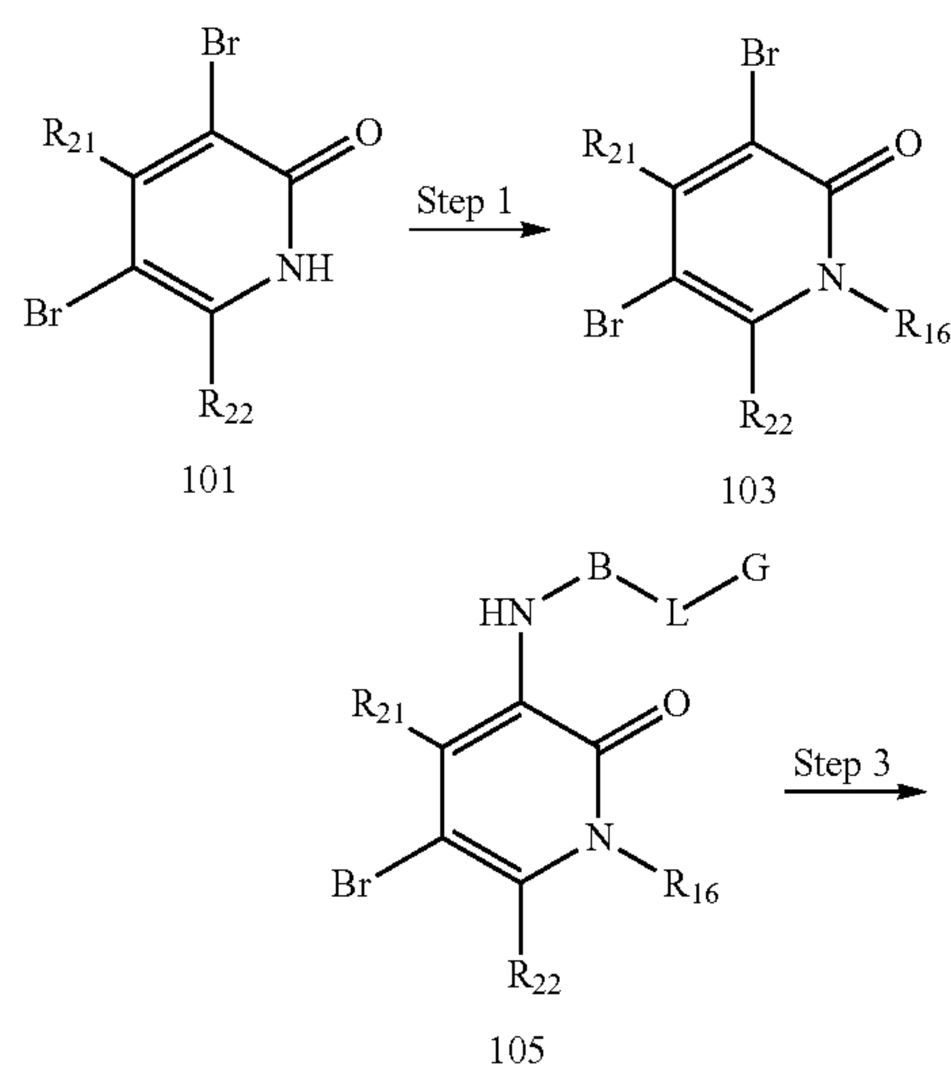
Reaction Scheme 1
