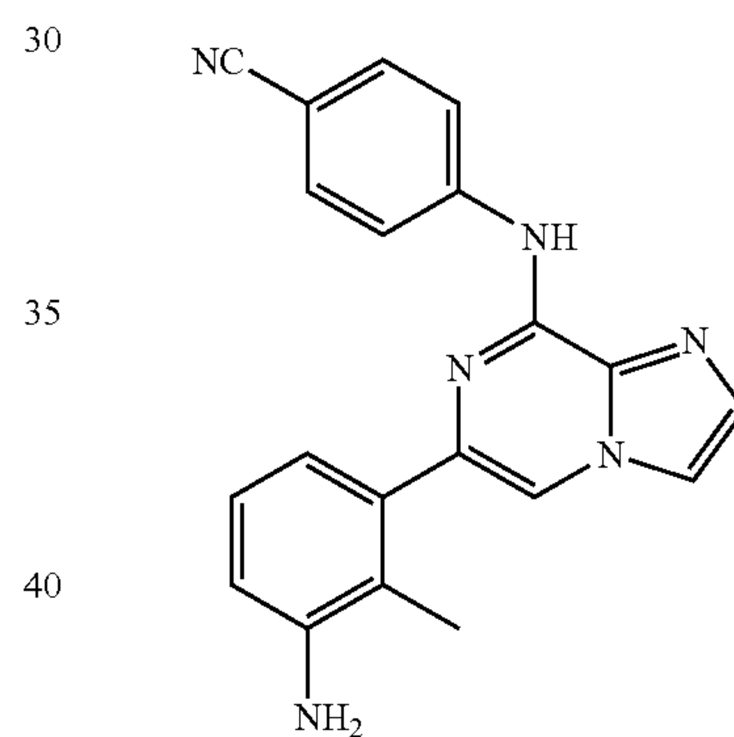
4-[6-(3-Amino-2-methyl-phenyl)-imidazo[1,2-a]pyrazin-8-ylamino]-benzonitrile
