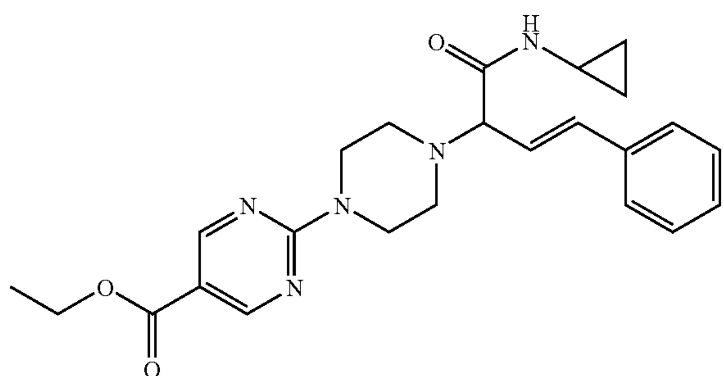
Interm. 32; Ex. [A5]; mp. 221° C.
