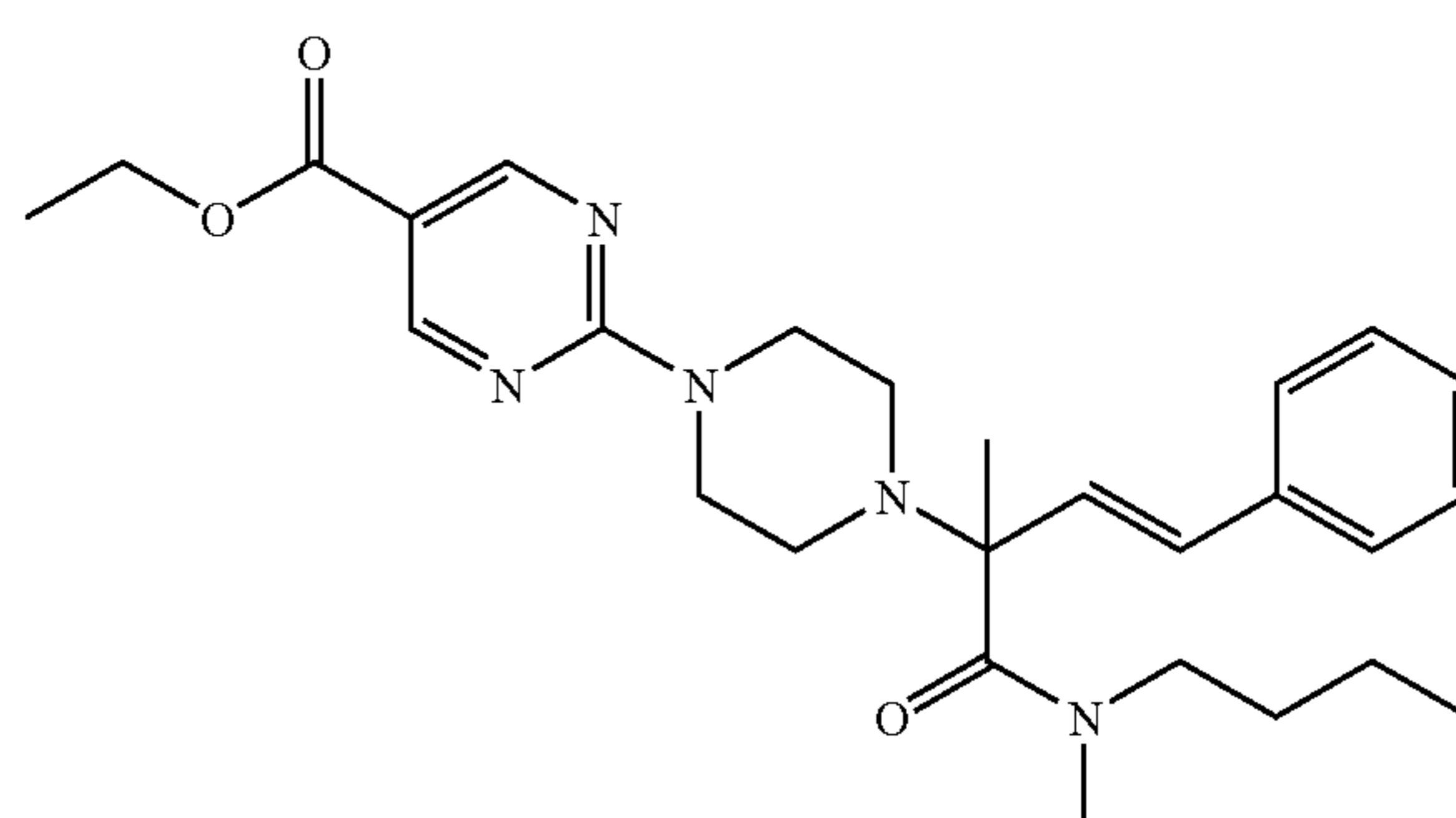
Interm. 37; Ex. [A5]
