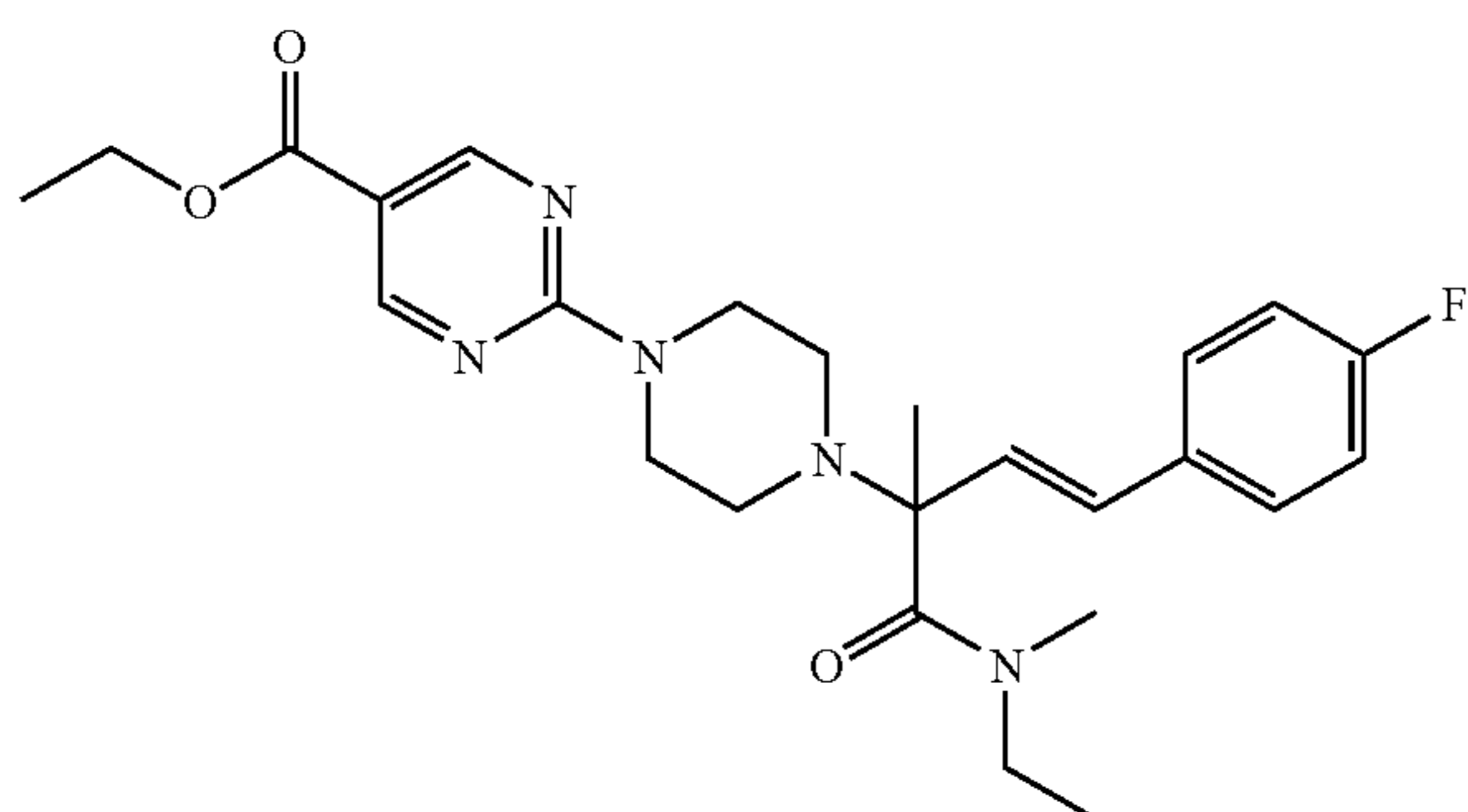
Interm. 31; Ex. [A5]; mp. 196° C.
