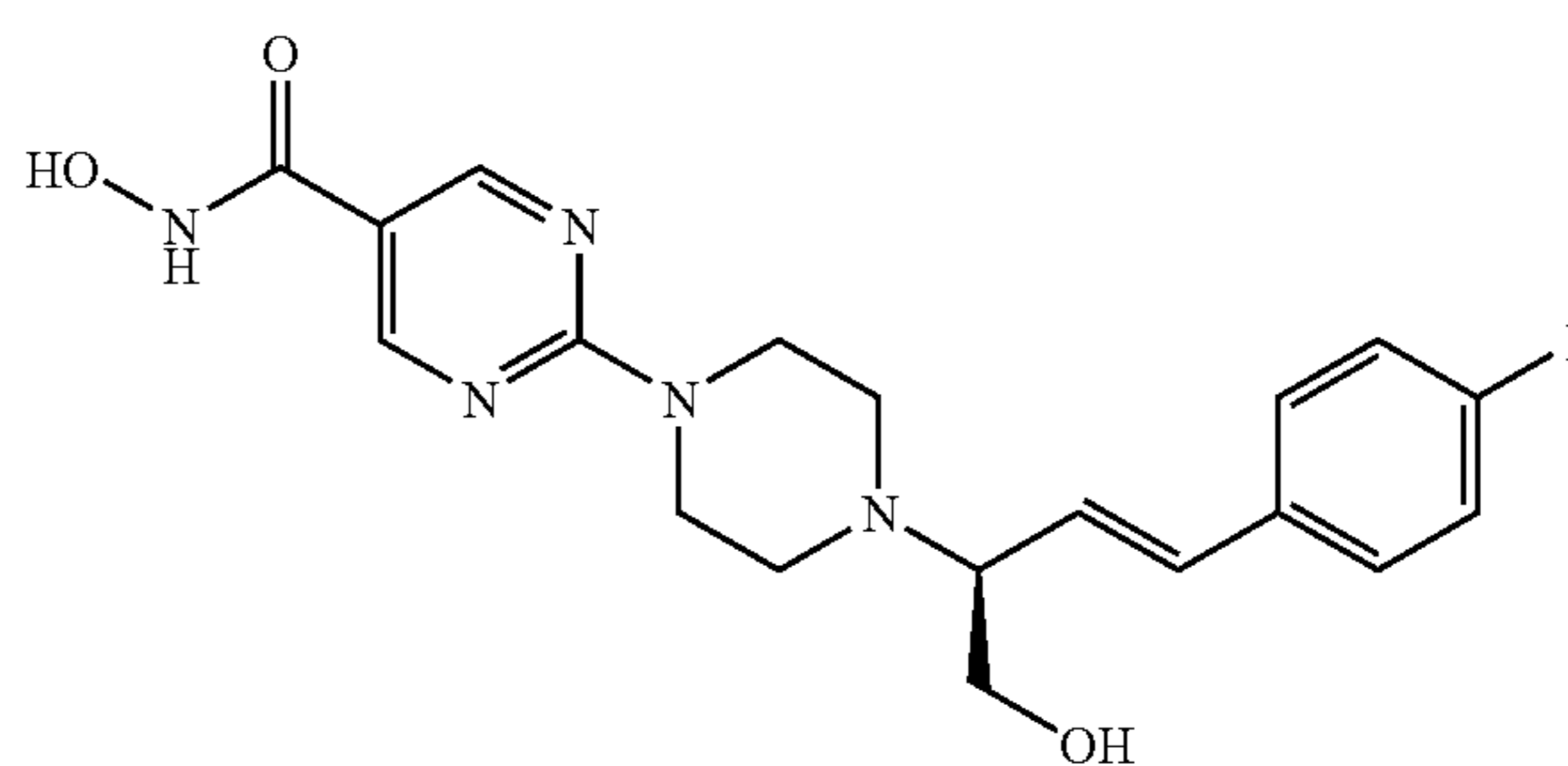
Compound No. 33; •HCl; enantiomer A
