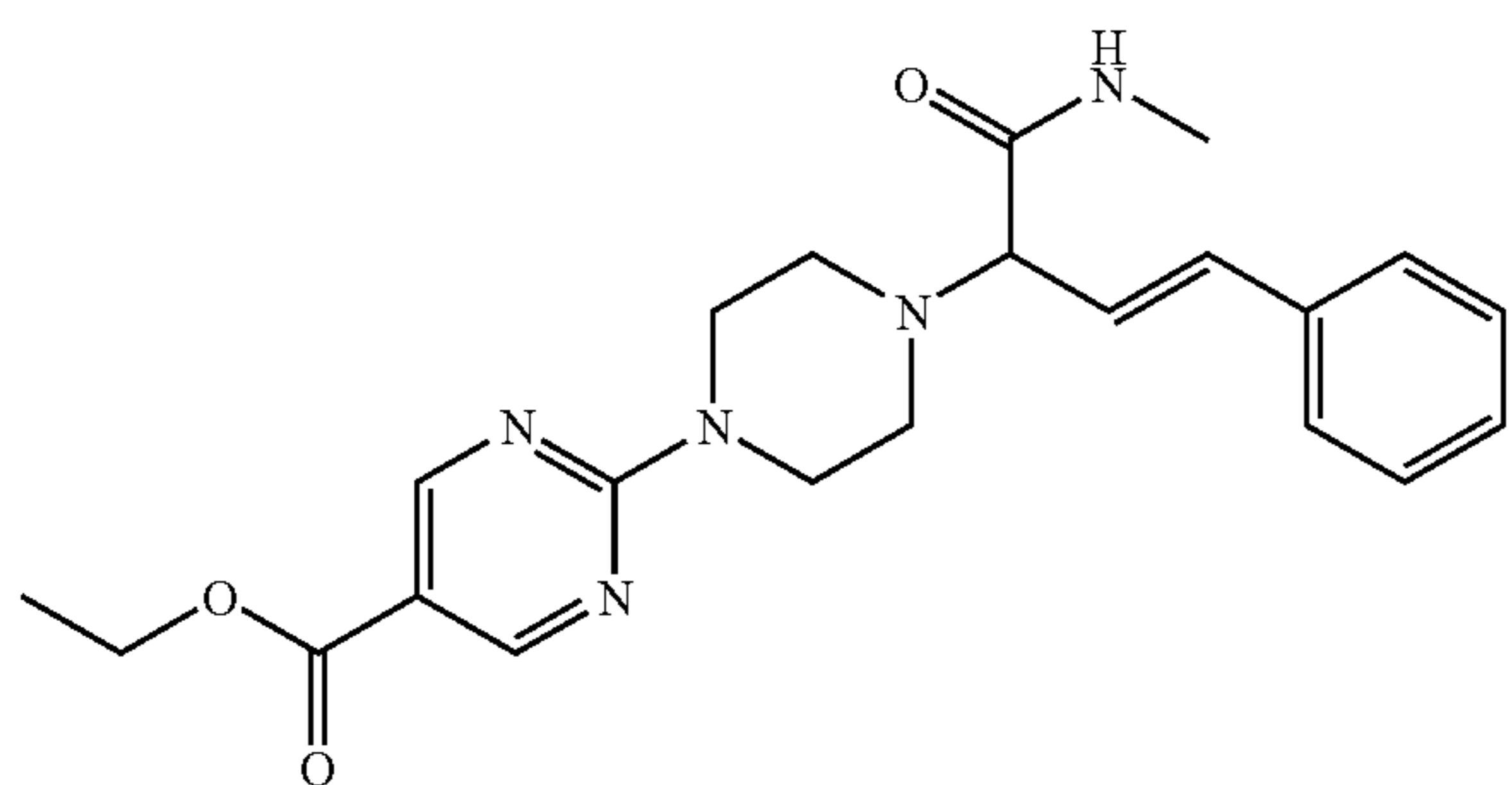
Interm. 33; Ex. [A5]
