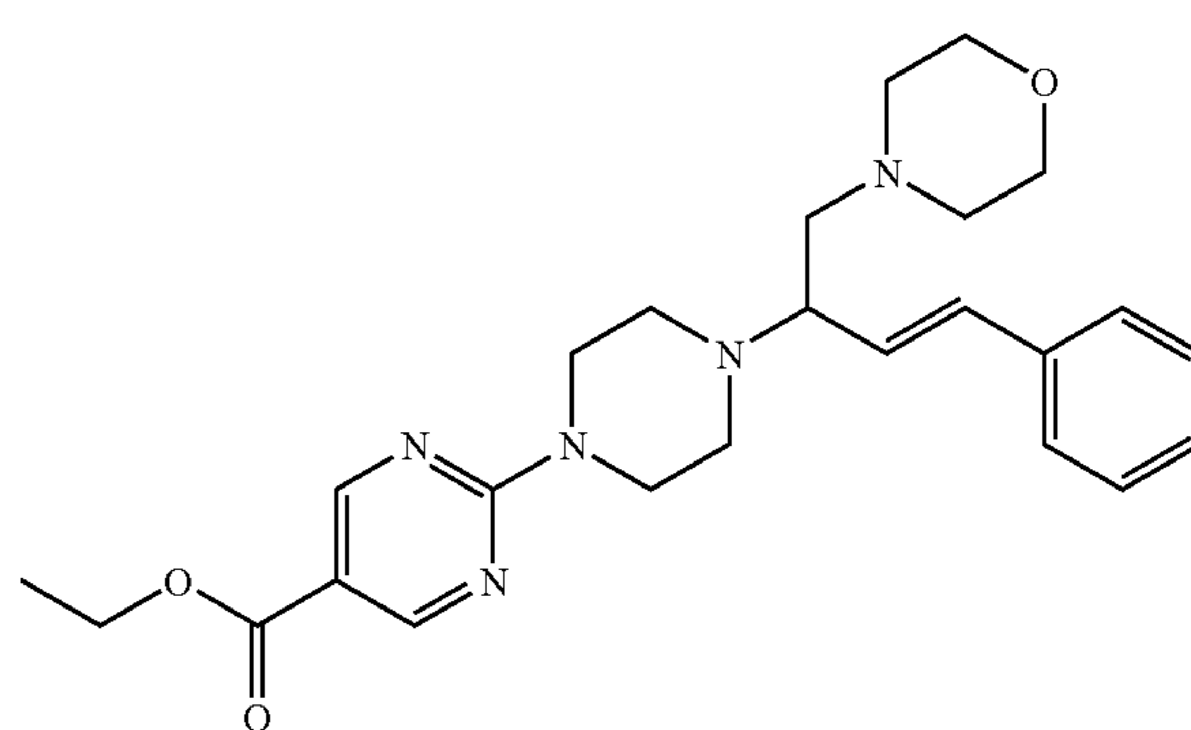
Interm. 38; Ex. [A2]
