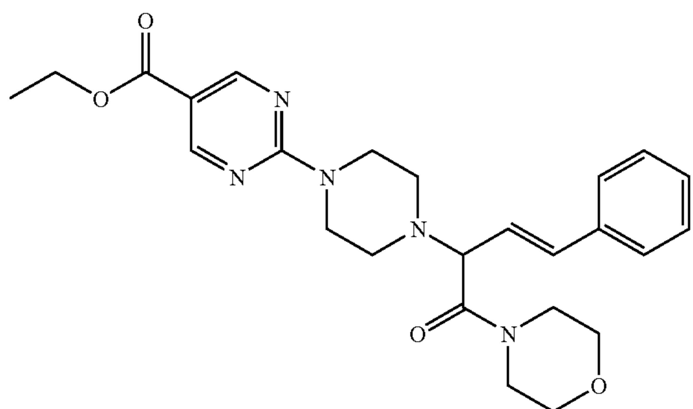
Interm. 34; Ex. [A5]
