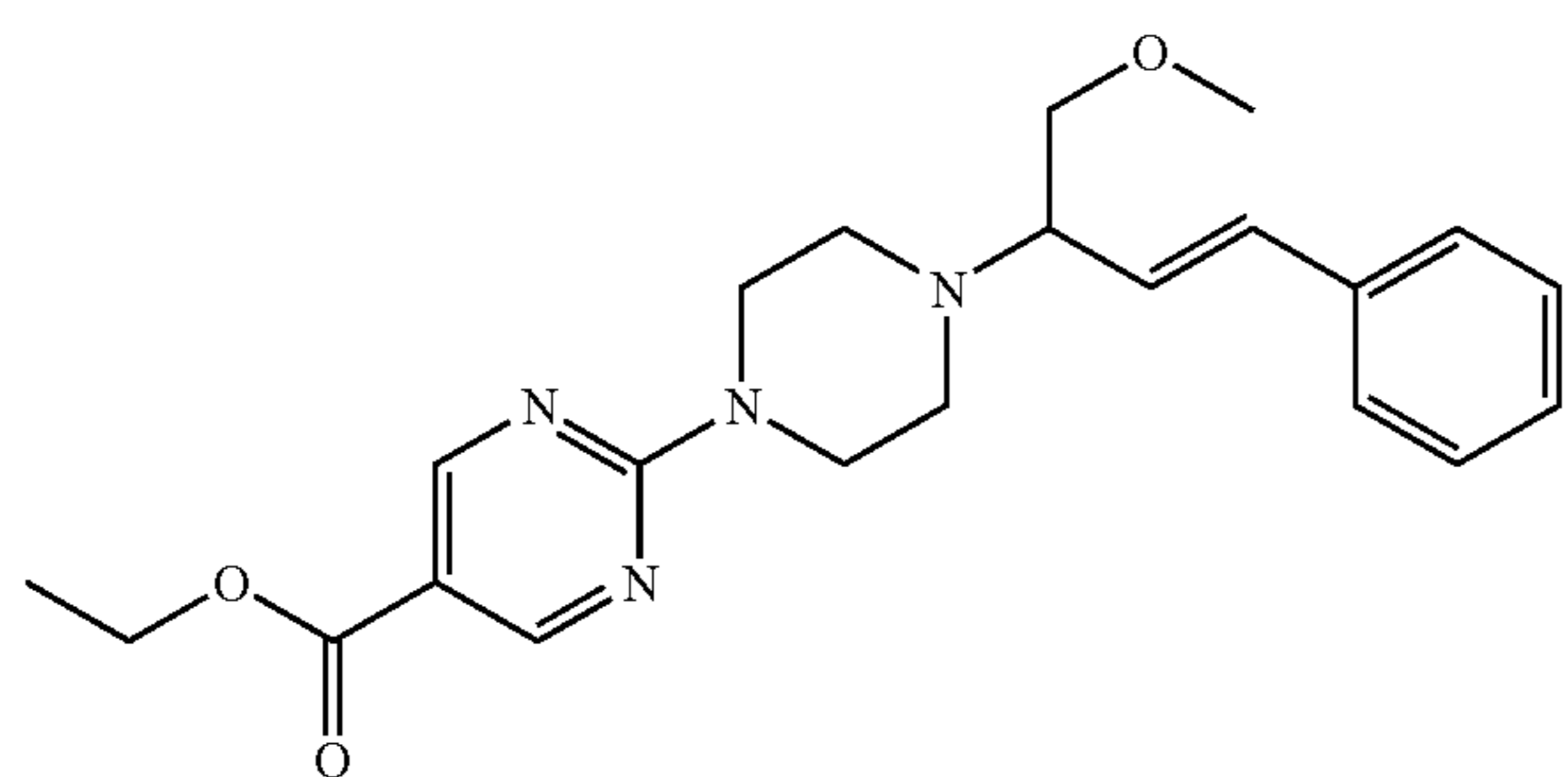
Interm. 22; Ex. [A6]
