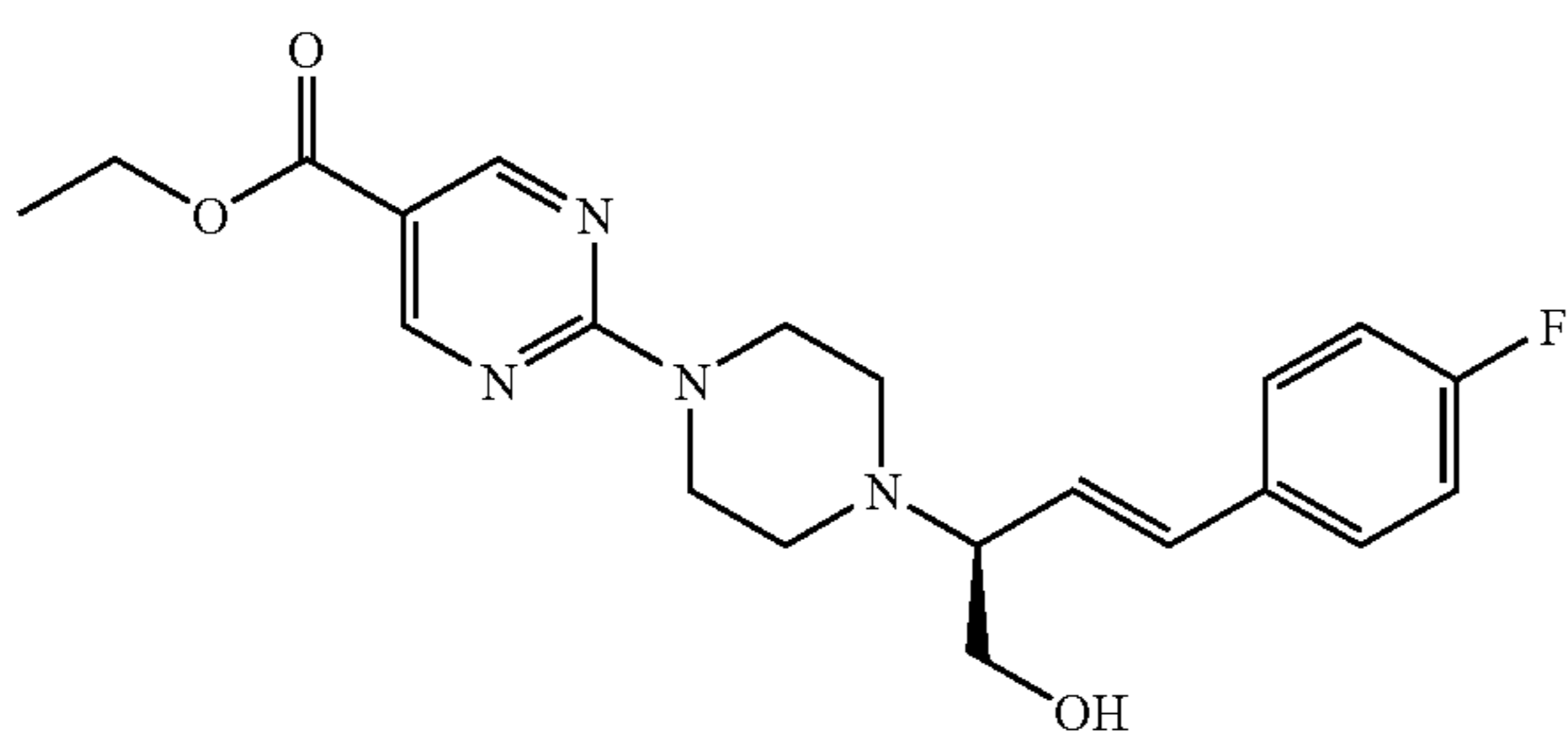
Interm. 42; Ex. [A1] (enantiomer A)
