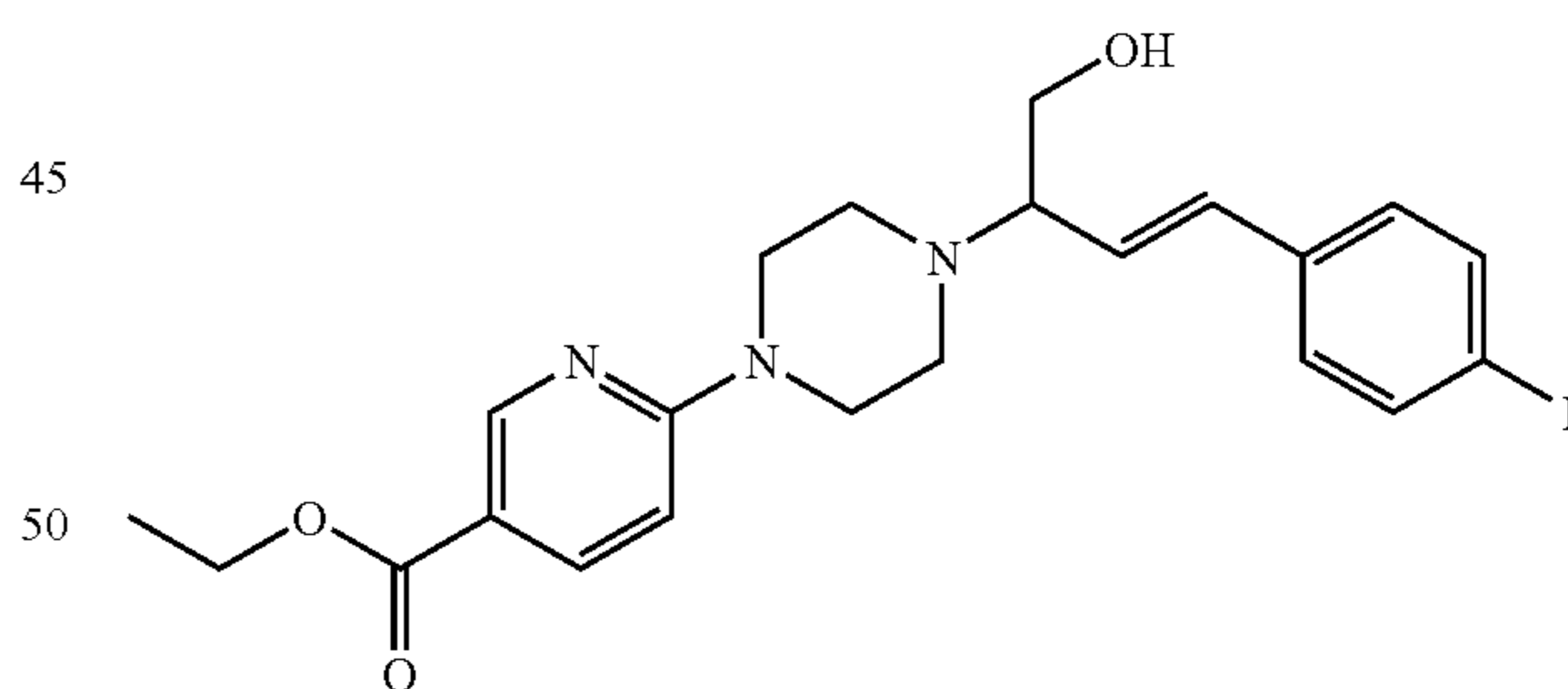
Interm. 25; Ex. [A7]
