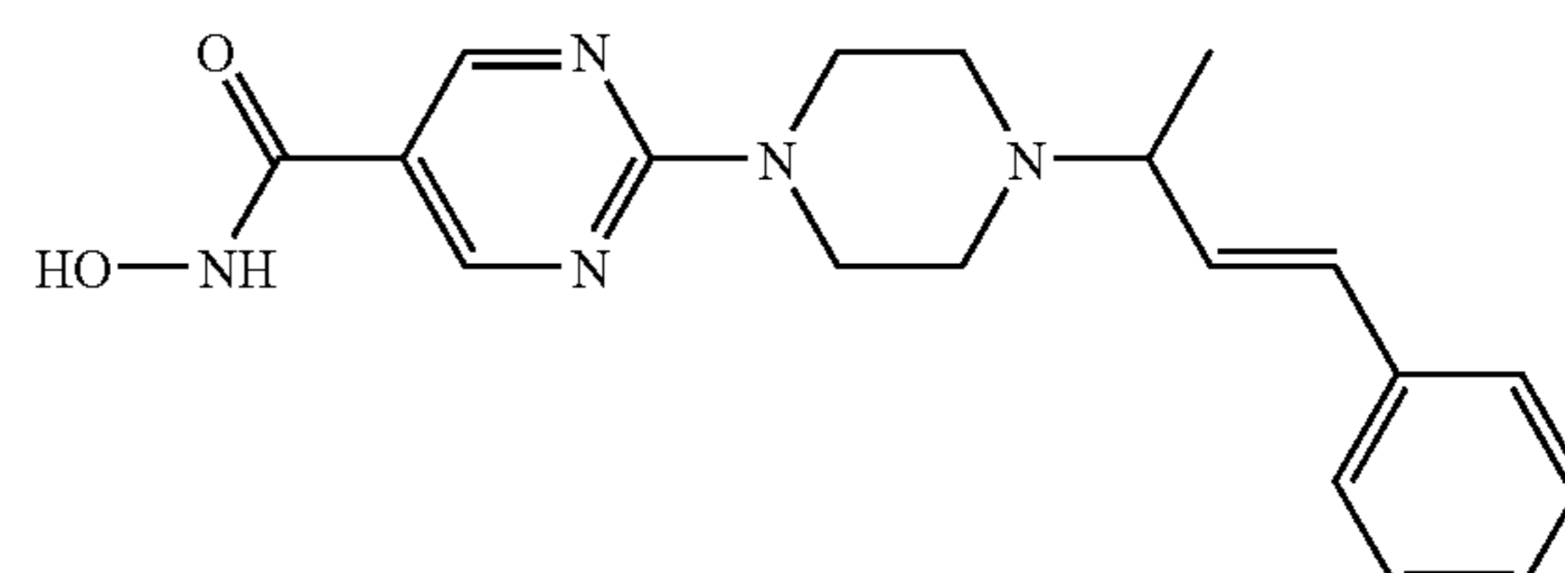
Compound No. 7; C 2 HF 3 O 2 ; (E)
