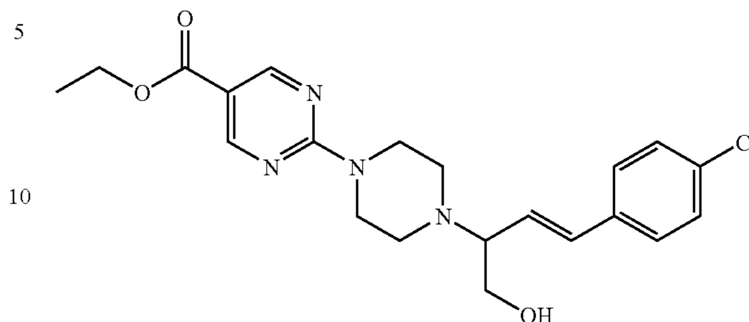
Interm. 4; Ex. [A1]; mp. 110.4° C.
