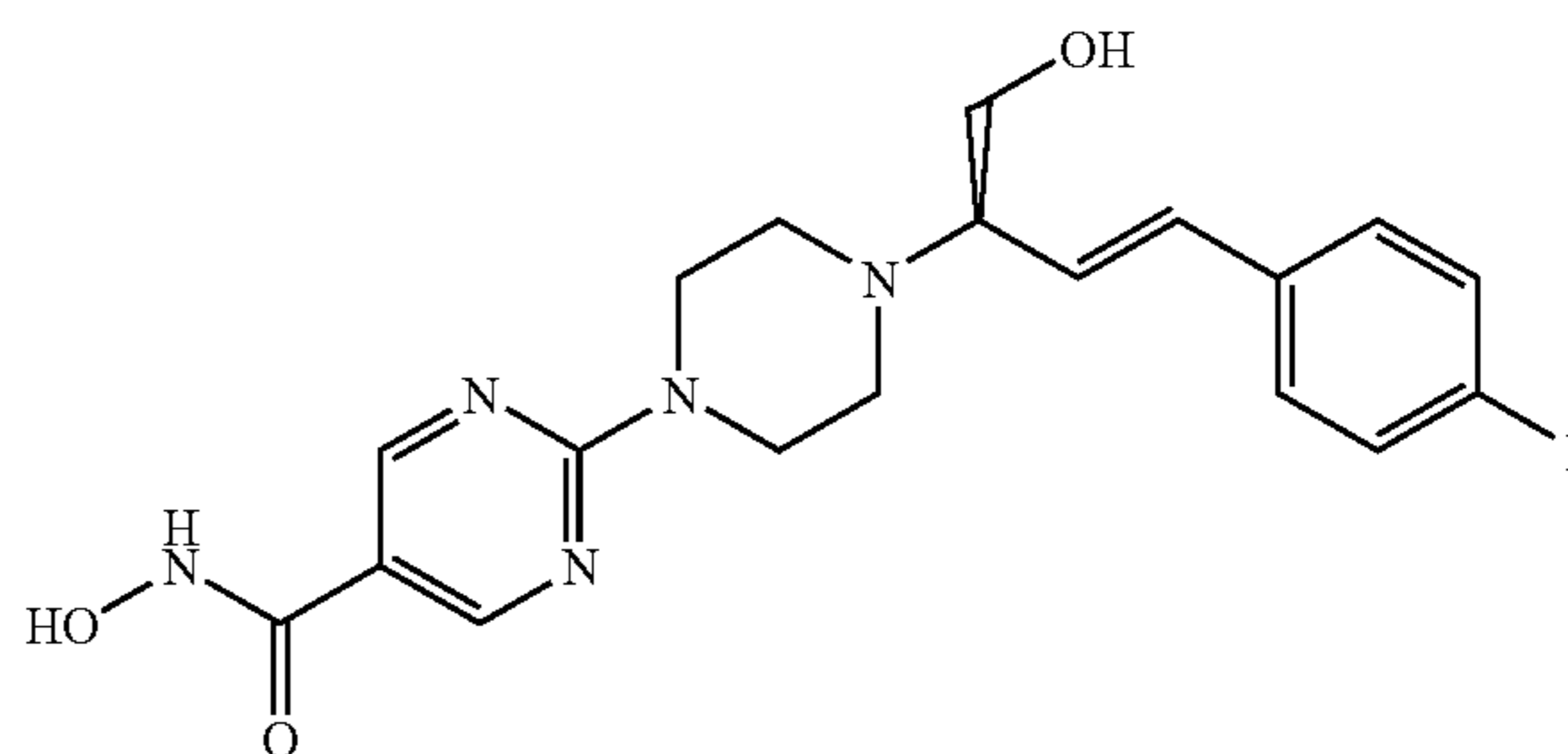
Compound No. 34; •HCl; enantiomer B
