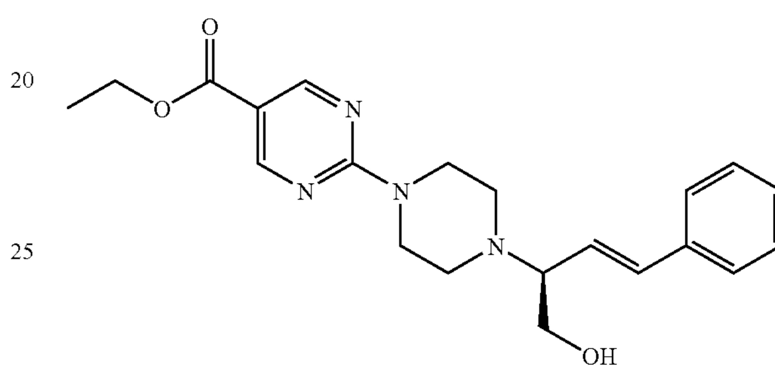
Interm. 44; Ex. [A1]; mp. 167° C. (enantiomer A)
