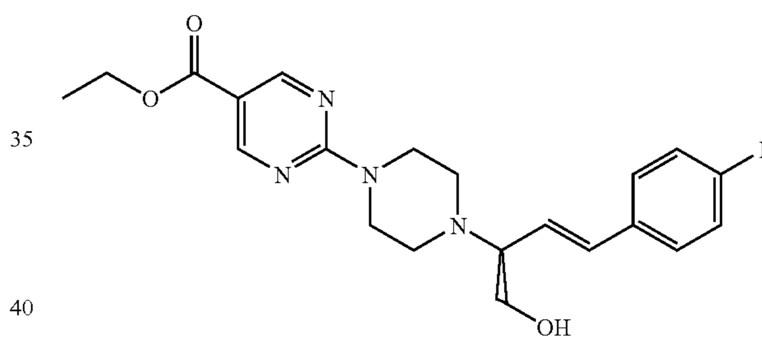
Interm. 45; Ex. [A1] (enantiomer B)
