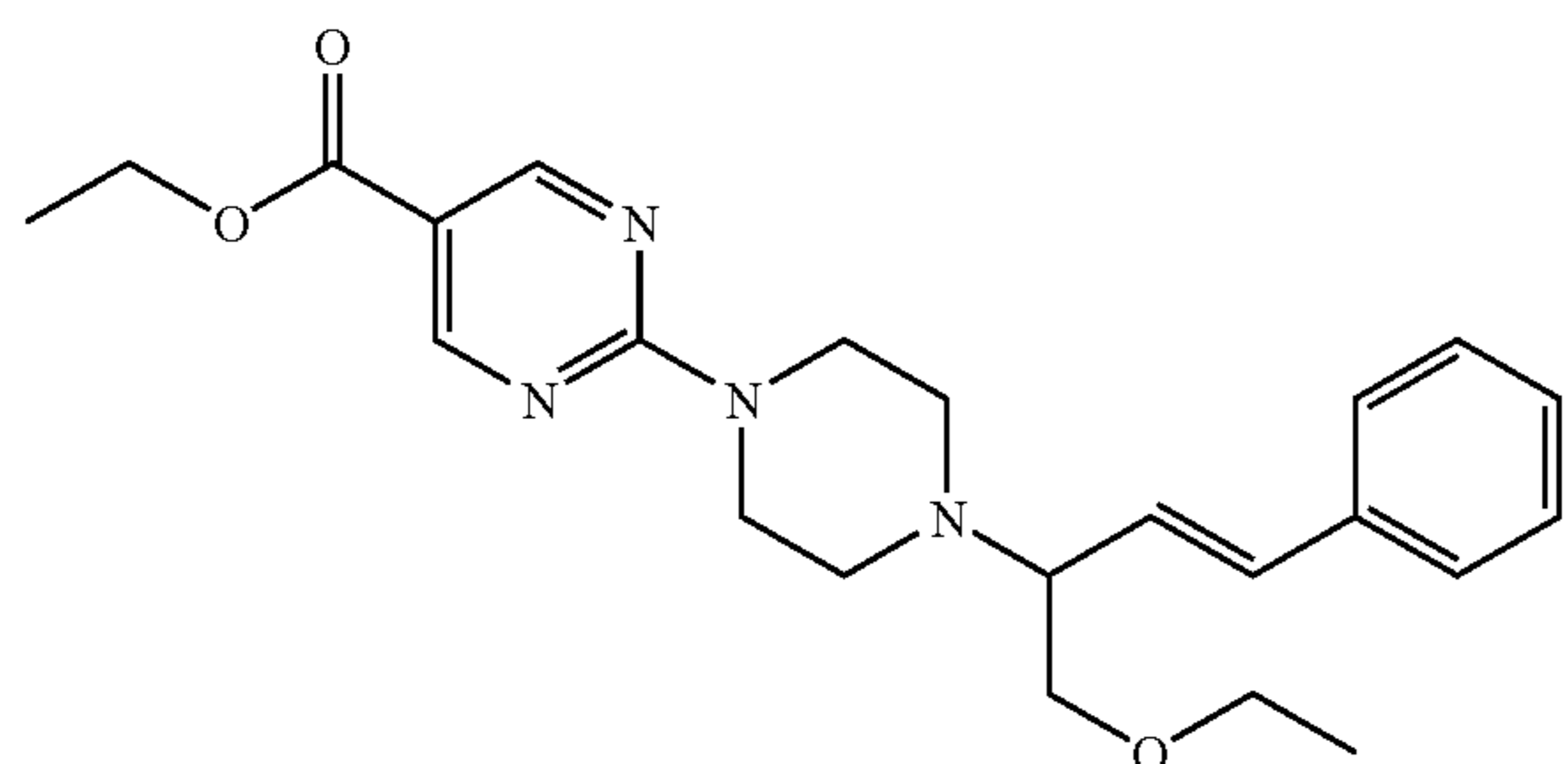
Co. No. 41; Ex. [A6]
