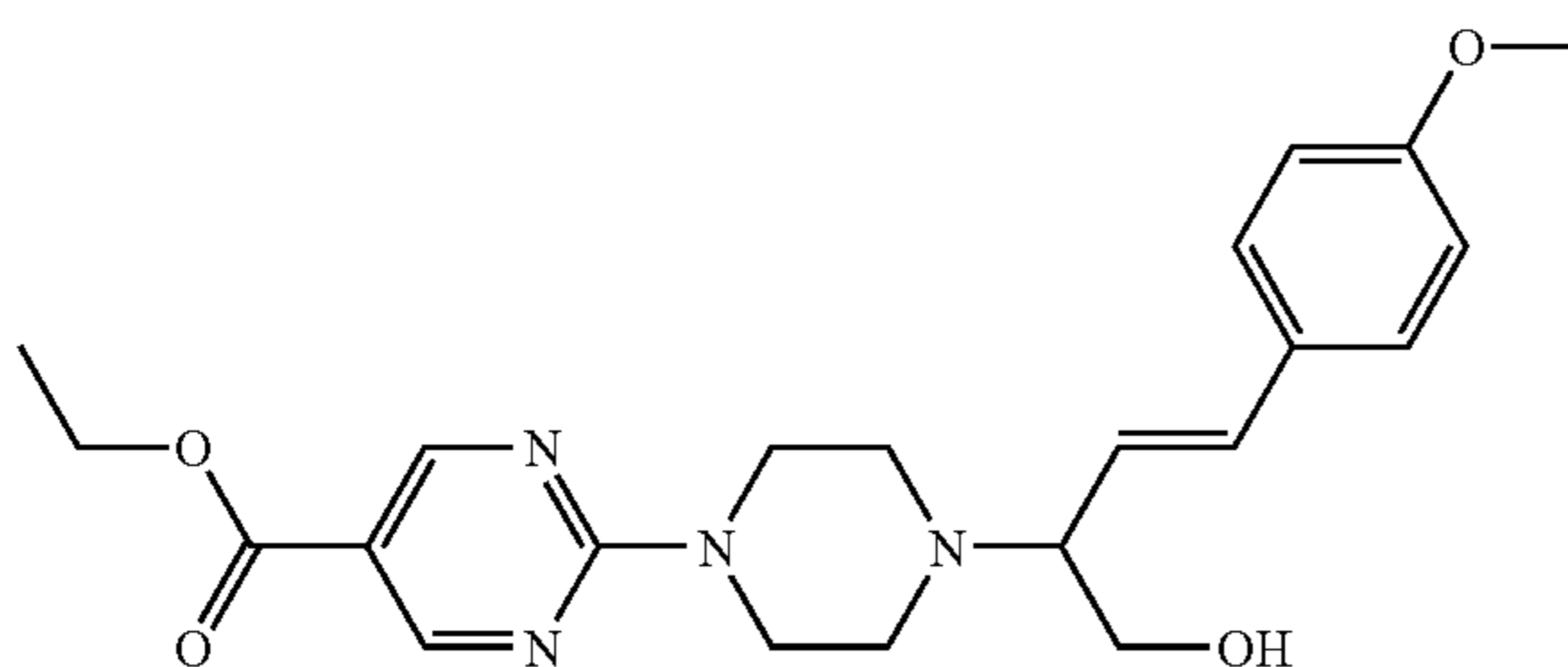
Interm. 9; Ex. [A1]
