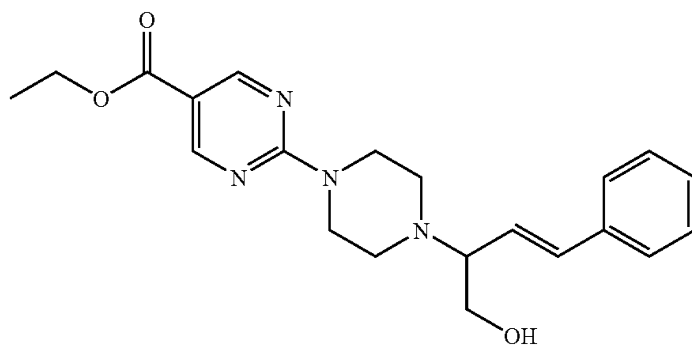
Interm. 1; Ex. [A1]; mp. 128° C.
