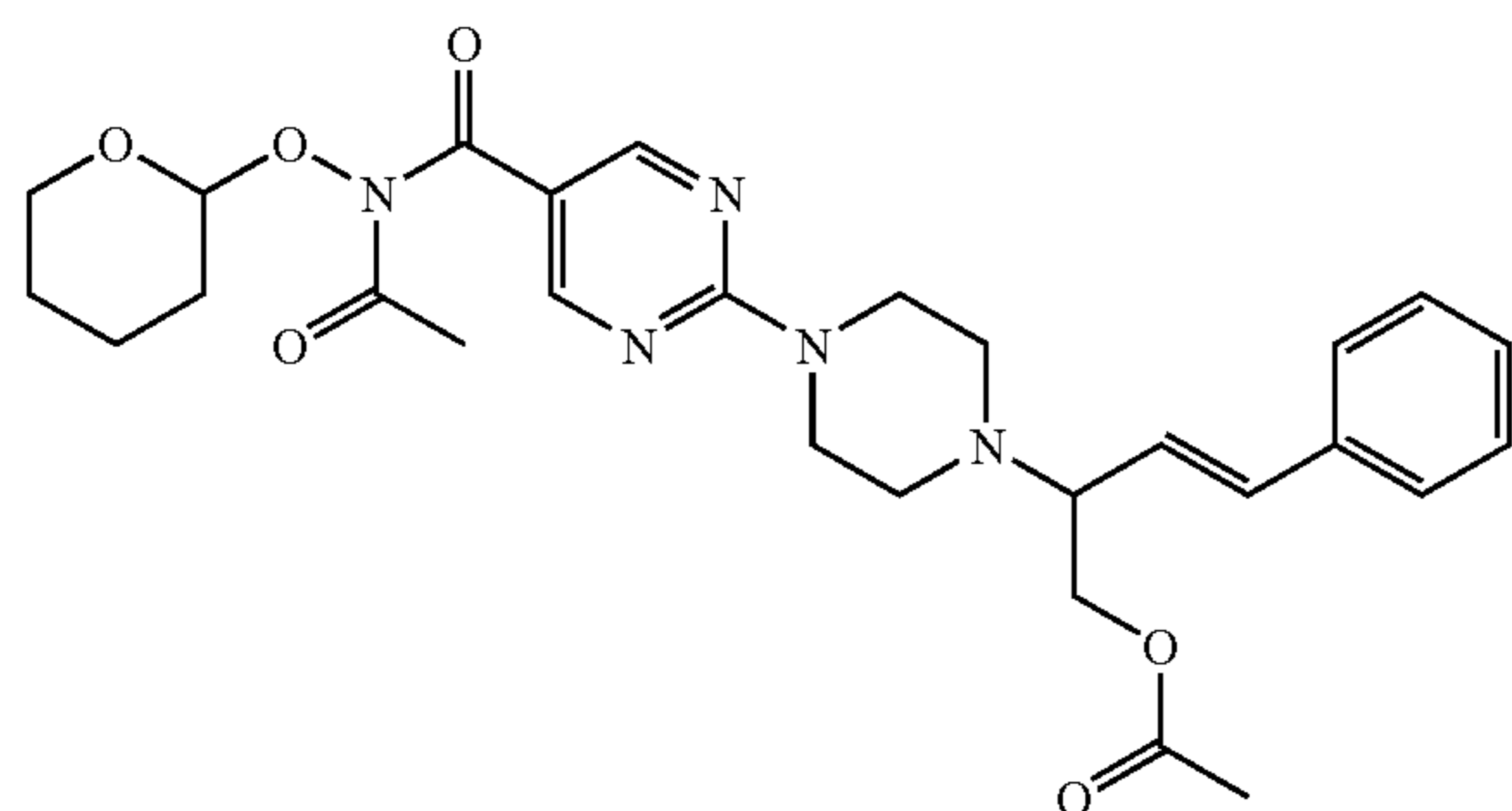
intermediate 28: free base intermediate 29: C 2 H 2 O 4 (1:1)
