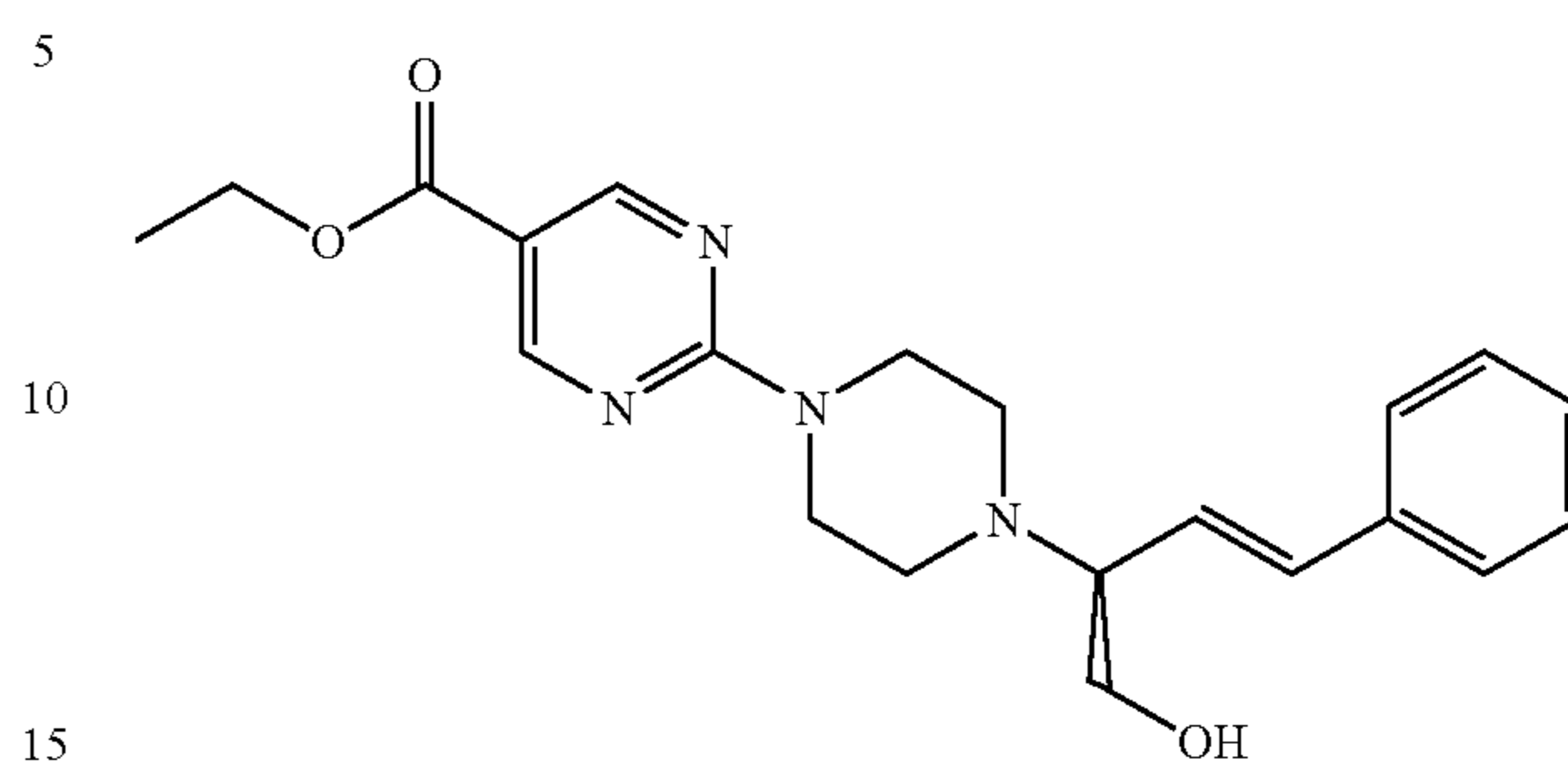
Interm. 43; Ex. [A1]; mp. 146° C. (enantiomer B)
