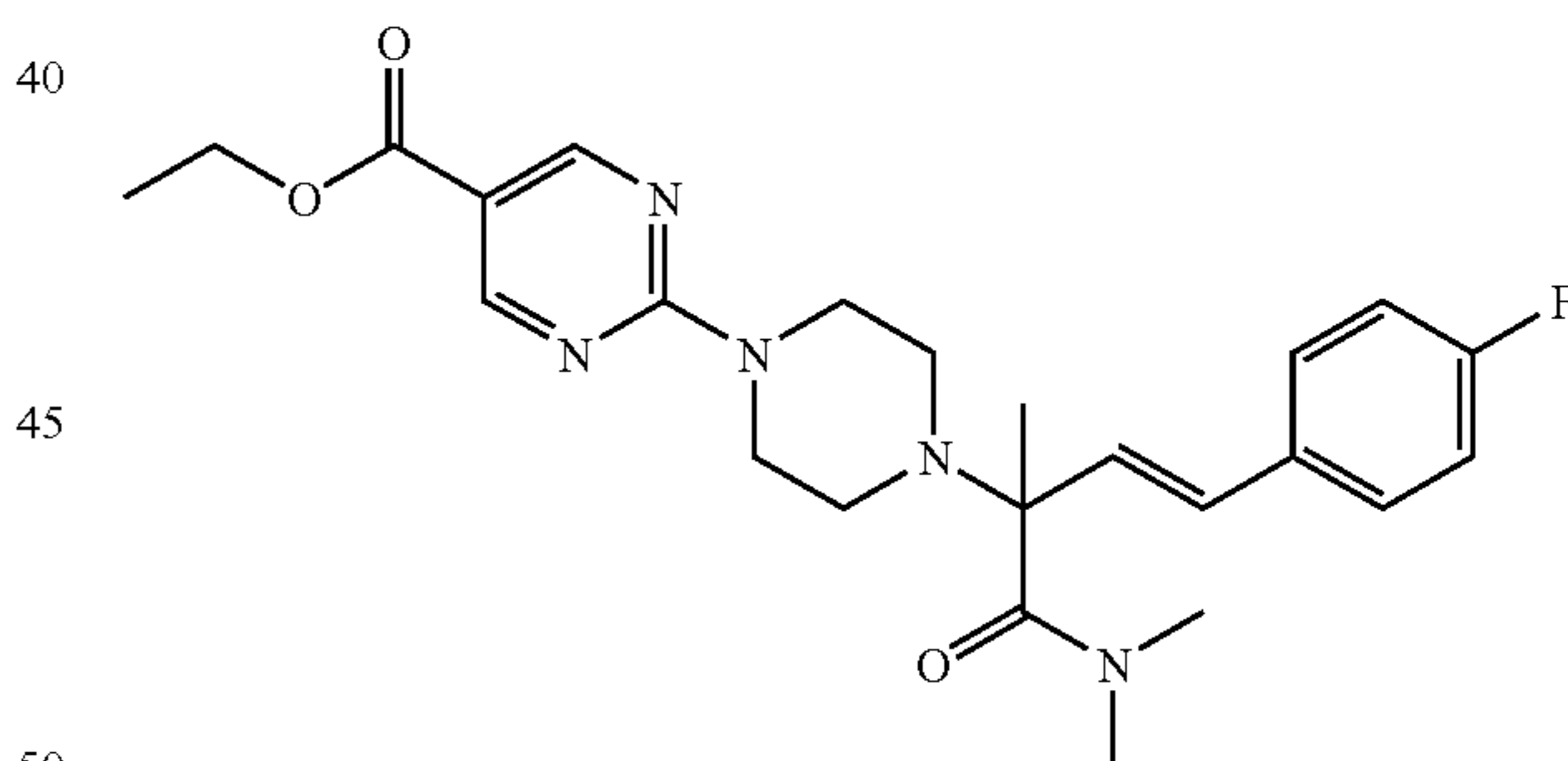
Interm. 19; Ex. [A5]; mp. 195° C.
