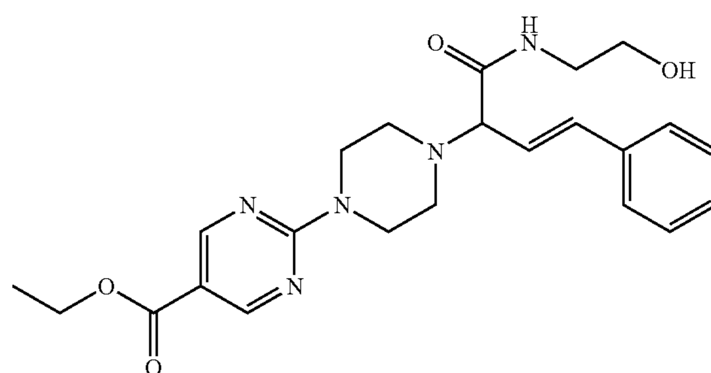
Interm. 36; Ex. [A5]; mp. 144° C.
