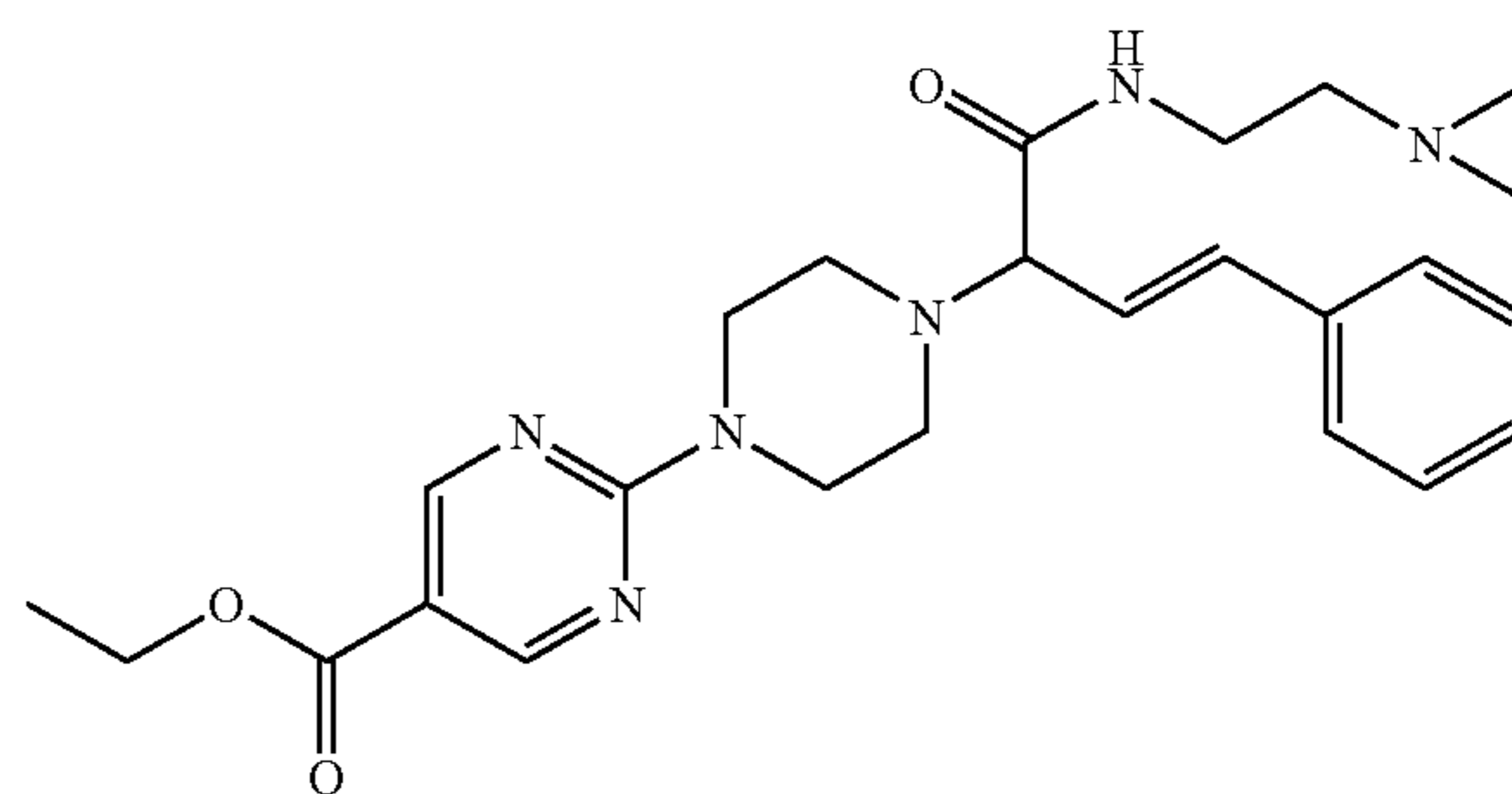
Interm. 35; Ex. [A5]
