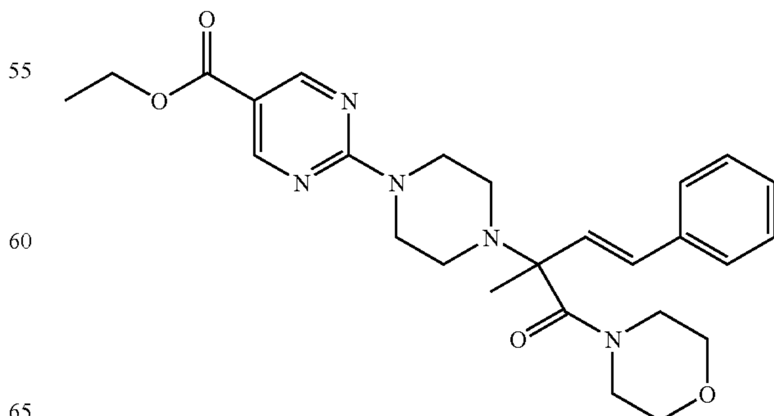
Interm. 30; Ex. [A5]
