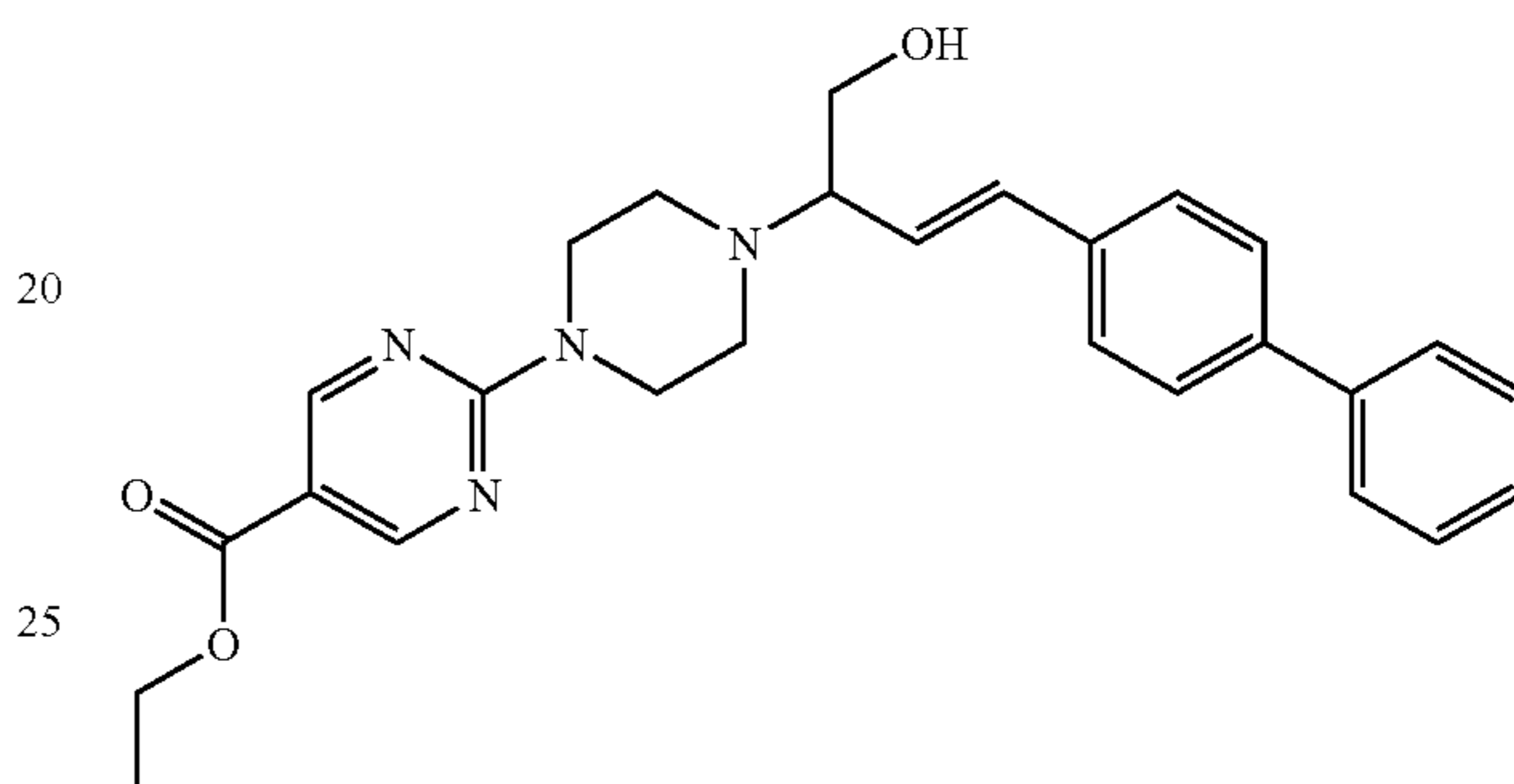
(E); interm. 10; Ex. [A1]; mp. 139° C.
