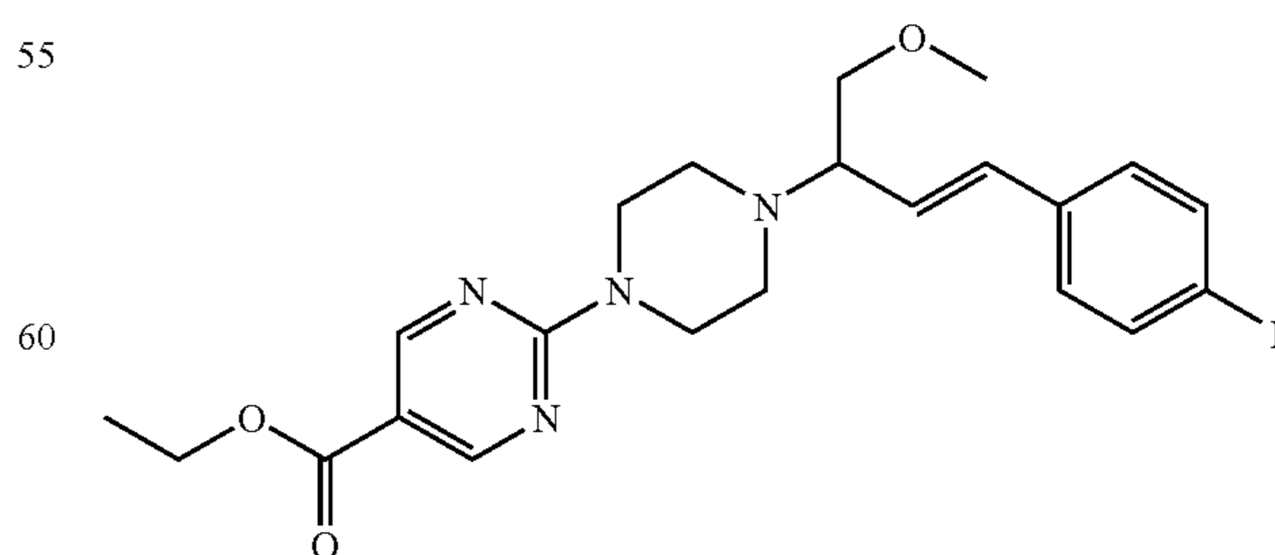
Interm. 46; Ex. [A6]
