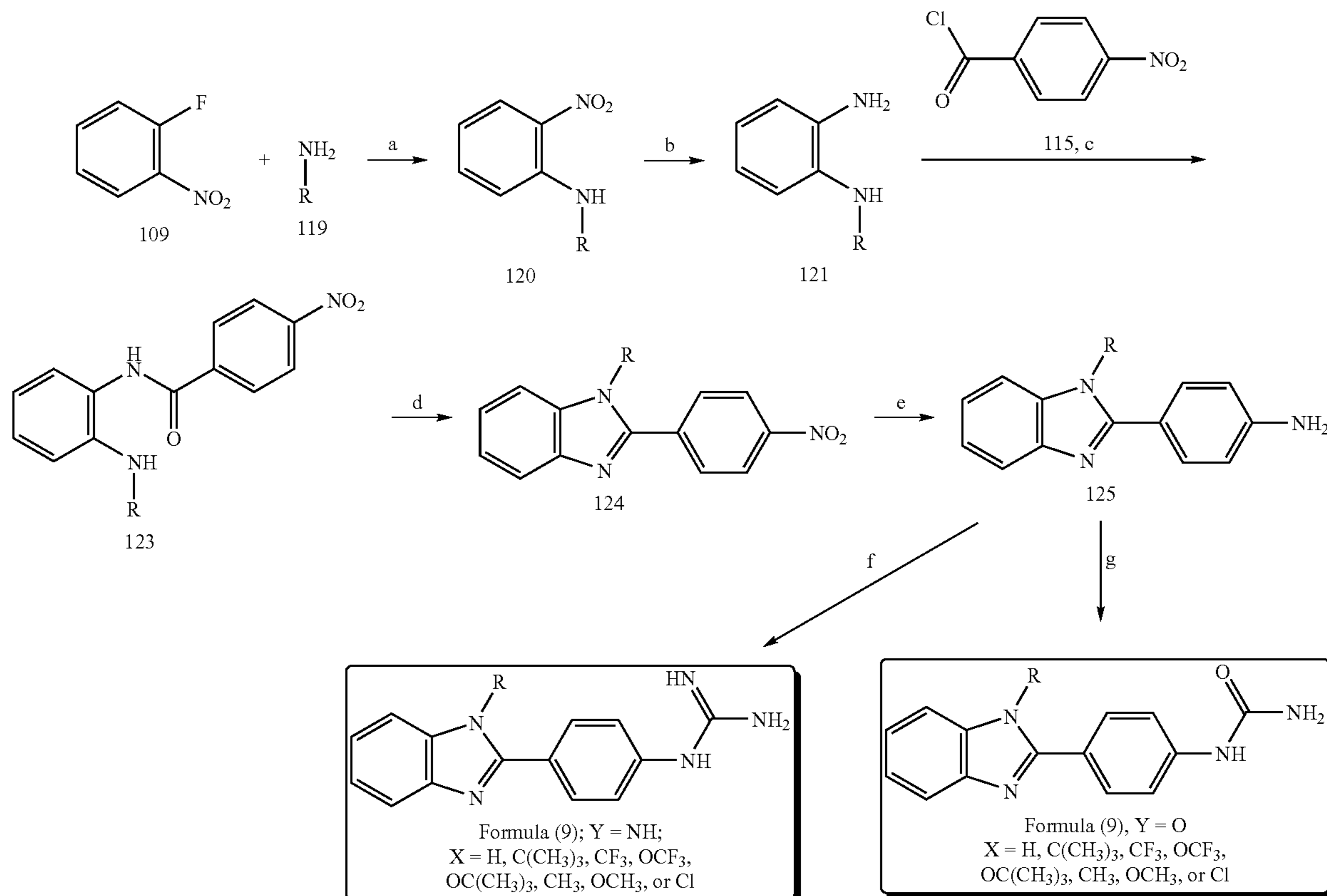
Scheme 4
