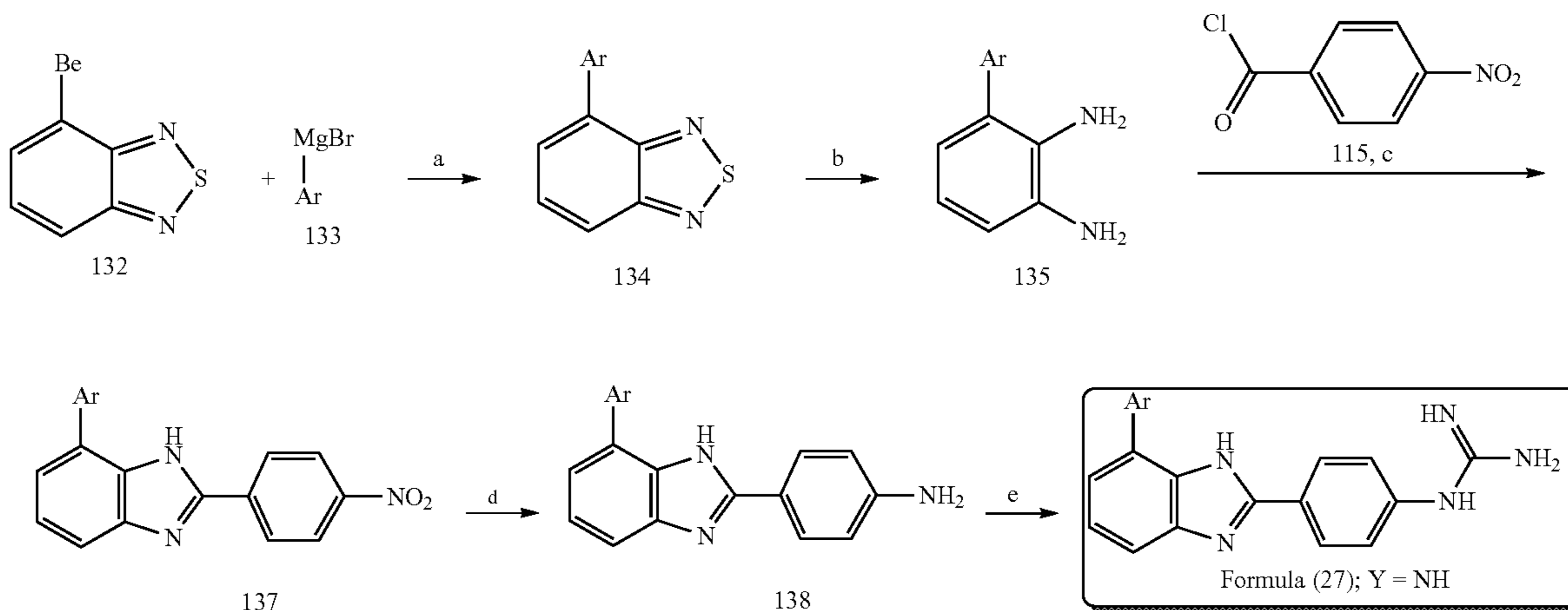
Scheme 9
