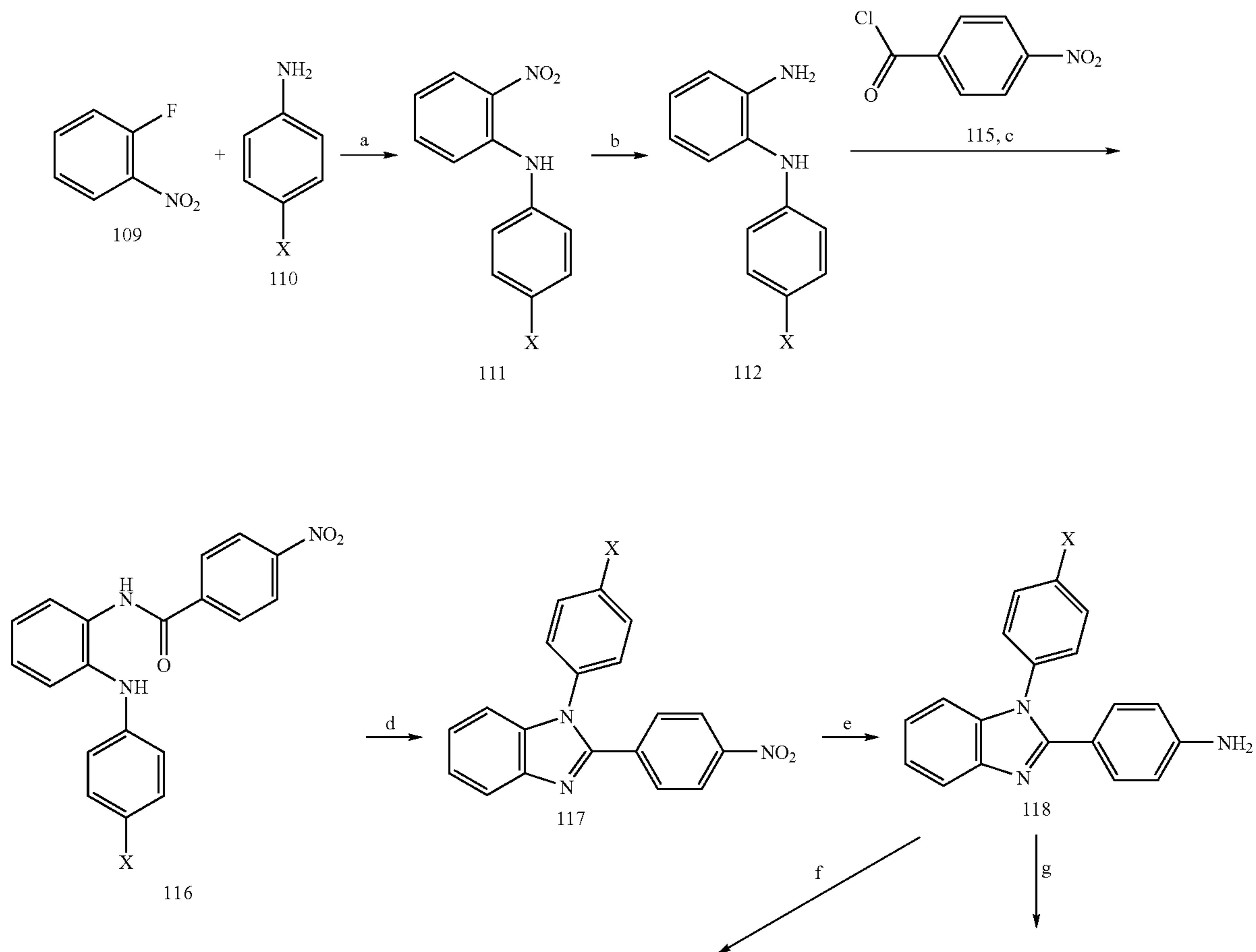
Scheme 2
