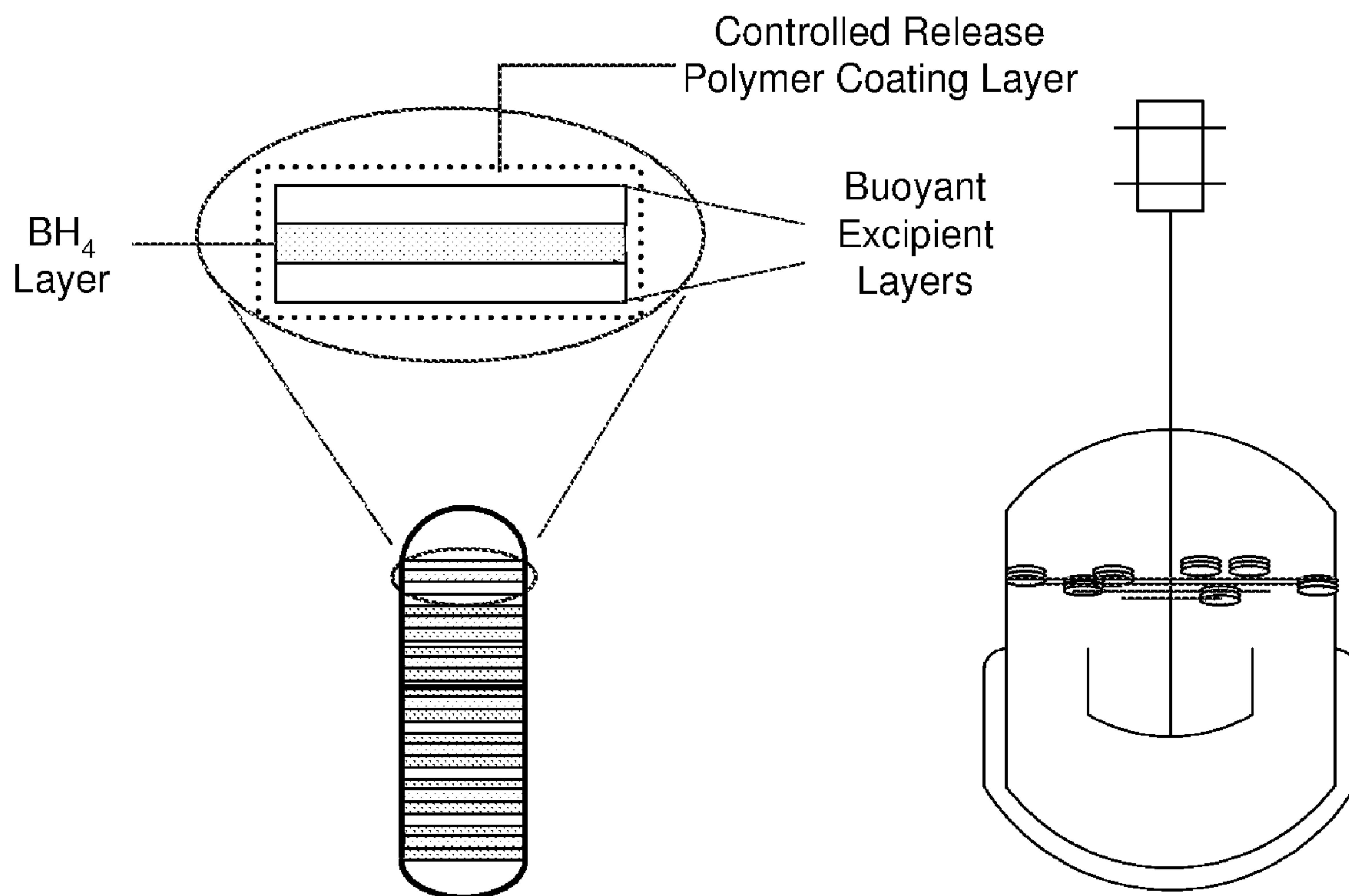
Schematic Diagram of Floating Dosage Form
