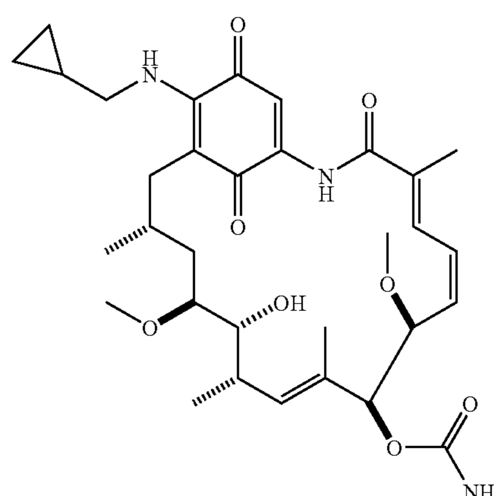
17-cyclopropylmethylaminogeldanamycin
