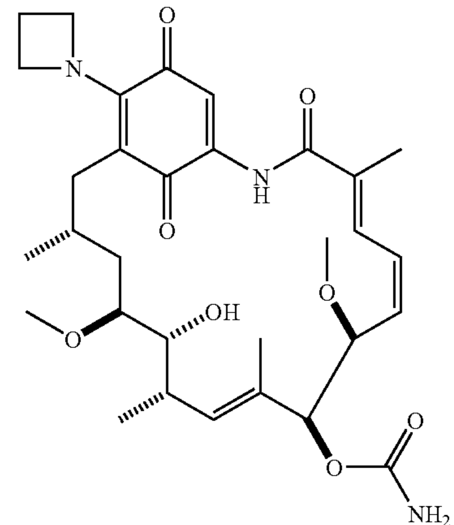
17-azetidinylgeldanamycin
