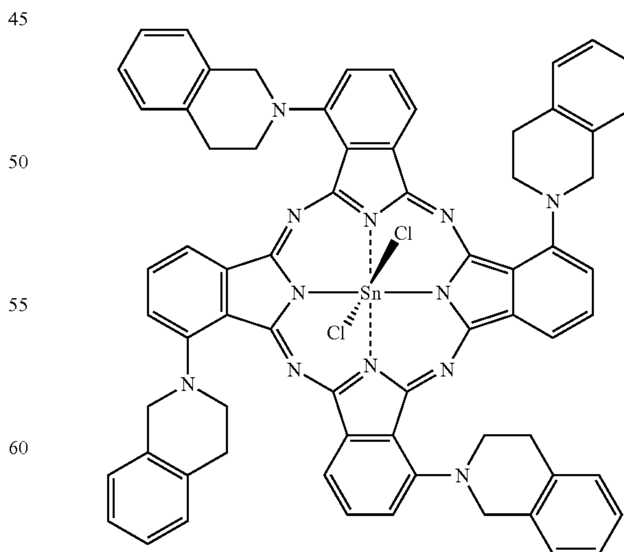
Tin(IV) tetrakis(1,2,3,4-tetrahydroisoquinolyl)phthalocyanine dichloride (11)
