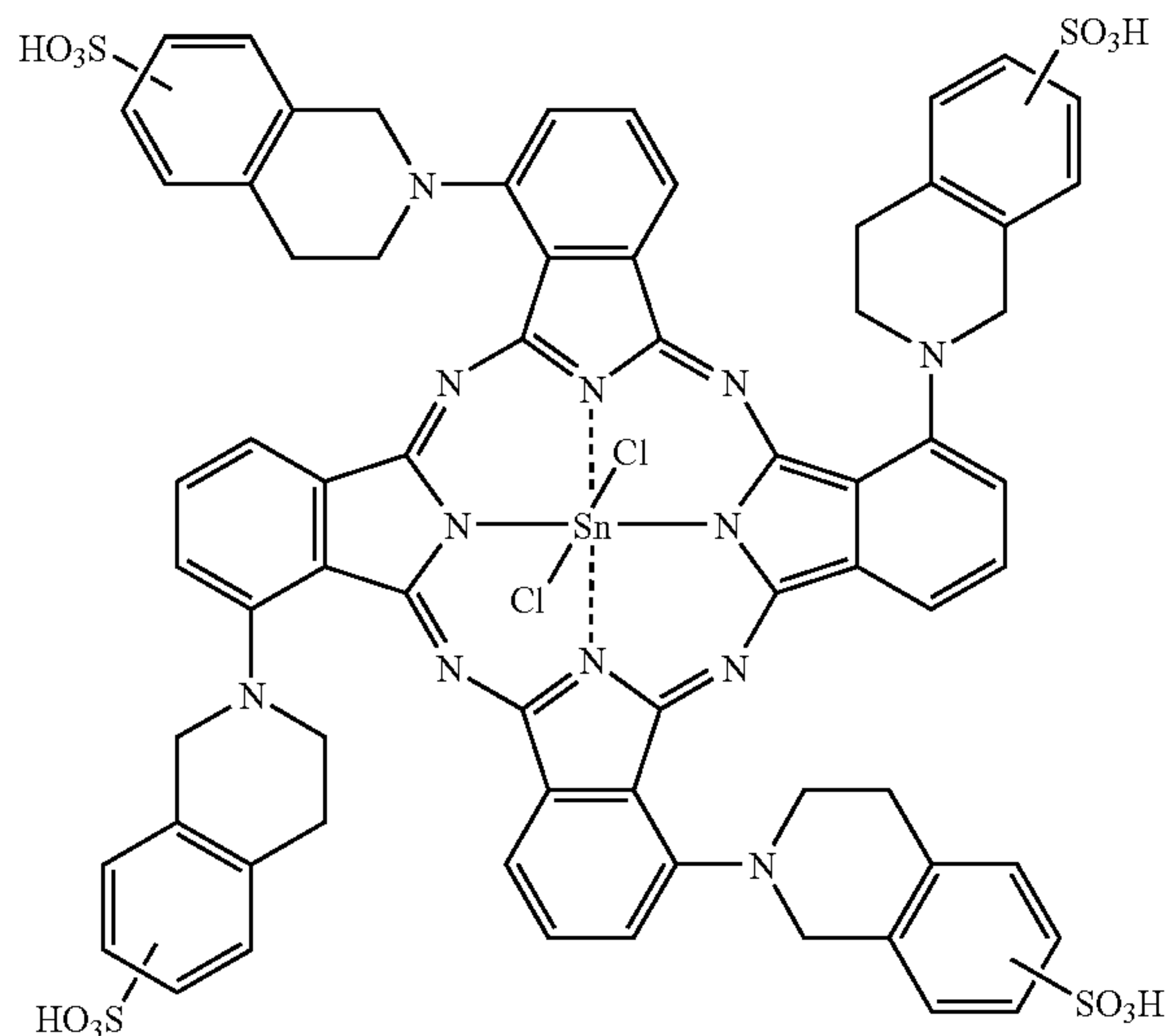
Sulfonation of tin(IV) tetrakis(1,2,3,4-tetrahydroisoquinolyl)phthalocyanine dichloride
