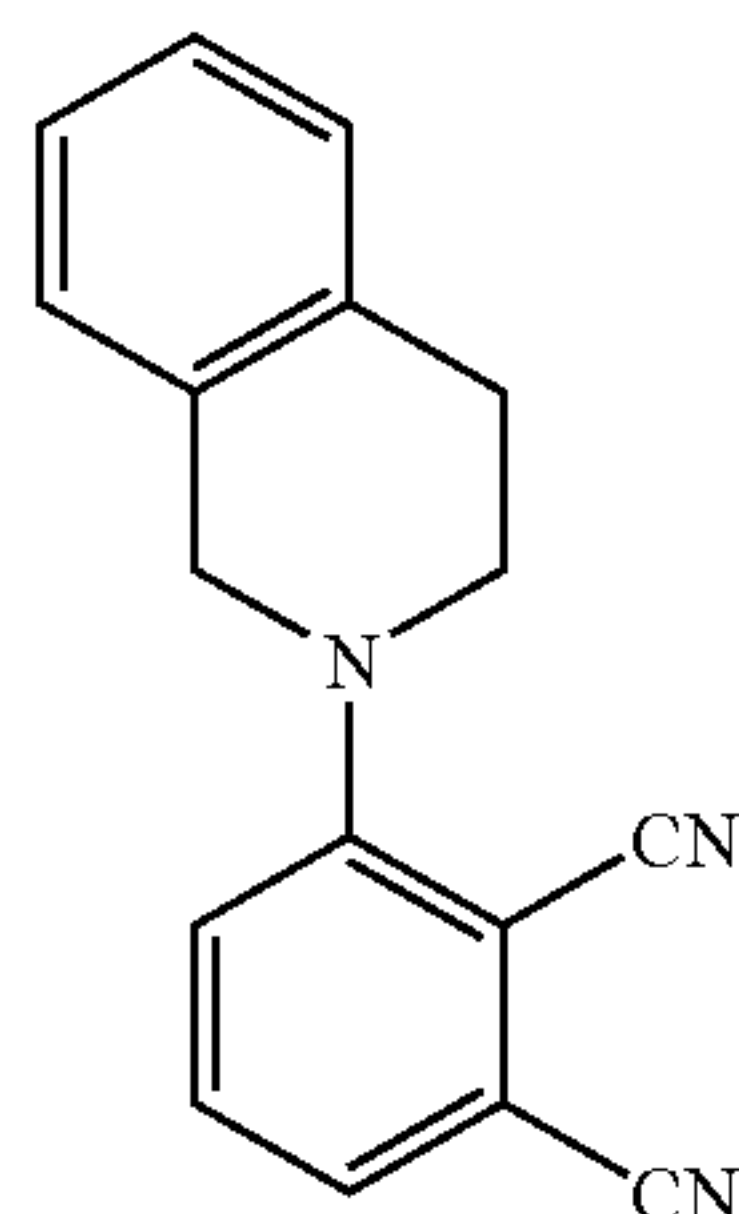
3-(1,2,3,4-Tetrahydroisoquinolyl)phthalonitrile (9)
