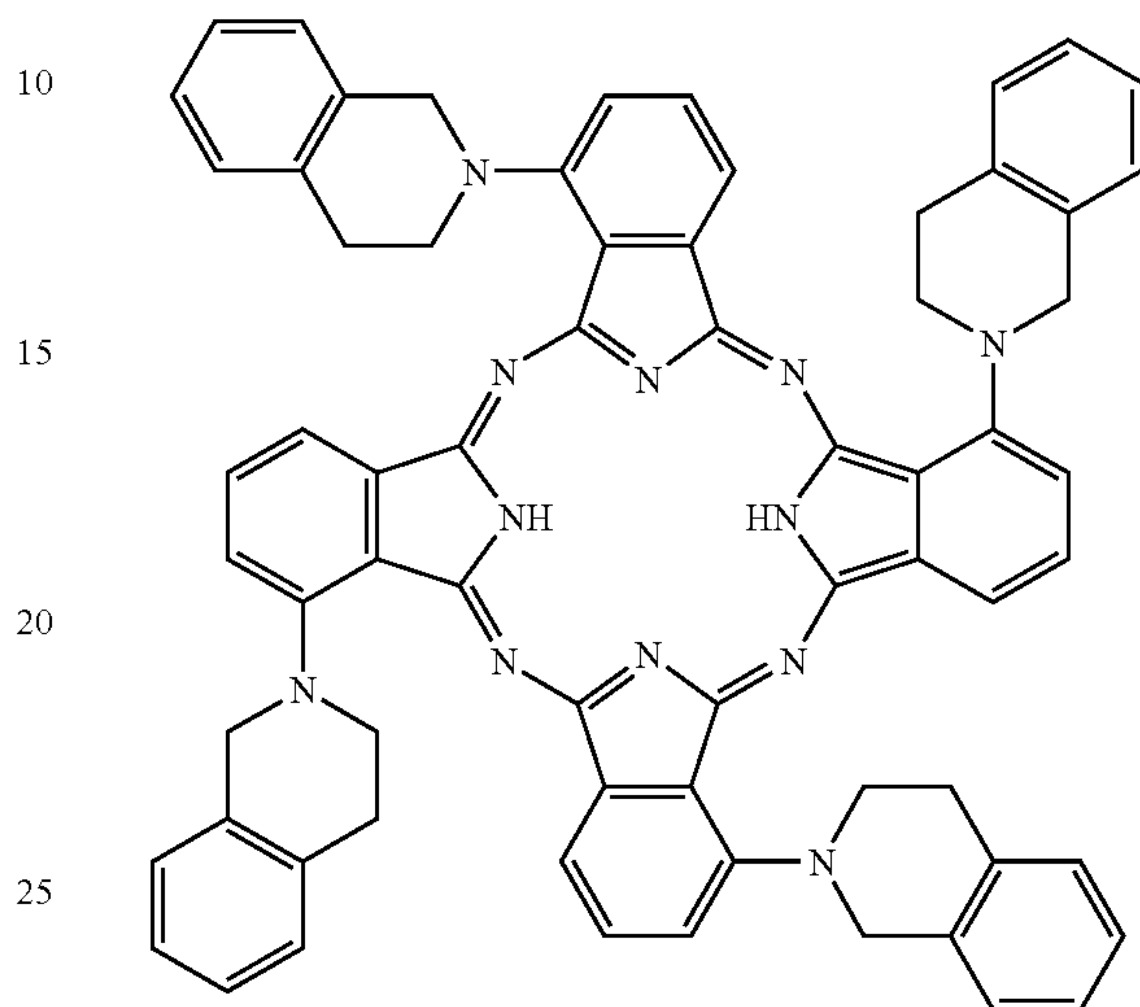
Tetrakis(1,2,3,4-tetrahydroisoquinolyl)phthalocyanine (10)
