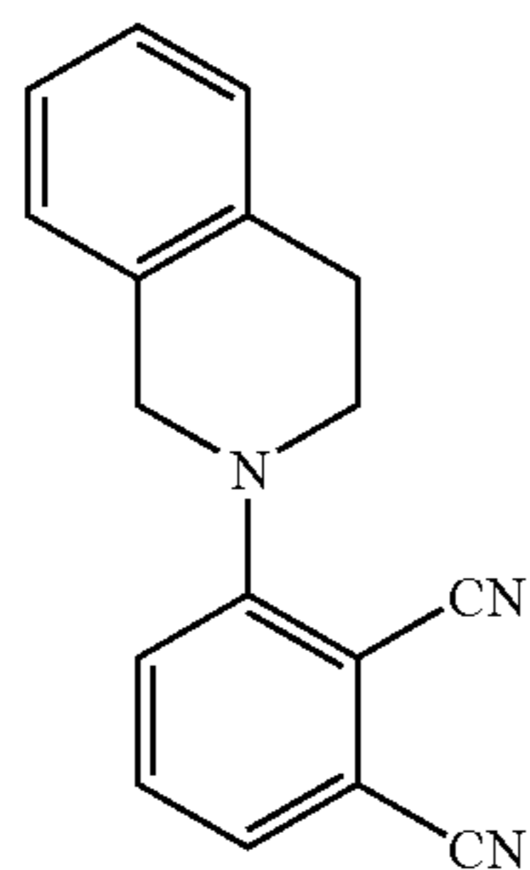
3-(1,2,3,4-Tetrahydroisoquinolyl)phthalonitrile (9)
