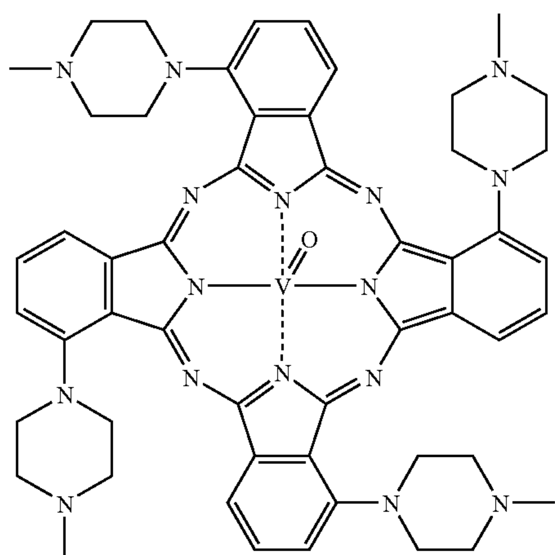
Oxovanadium(IV) tetrakis(N-methylpiperazino)phthalocyanine (8)
