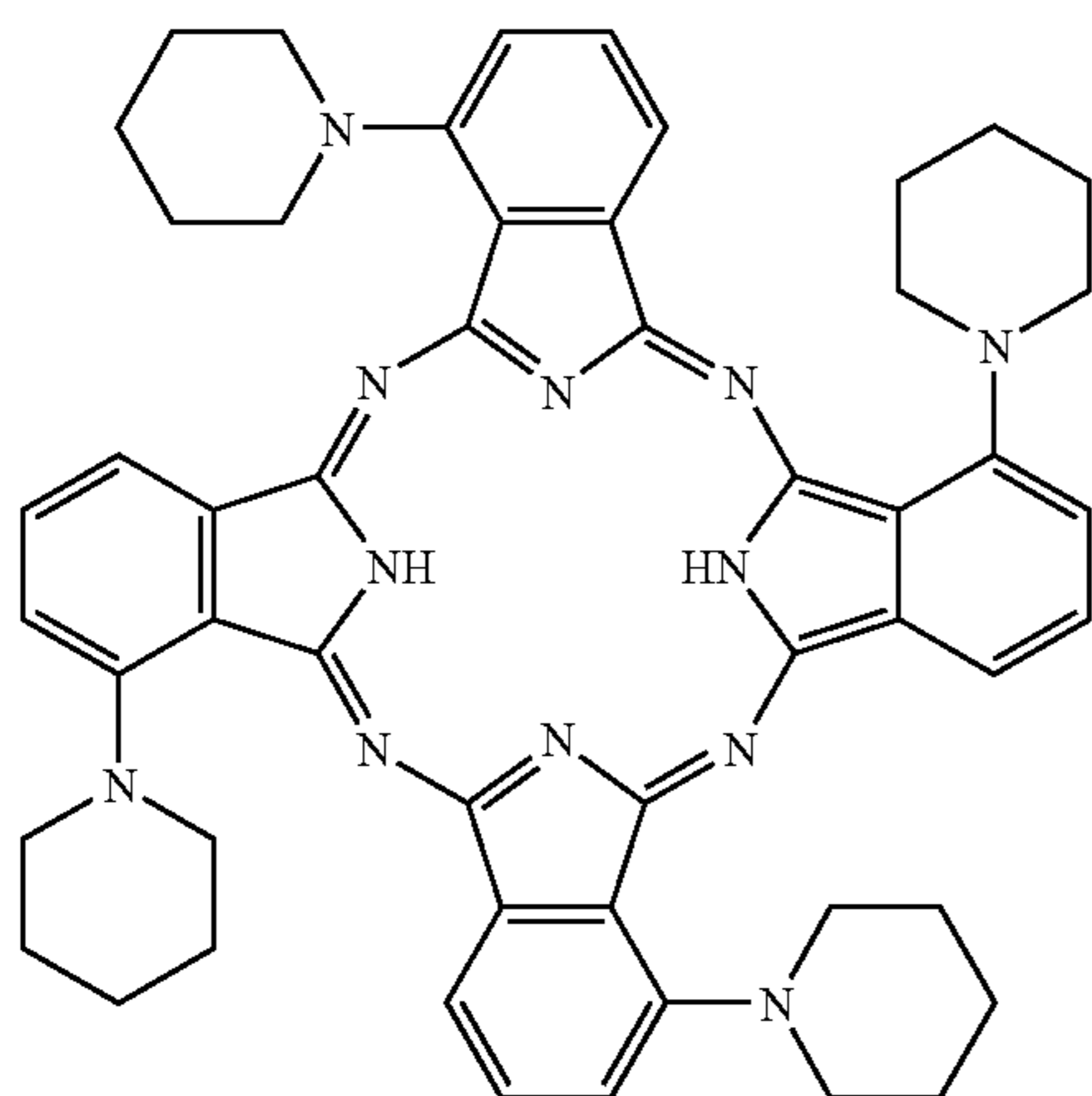
Tetrapiperidinophthalocyanine (4)
