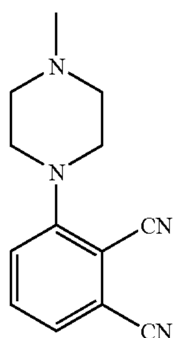
3-(N-methylpiperazino)phthalonitrile (5)
