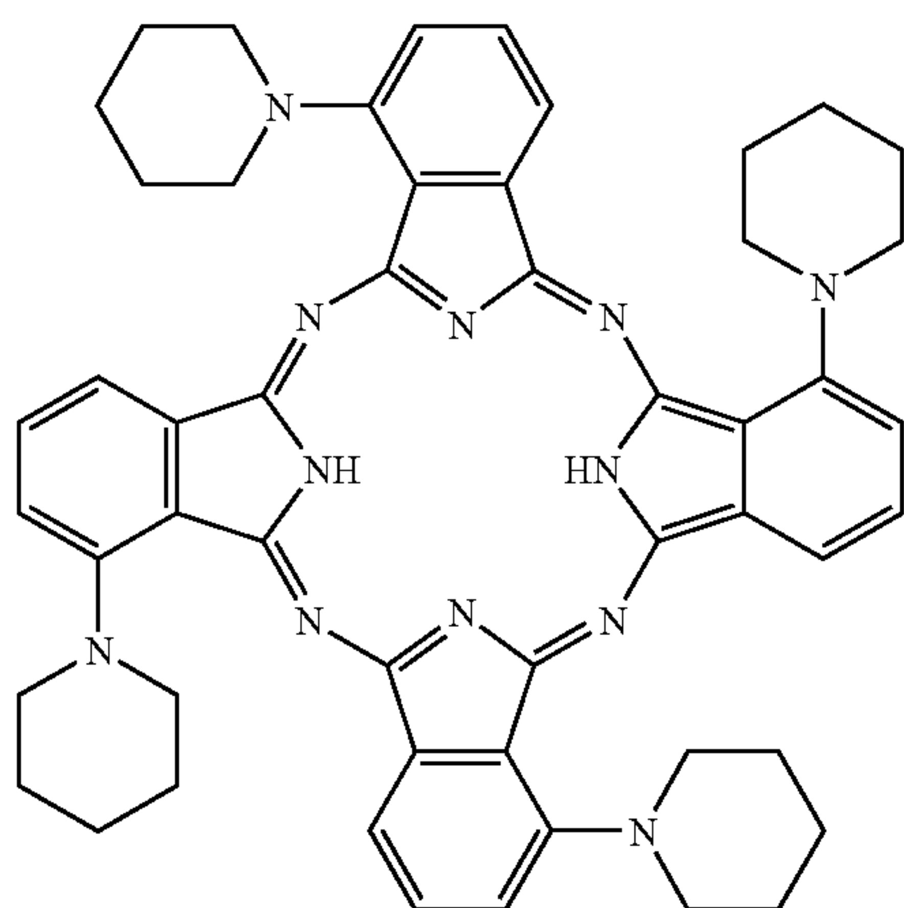
Tetrapiperidinophthalocyanine (4)
