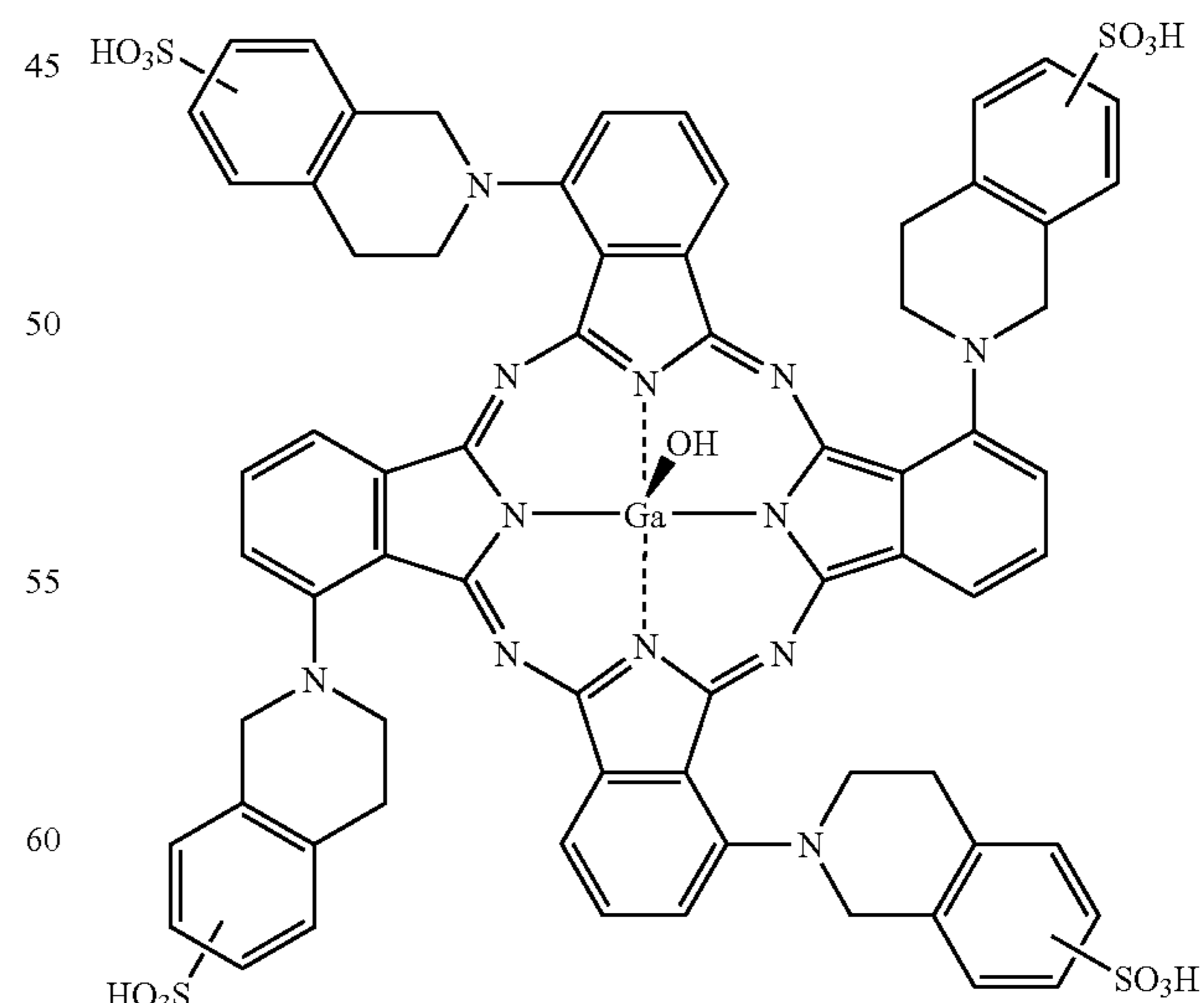
Sulfonation of gallium(III) tetrakis(1,2,3,4-tetrahydroisoquinolyl)phthalocyanine hydroxide
