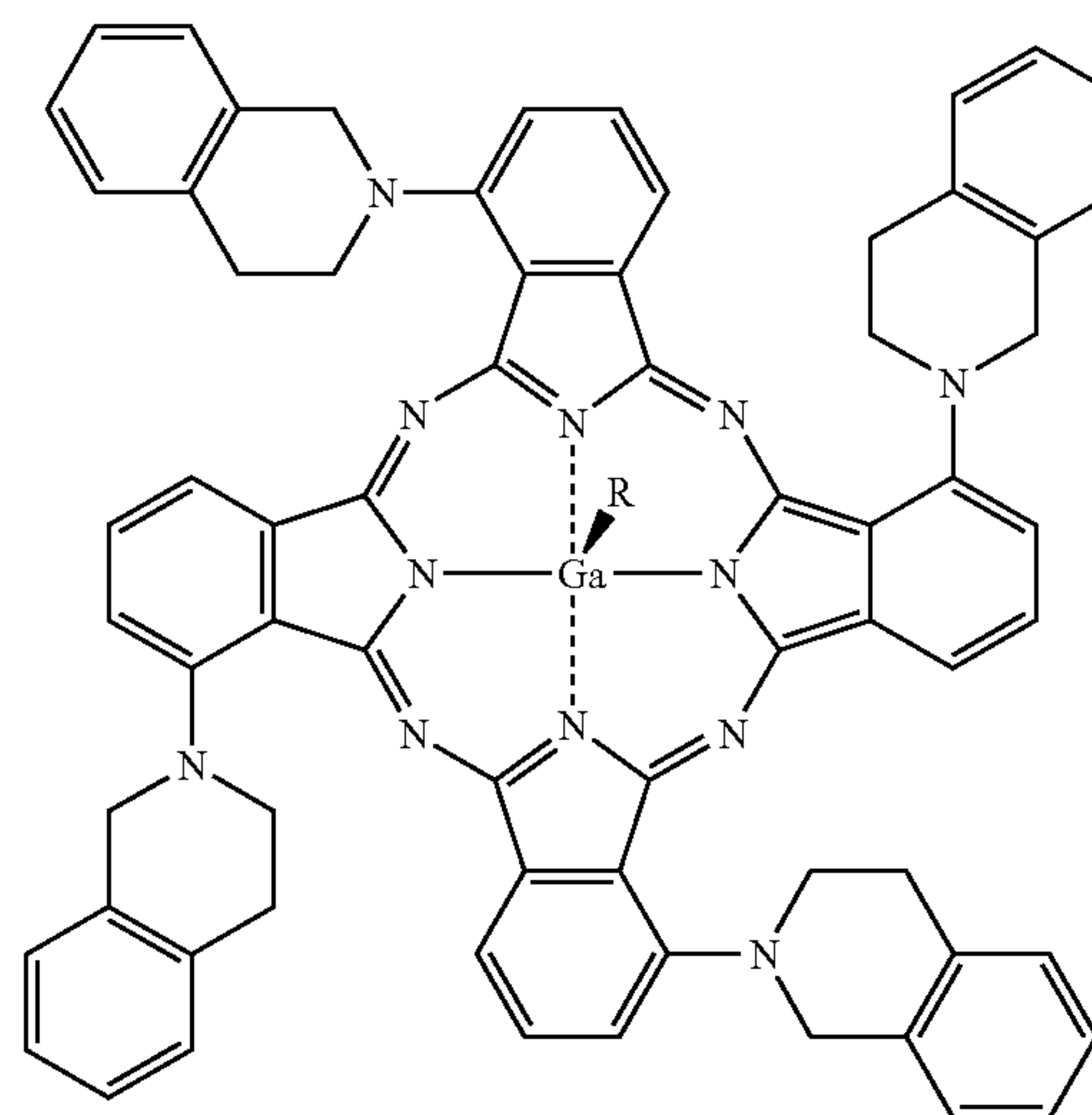
Gallium(III) tetrakis(1,2,3,4-tetrahydroisoquinolyl)phthalocyanine acetylacetonate (13)
