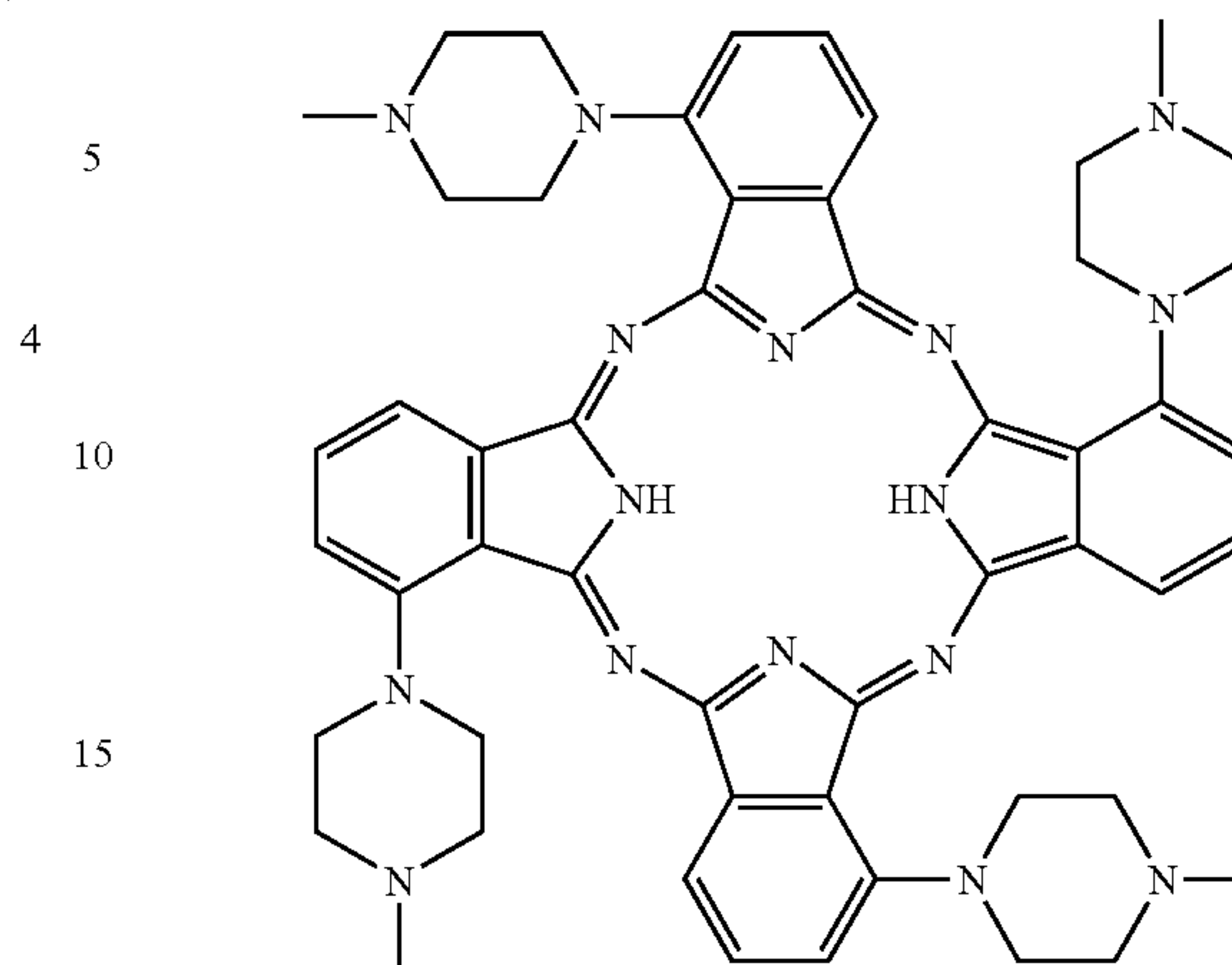
Tetrakis(N-methylpiperazino)phthalocyanine (6)
