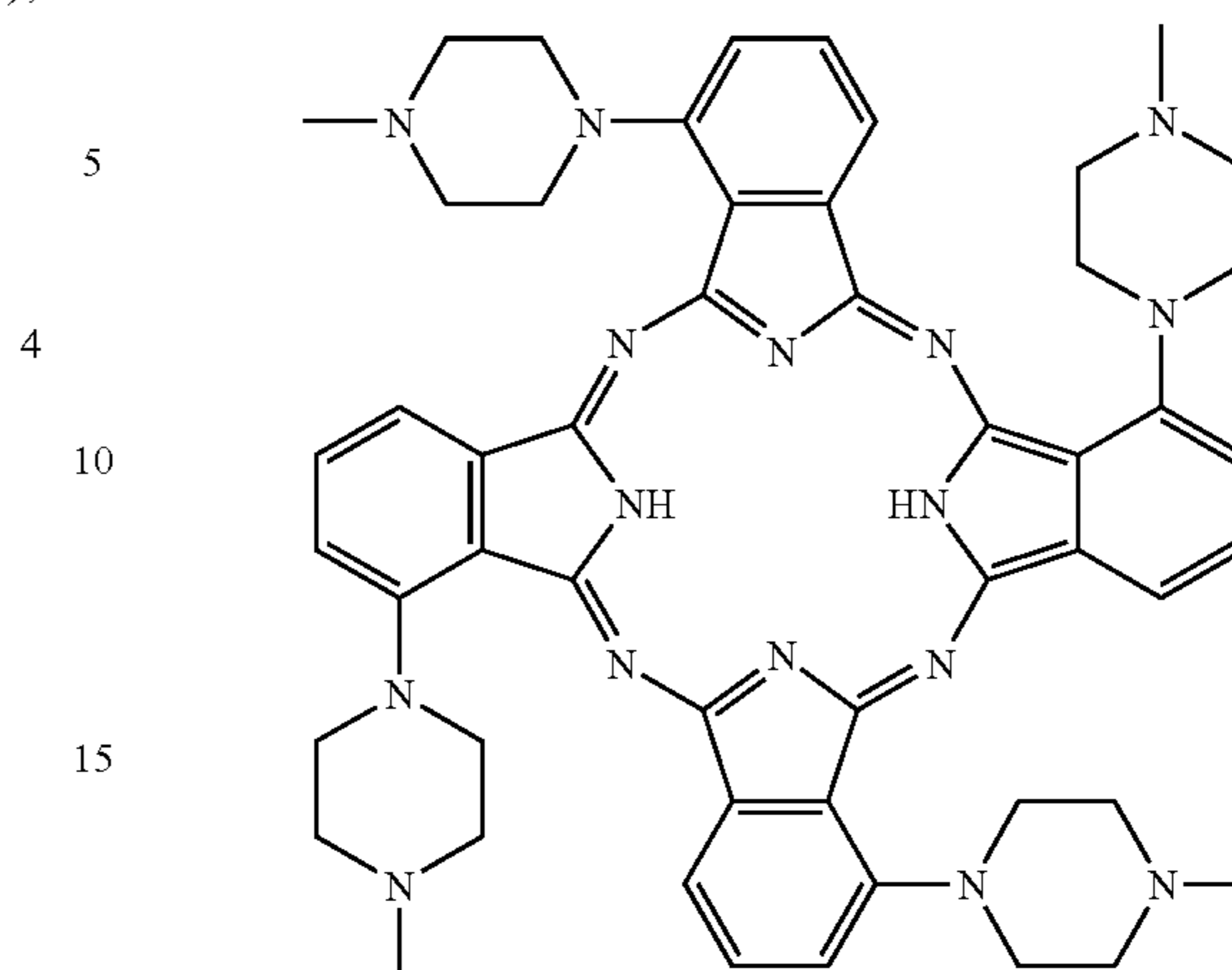
Tetrakis(N-methylpiperazino)phthalocyanine (6)
