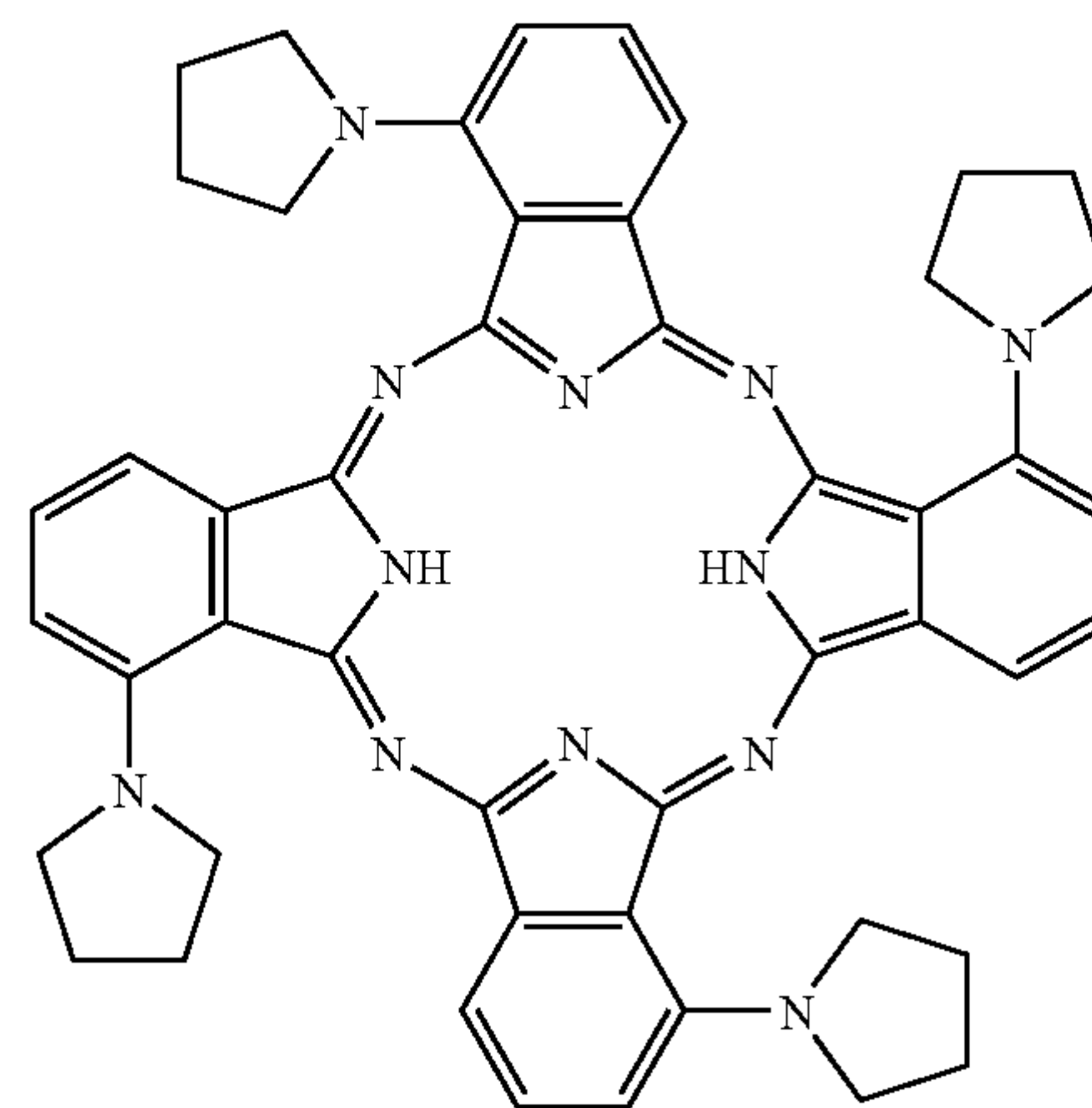
Tetrapyrrolidinophthalocyanine (2)
