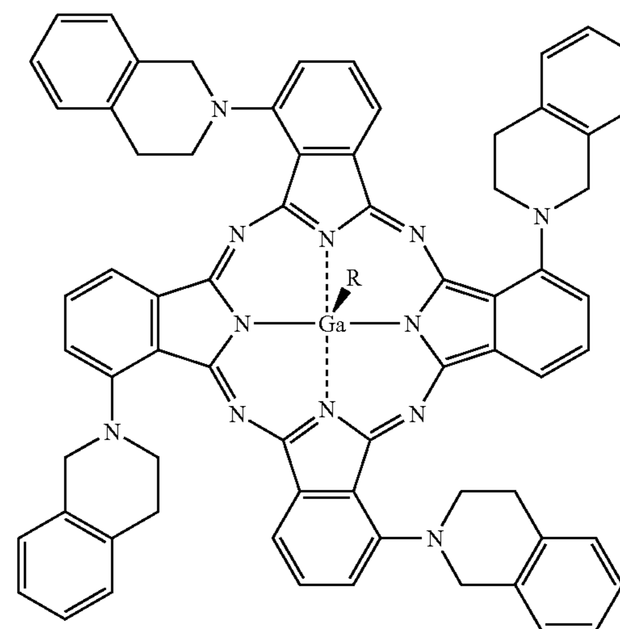
Gallium(III) tetrakis(1,2,3,4-tetrahydroisoquinolyl)phthalocyanine acetylacetonate (13)
