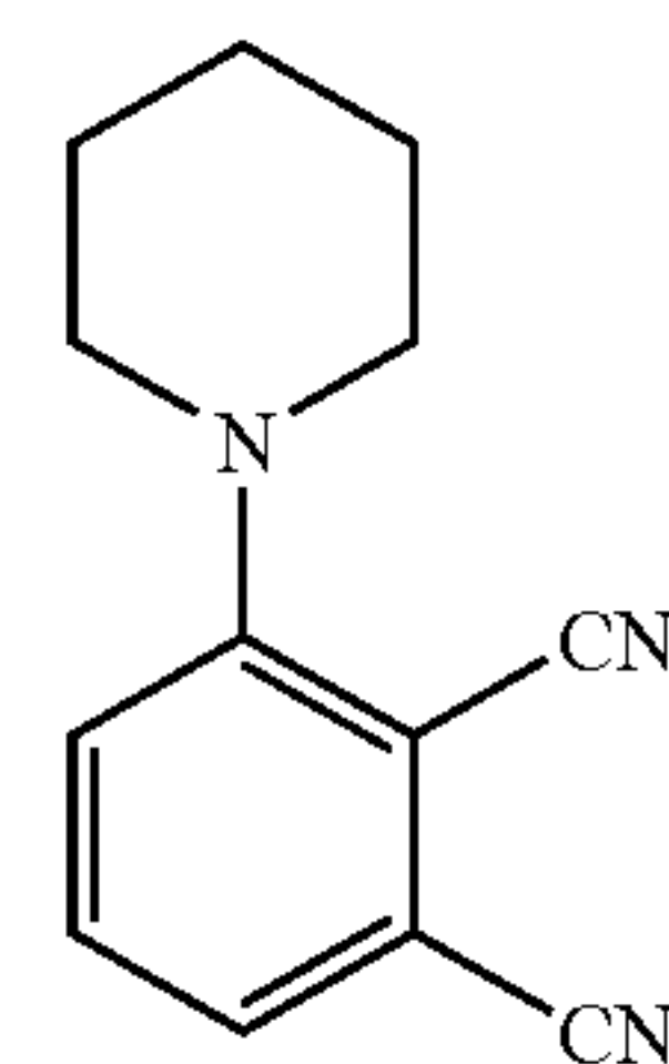
3-Piperidinophthalonitrile (3)
