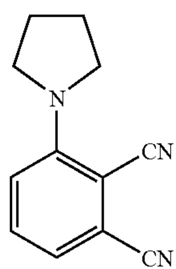
3-Pyrrolidinophthalonitrile (1)
