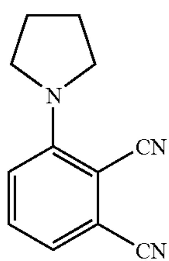
3-Pyrrolidinophthalonitrile (1)
