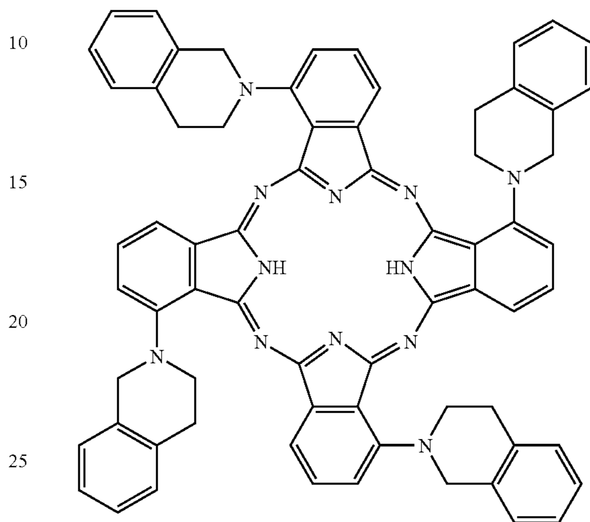
Tetrakis(1,2,3,4-tetrahydroisoquinolyl)phthalocyanine (10)
