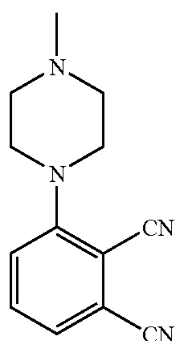
3-(N-methylpiperazino)phthalonitrile (5)
