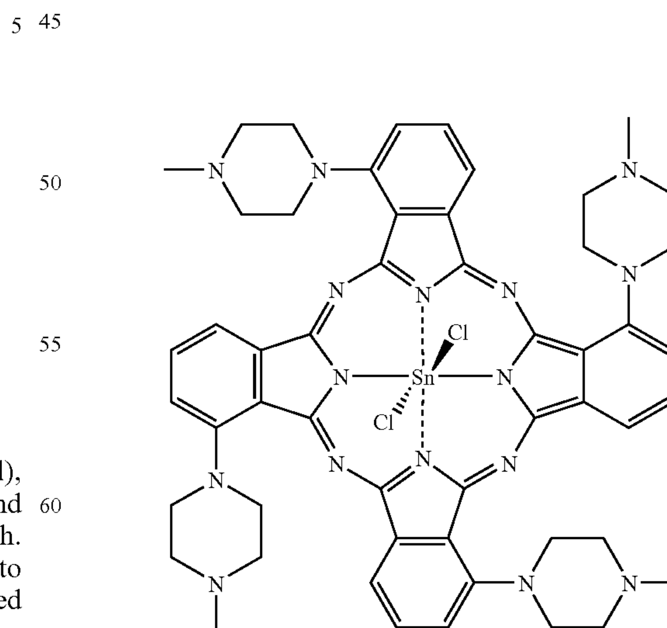
Tin(IV) tetrakis(N-methylpiperazino)phthalocyanine dichloride (7)
