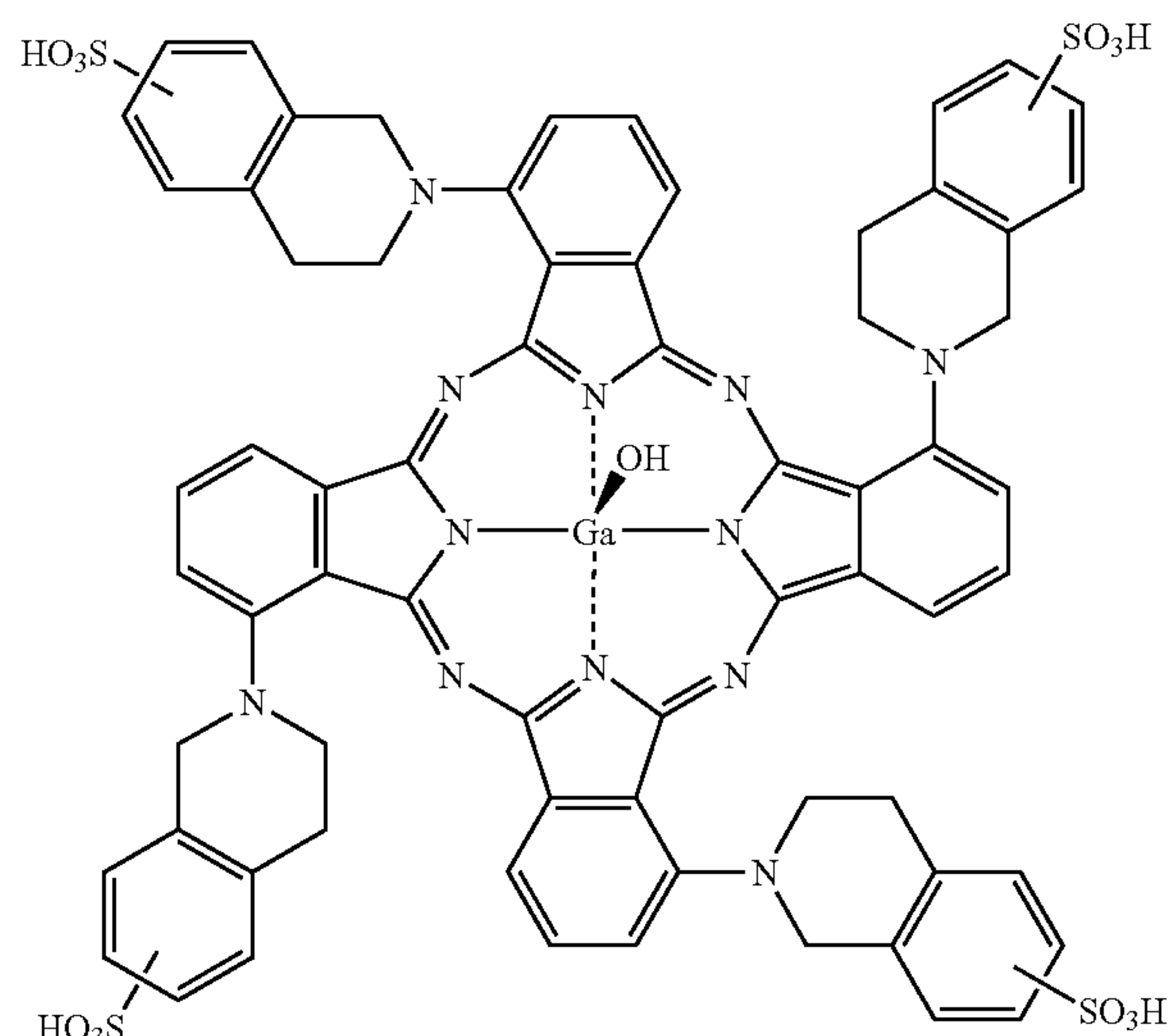
Sulfonation of gallium(III) tetrakis(1,2,3,4-tetrahydroisoquinolyl)phthalocyanine hydroxide
