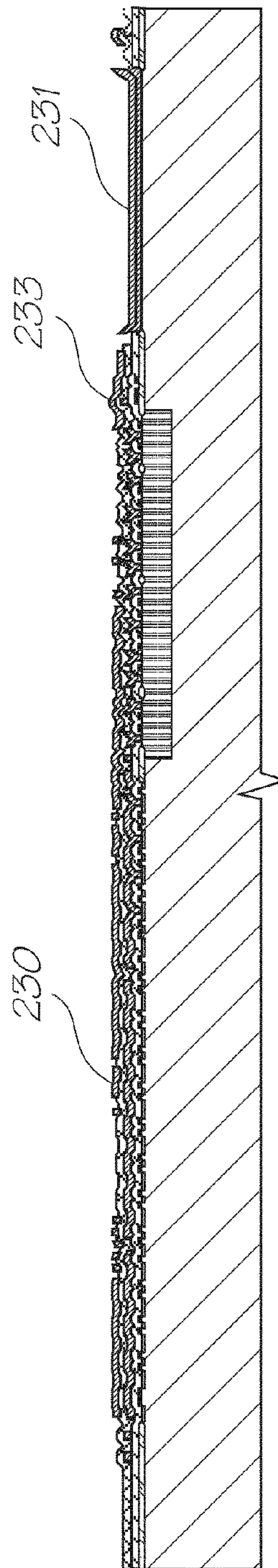
Deposit metal 2
