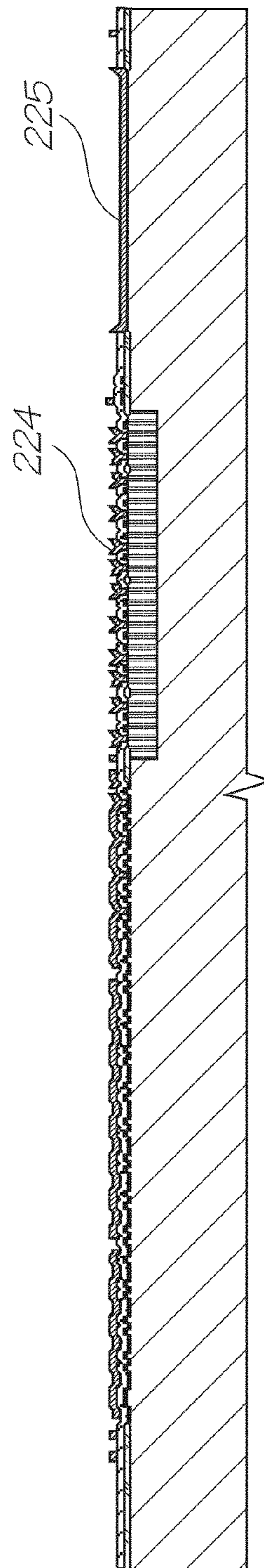
Deposit Metal 1
