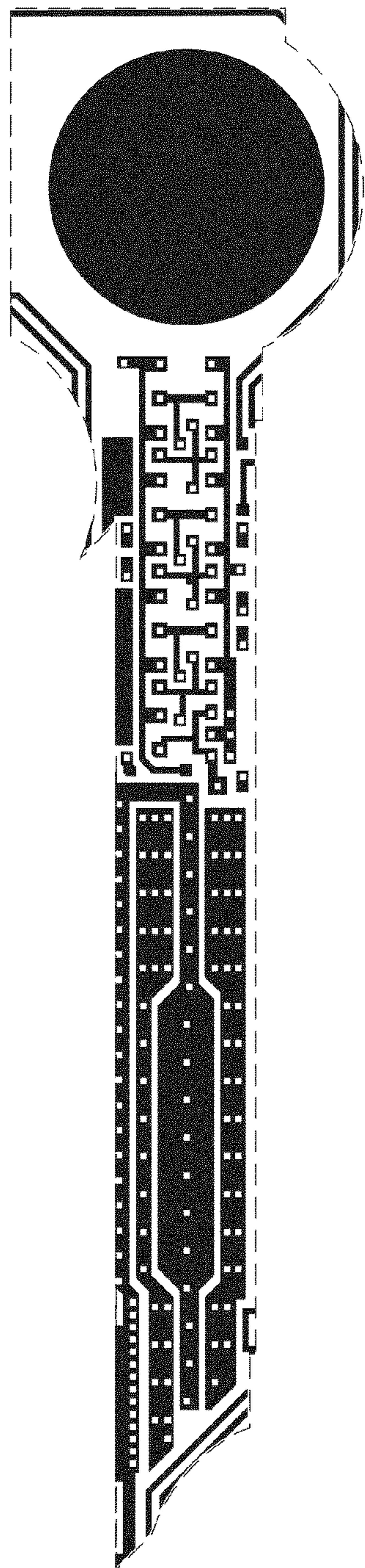
Metal 1 mask
