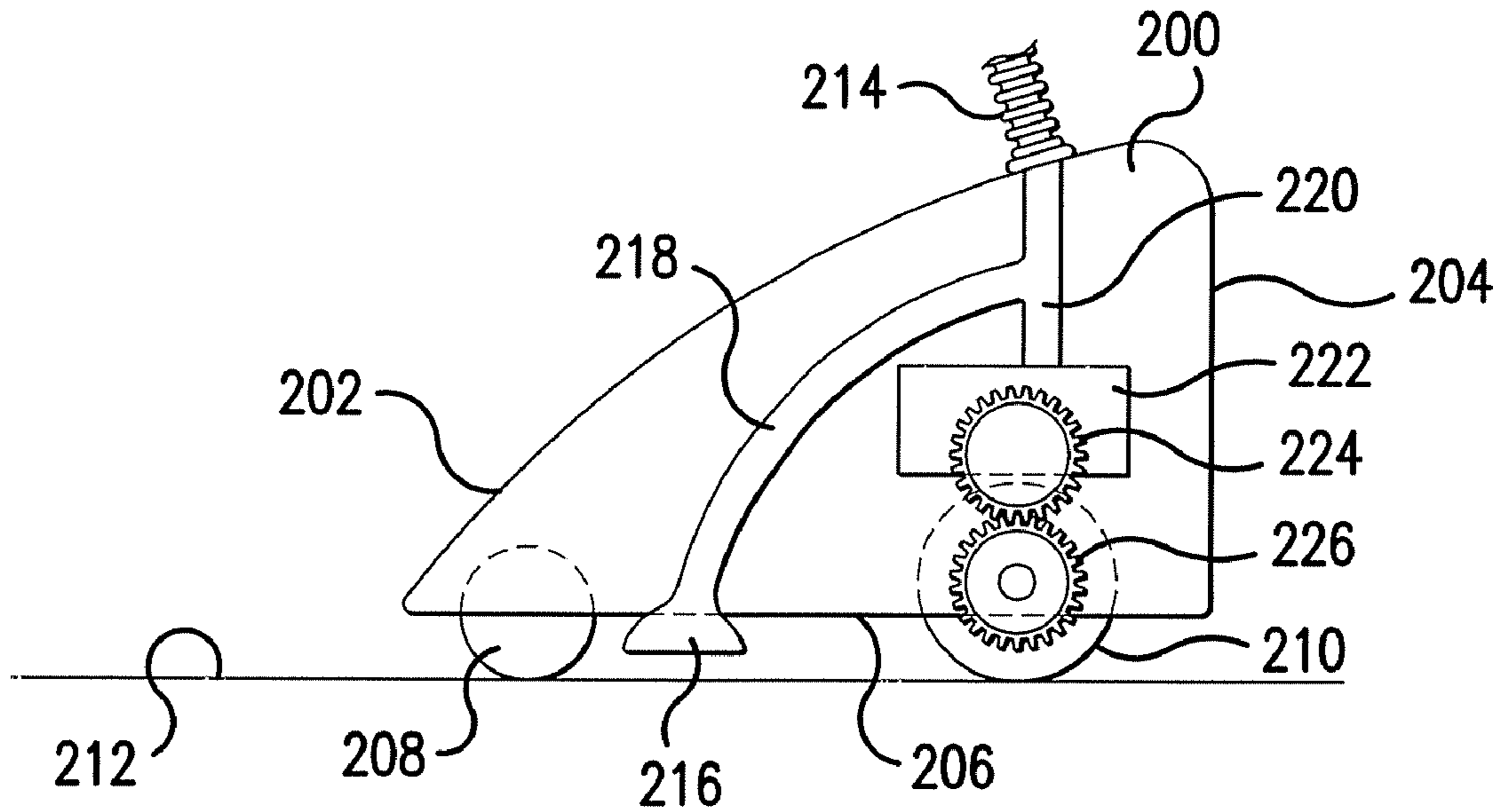
FIG. 9 CONVENTIONAL ART
