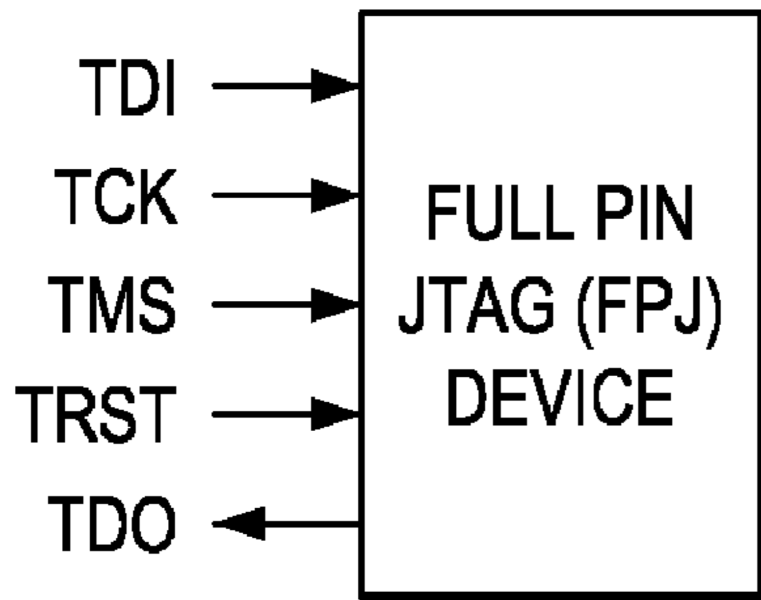
FIG. 1 (PRIOR ART)
