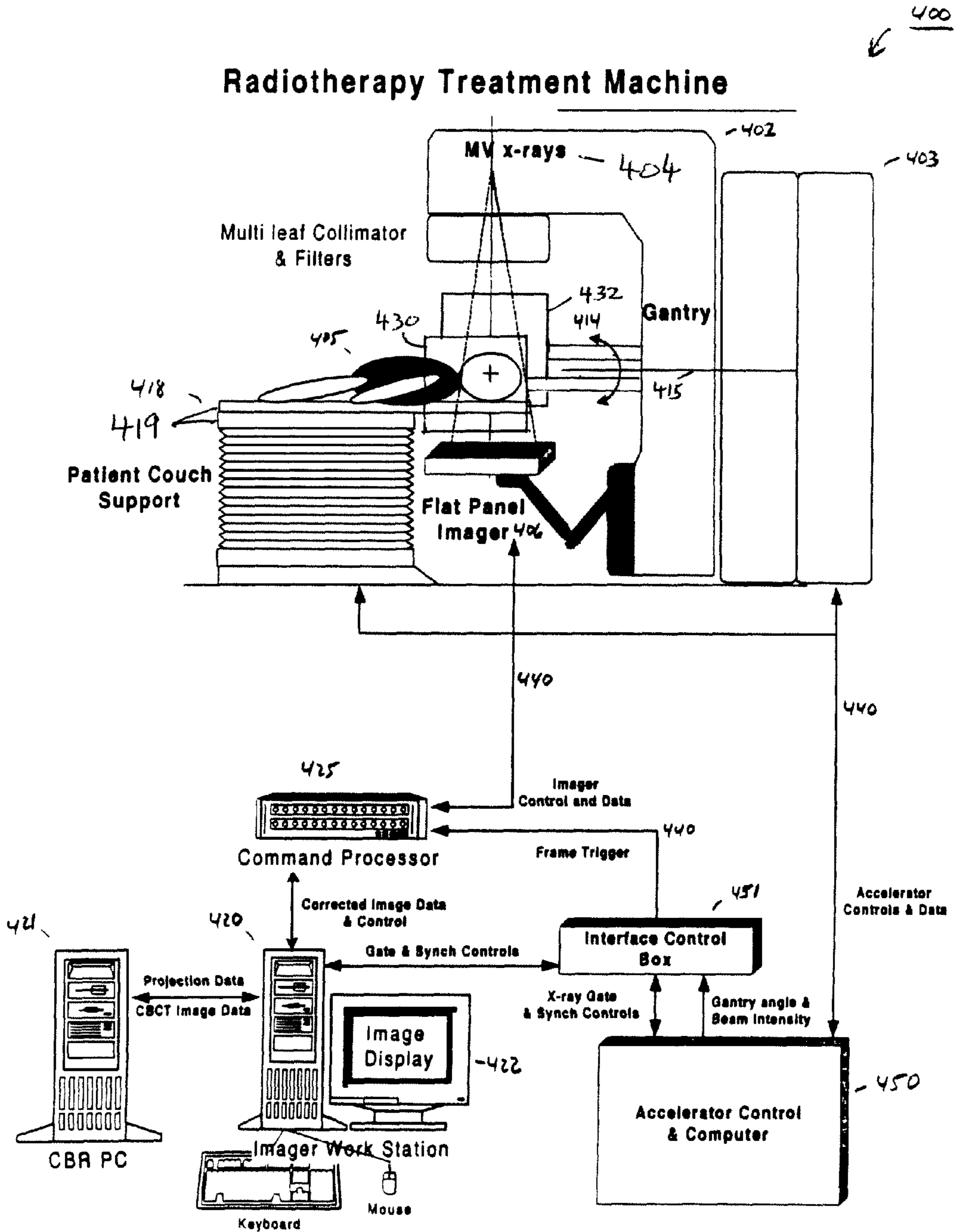
Figure 3- MV Cone Beam CT Diagram
