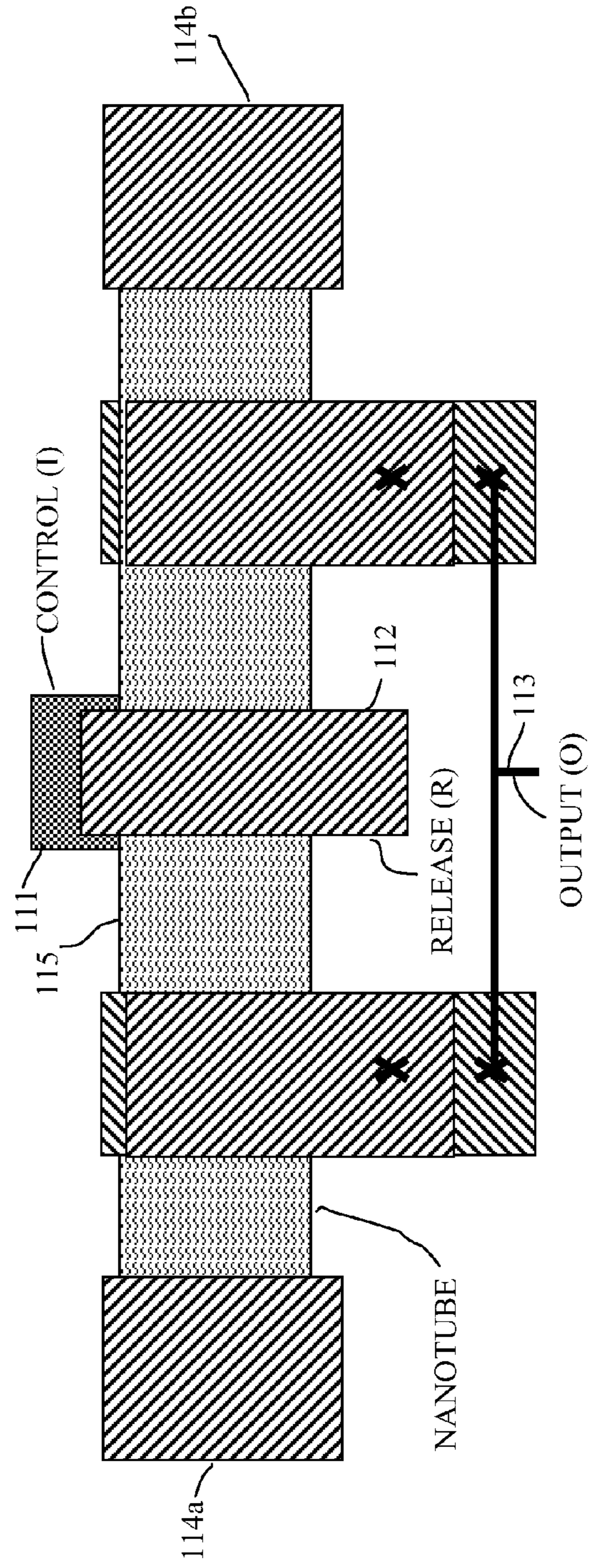
Figure 1B: NT Device - Top View - Suspended Region
