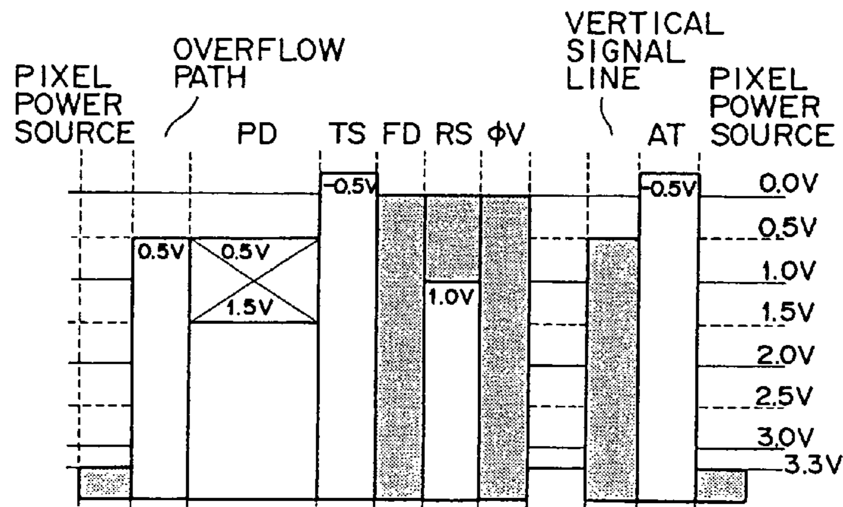
FIG. 4A t < t_1 NON-SELECTION STATE
