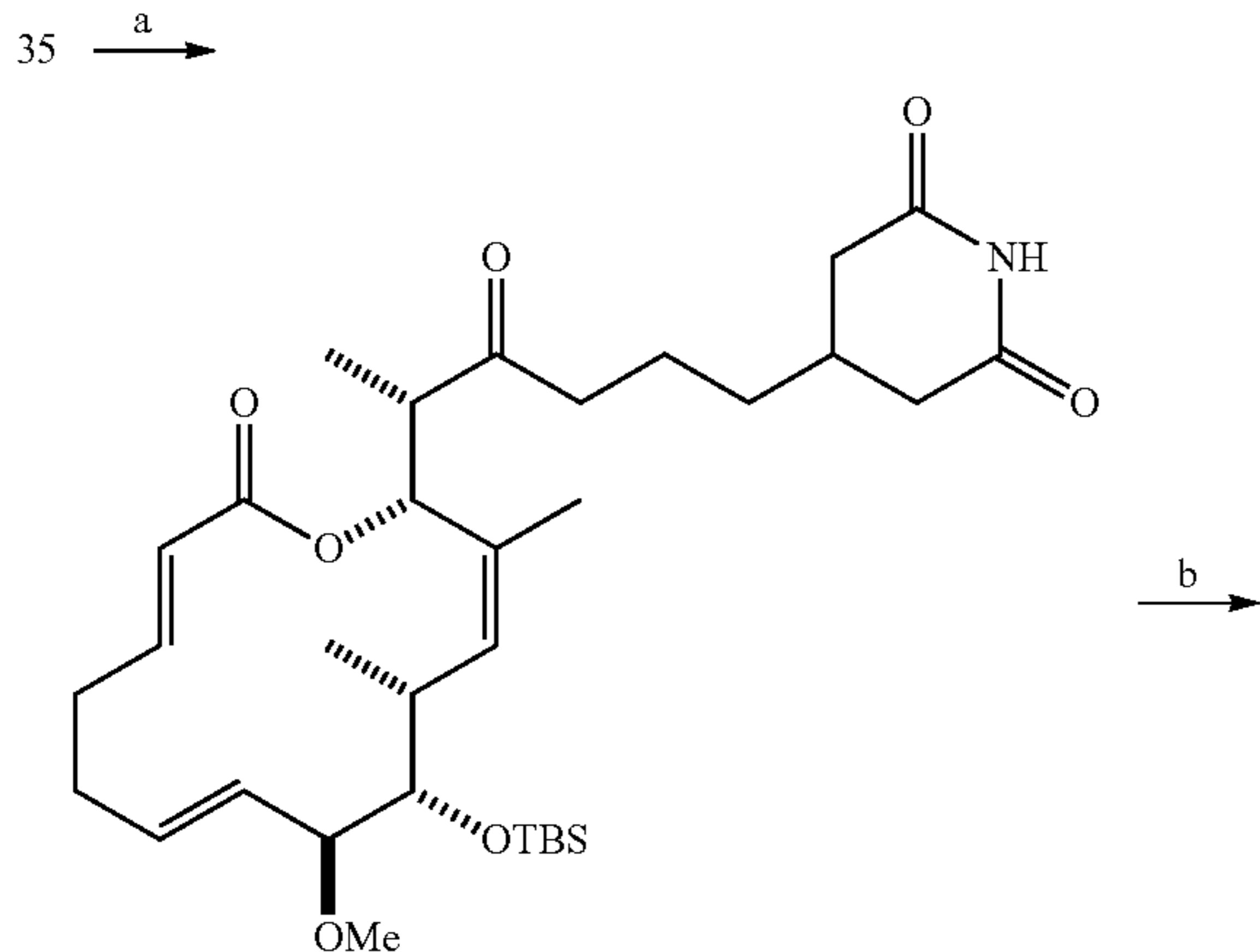
Scheme 23. RCM and Deprotection Leading to (+)-Migrastatin (1) a
