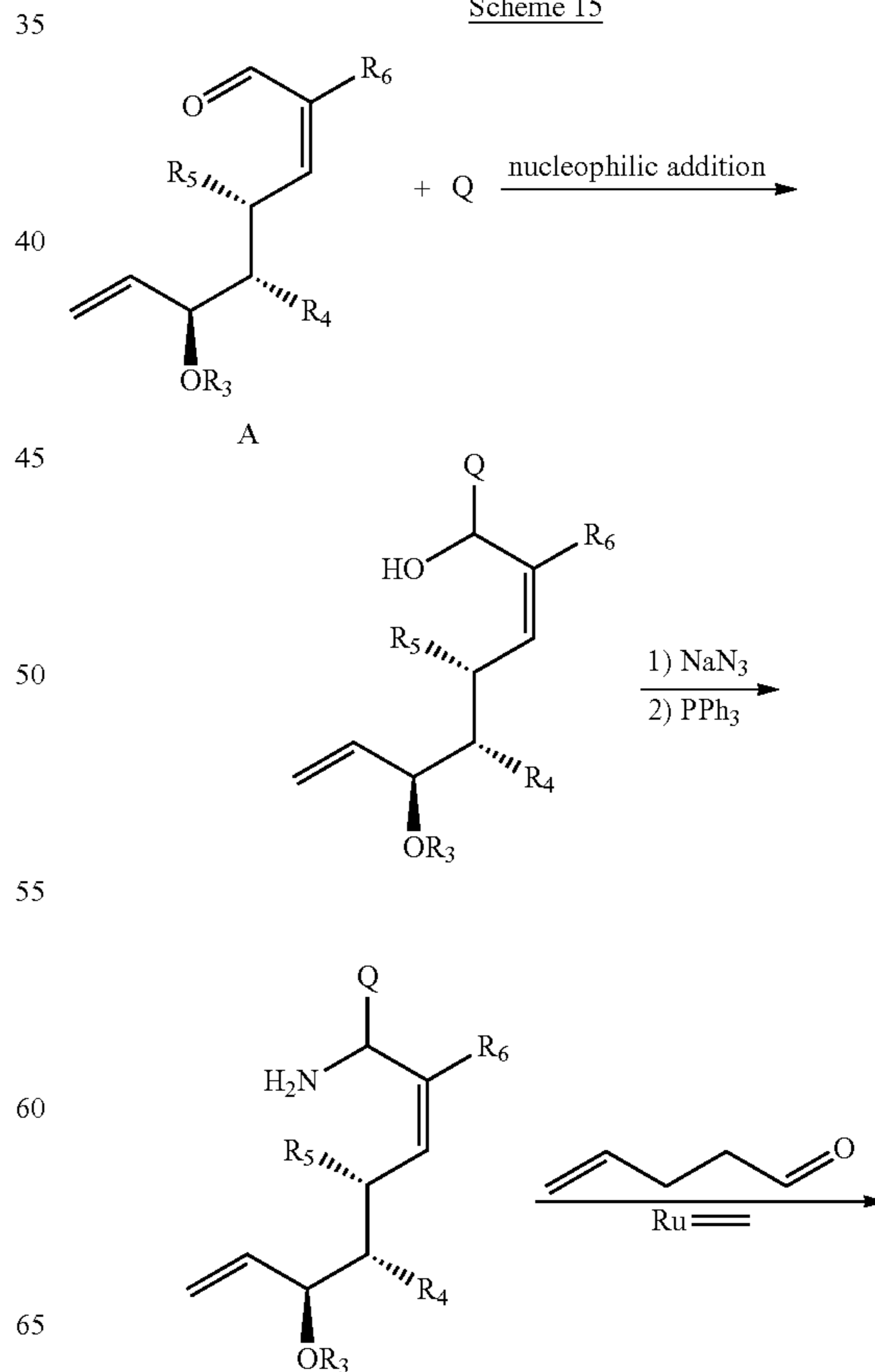
Scheme 15
