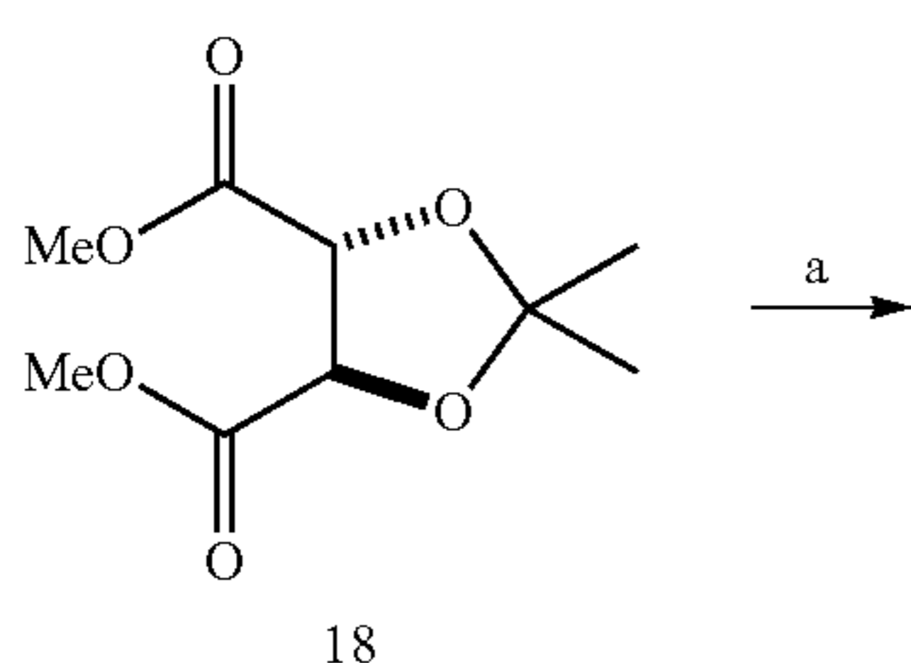
Scheme 19. Synthesis of Dihydropyrone 21 by a Cyclocondensation (LACDAC) a
