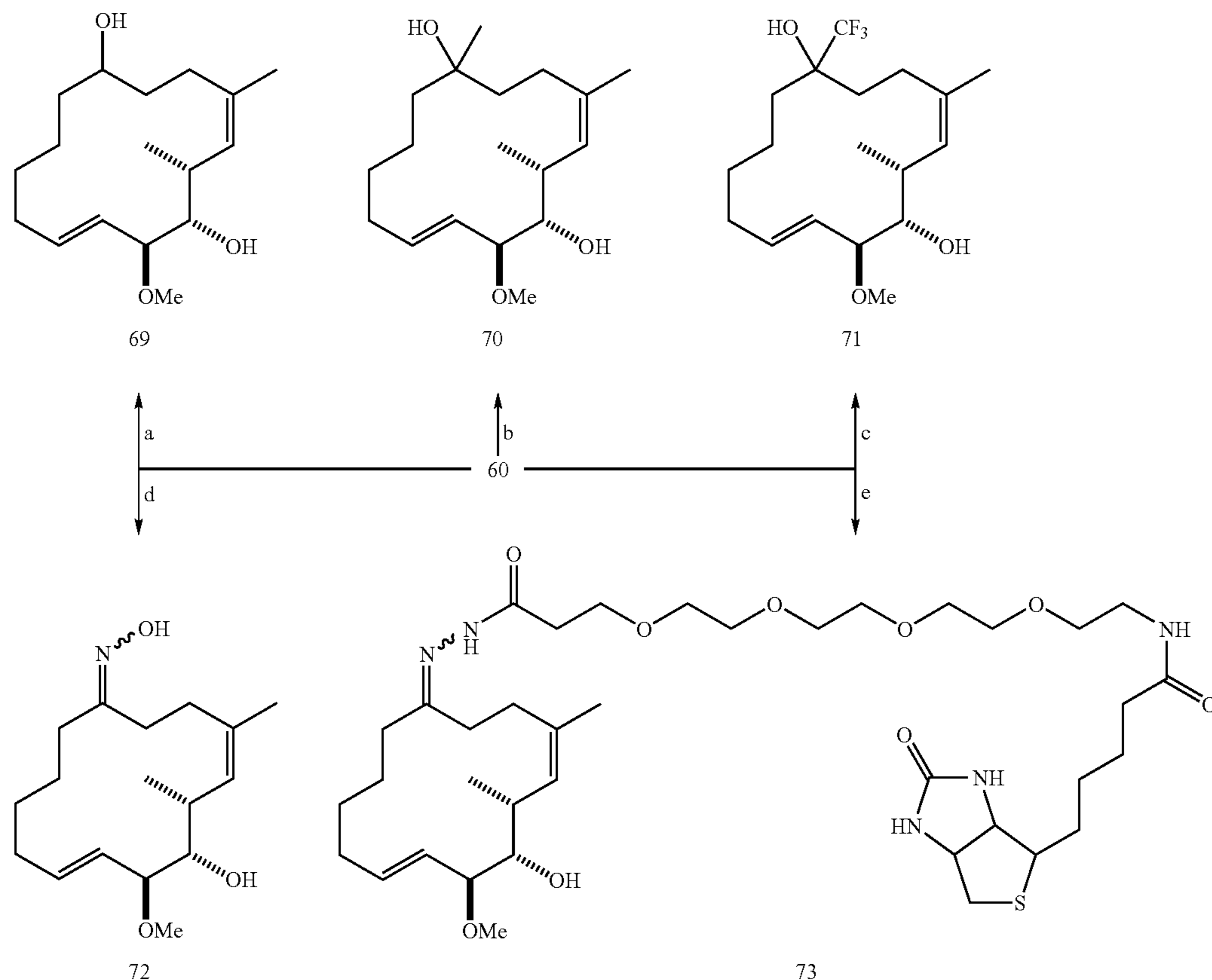
Scheme 30. Derivation of Macroketone 60 a
