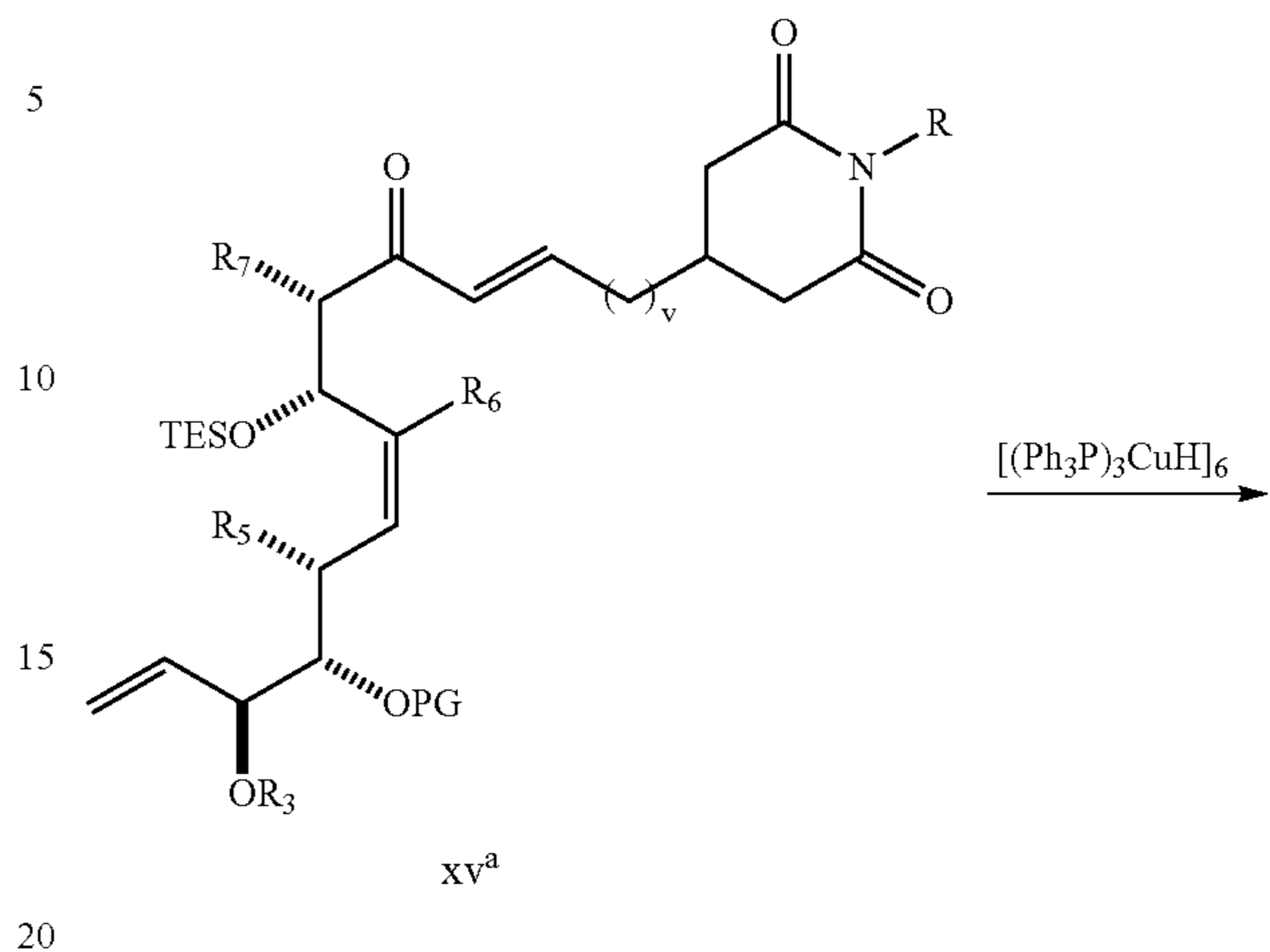
Scheme 8
