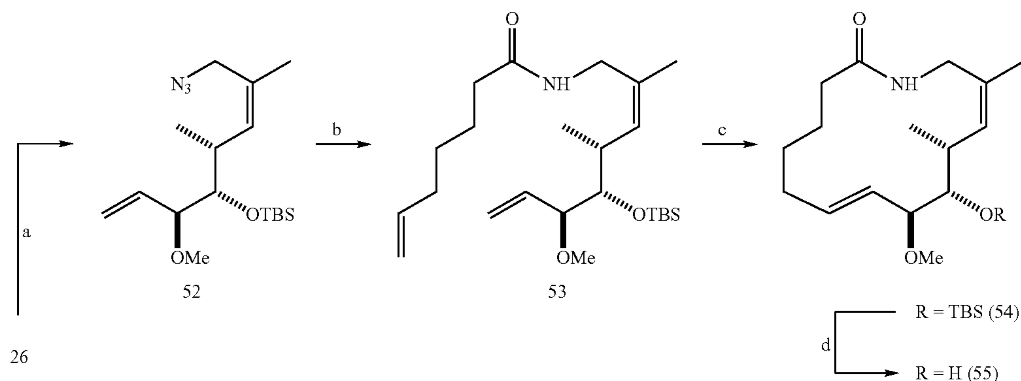
Scheme 28. Synthesis of Macrolactam 55 and Macroketone 60 a
