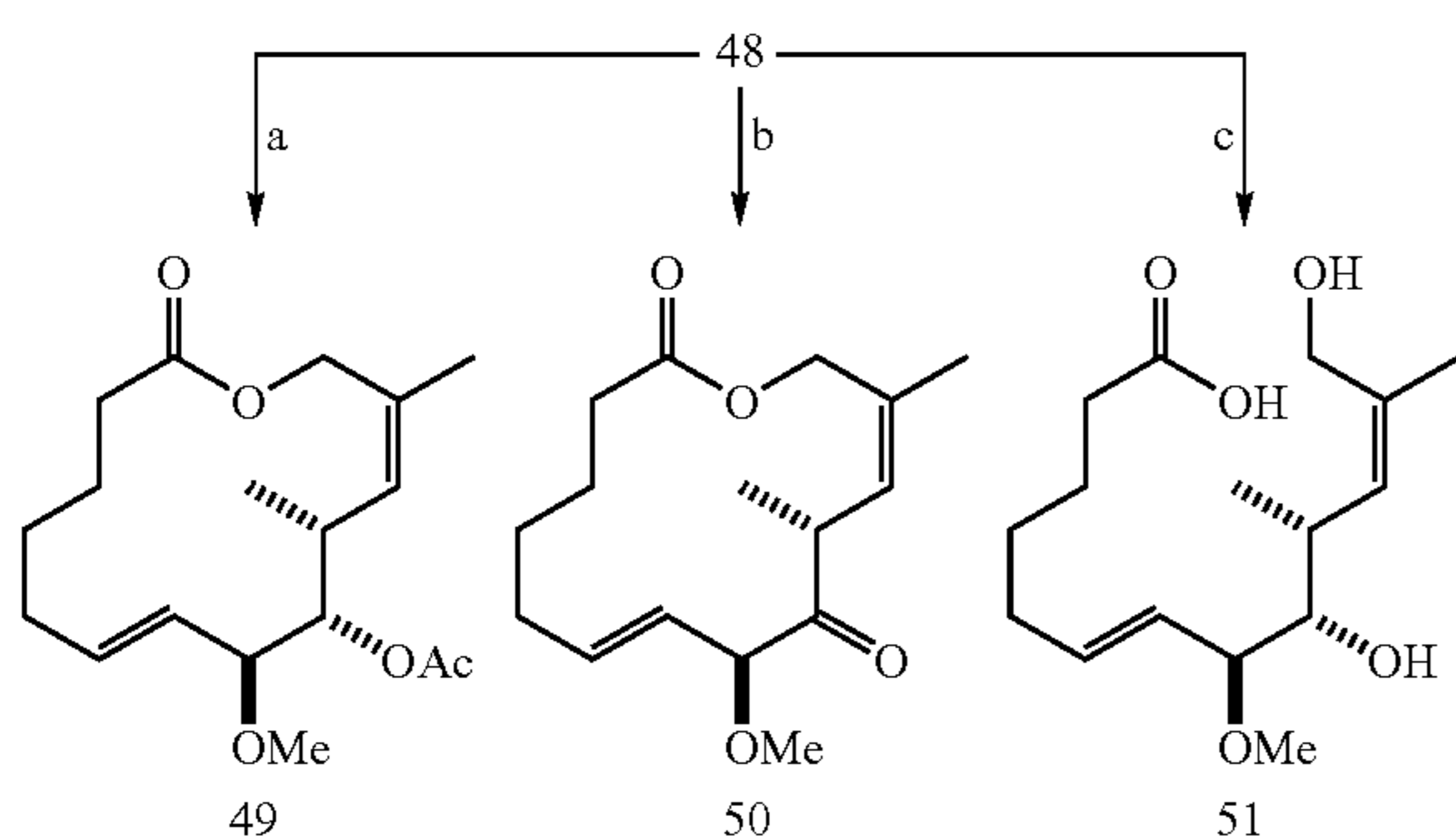
Scheme 27. Modification of Macrolactone 48 at the C9 position and Hydrolysis of 48 a
