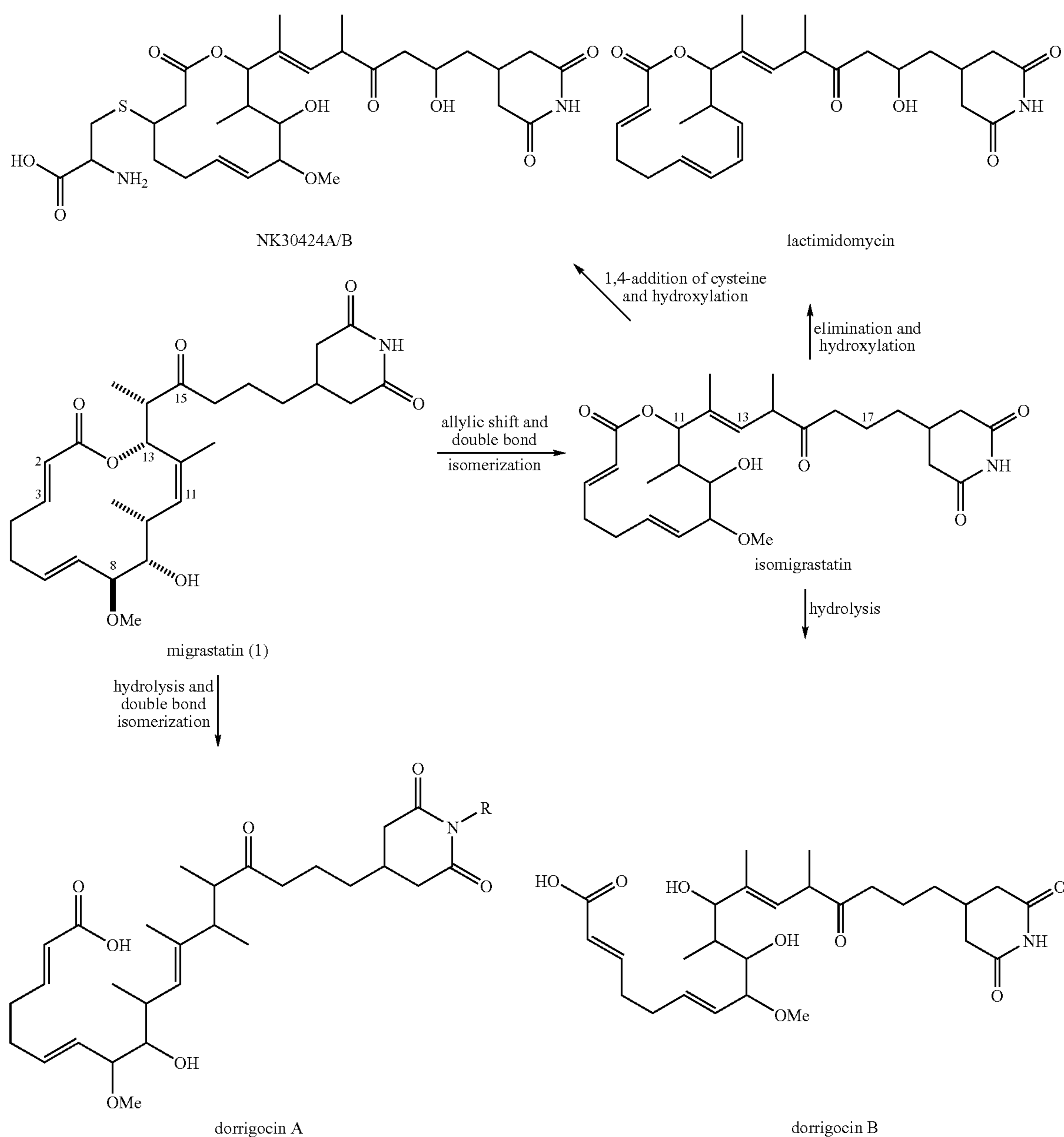
Scheme 16. Structure of Migrastatin and Related Natural Products
