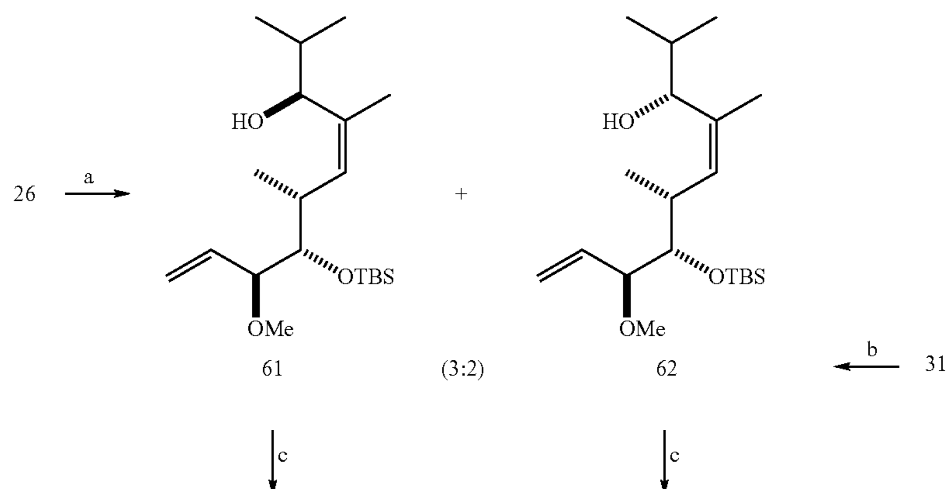
Scheme 29. Synthesis of the Diastereomeric Isopropyl Macrolactones 65 and 68 a
