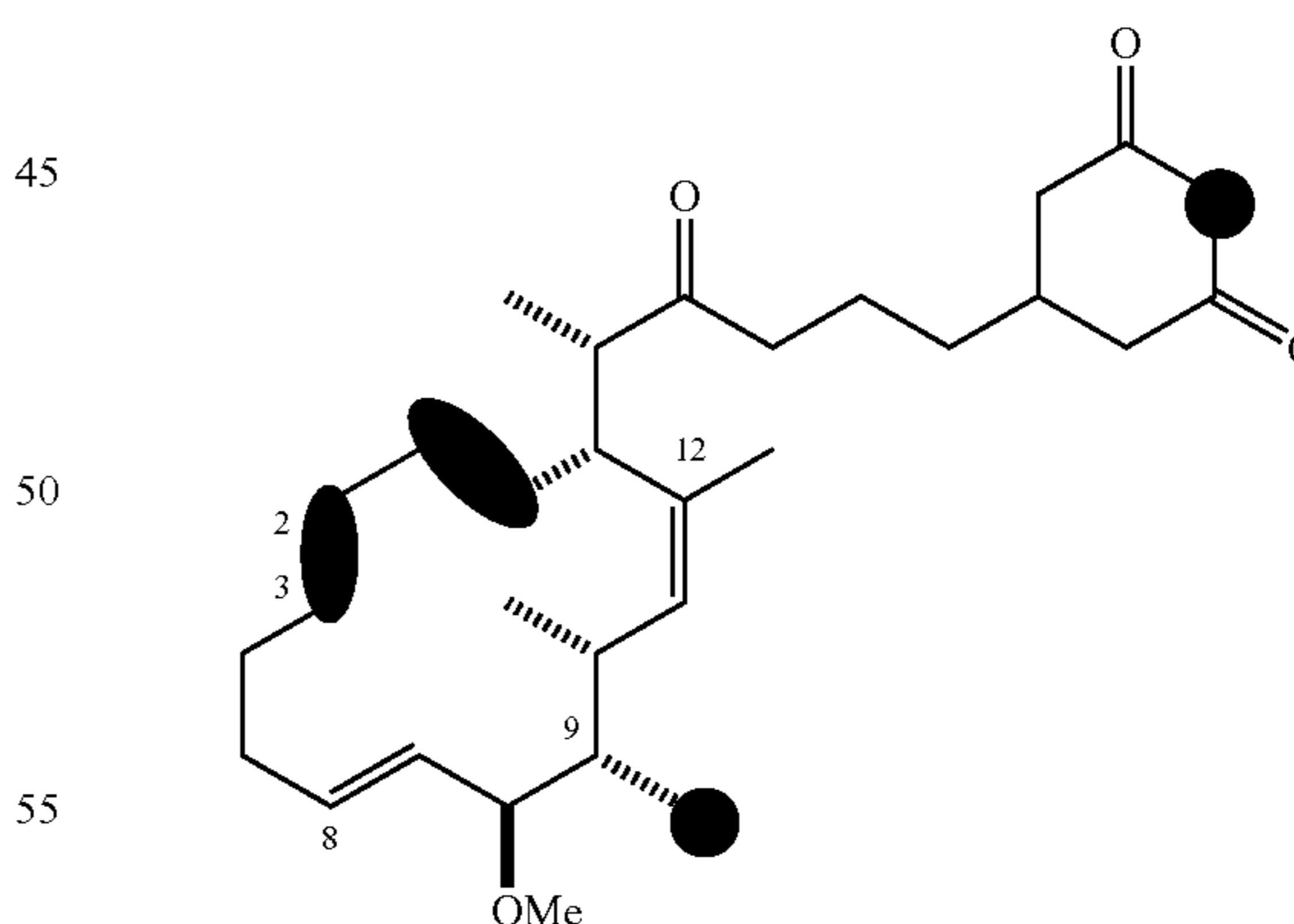
Scheme 23. RCM and Deprotection Leading to (+)-Migrastatin (1) a
