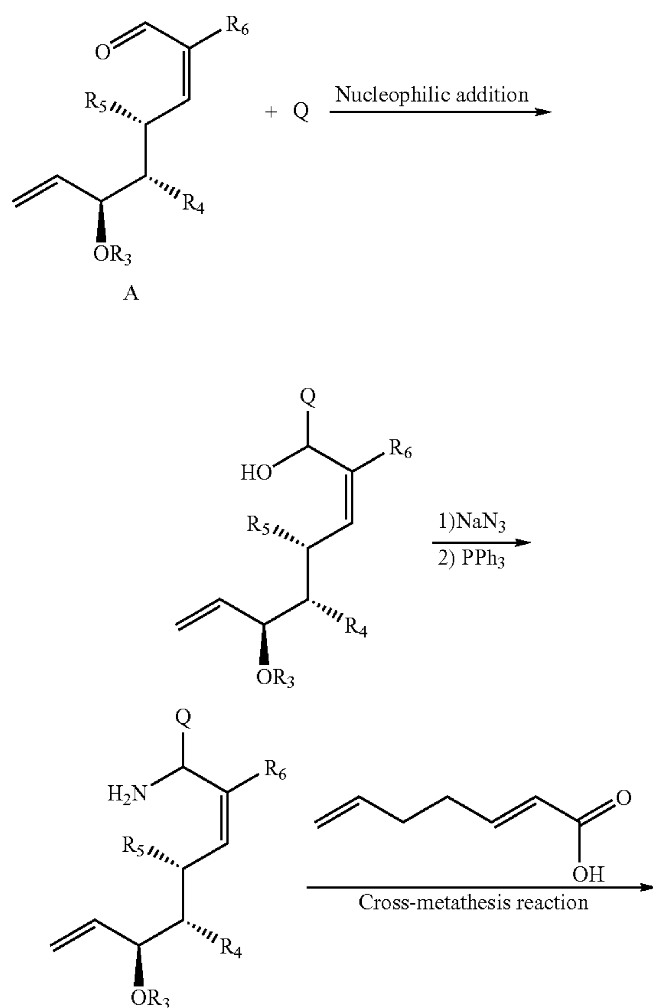
Scheme 14
