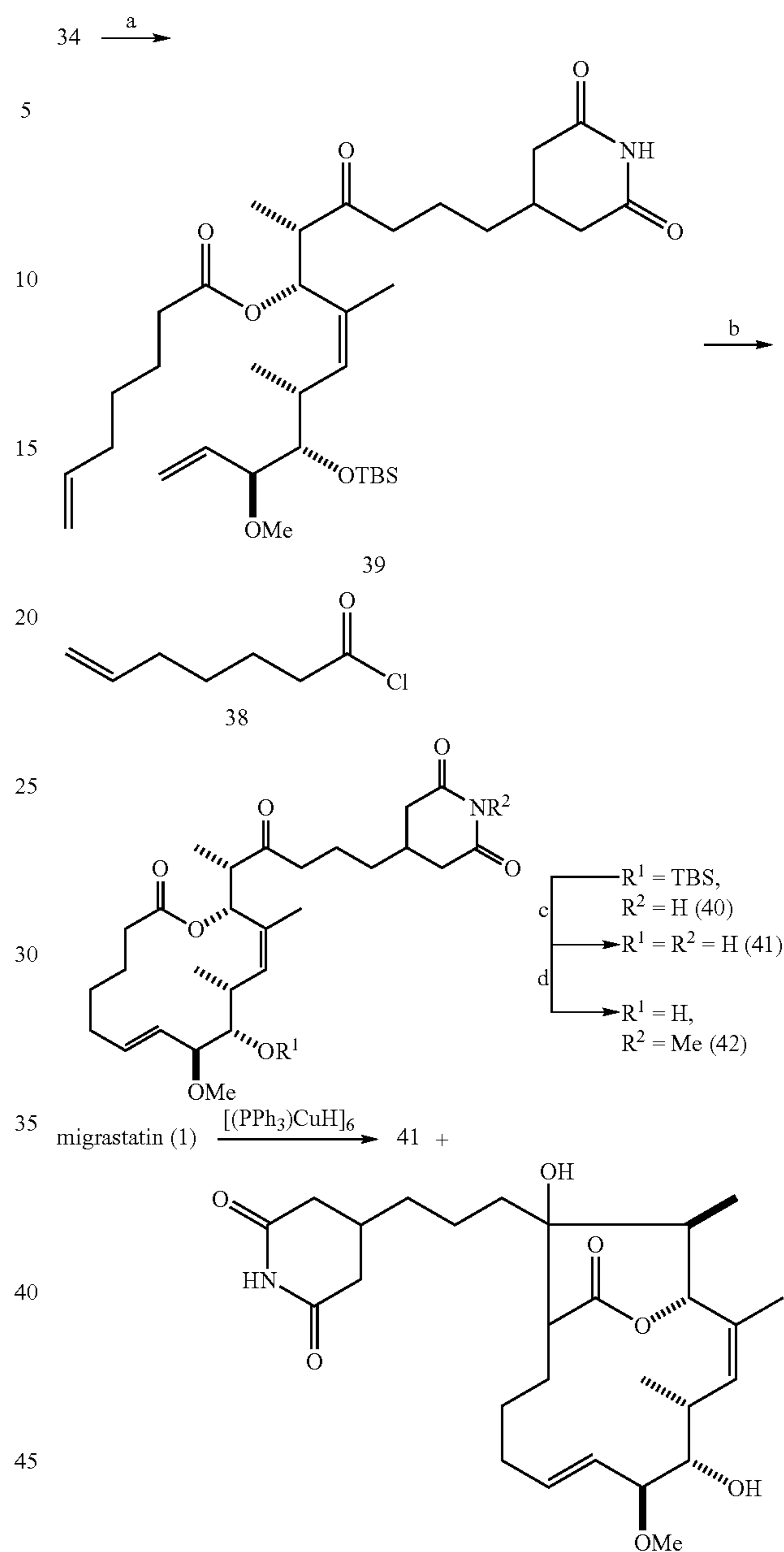
Scheme 24. Preparation of Migrastatin Analogs 41 and 42 a
