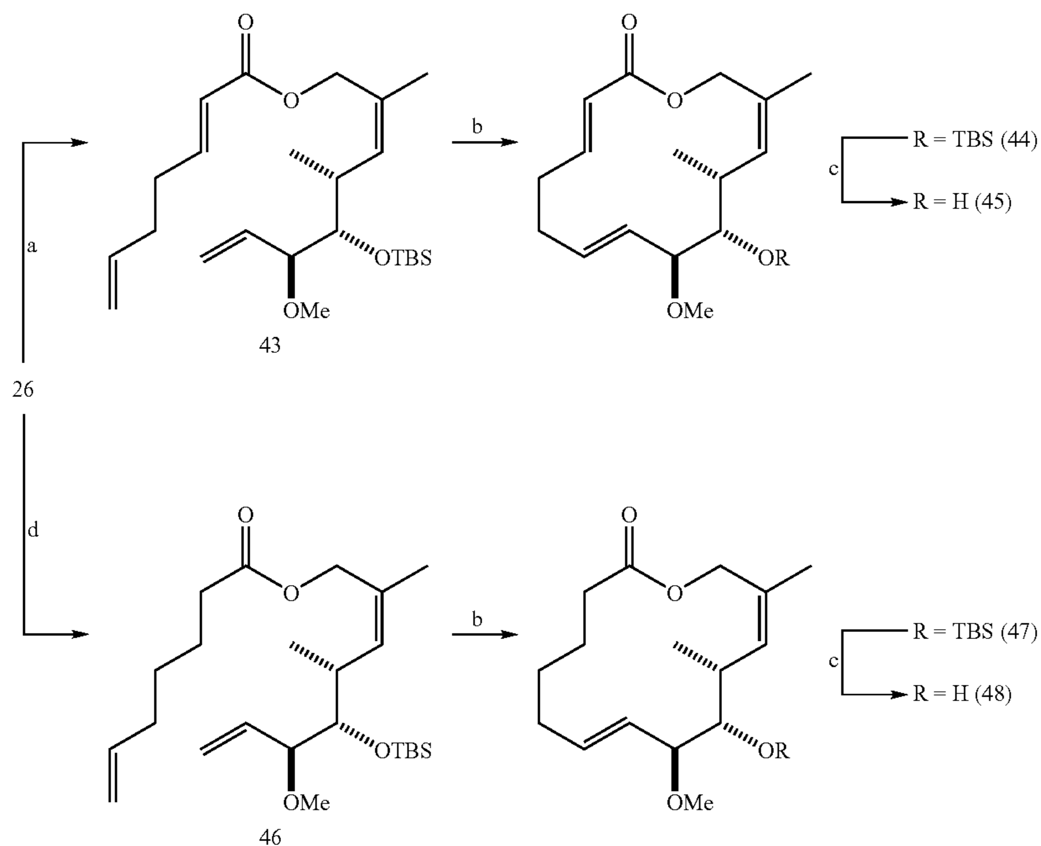
Scheme 25. Synthesis of Migrastatin Core 45 and Macrolactone 48 a
