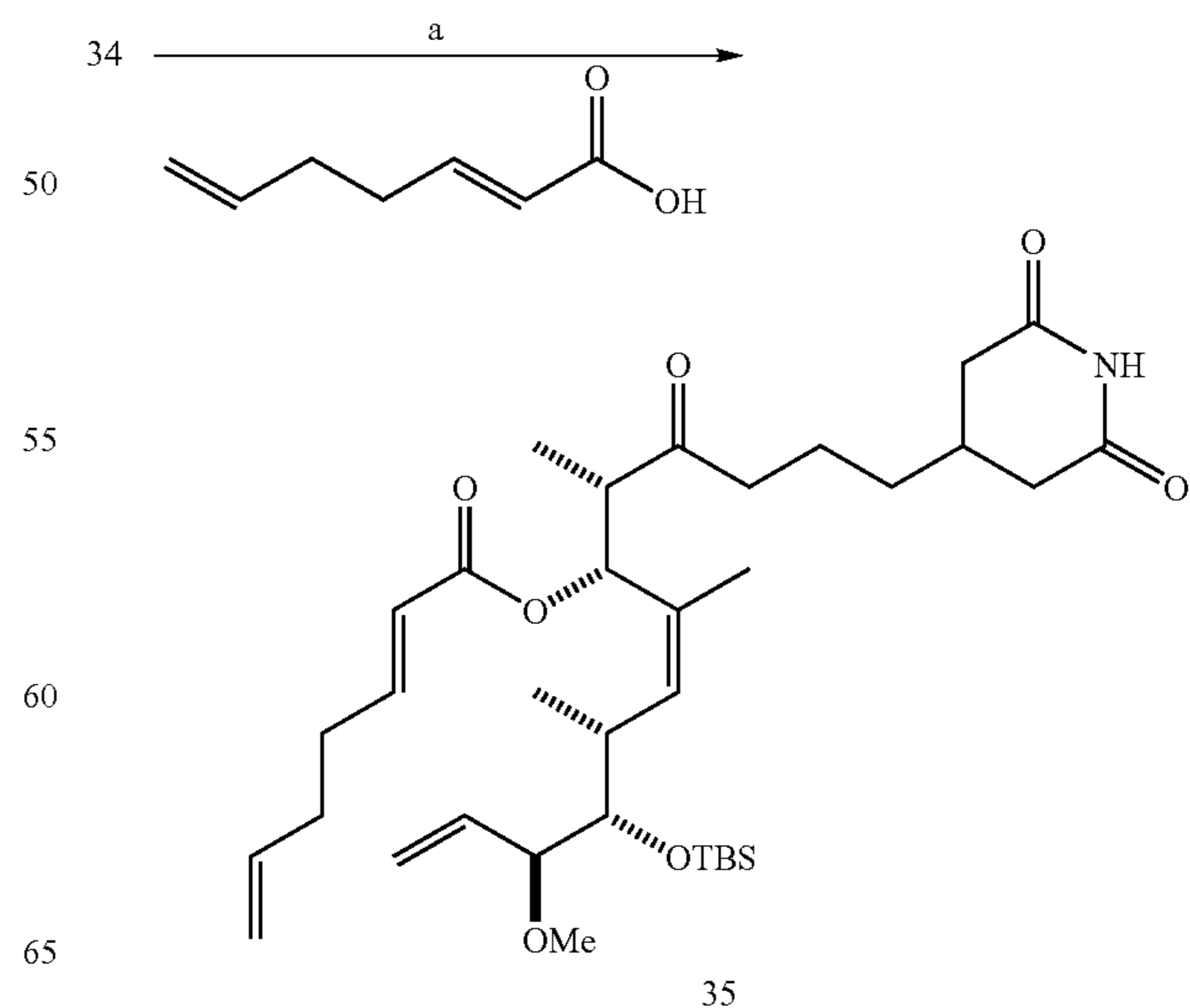
45 Scheme 22. Acylation of Alcohol 34 by a Modified Yamaguchi Procedure a
