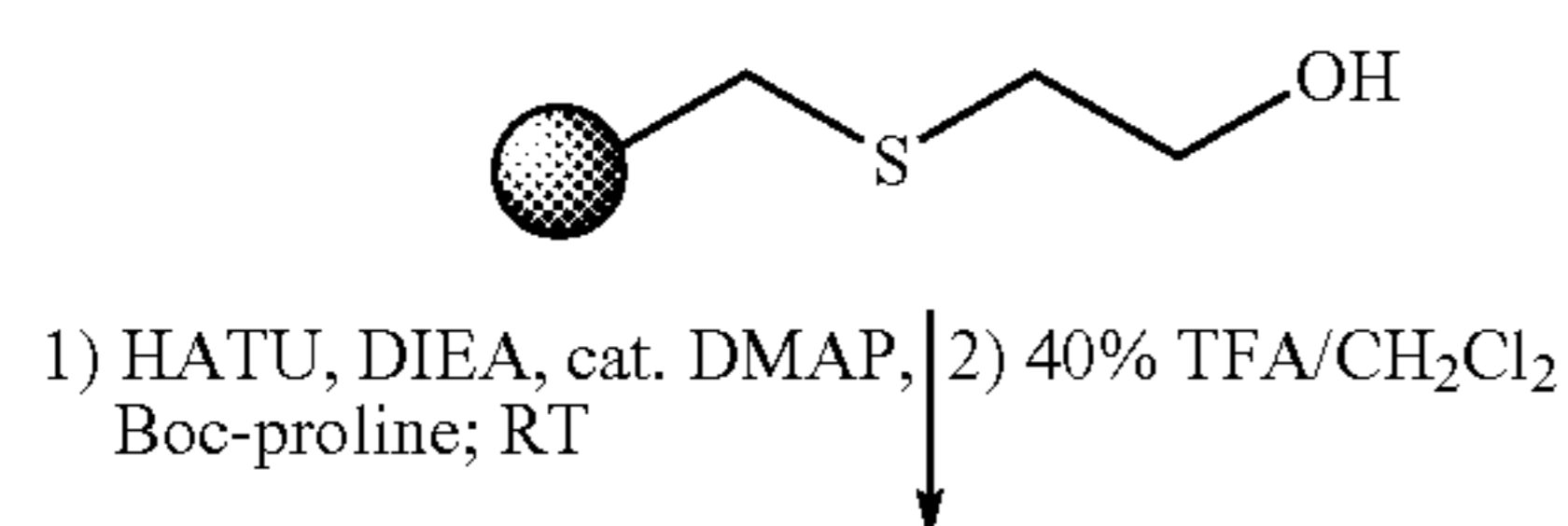
Scheme 9. Amino acid amides of 5'-adenosinecarboxylic acid derivatives and 8-azaadenosine-5'-carboxylic acid derivatives using solid phase techniques.
