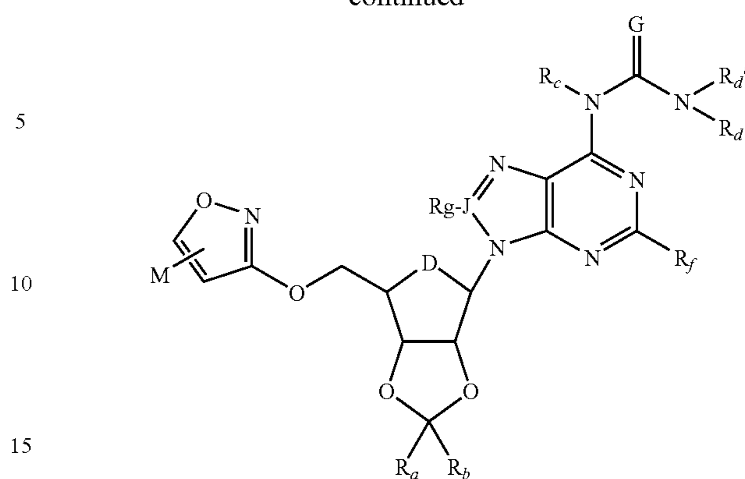
Scheme 2. Preparation of 5'-modified ethers by Mitsunobu coupling of phenols.
