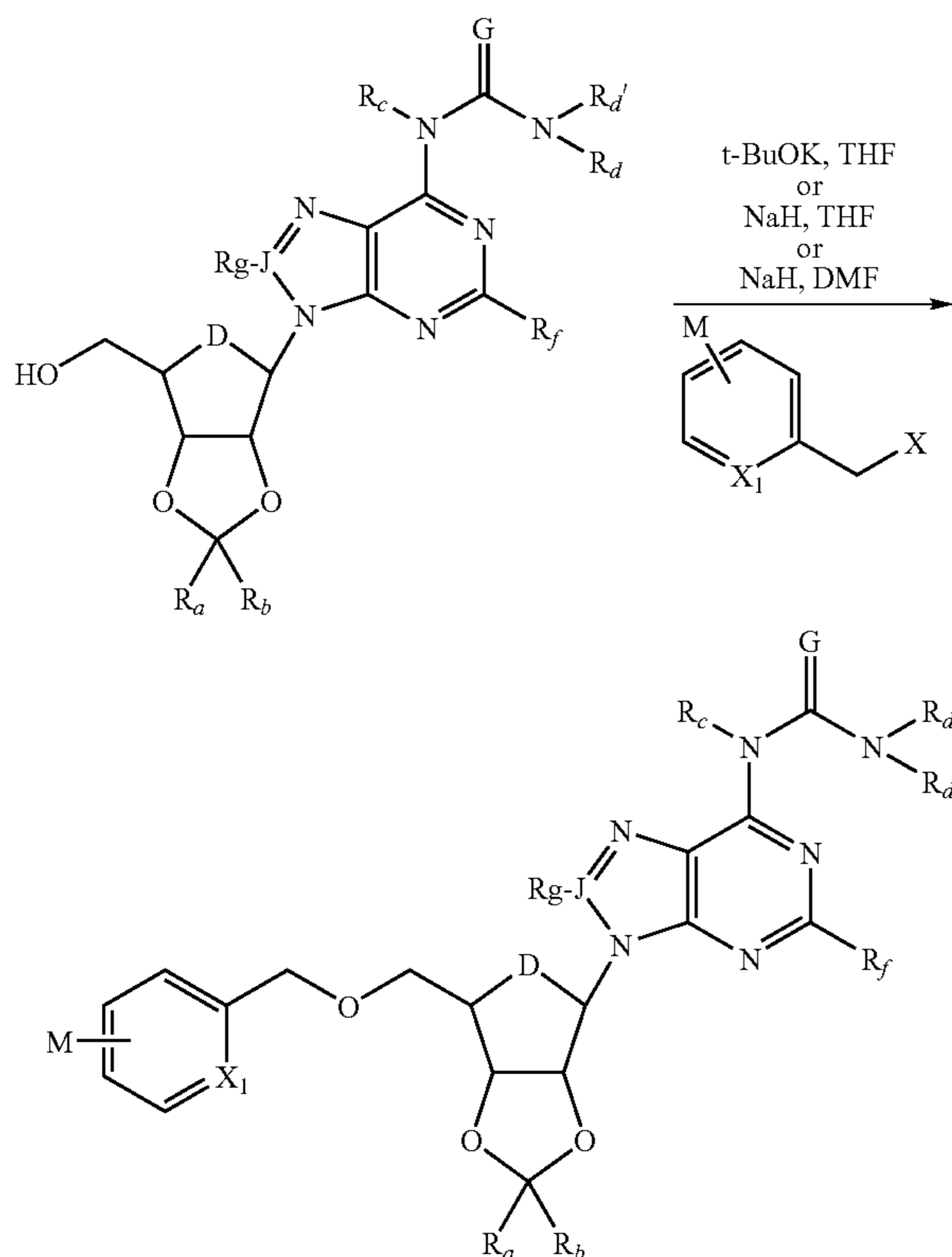
Scheme 12. Preparation of 5'-substituted ethers.
