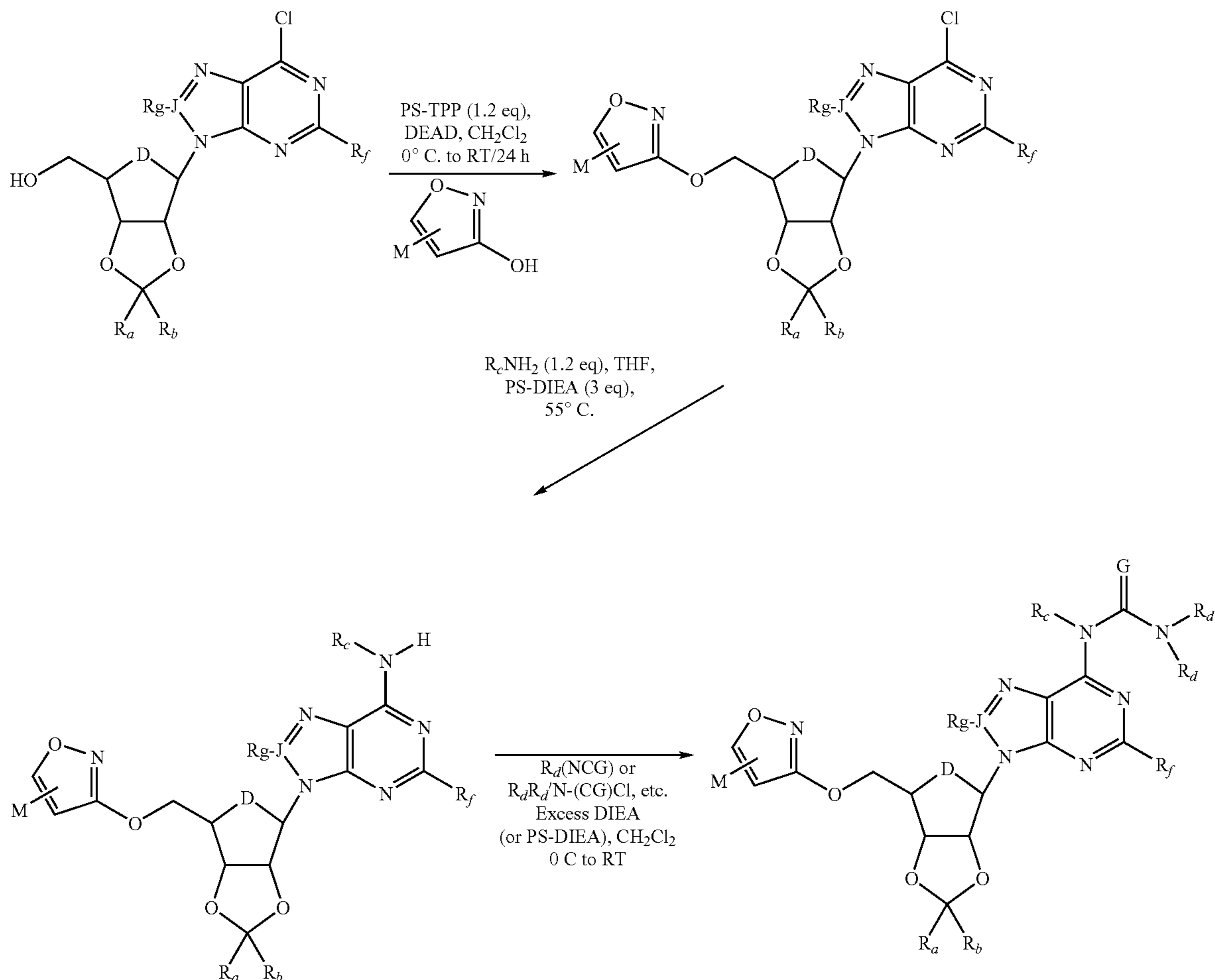
Scheme 6. Solution phase synthesis of 5'-heteroaromatic ether-N 6 -derivatives by Mitsunobu reaction, 6-chloride displacement, and N 6 -amine derivatization.
