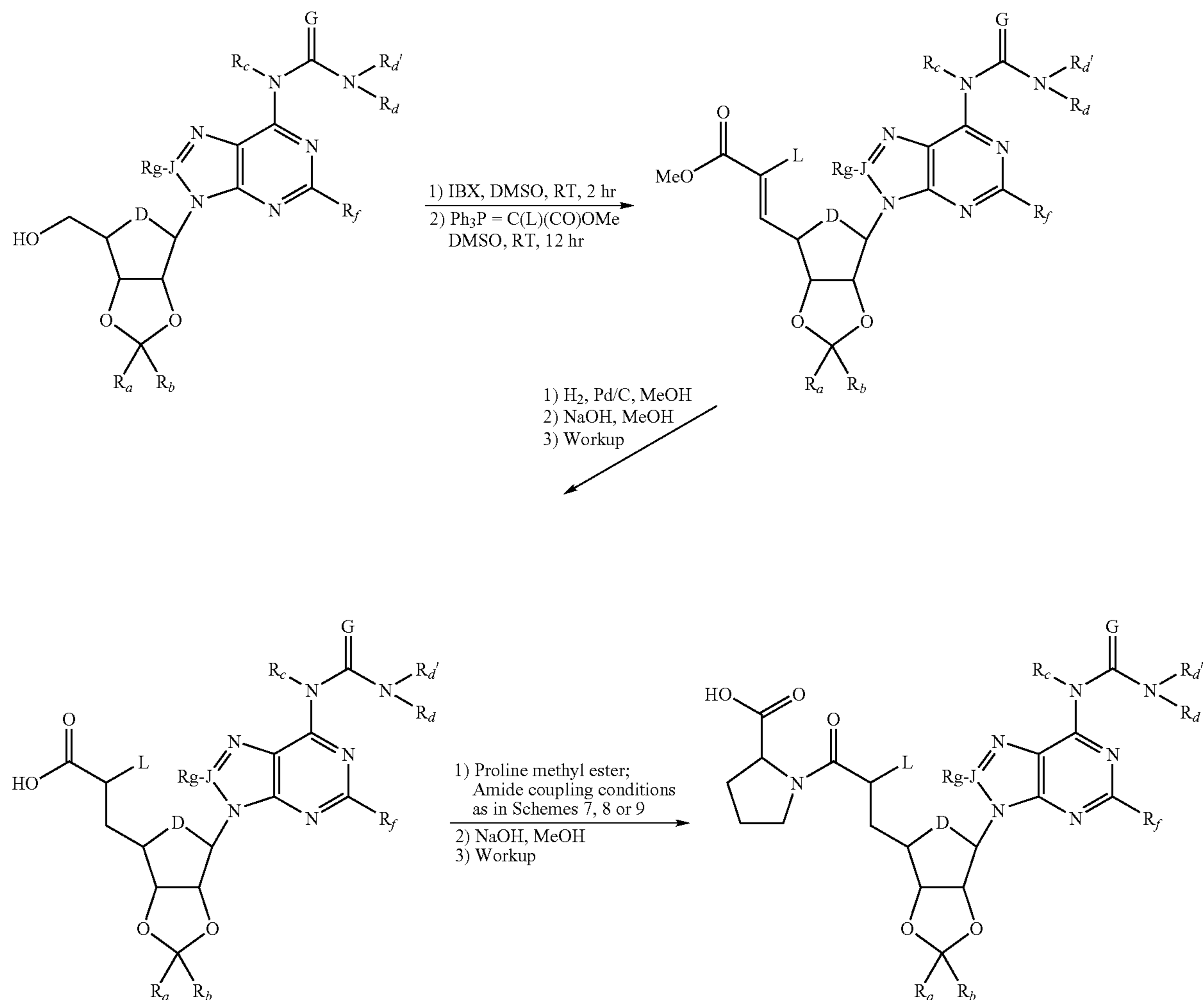
Scheme 11. Homologation of adenosine derivatives, including steps involving oxidation, Wittig or Horner-Emmons Reaction, reduction and coupling with amines.
