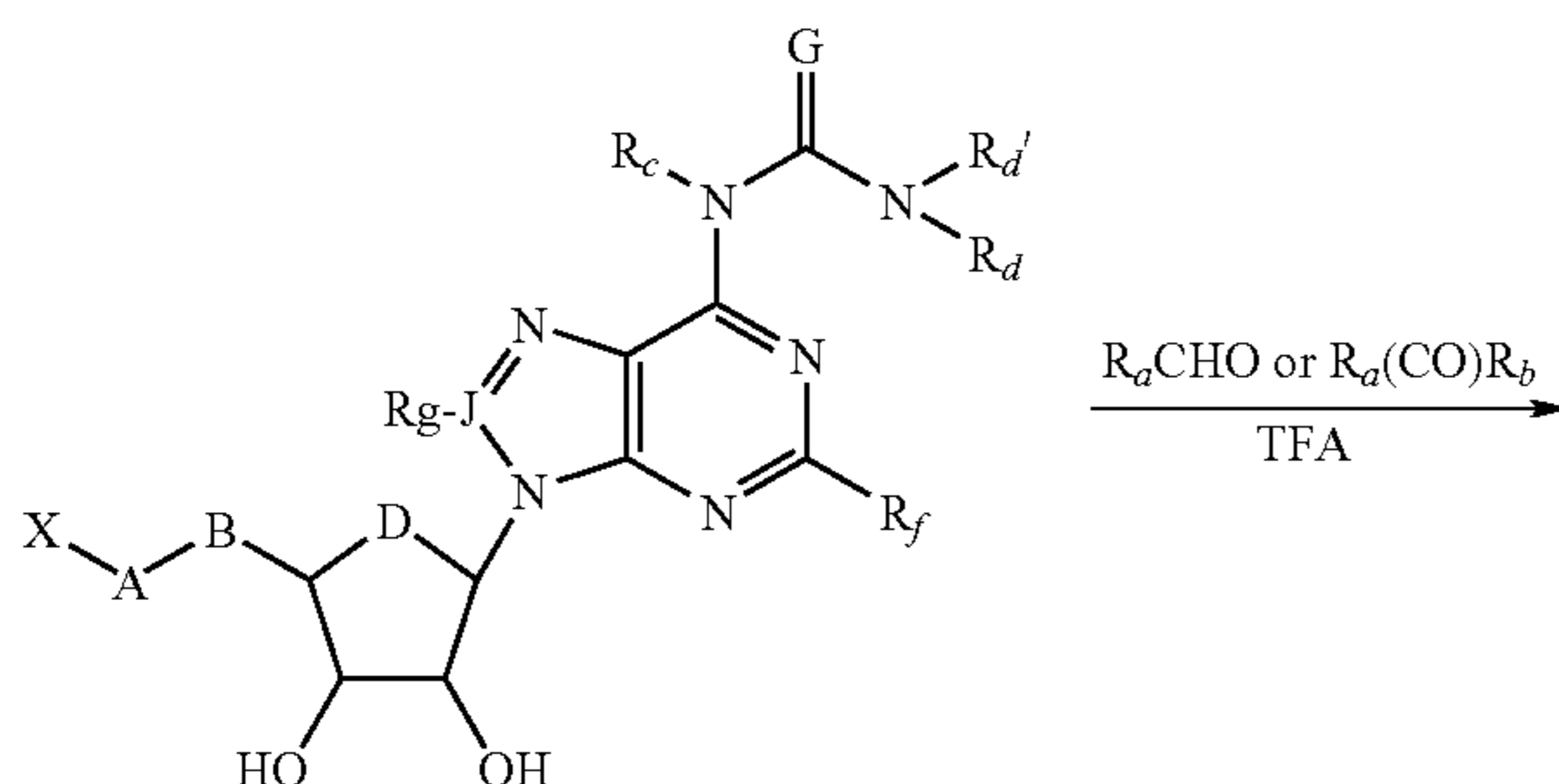
Scheme 13. Preparation of 2,3-acetals and -ketals.
