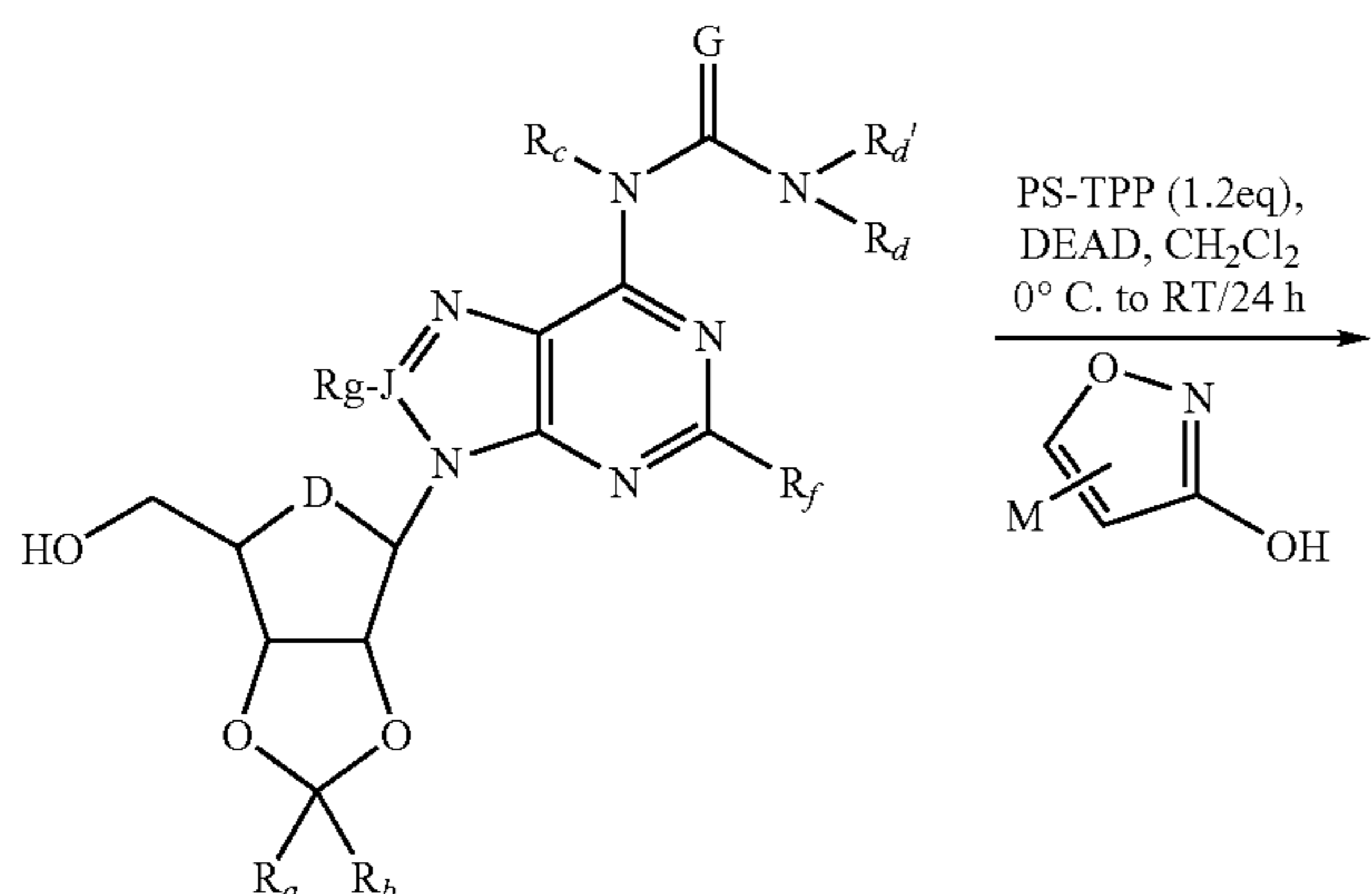
Scheme 3. Preparation of 5'-modified isoxazole ethers by Mitsunobu coupling of isoxazole derivatives.
