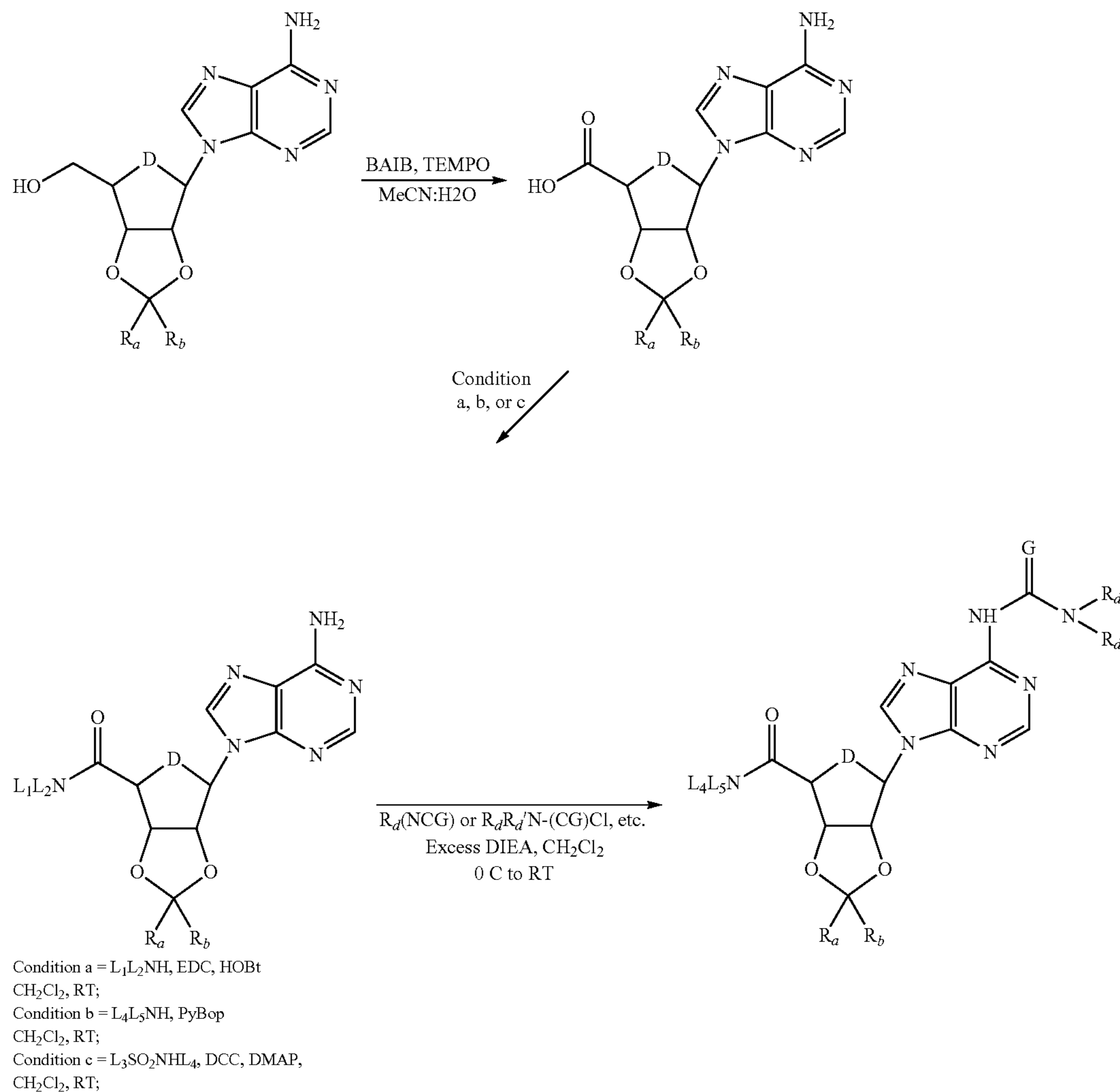
Scheme 7. Synthesis of 2',3'-O-Isopropylideneadenosine-5'-carboxylic acid, related acetals and ketals, and their use as intermediates for the synthesis of compounds of this invention.
