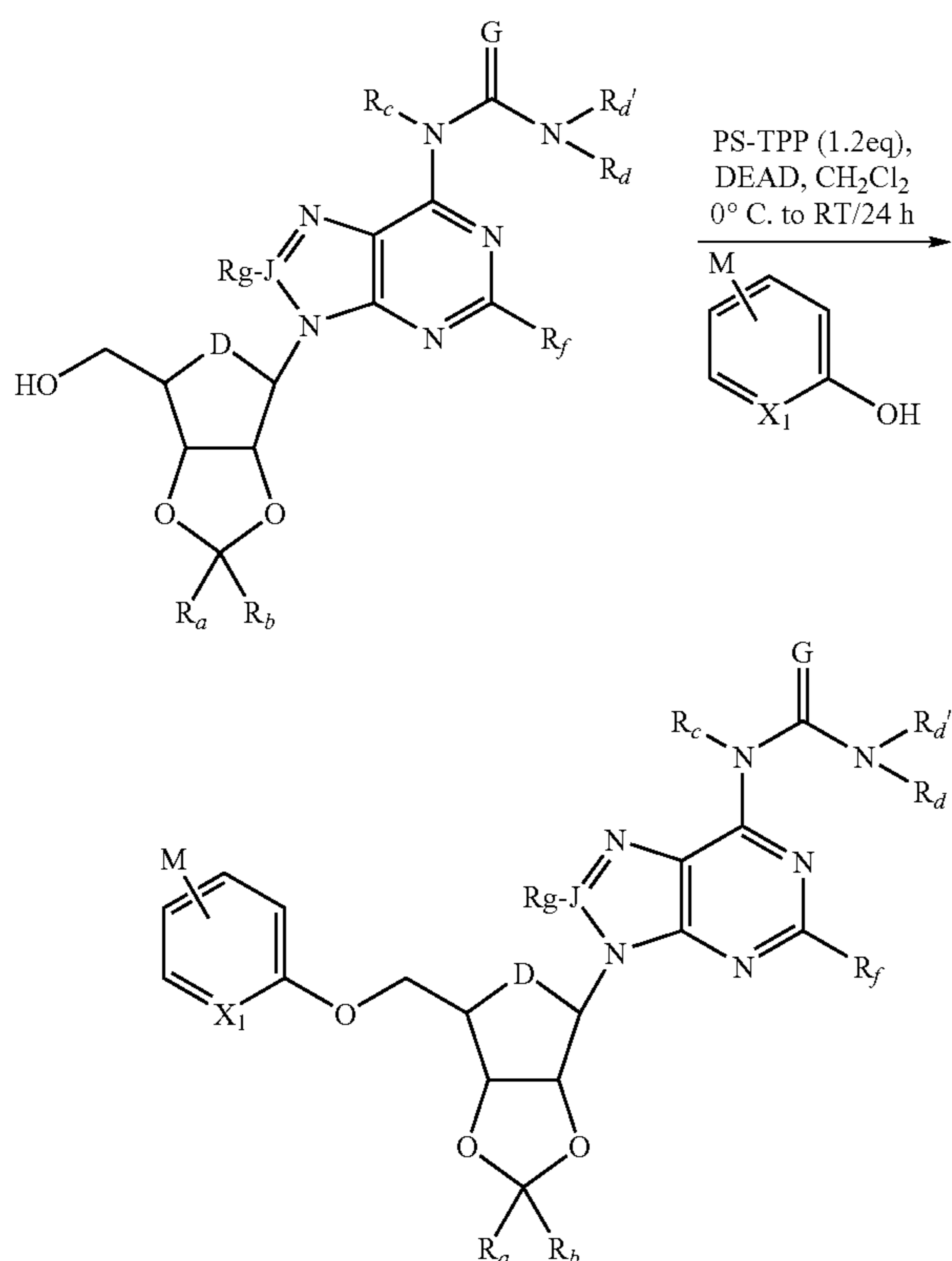
Scheme 2. Preparation of 5'-modified ethers by Mitsunobu coupling of phenols.
