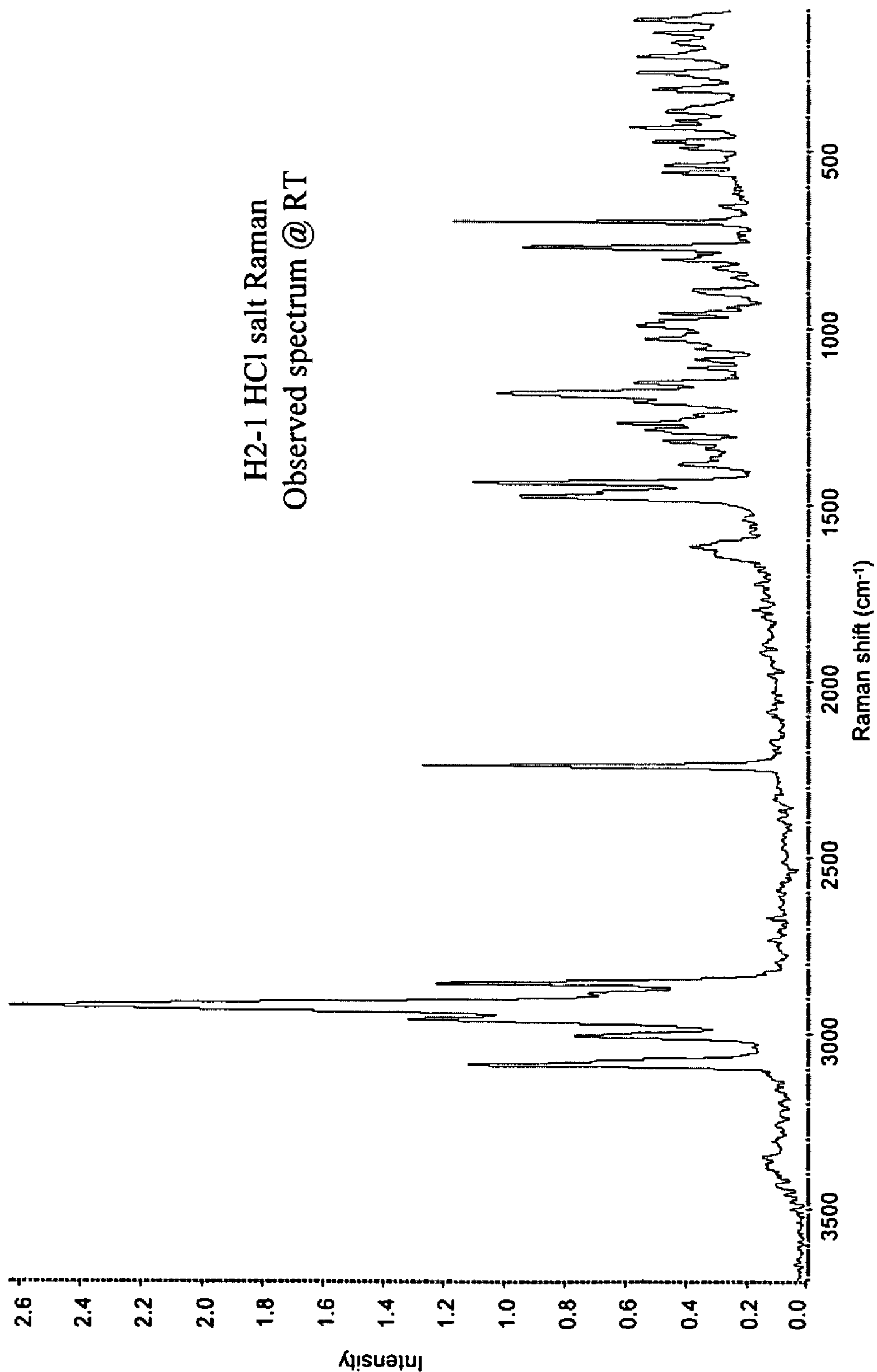
FIG. 9 H2-1 HCl salt Raman
