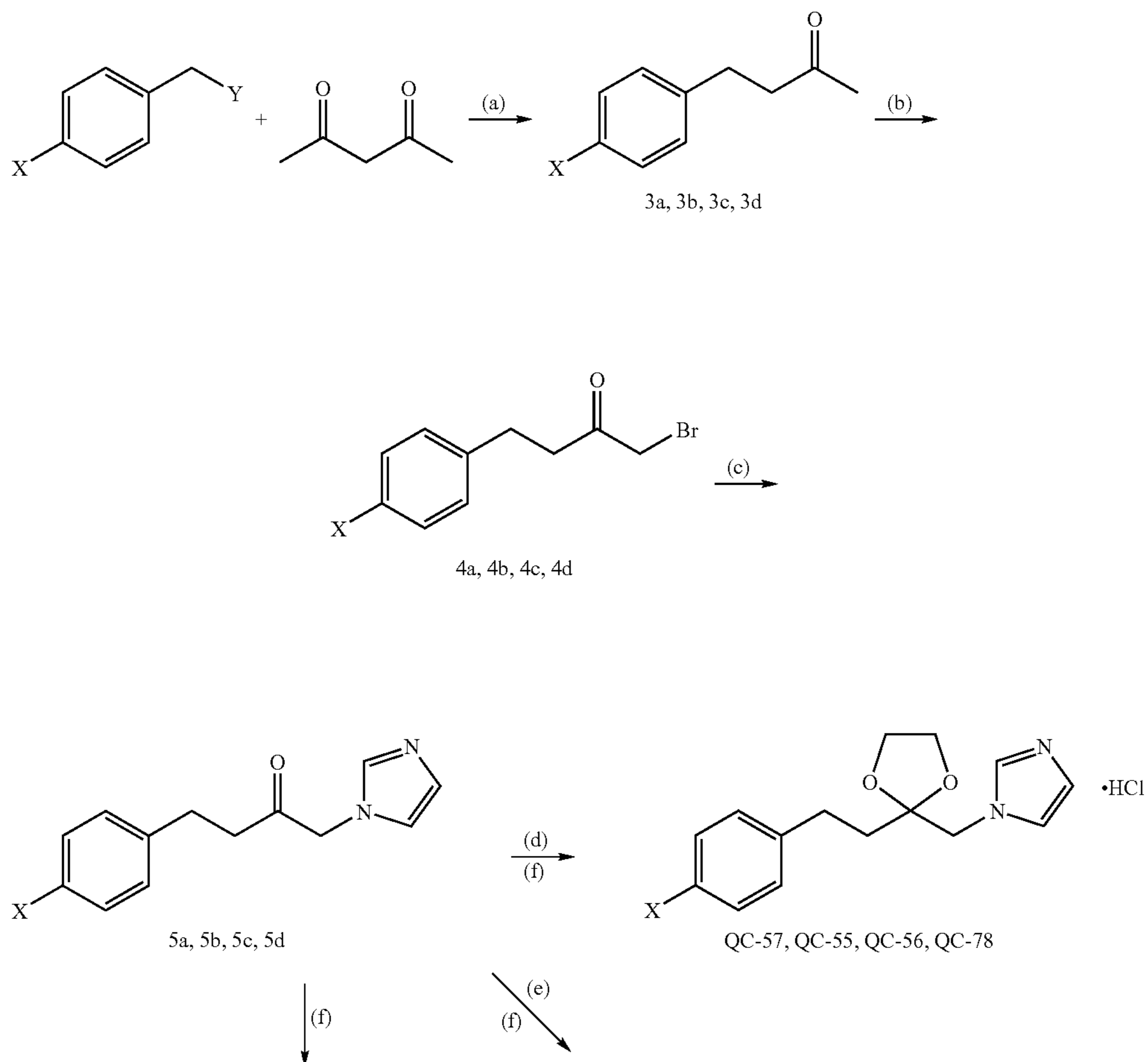
Scheme 2. General approach for the synthesis of imidazole-ketones, imidazole-dioxolanes, and imidazole-alcohols.
