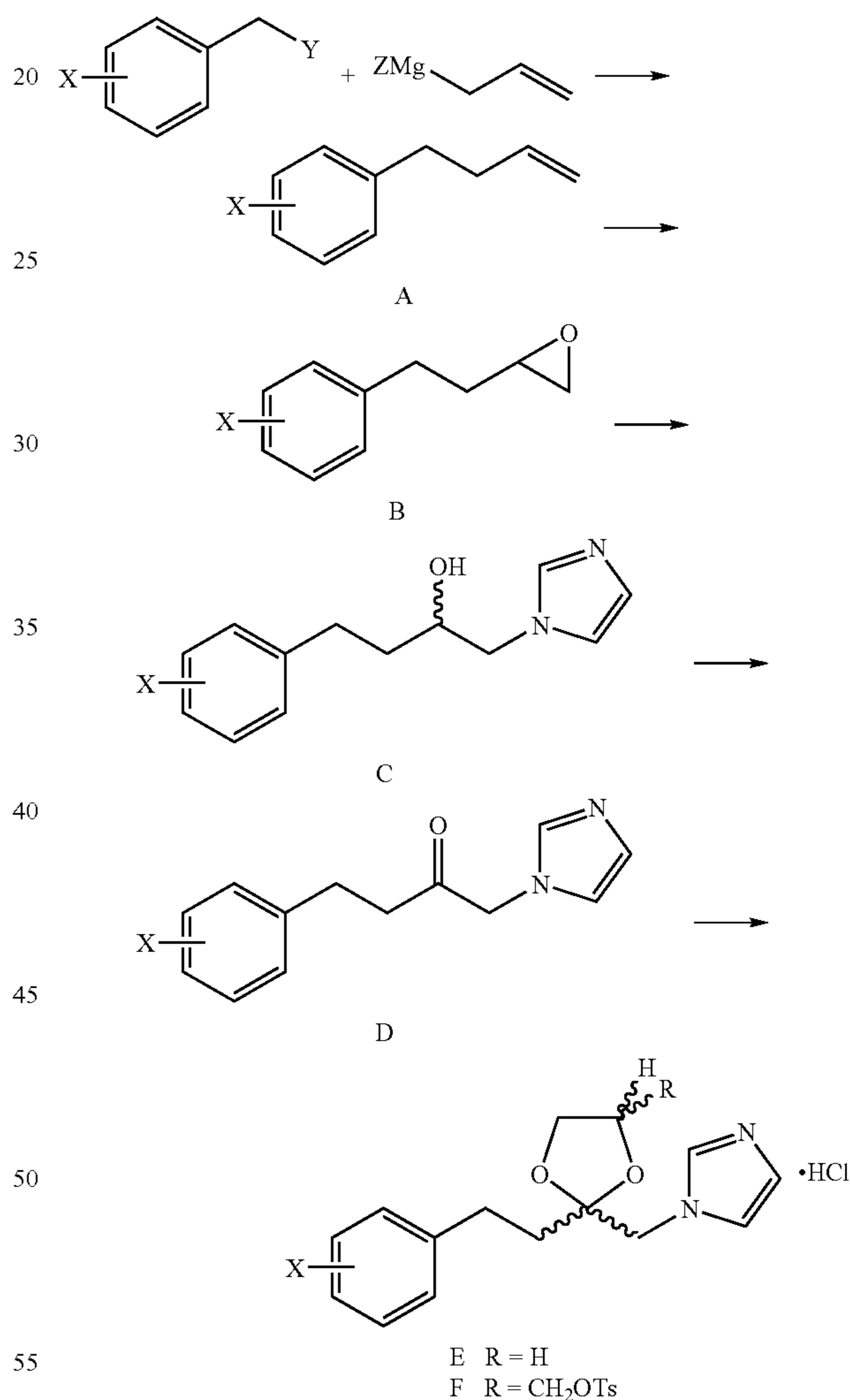
Scheme 7. General approach for the large-scale production of 2-[2-(substituted-phenyl)ethyl]-2-[(1H-imidazol-1-yl)methyl]-1,3-dioxolane derivatives.
