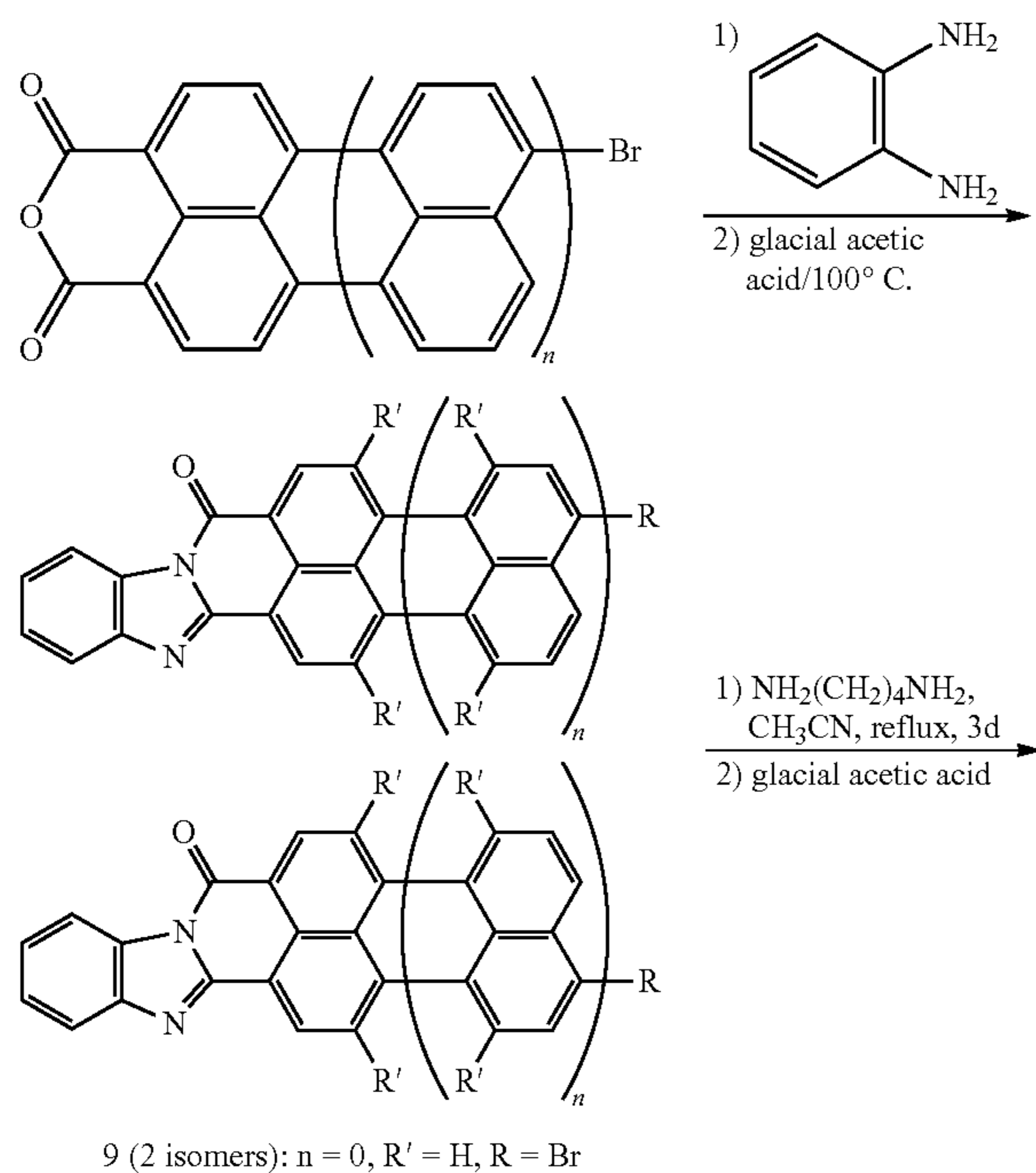
Scheme 5: Synthetic Scheme for Compounds VI
