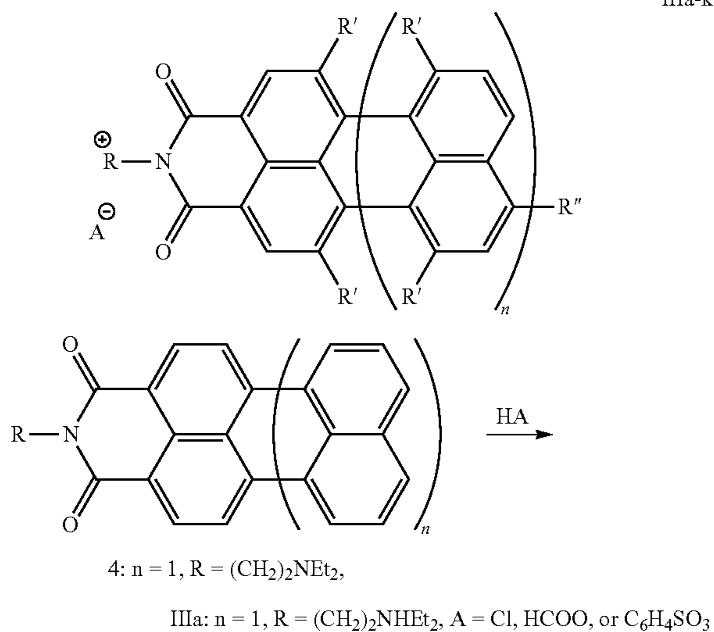
Scheme 2: Synthesis of Monoamides III
