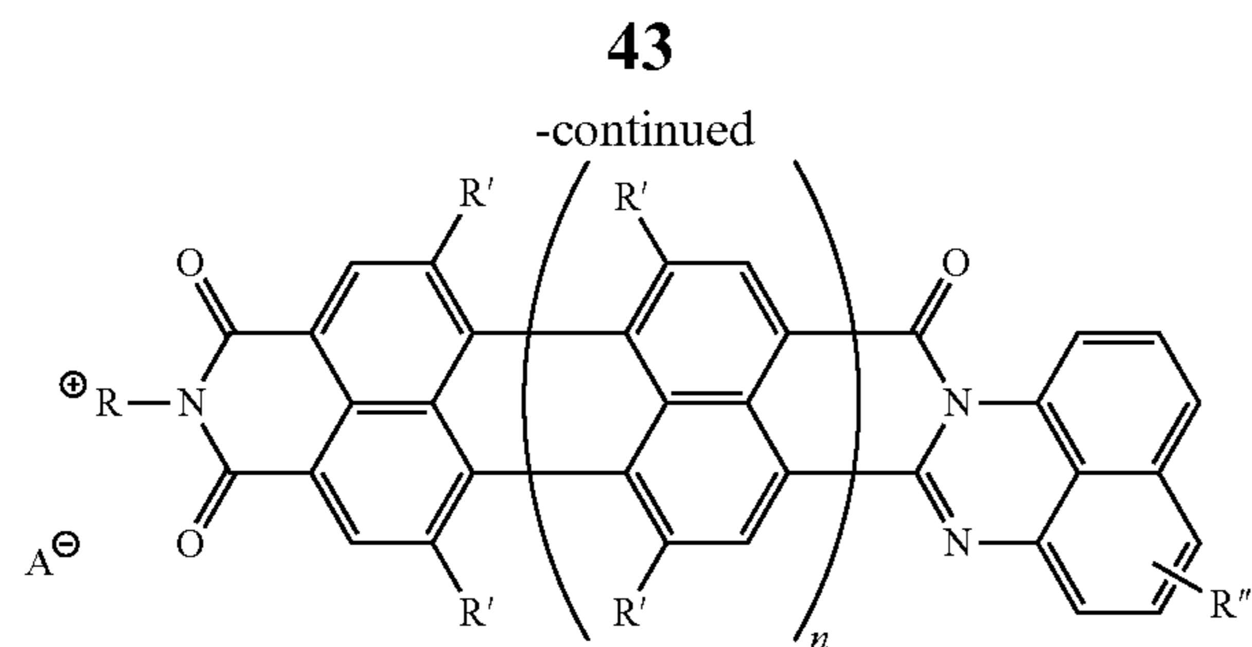
IVf: n = 0 , R' = H , R = (CH_2)_2NHEt_2 , R'' = H , A = CH_3COO^- :
