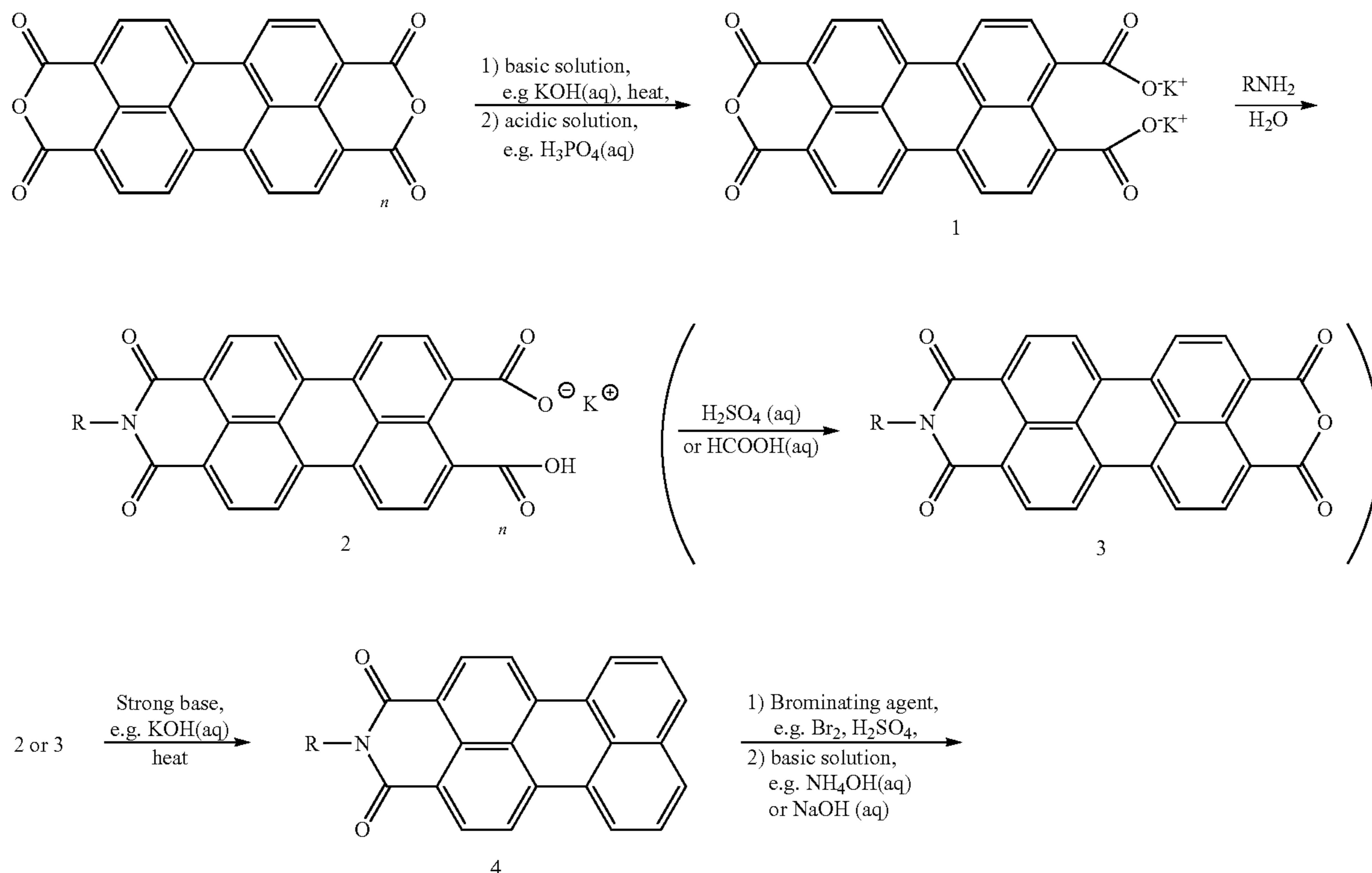
Scheme 1. Synthesis of compounds of Formula I.
