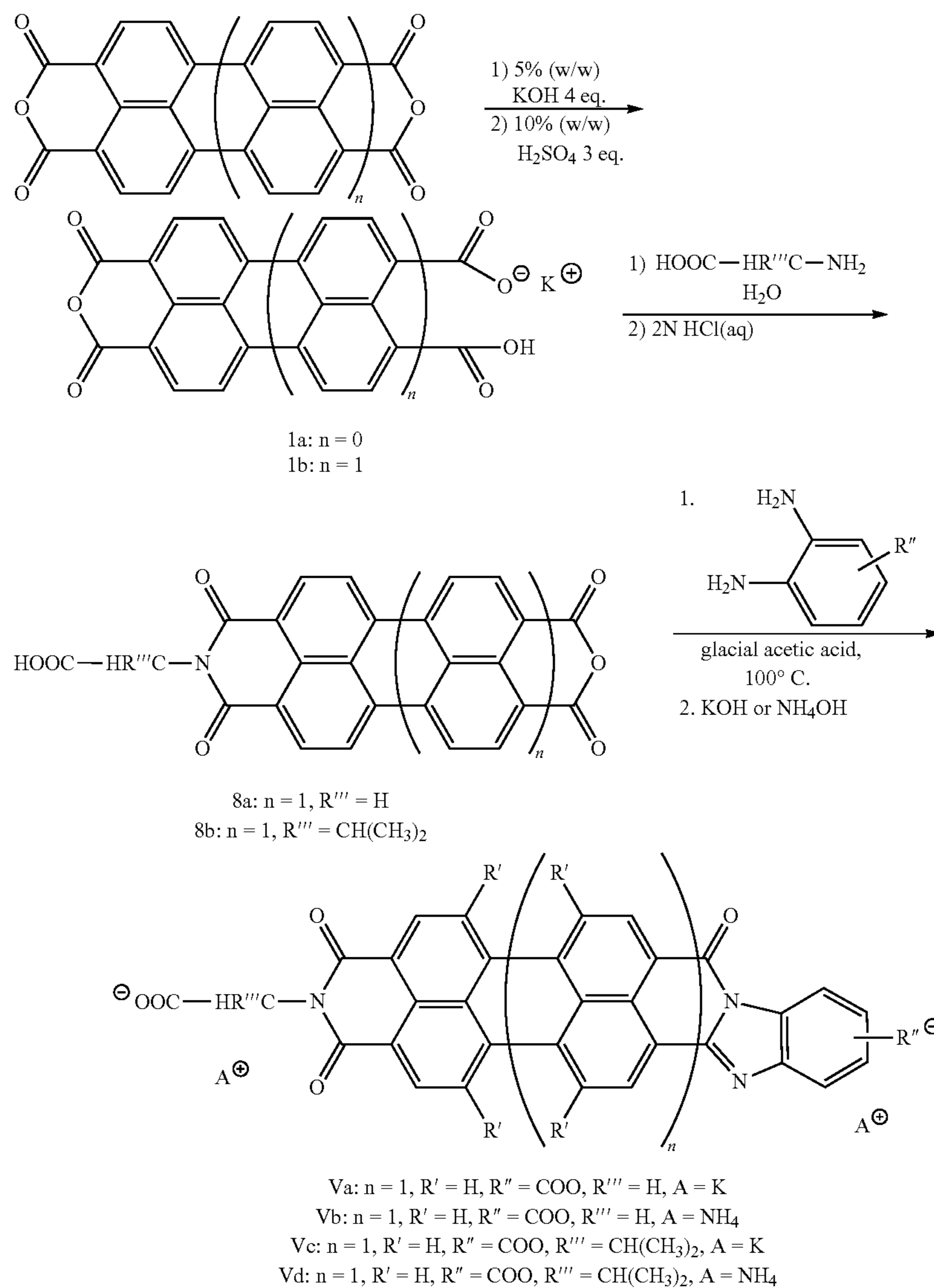
Scheme 4. Synthetic scheme for compounds V.
