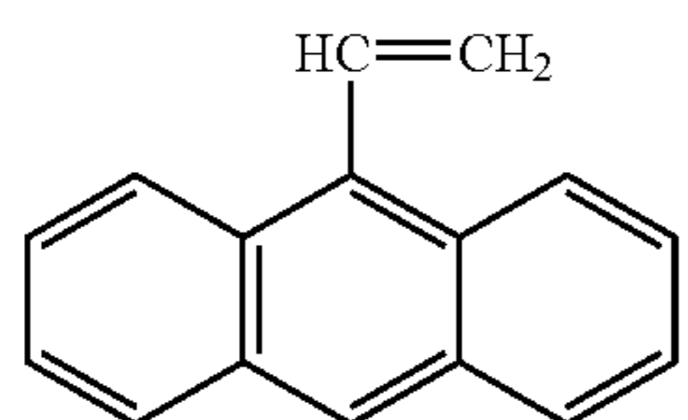
9-vinyl anthracene
