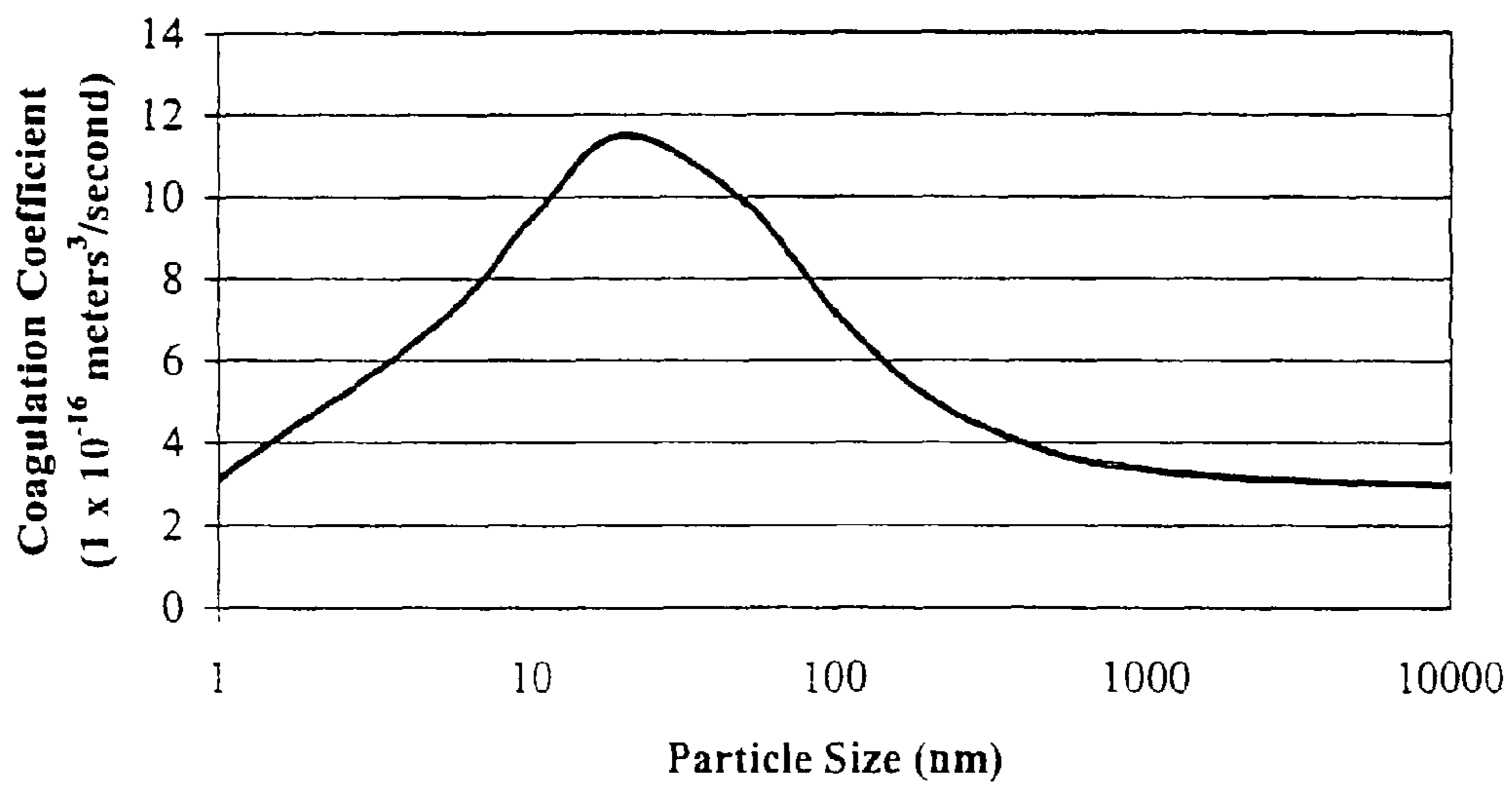
Coagulation Coefficient vs. Particle Size
