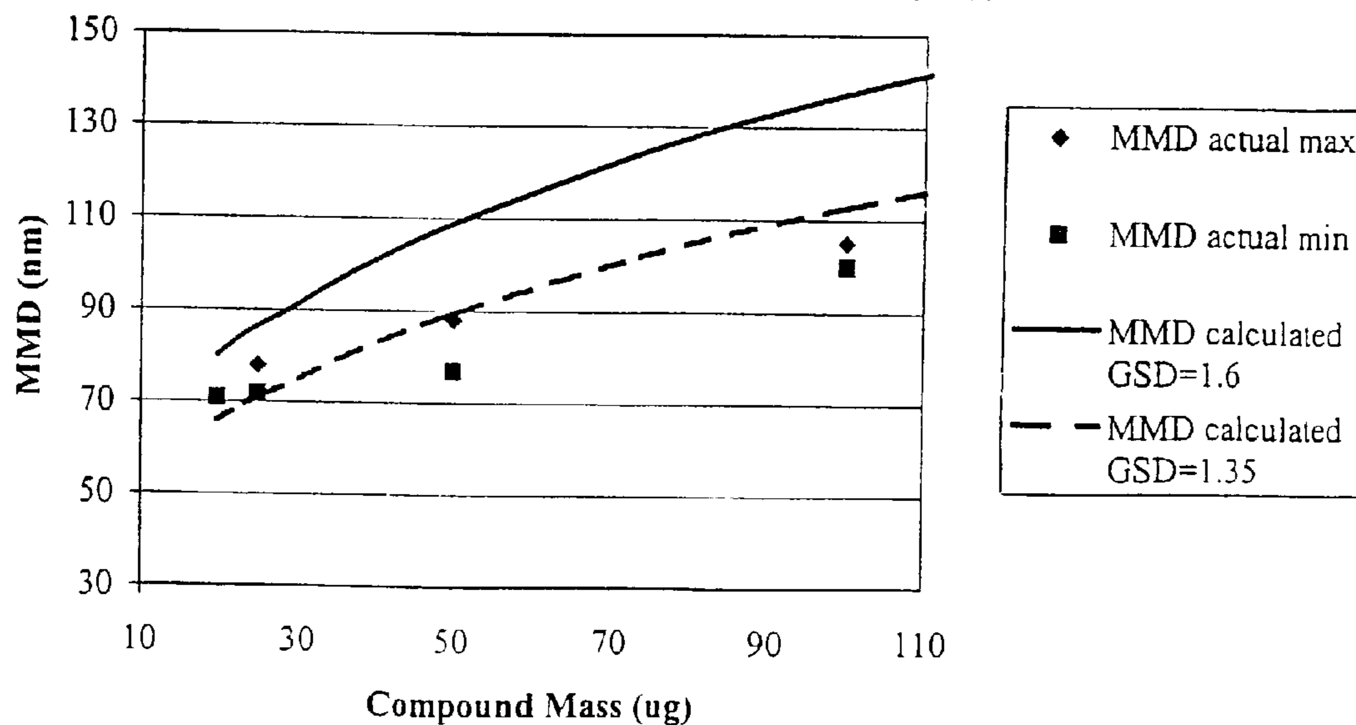
Actual vs Calculated Particle Diameter (MMD) for Number Concentration of 0.5 \times 10^9/cc
