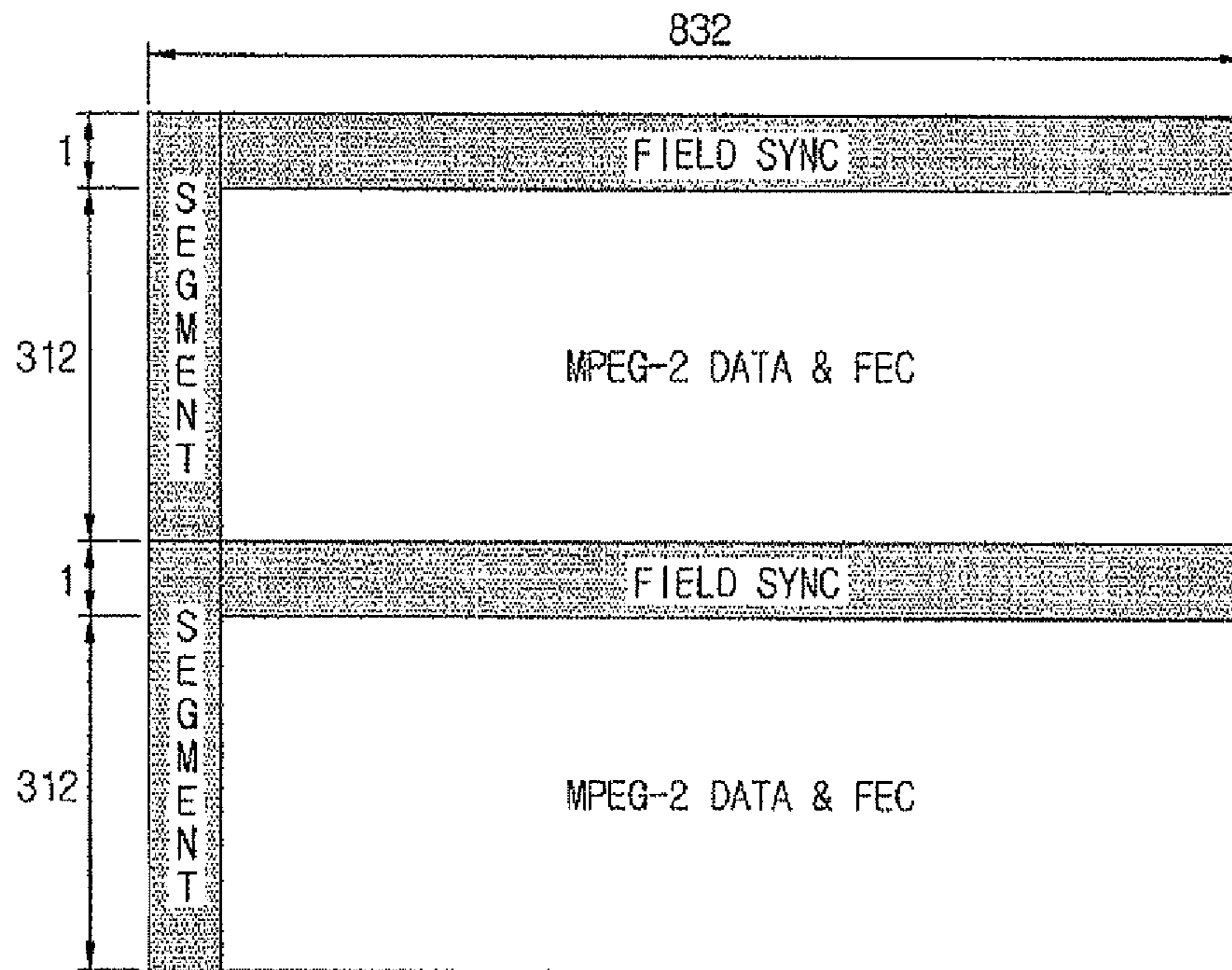
FIG. 2 (RELATED ART)
