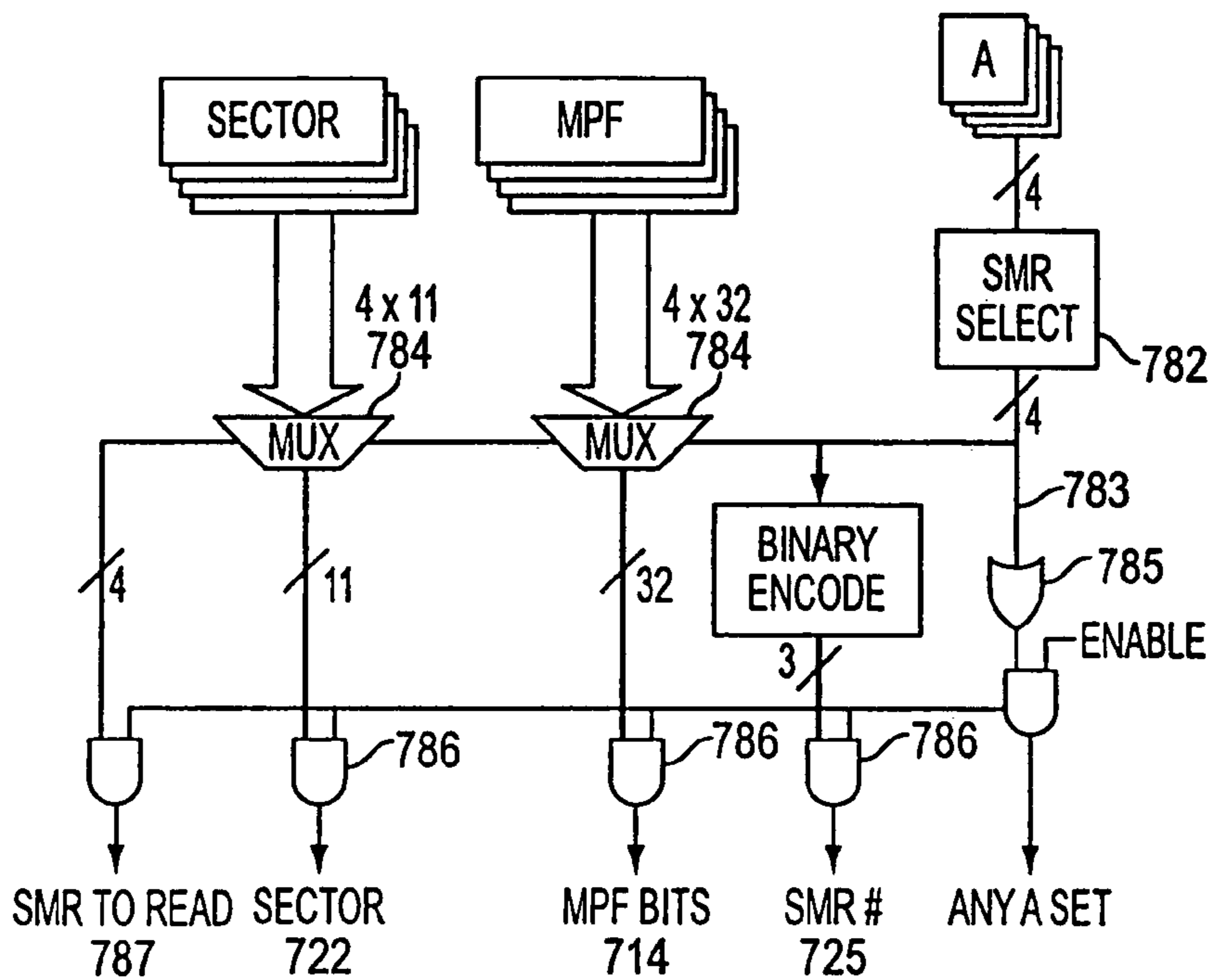
DMU_Status read FIG. 7H
