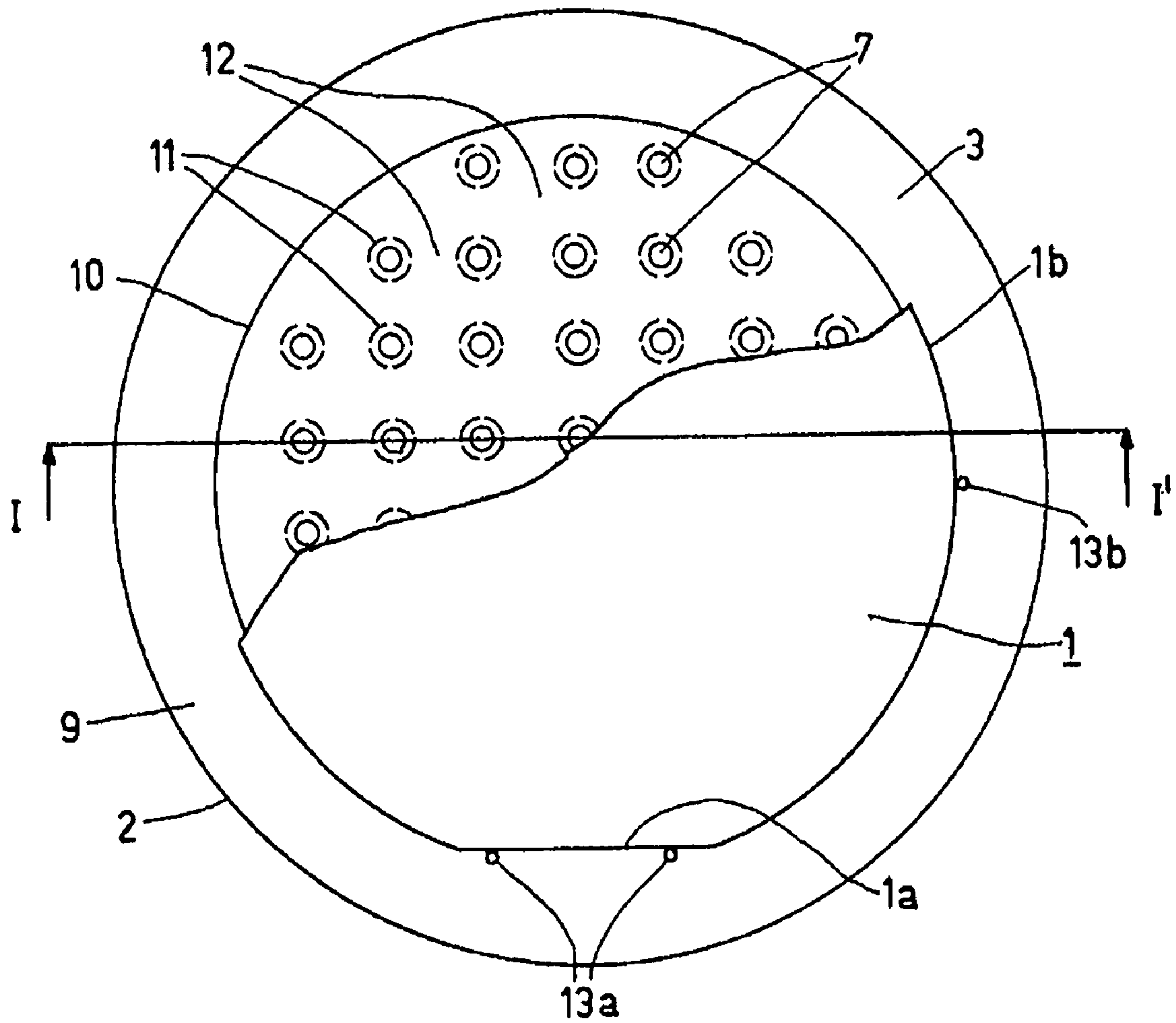
Fig. 3 PRIOR ART
