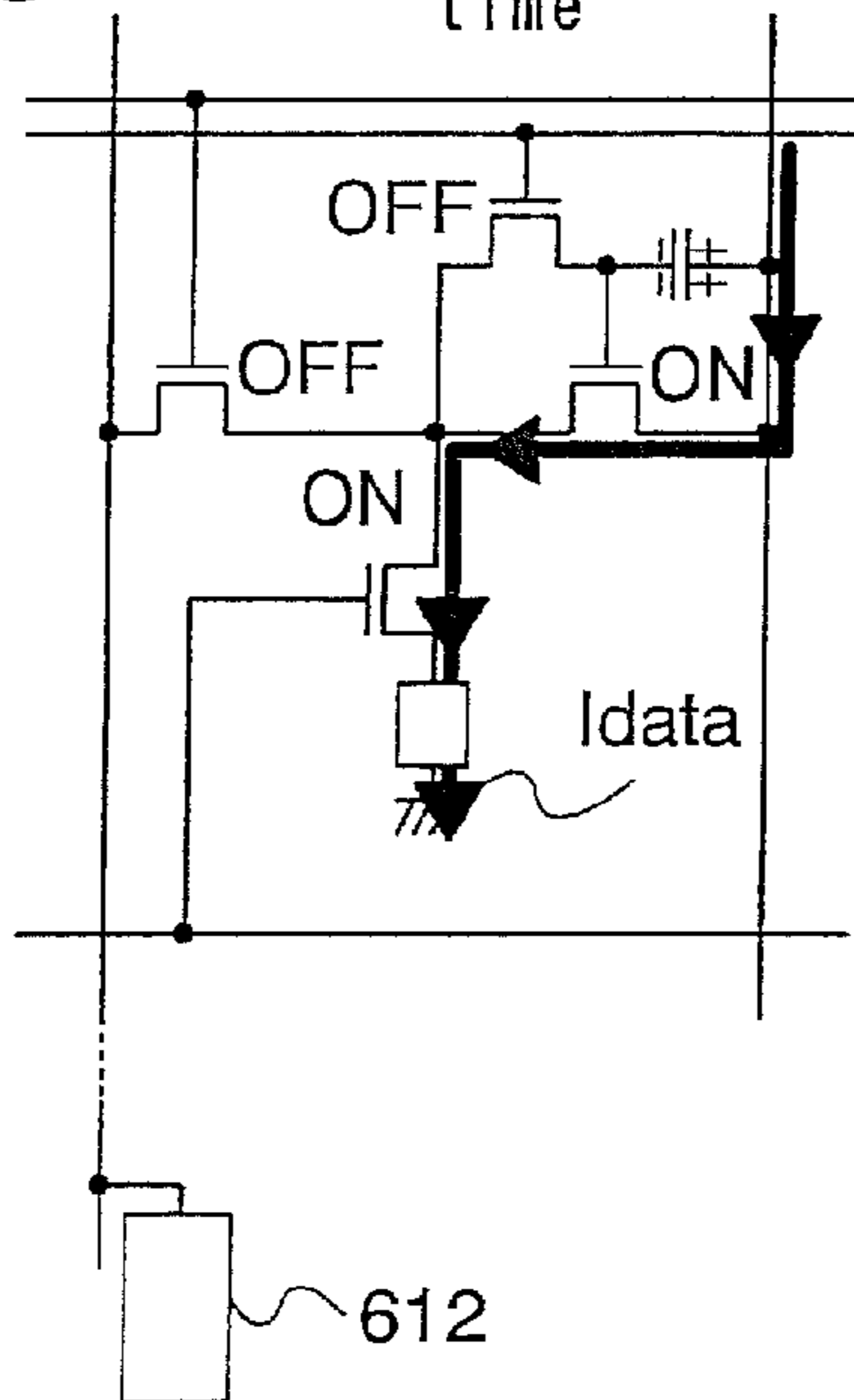
Fig. 17C light emitting time
