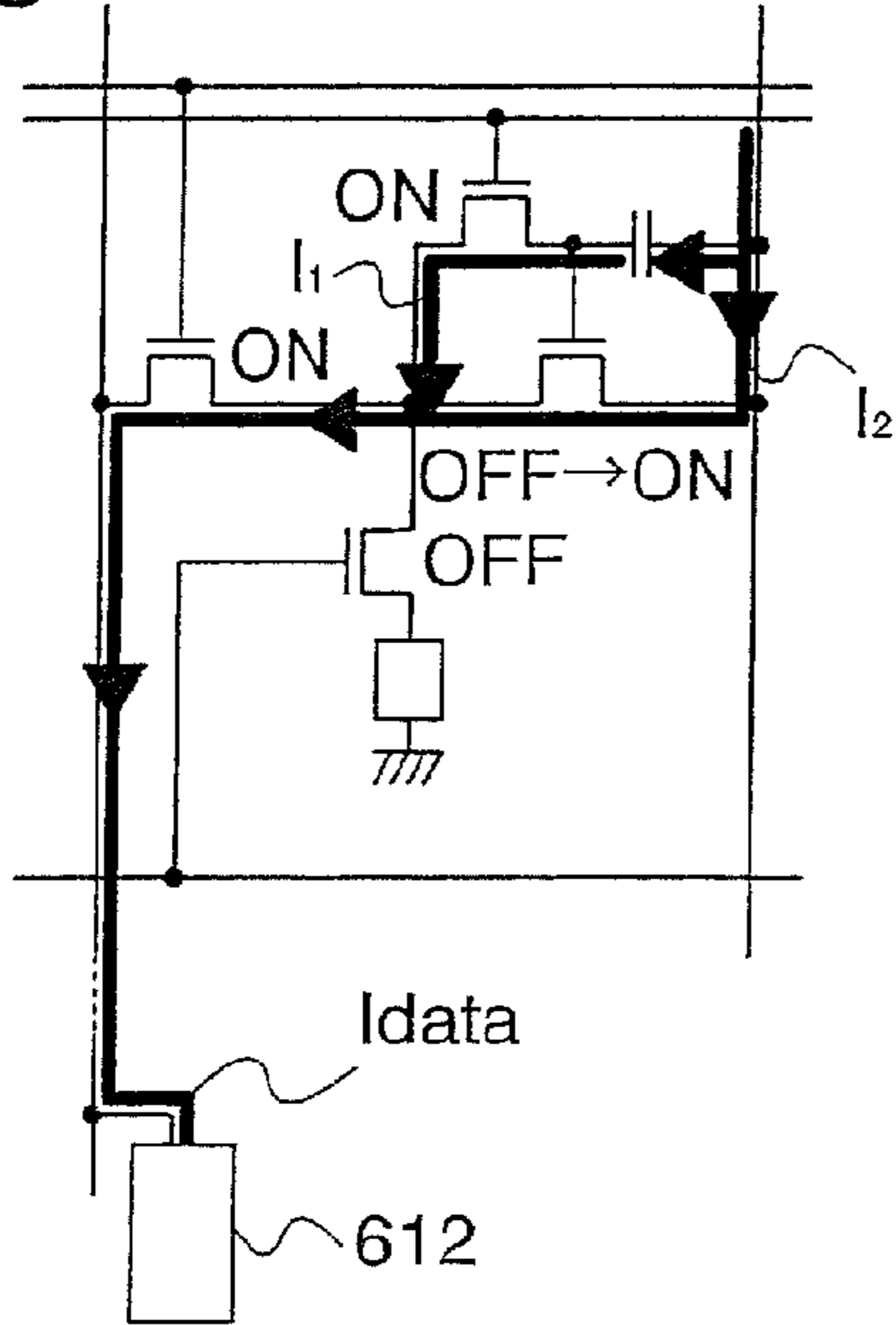
Fig. 17A signal input time
