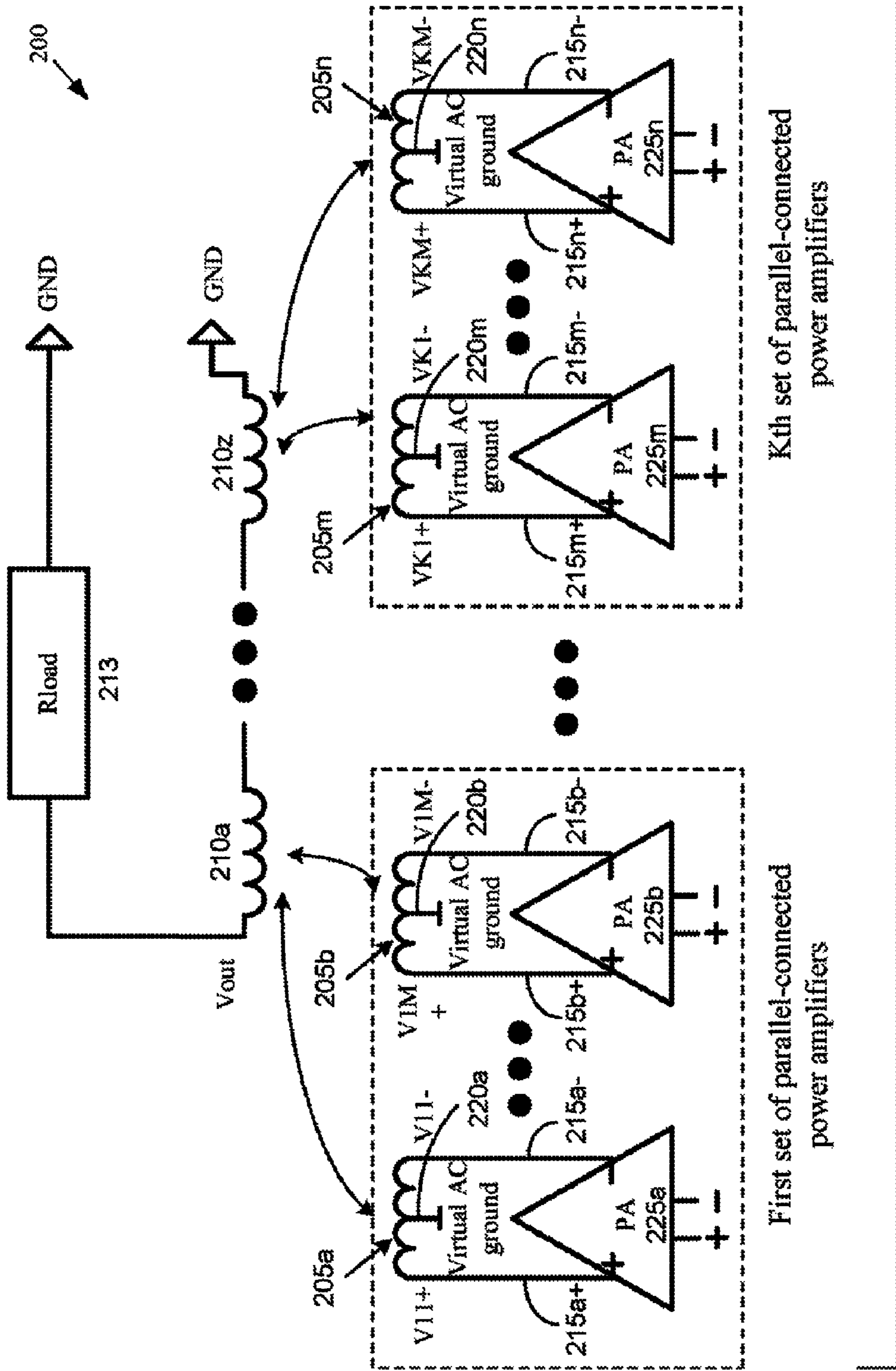
K sets of parallel-connected power amplifiers
