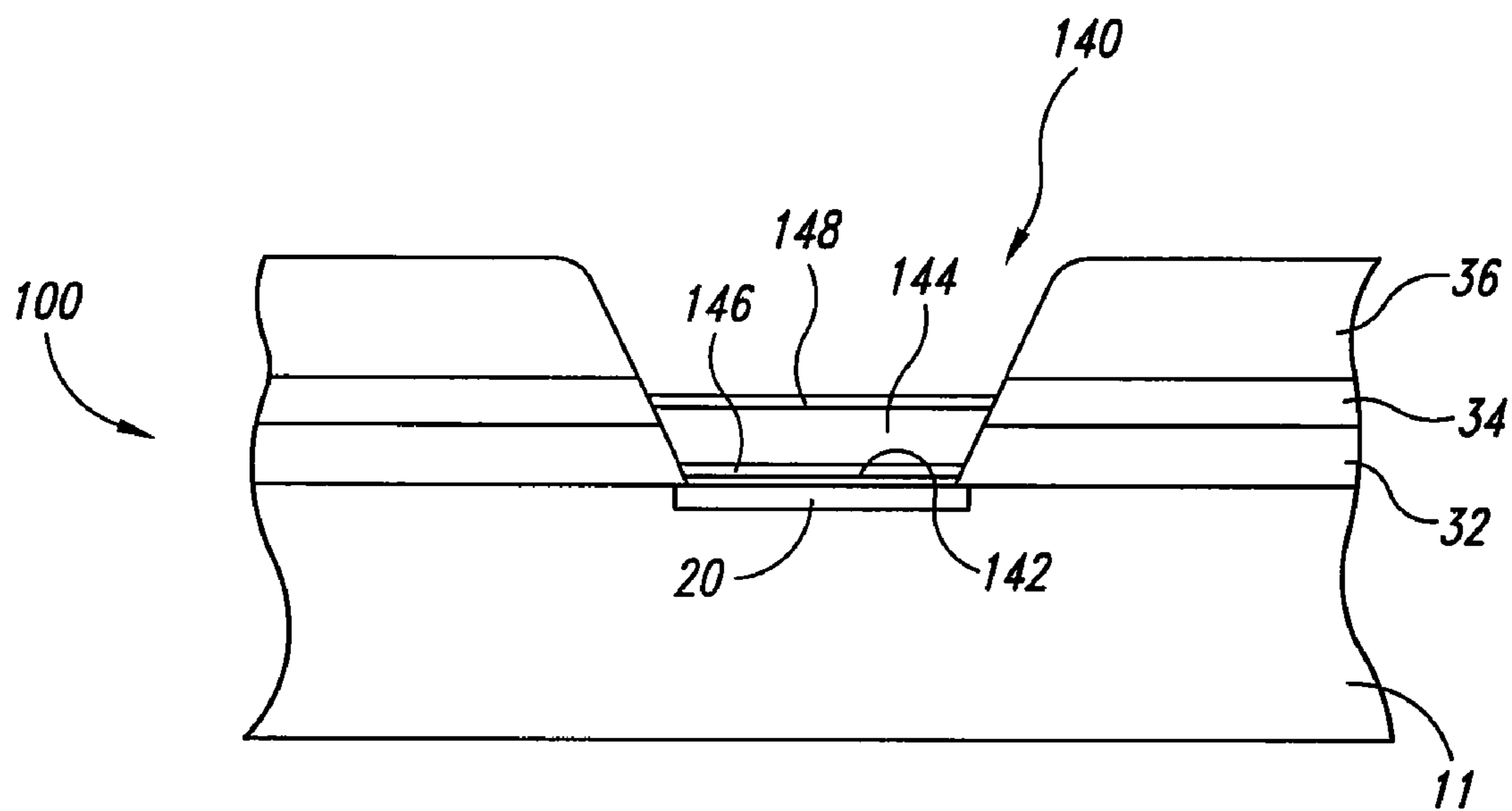
Fig. 2 (Prior Art)
