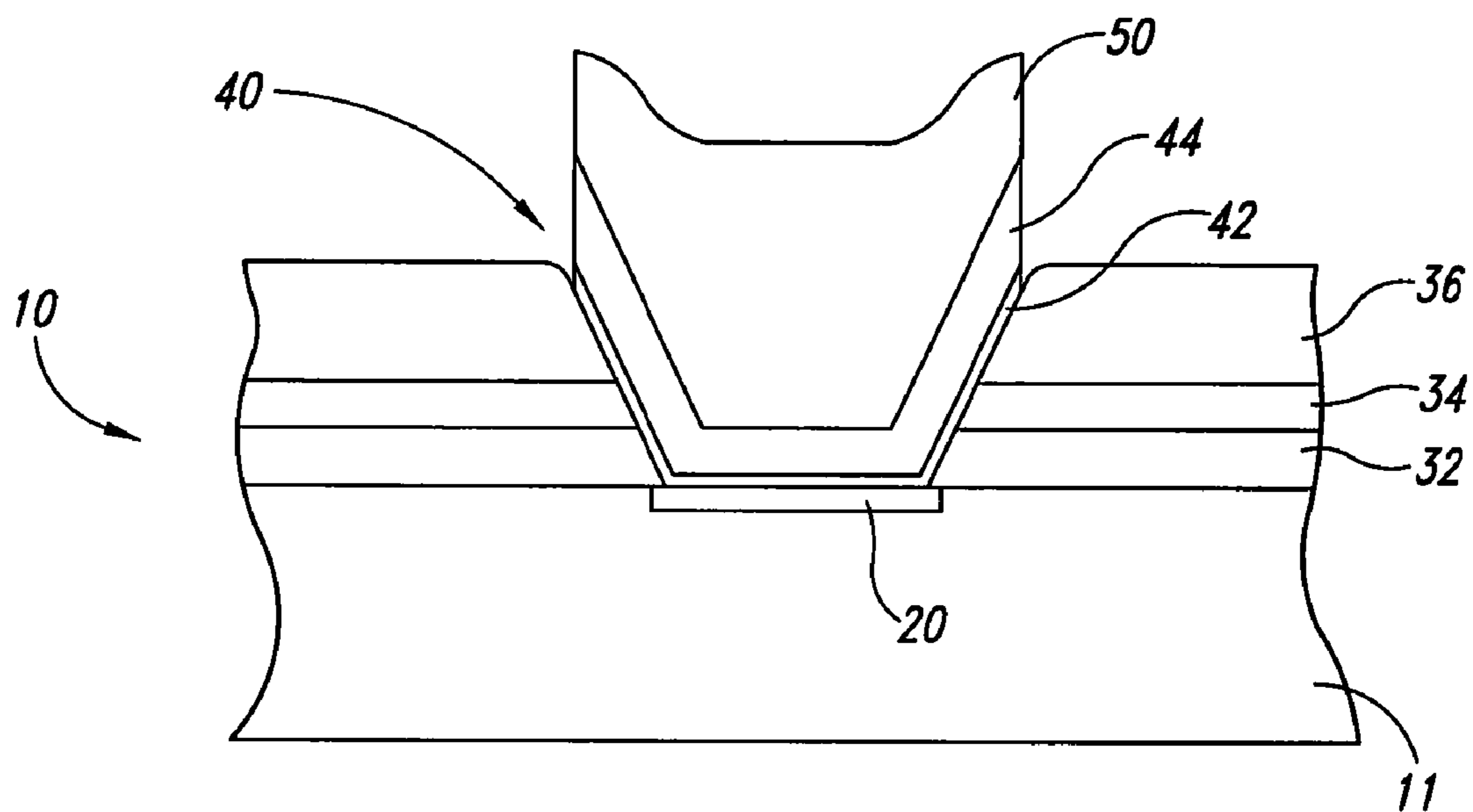
Fig. 1 (Prior Art)
