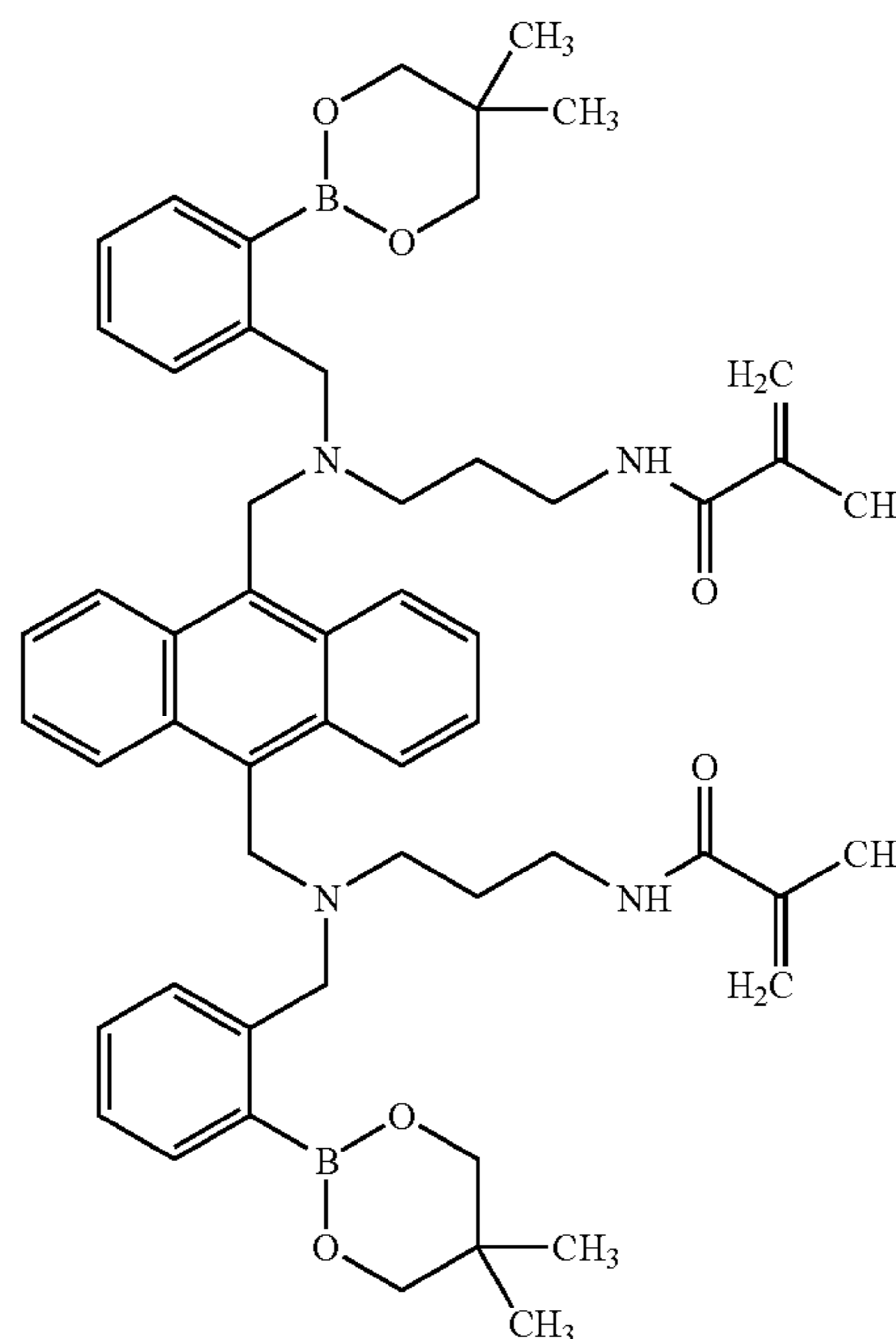
B. 9,10-bis[N-[2-(5,5-dimethyl-[1,3,2]dioxaborinan-2-yl)benzyl]-N-[3-(methacrylamido)propylamino]methylanthracene
