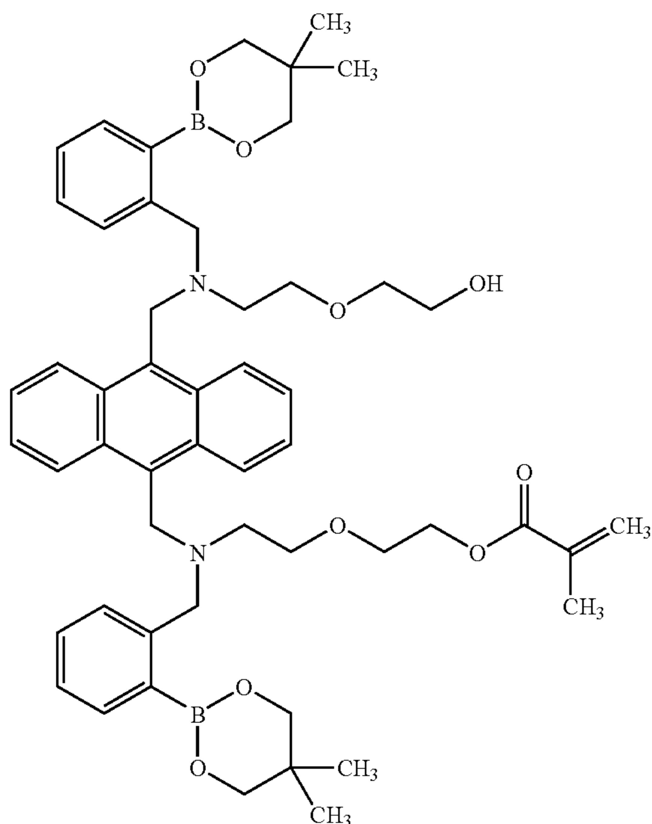
C. 9-[N-[2-(5,5-dimethyl-1,3,2)dioxaborinan-2-yl)benzyl]-N-[2-(2-methacryloyloxyethoxy)ethylamino]methyl]-10-[N-[2-(5,5-dimethyl-1,3,2)dioxaborinan-2-yl)benzyl]-N-[2-(2-hydroxyethoxy)ethylamino]methyl]anthracene. (Single-methacrylate monomer)
