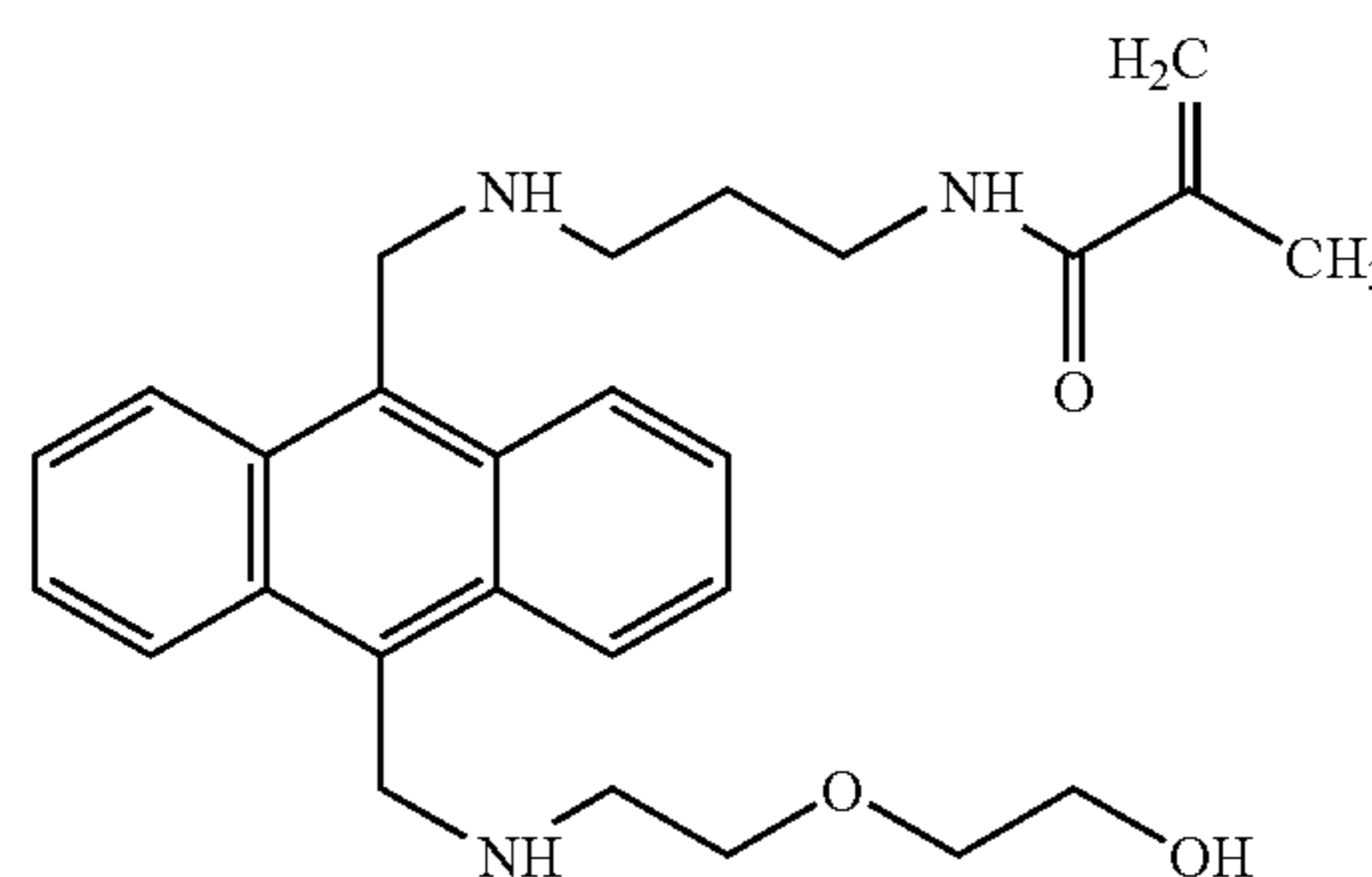
B. 9-[[2-(2-hydroxyethoxy)ethylamino]methyl]-10-[[[3-methacrylamido)propylamino]methyl]anthracene
