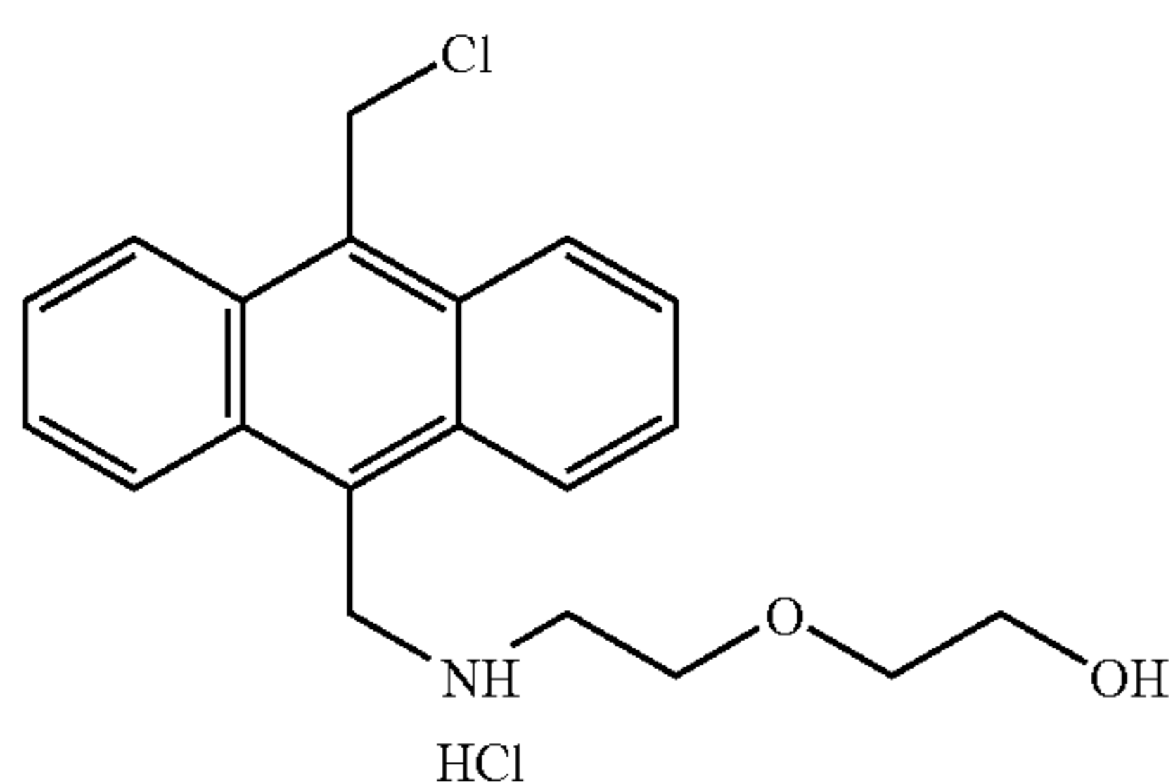
A. 9-chloromethyl-10-[[2-(2-hydroxyethoxy)ethylamino]-methyl]anthracene hydrochloride salt
