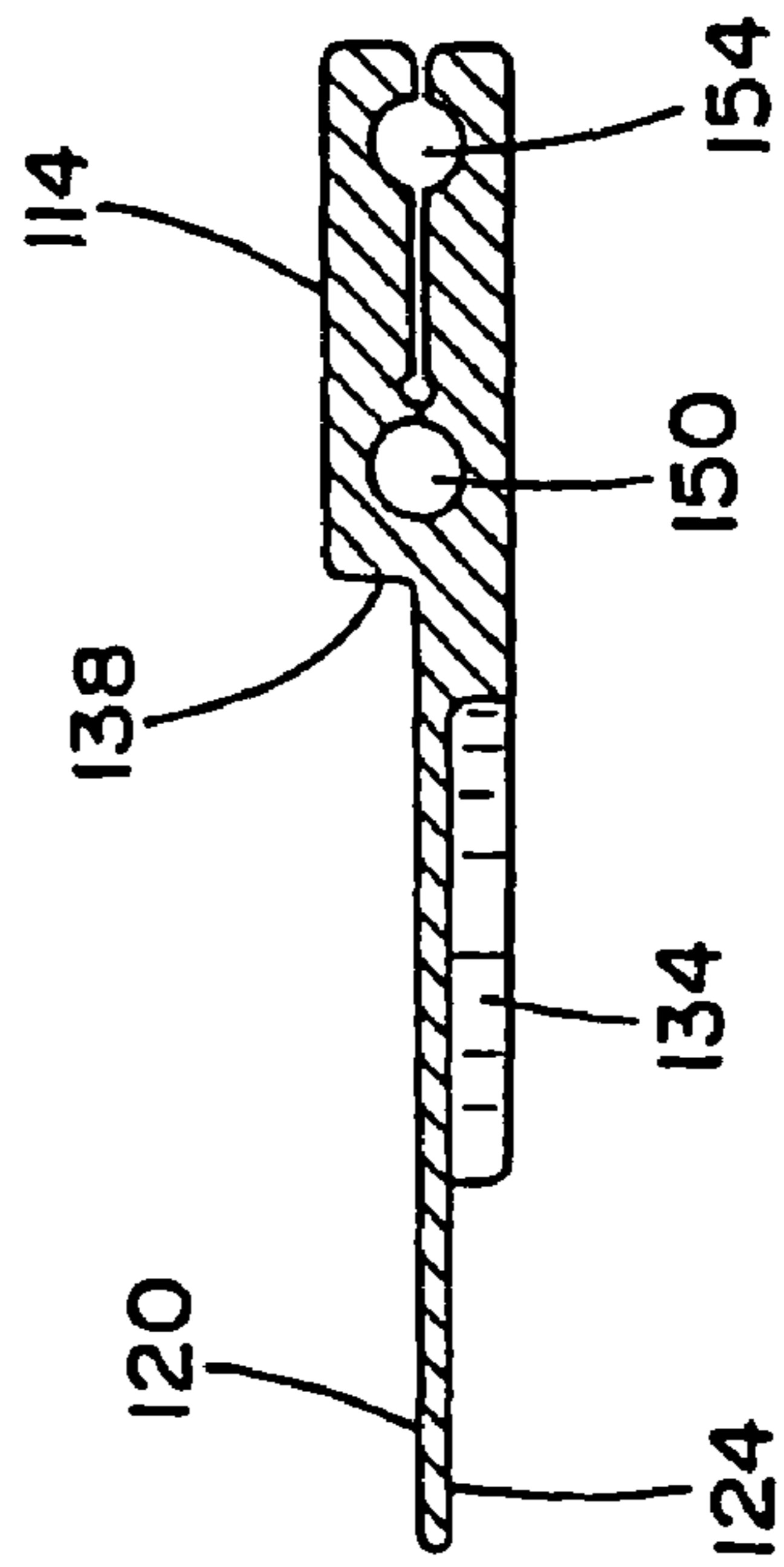
Section A-A FIG. 10c
