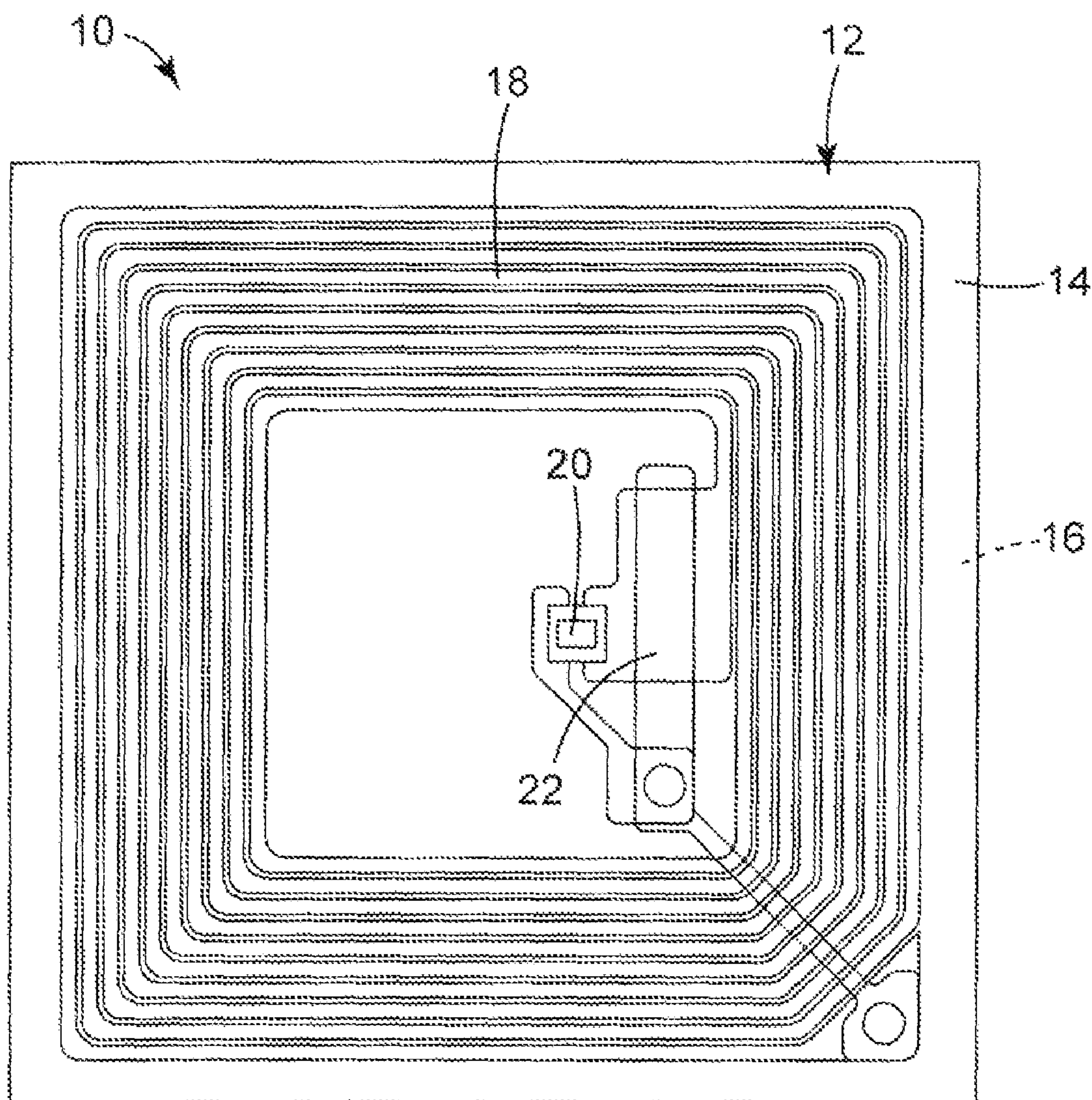
FIG. 1 (Prior Art)
