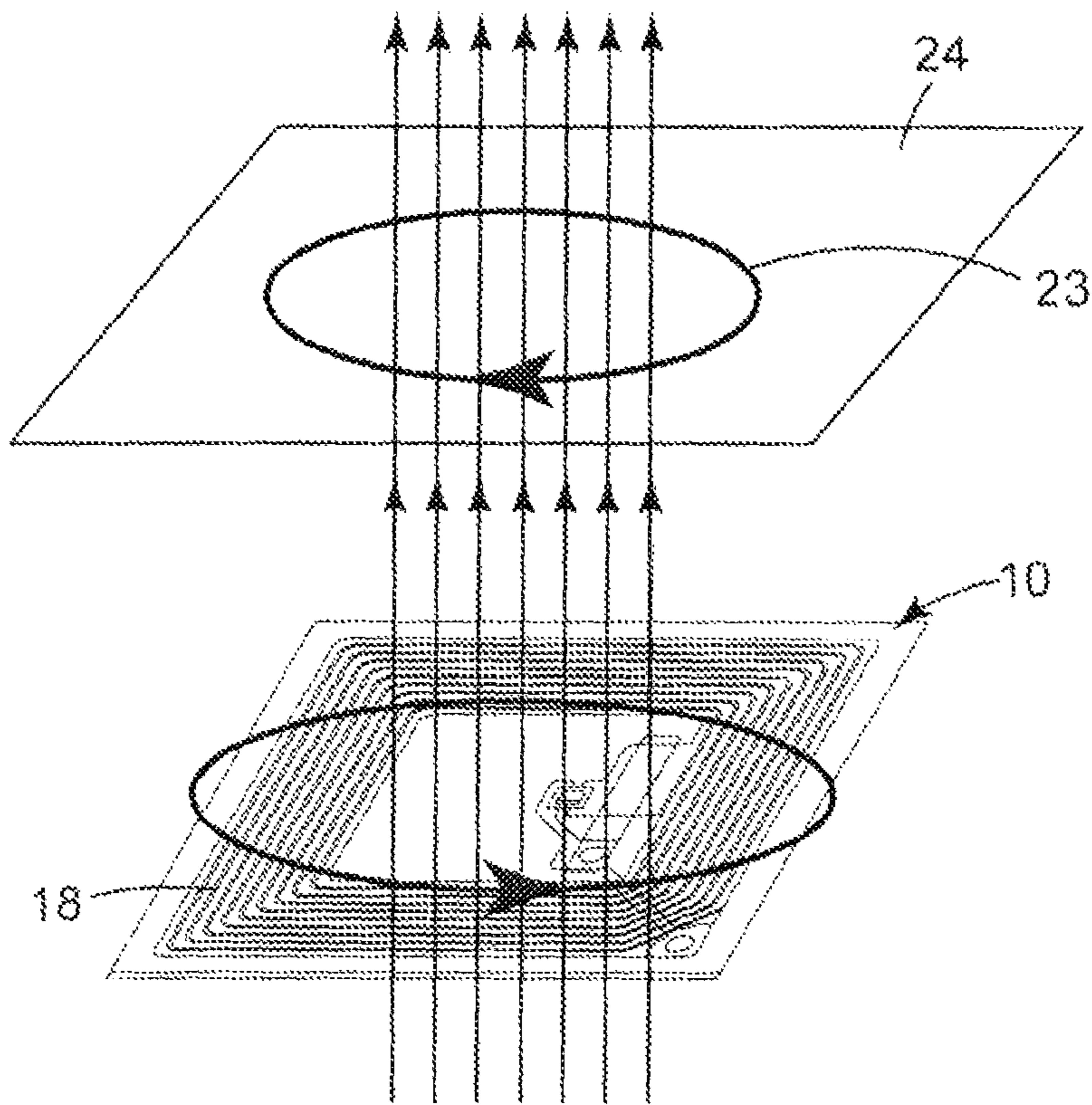
FIG. 3 (Prior Art)
