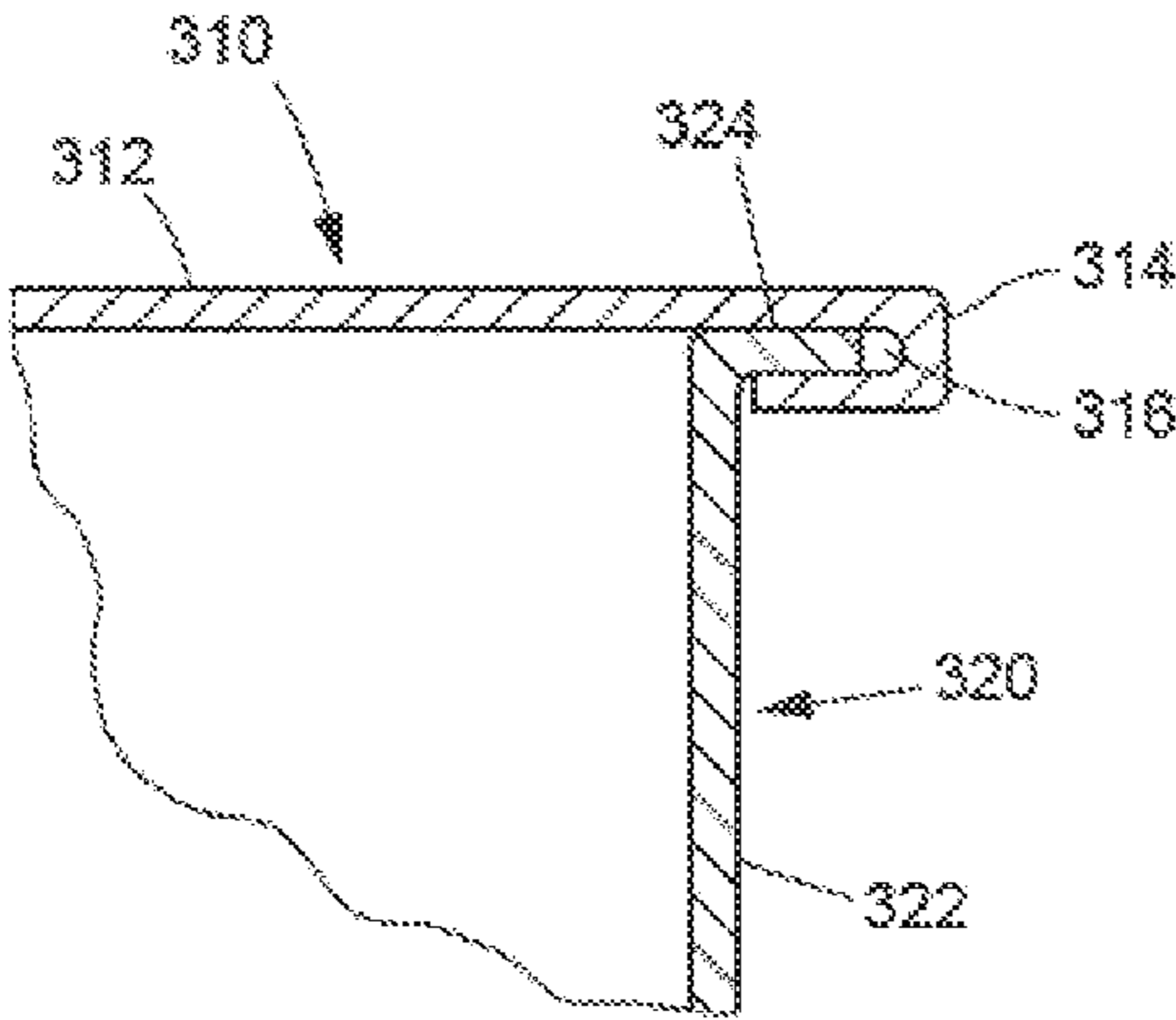
FIG. 3 PRIOR ART
