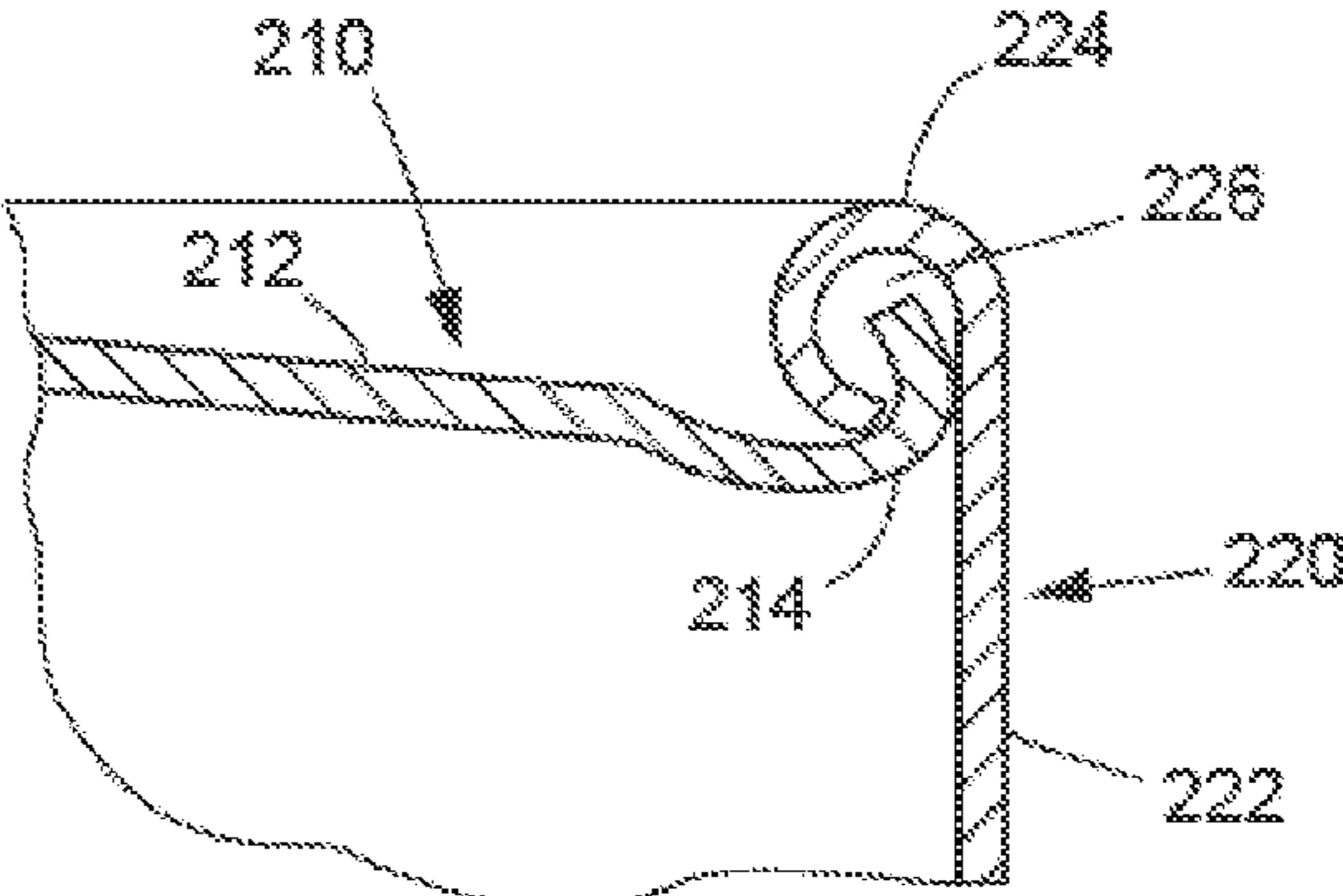
FIG. 2 PRIOR ART
