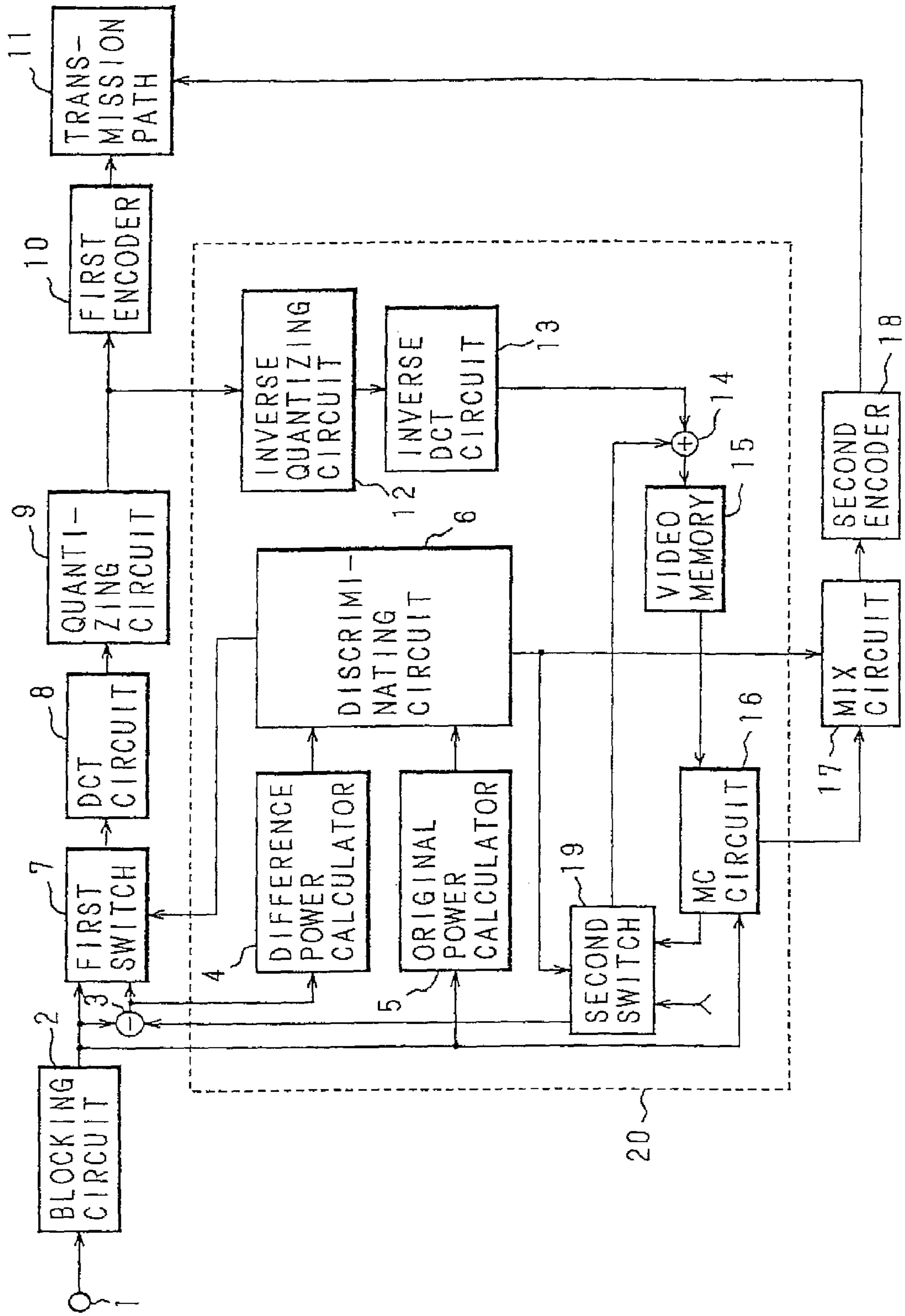
Fig. 2 Prior Art
