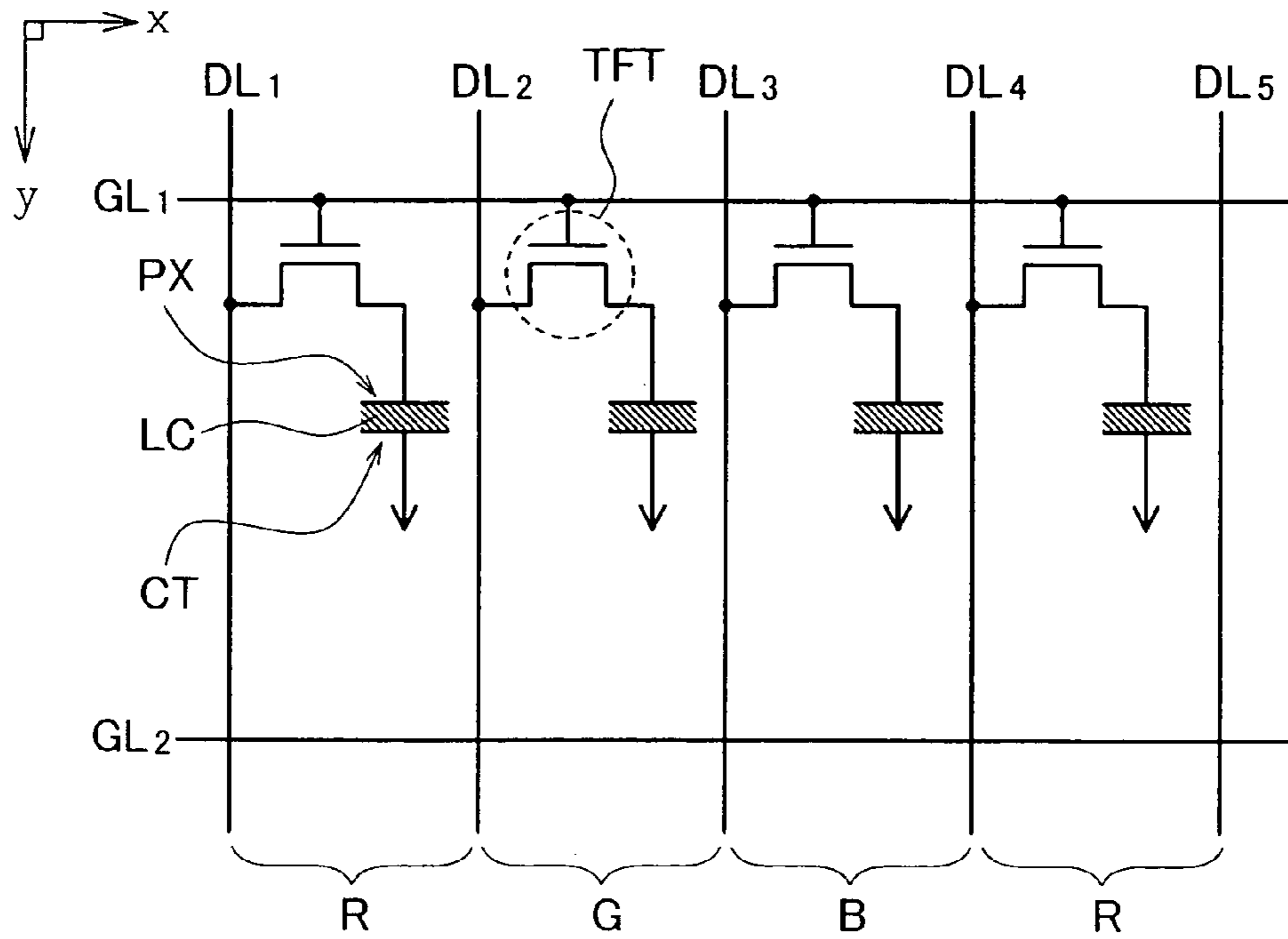
FIG. 7 Prior Art
