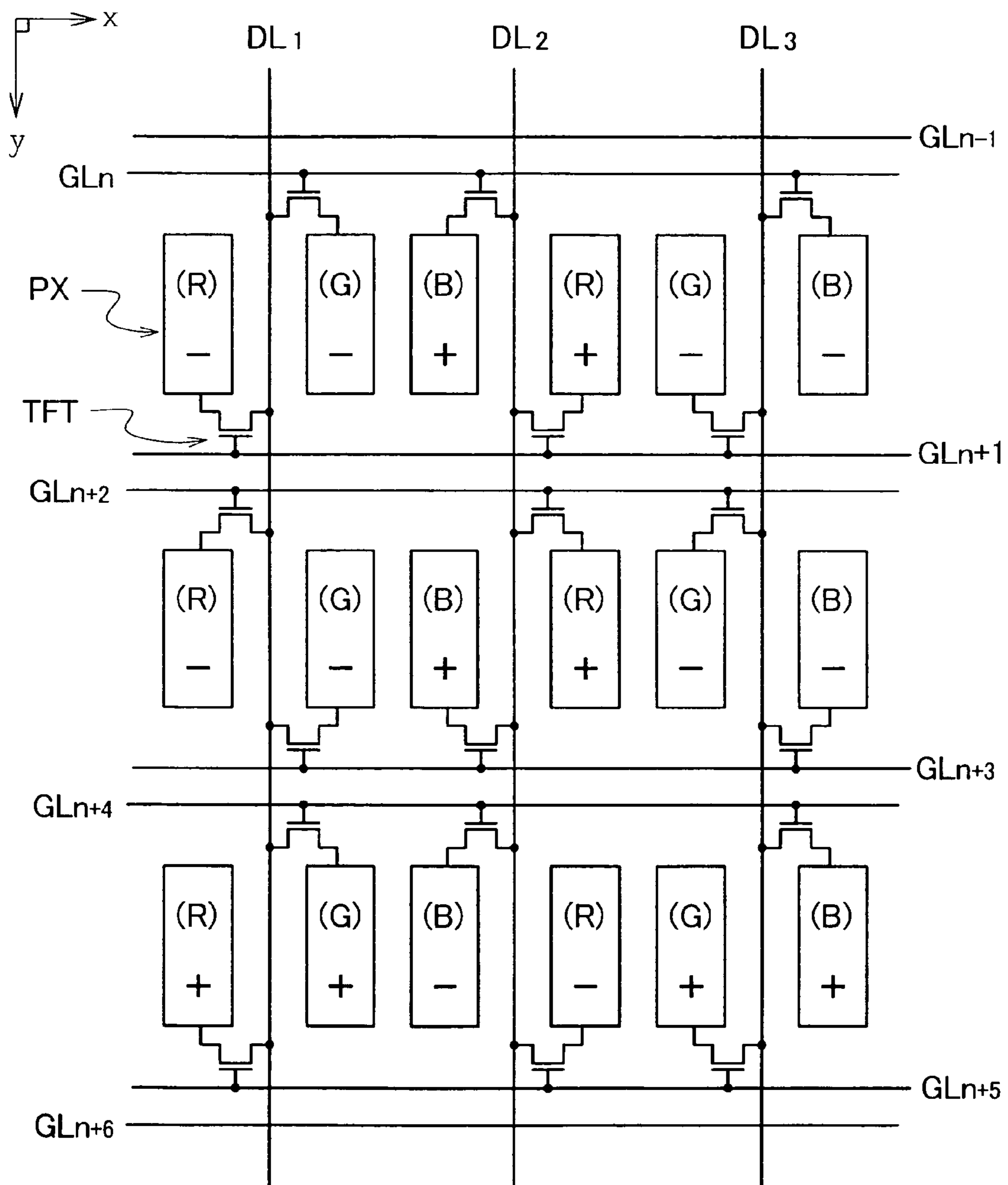
FIG. 10 Prior Art
