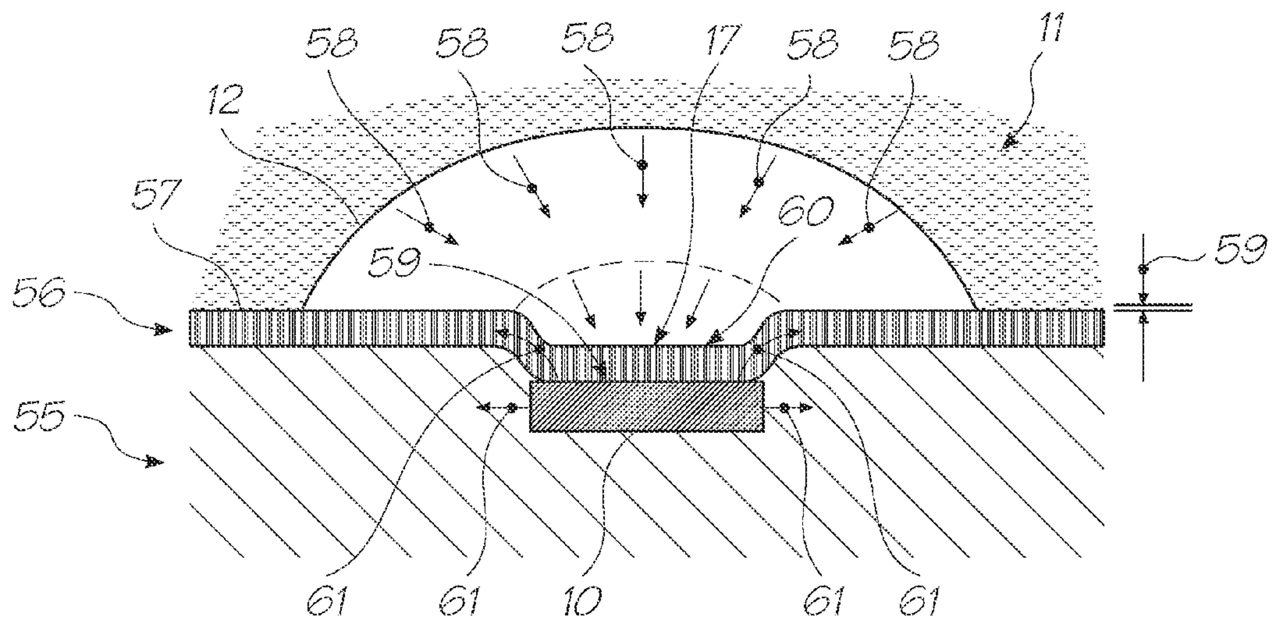
FIG. 47 (PRIOR ART)
