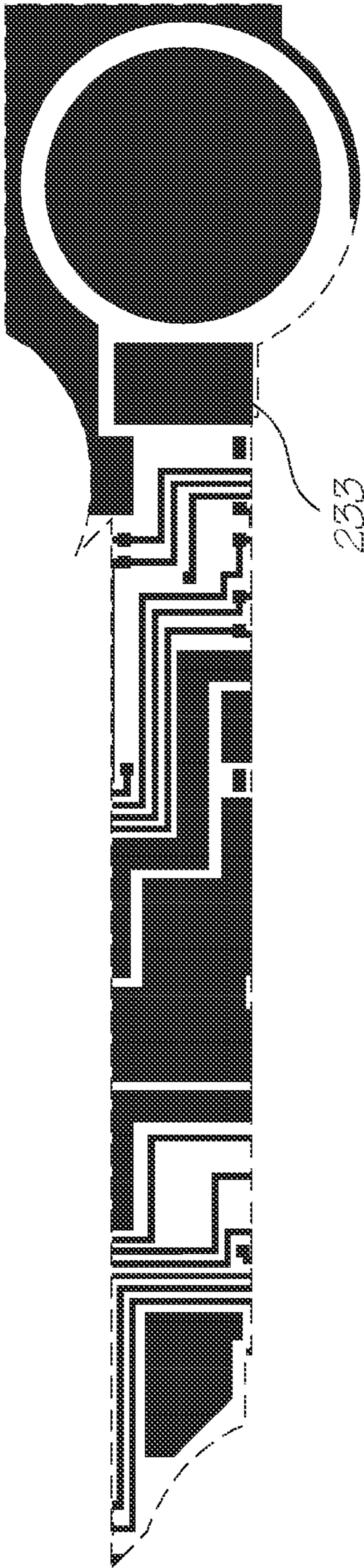
Metal 2 mask
