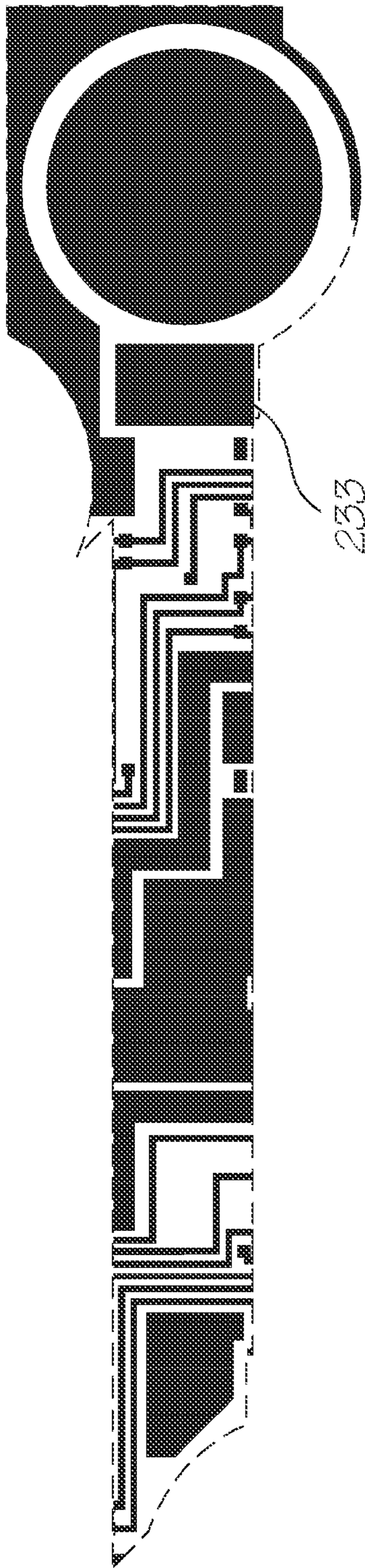
Metal 2 mask
