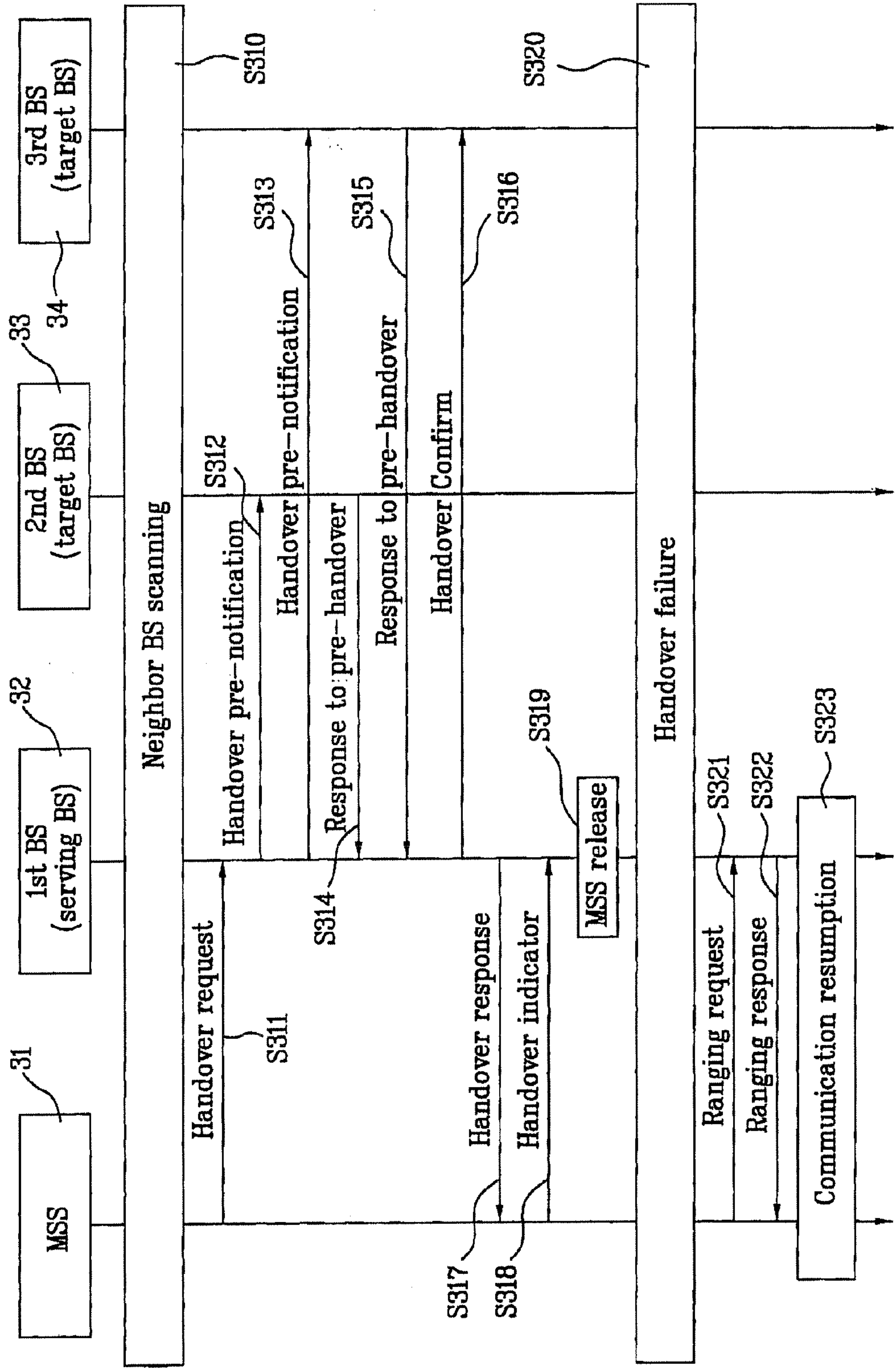
FIG. 3 Related Art
