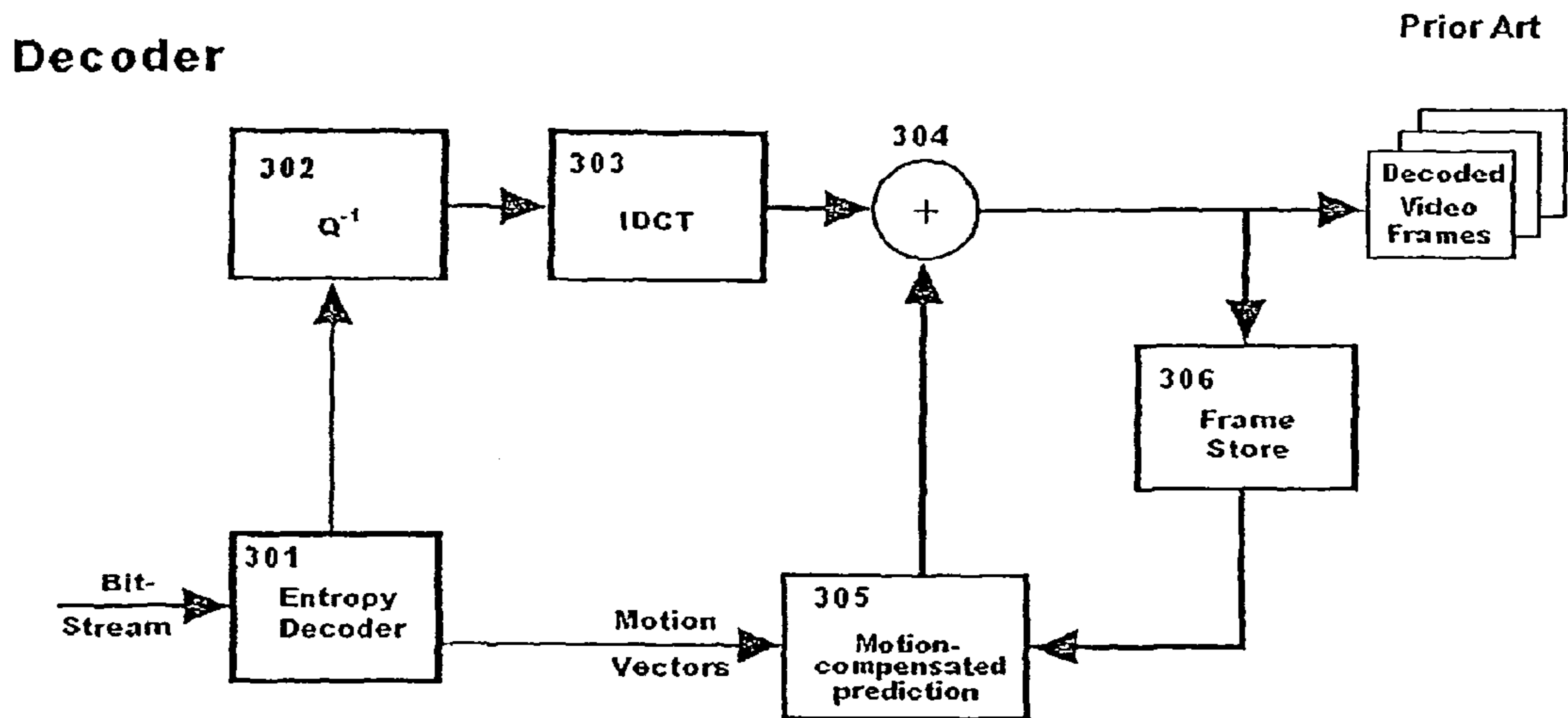
Figure 3 — Block Diagrams of Standard H.263 Encoder and Decoder
