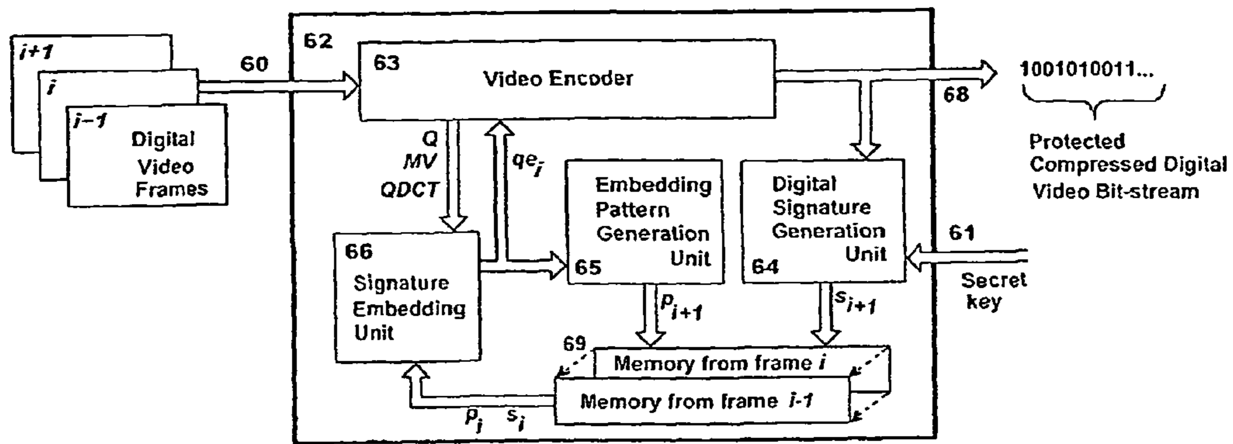
Figure 6 — Augmented Video Encoder
