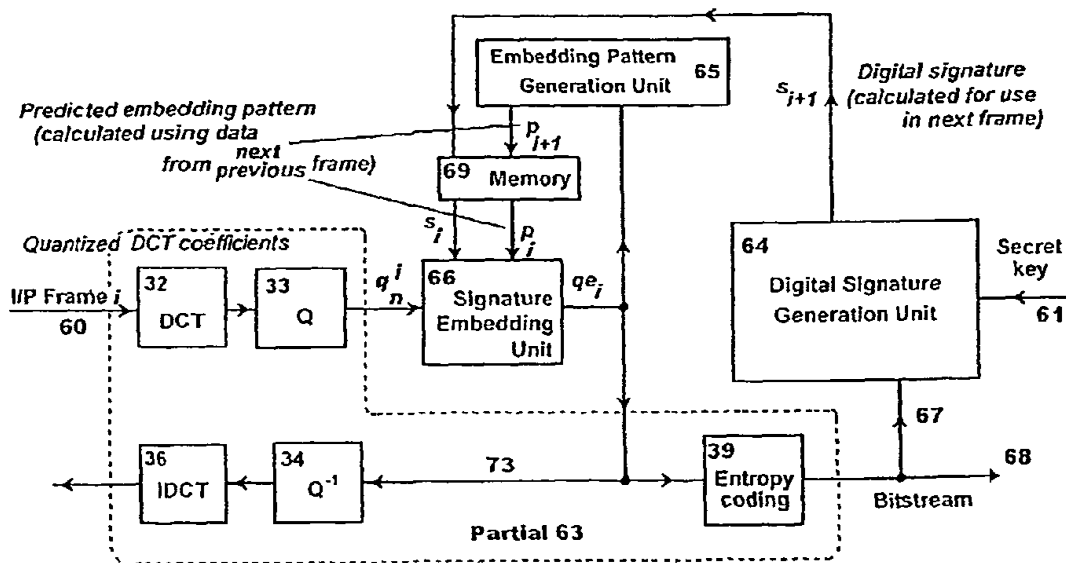
Figure 7 — Partial Detail of Augmented Video Encoder
