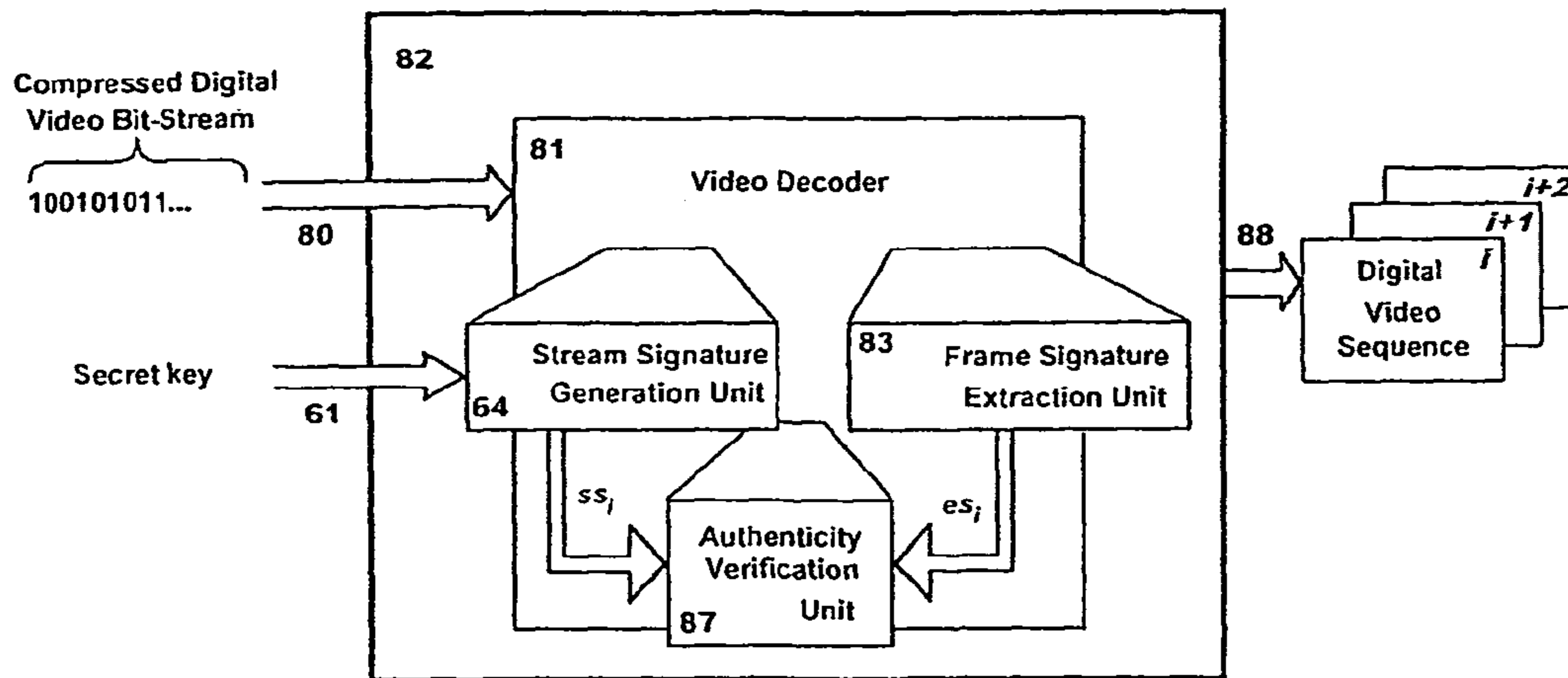
Figure 8 — Augmented Video Decoder
