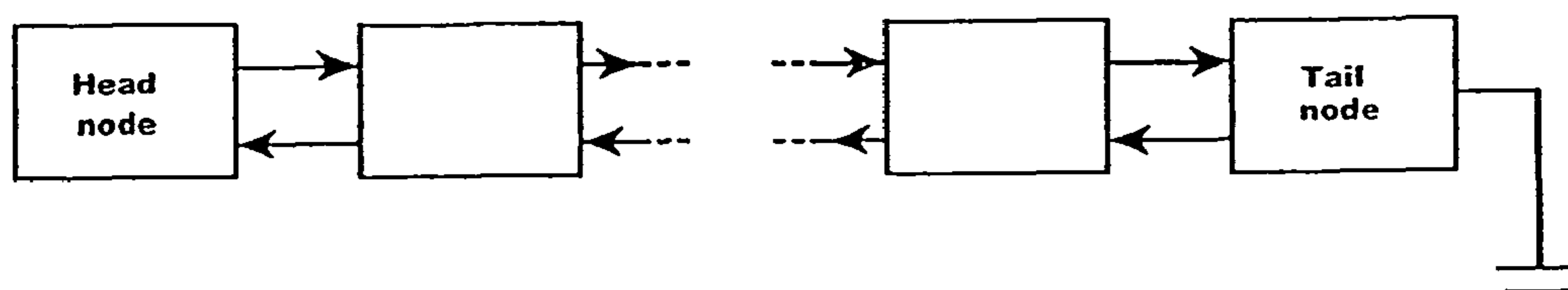
Figure 15 — Dynamic connected list
