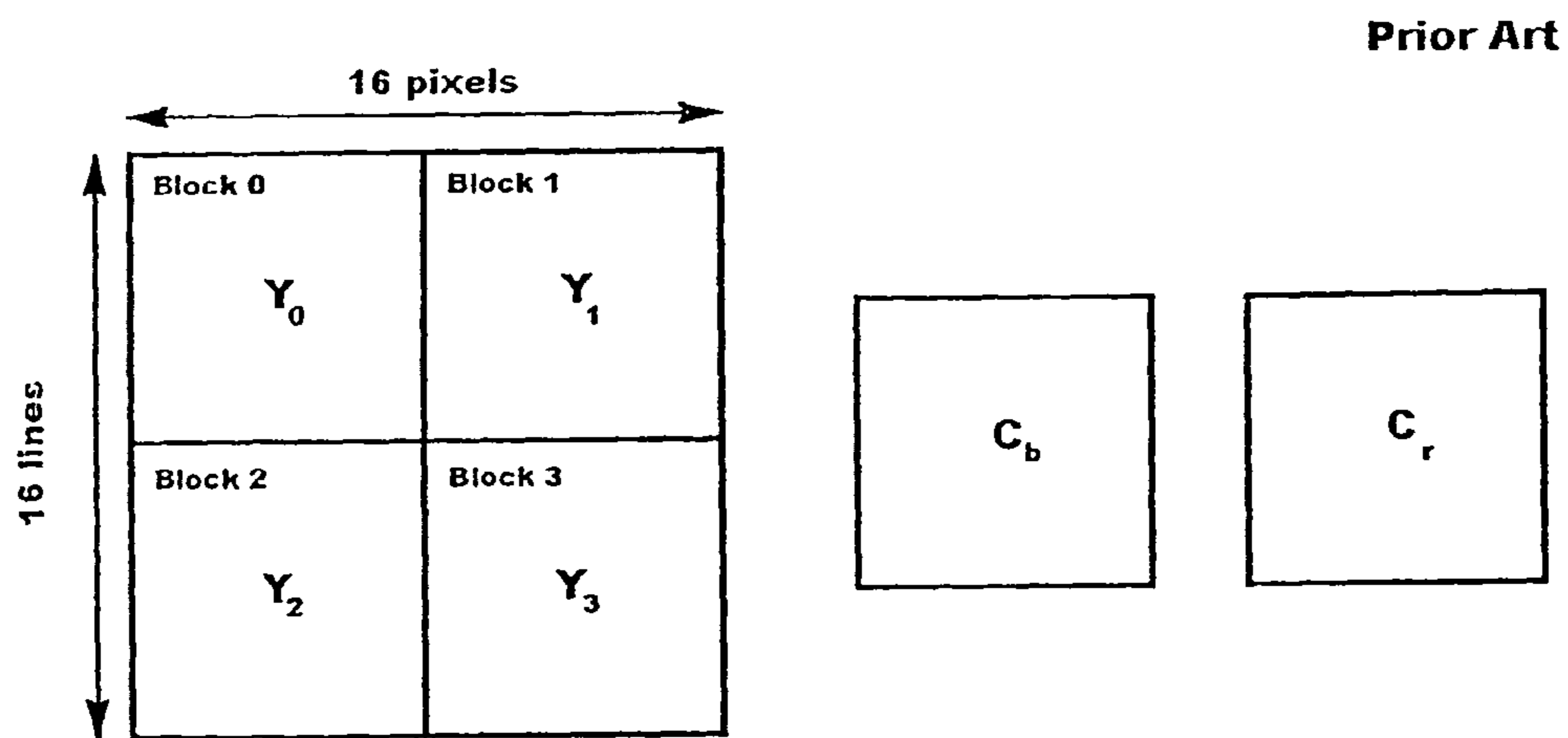
Figure 2 — Internal arrangement of blocks in a macroblock
