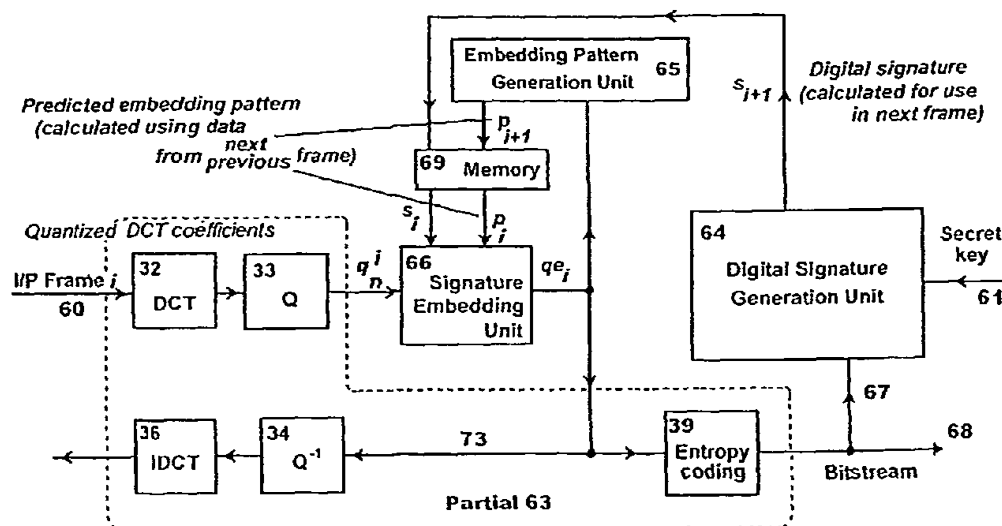
Partial Detail of Augmented Video Encoder
