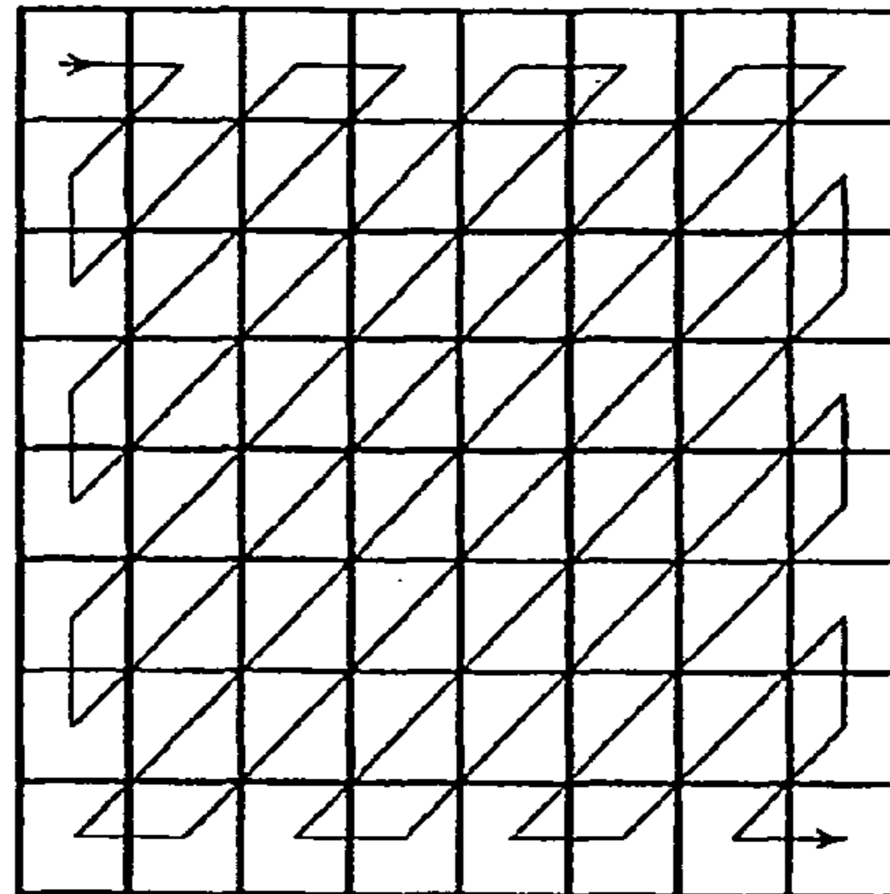
Figure 4 — Zig-zag block scanning
