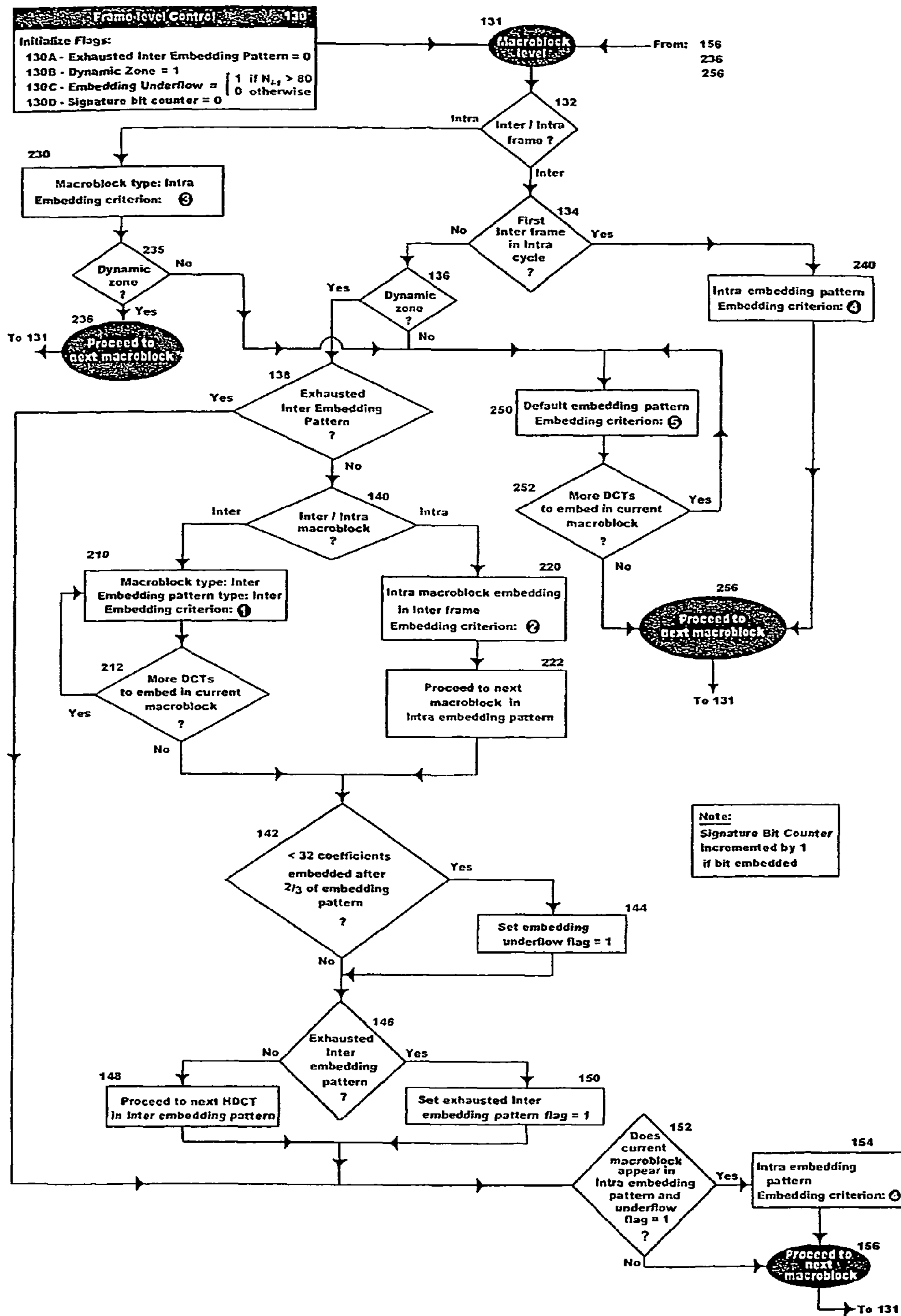
Figure 13 — Signature Bit Embedding in a Single Macroblock
