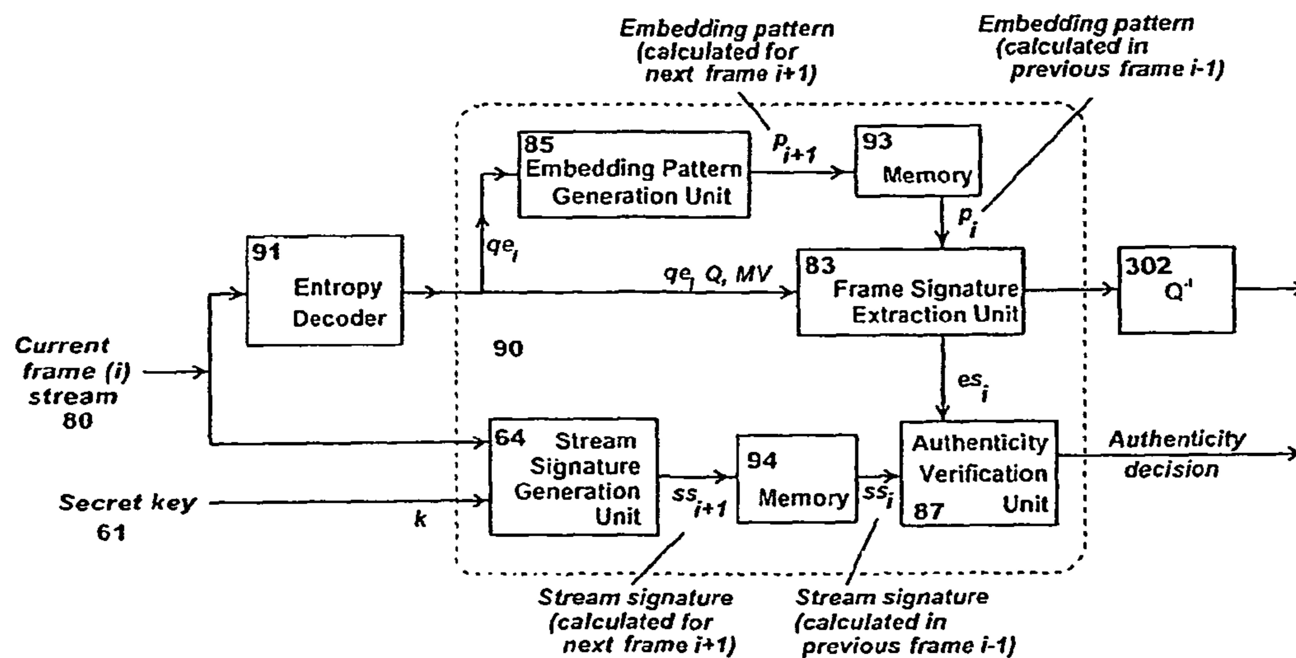
Figure 9 — Partial Detail of Augmented Video Decoder
