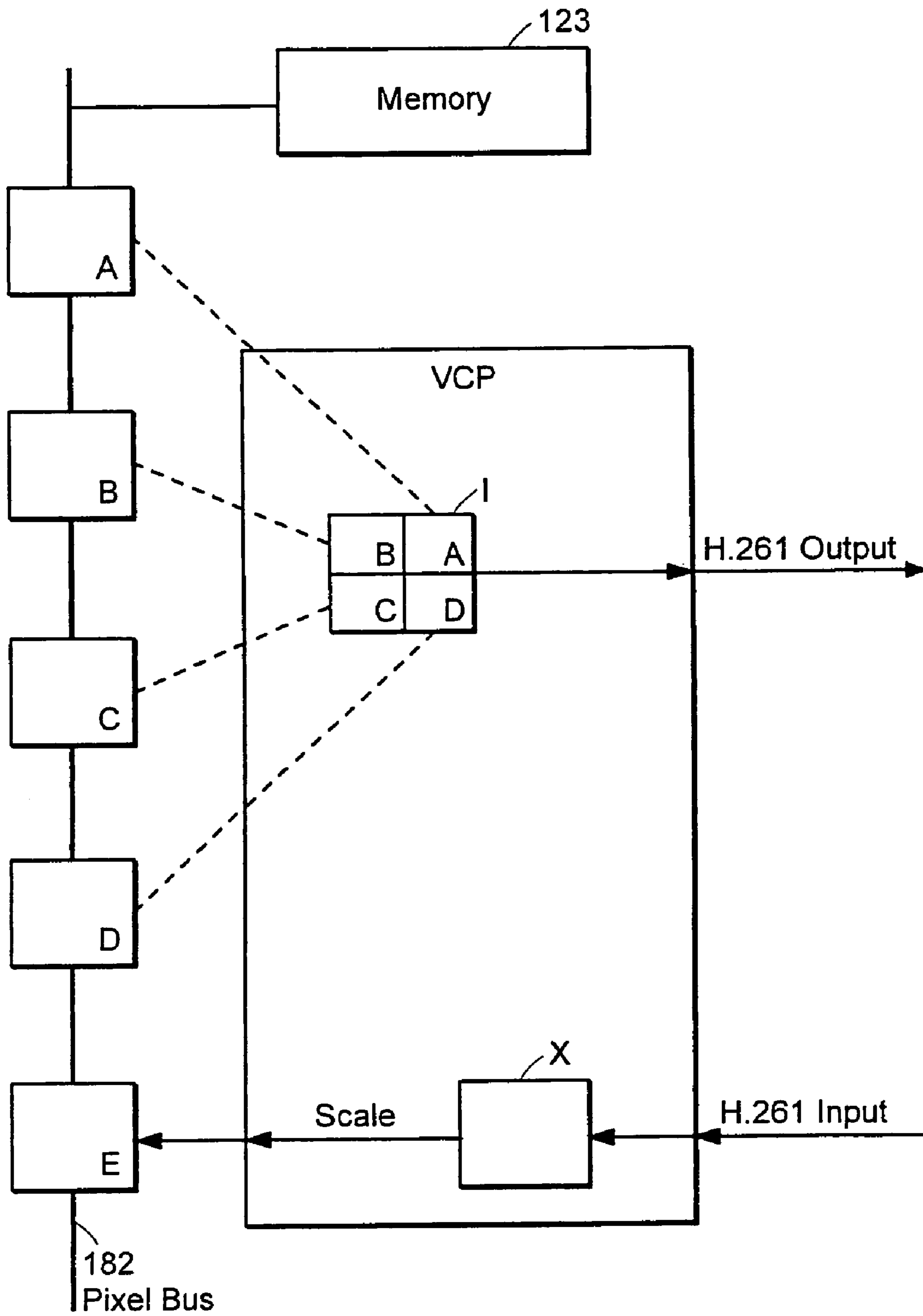
FIG. 4 PRIOR ART
