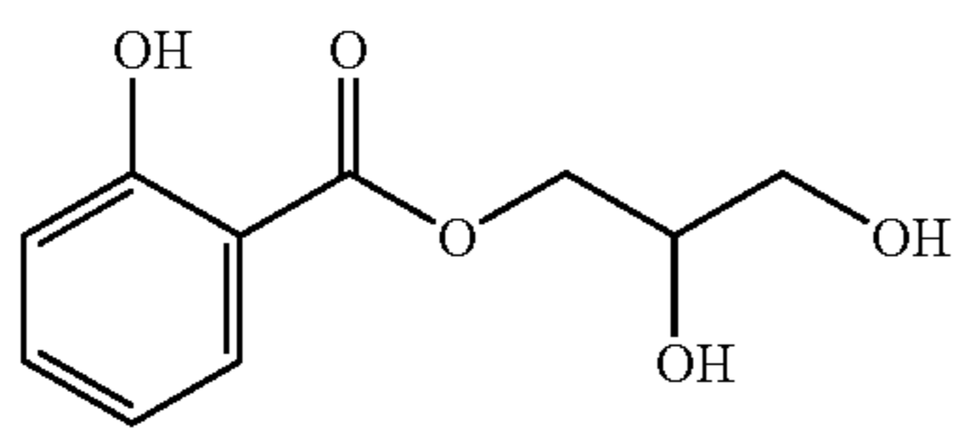
Glycerol Mono-Salicylate
