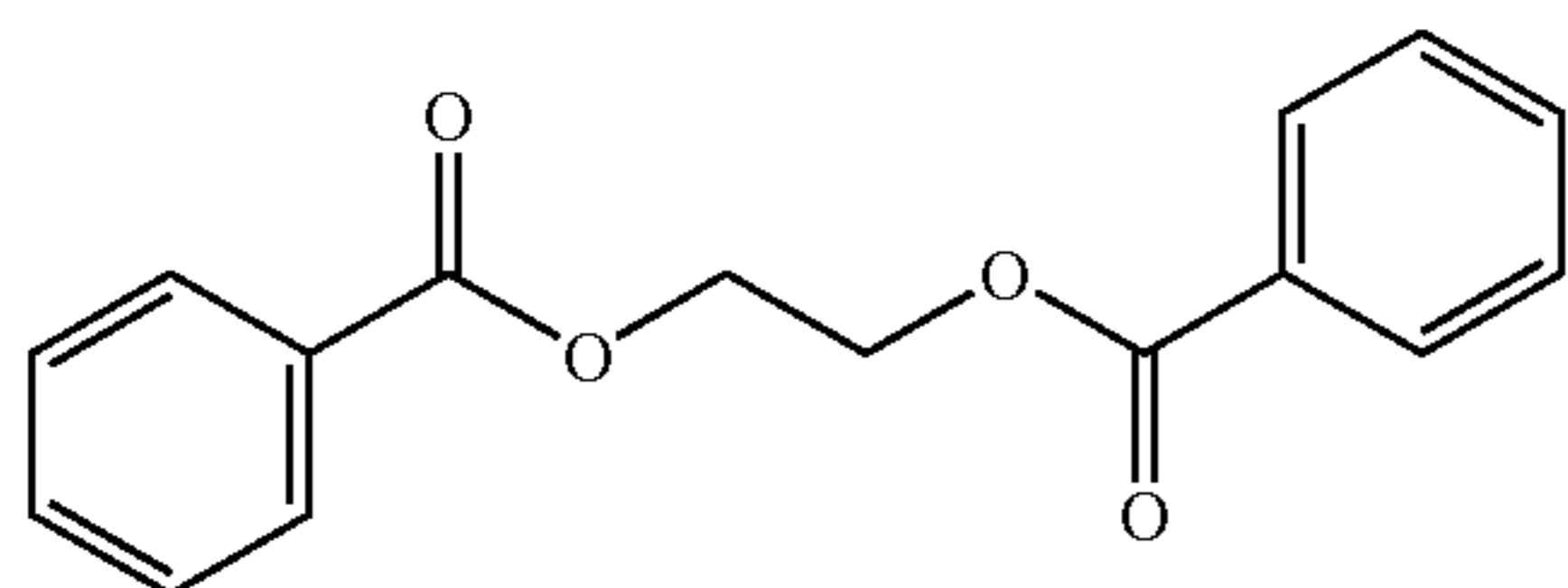
Ethylene Glycol Di-Benzoate
