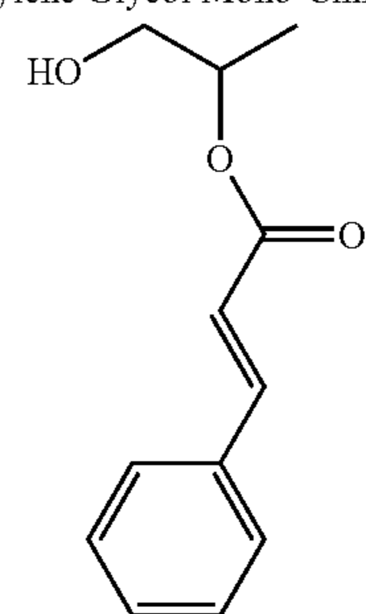
Propylene Glycol Mono-Cinnamate
