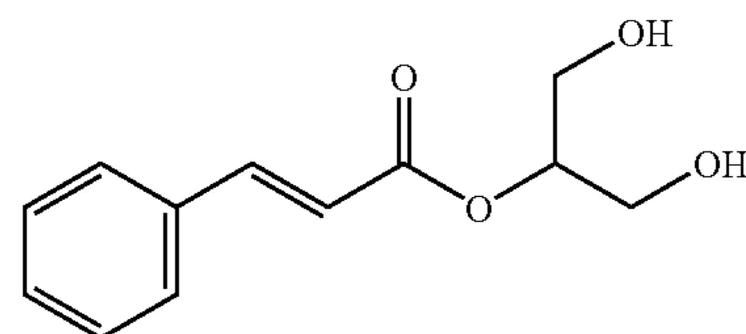
Glycerol Mono-Cinnamate
