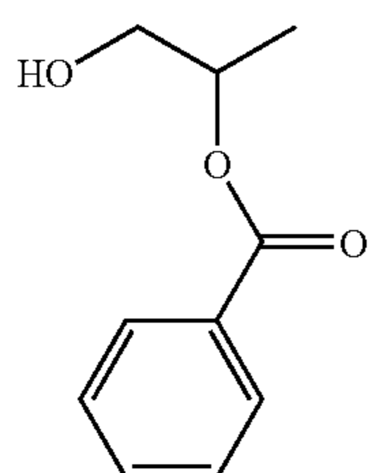
Propylene Glycol Mono-Benzoate
