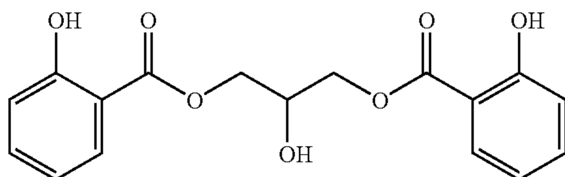
Glycerol Di-Salicylate
