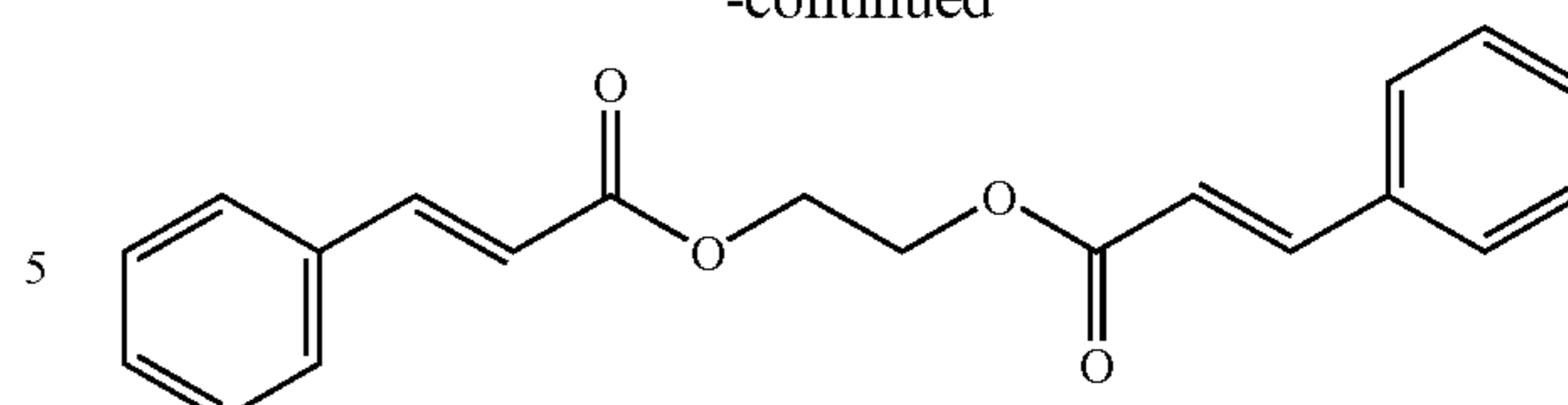
Ethylene Glycol Di-Cinnamate
