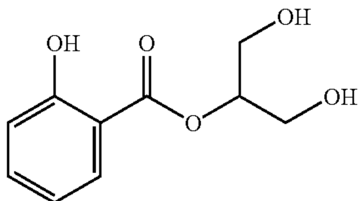
Glycerol Mono-Salicylate
