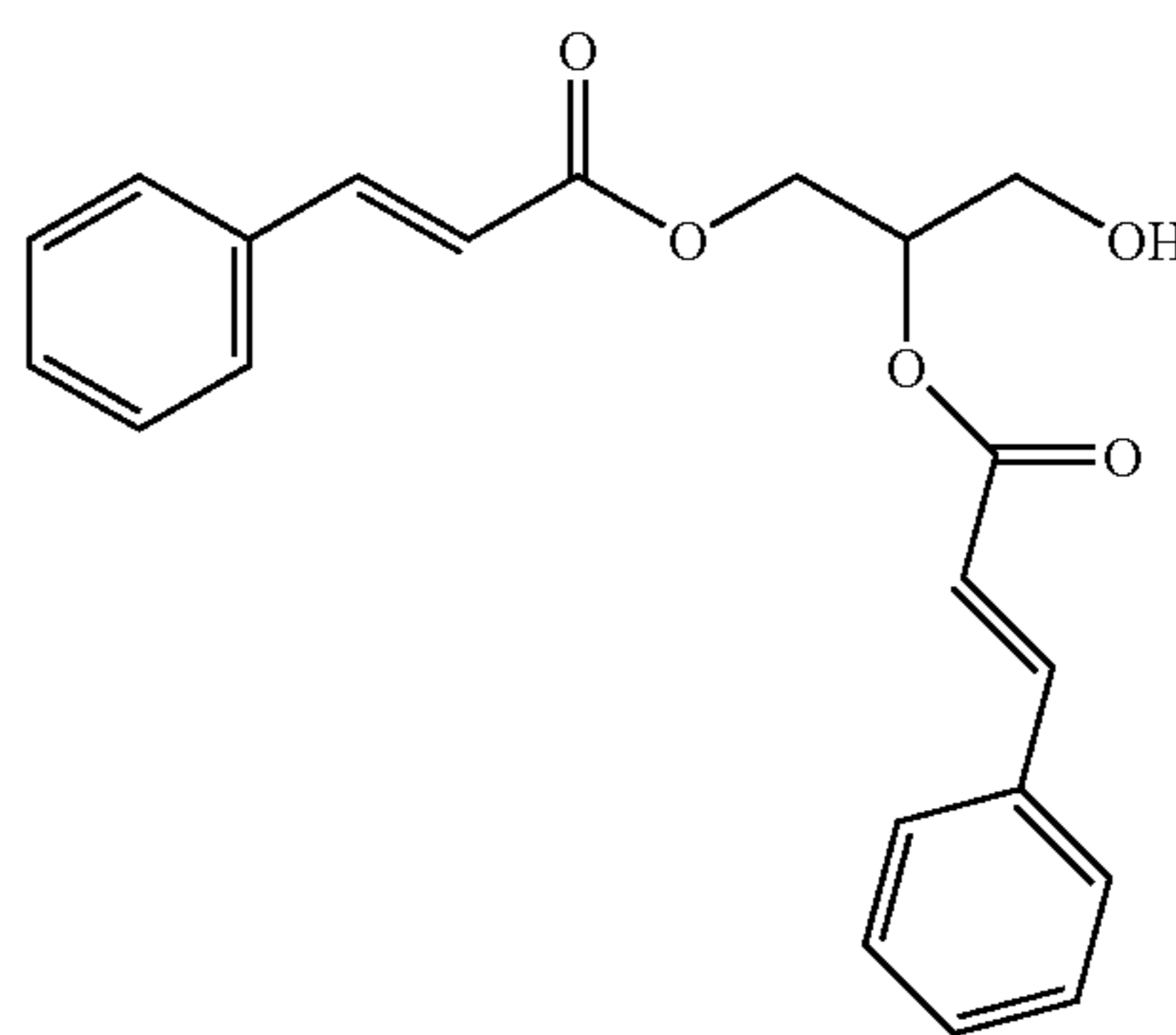
Glycerol Di-Cinnamate
