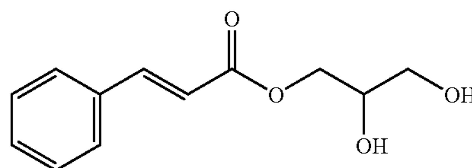
Glycerol Mono-Cinnamate
