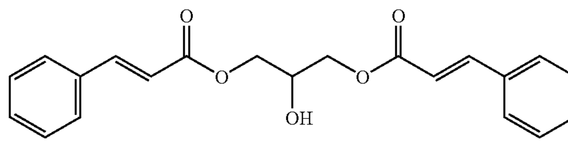
Glycerol Di-Cinnamate
