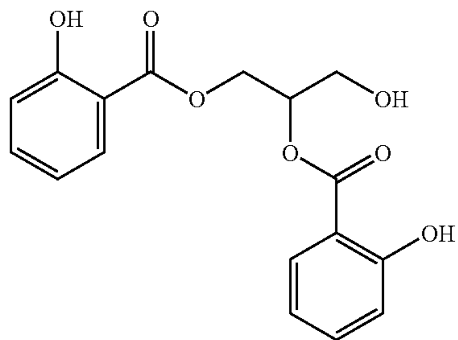
Glycerol Di-Salicylate
