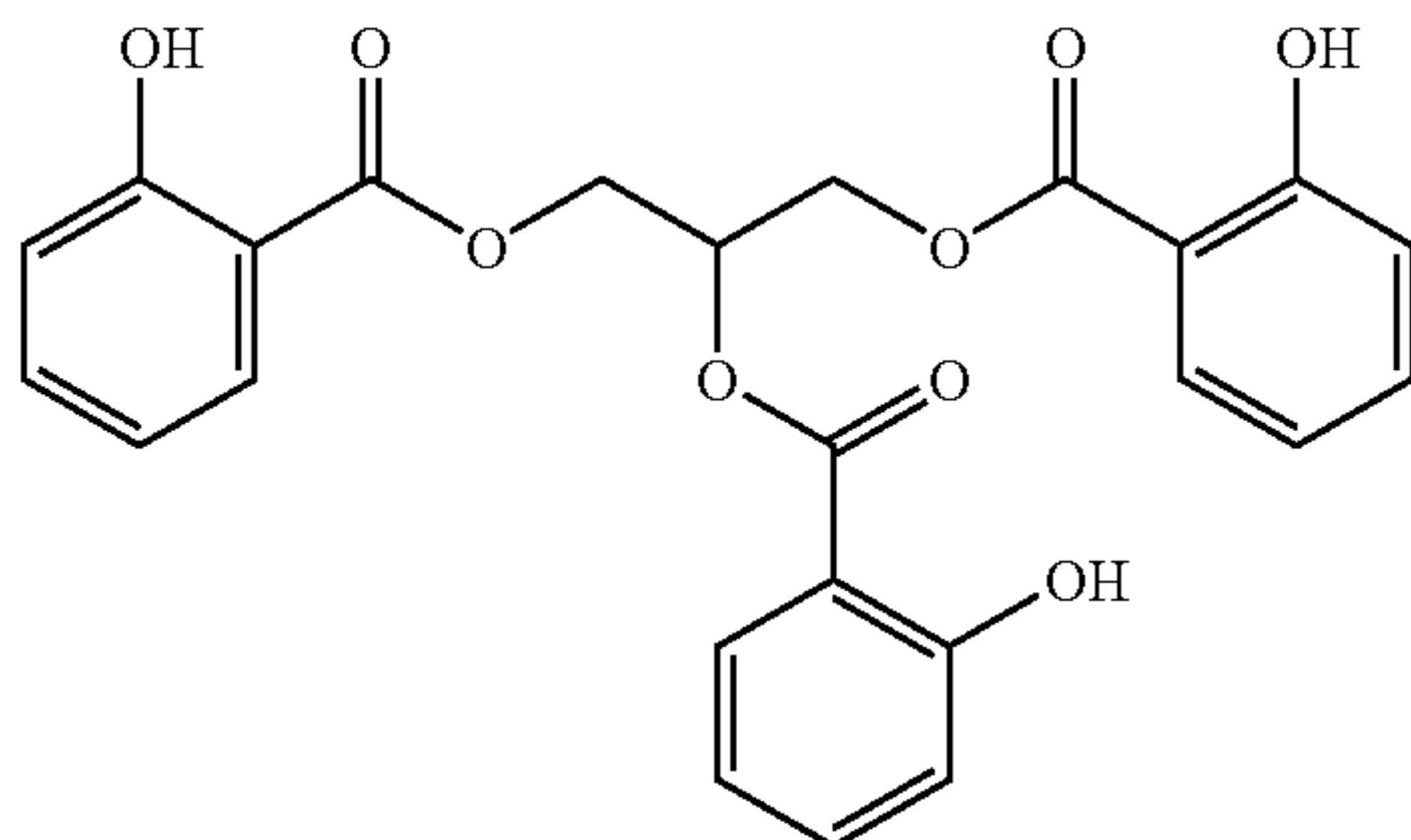
Glycerol Tri-Salicylate
