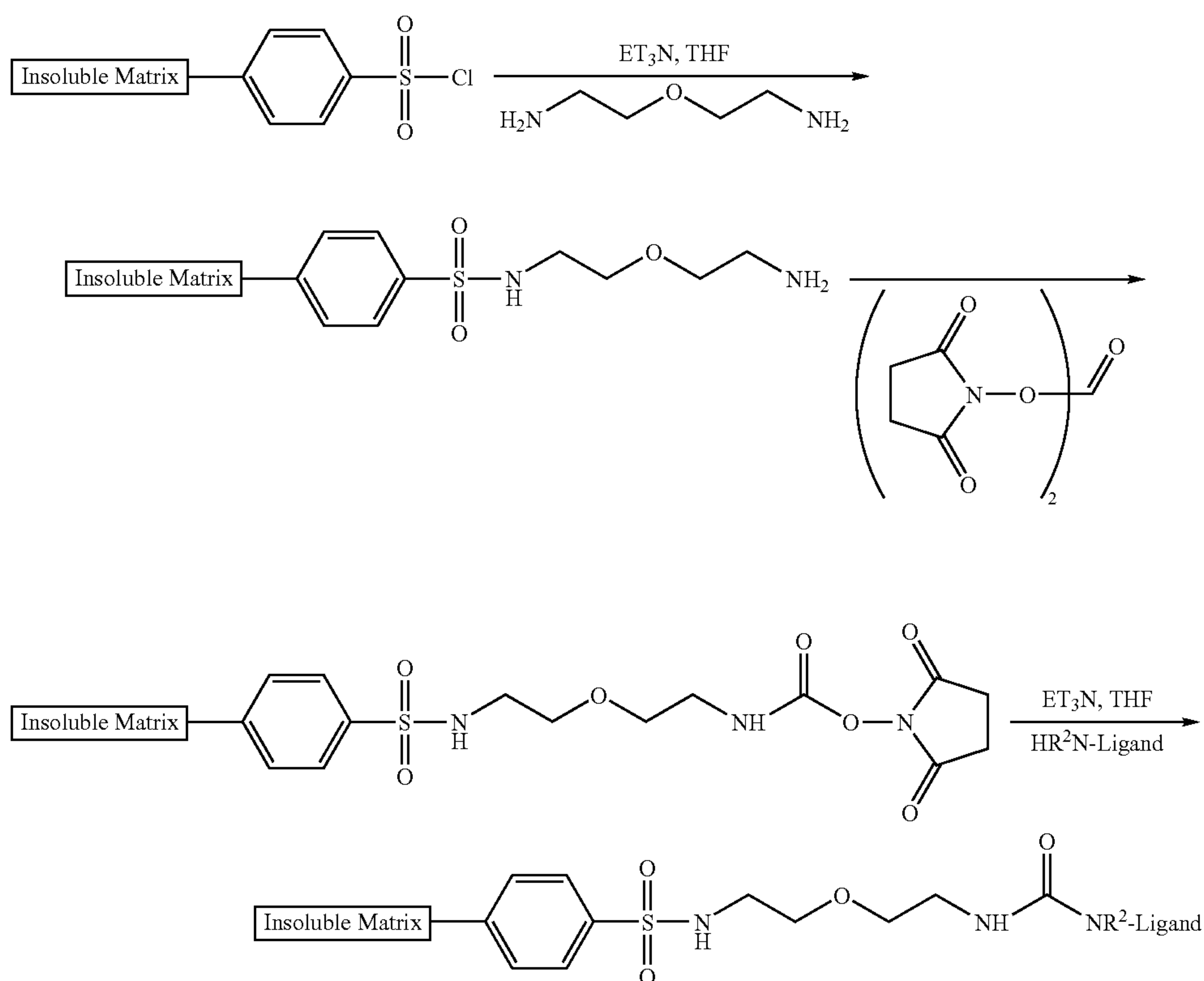
Scheme 4
