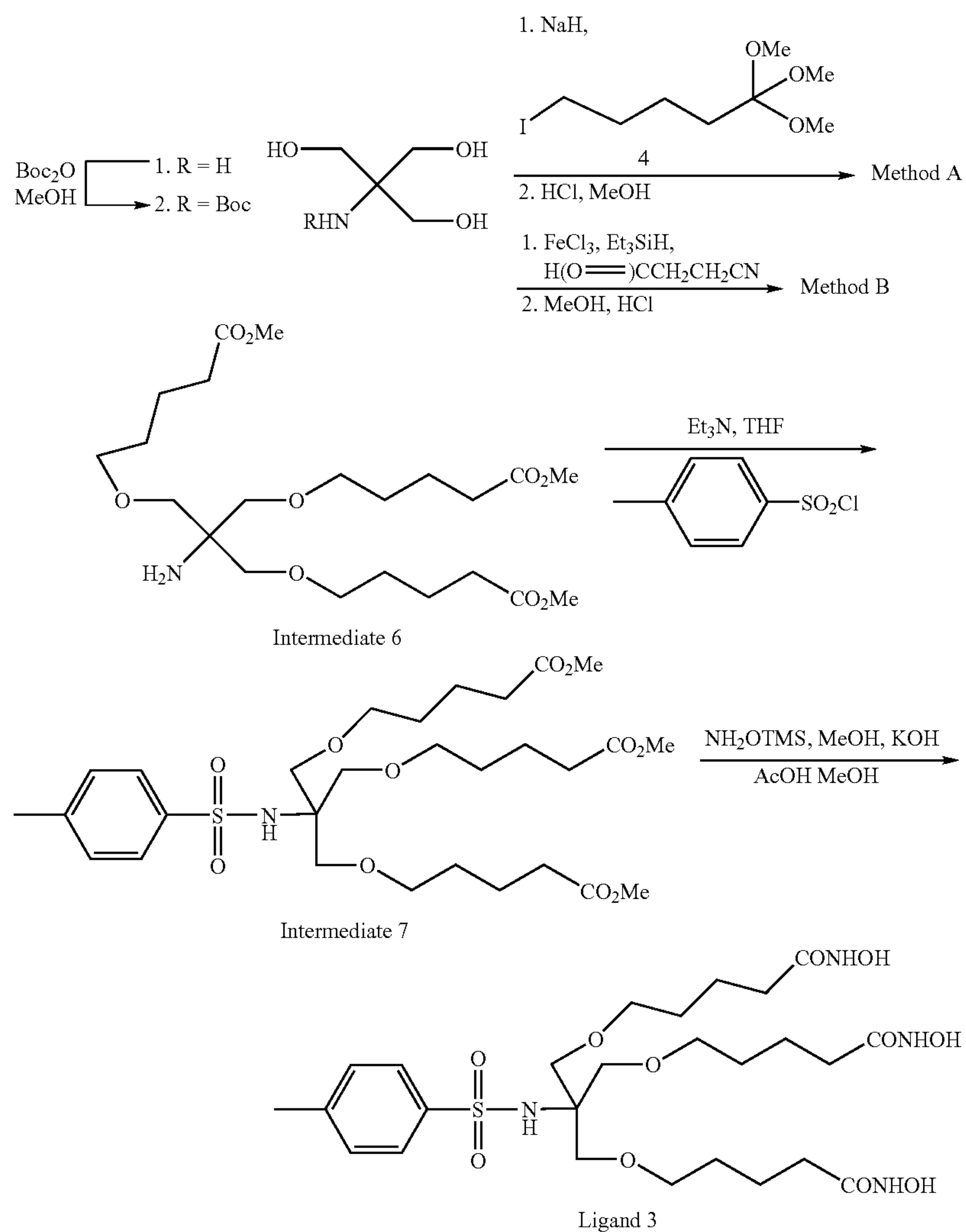
Scheme 7
