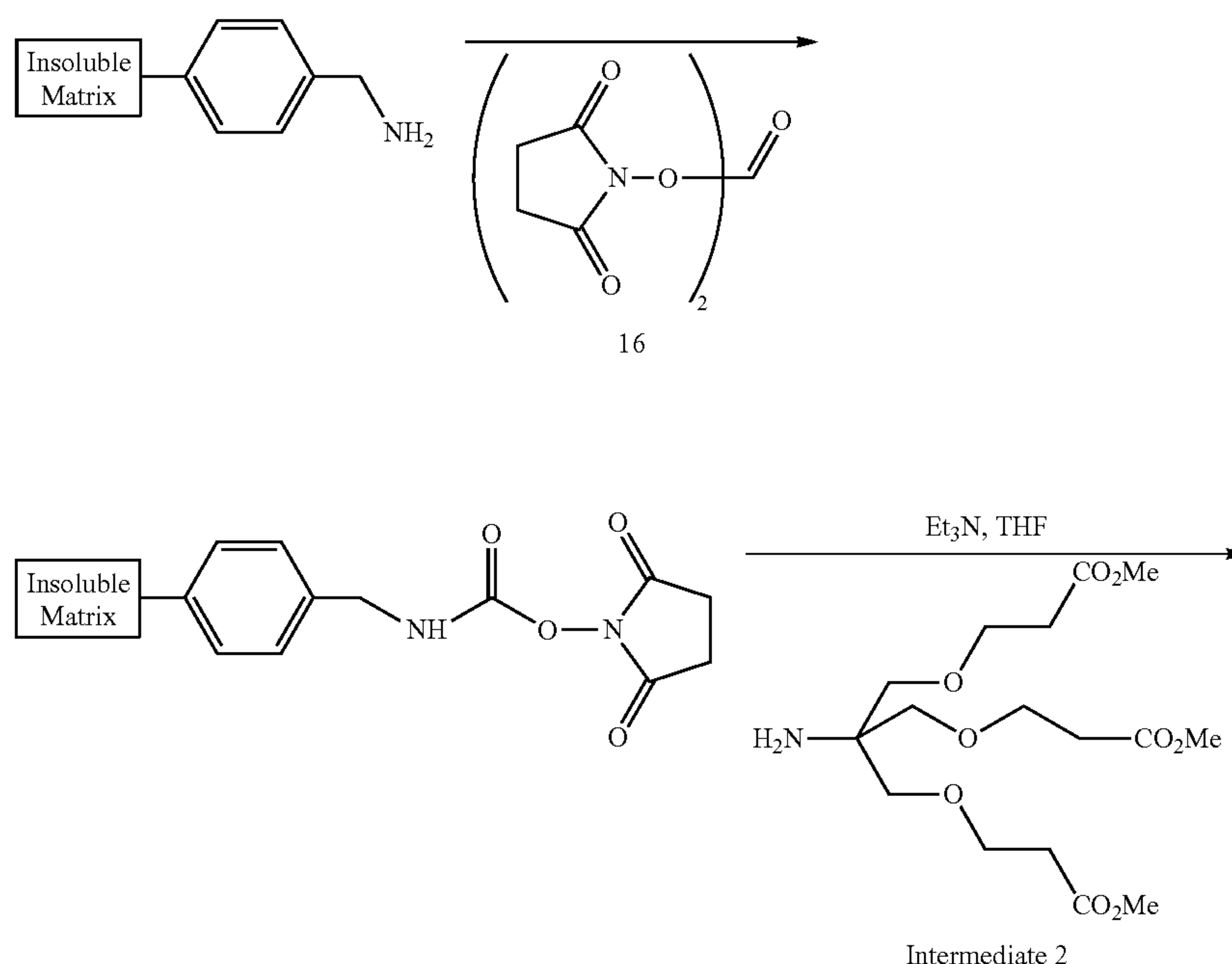
Scheme 15
