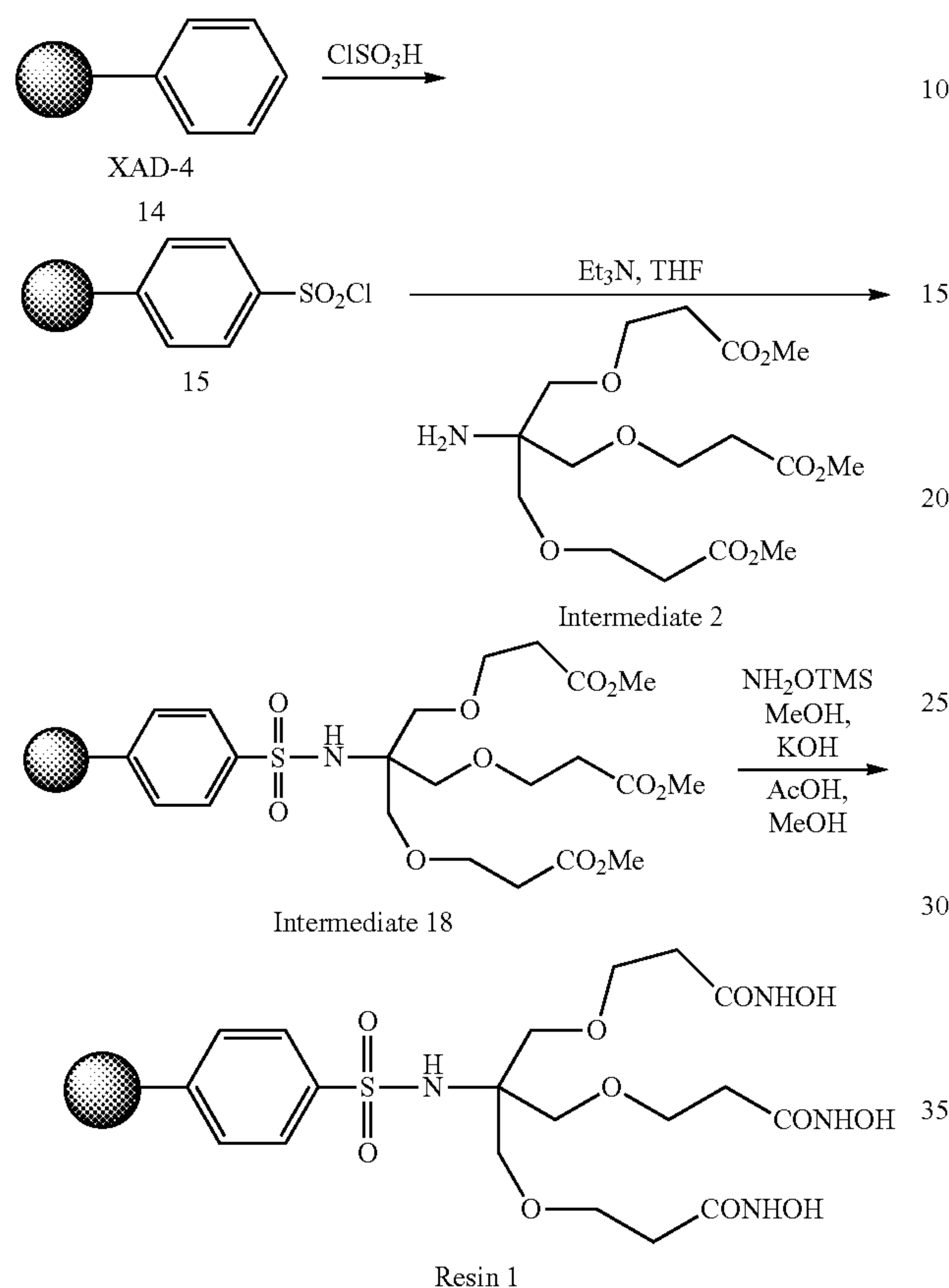
Scheme 12
