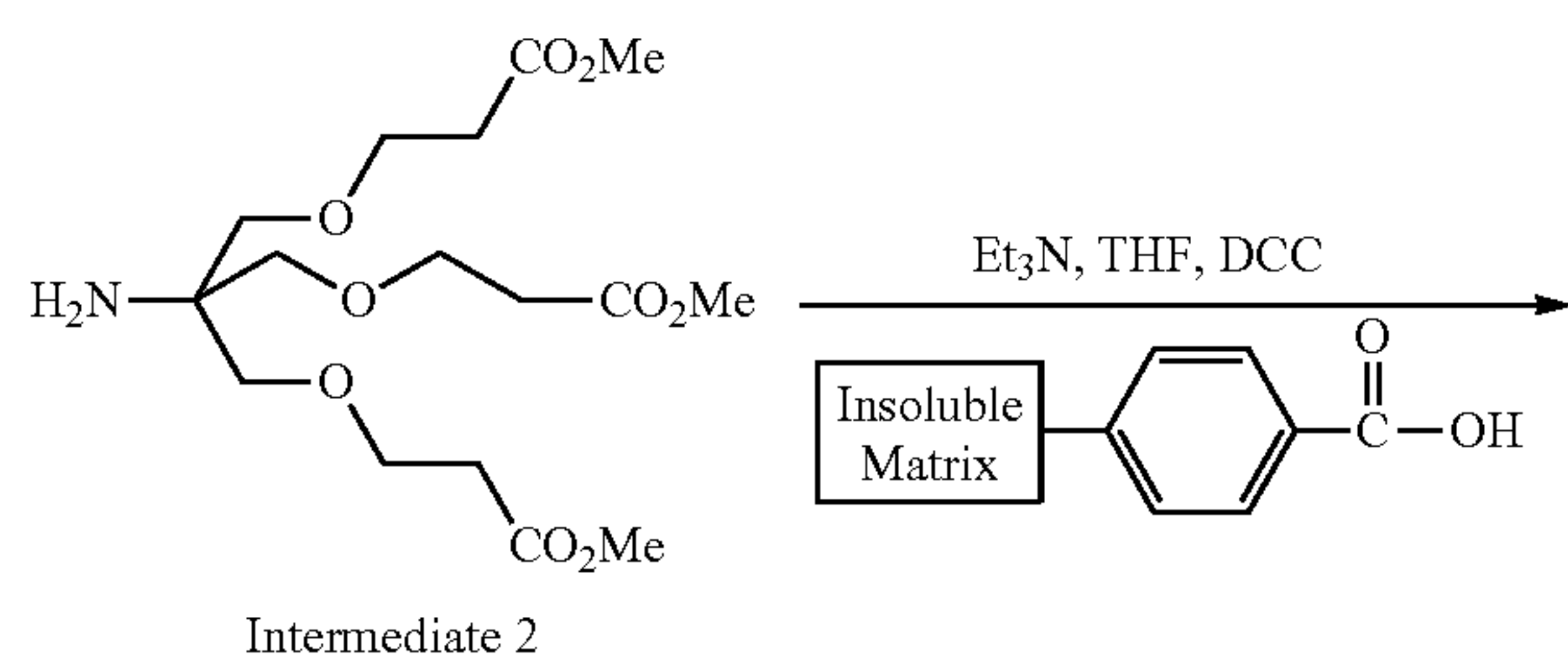
Scheme 14
