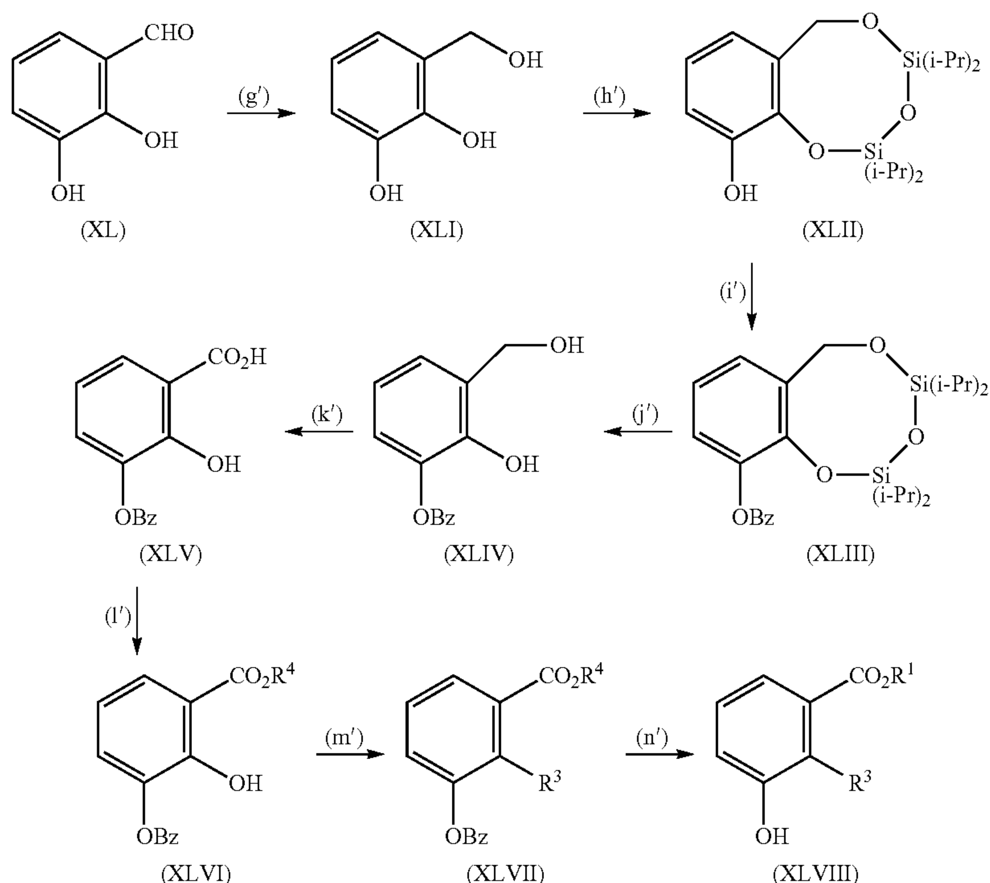
Reaction Scheme 9
