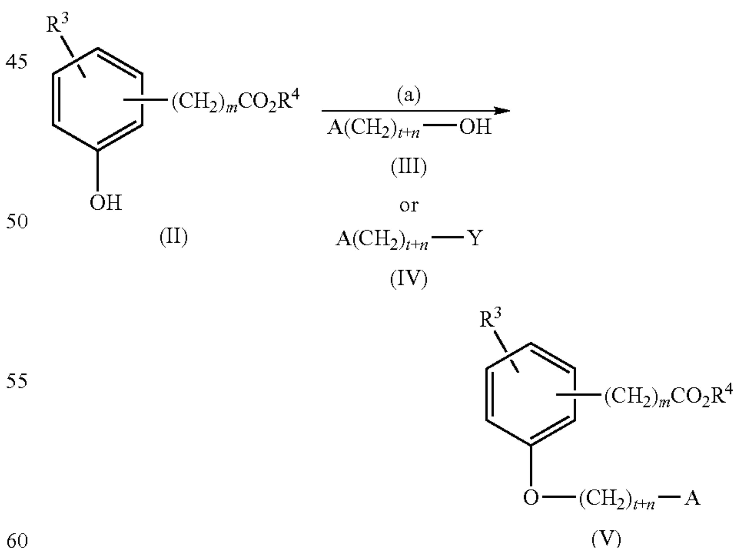
Reaction Scheme 1
