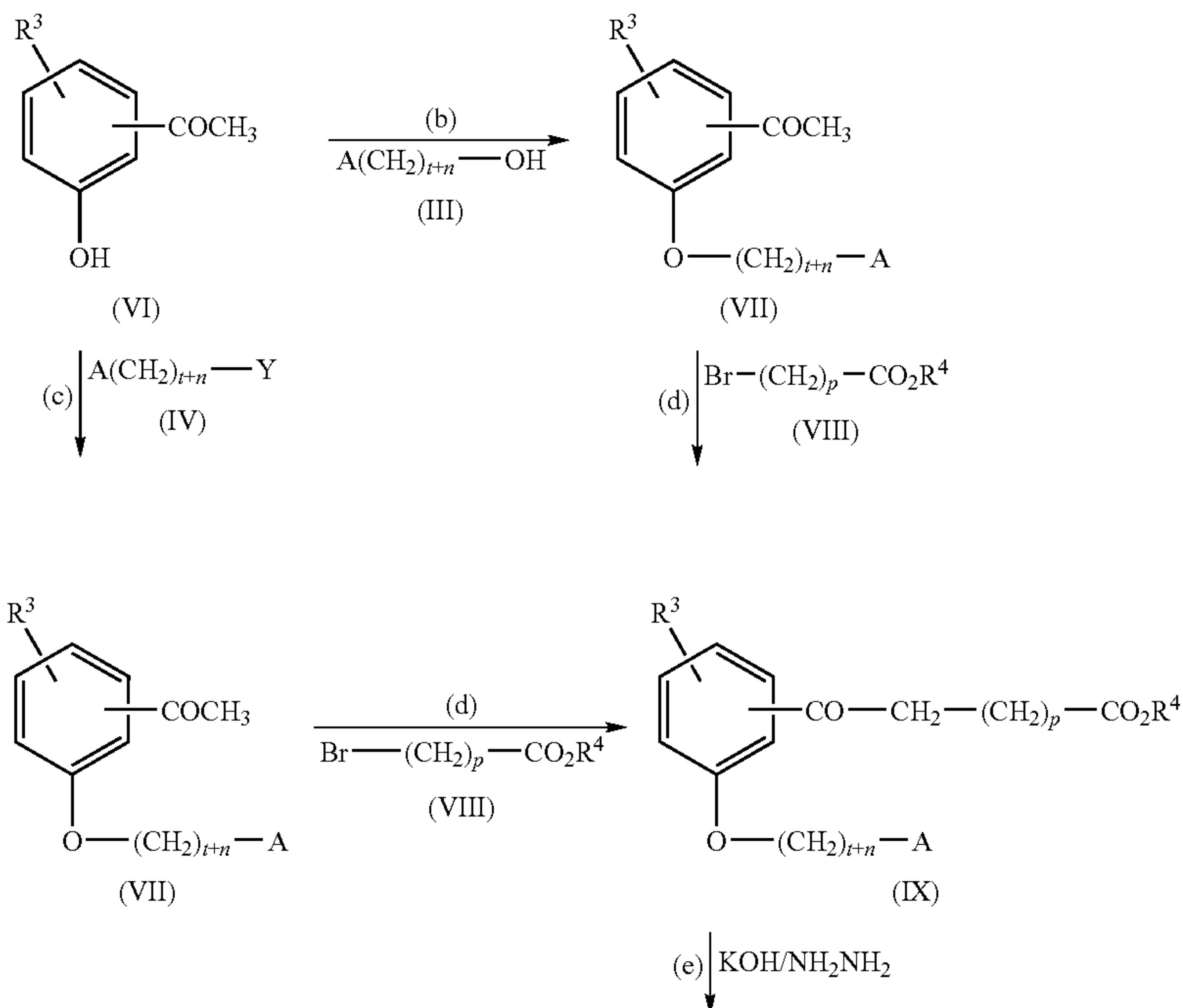
Reaction Scheme 2
