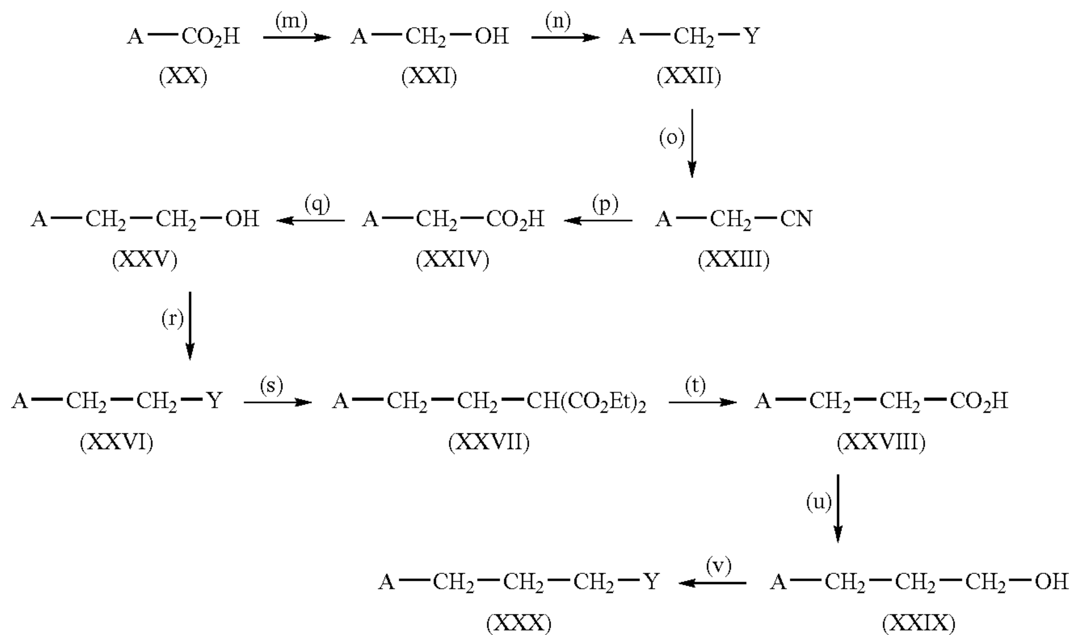
Reaction Scheme 5
