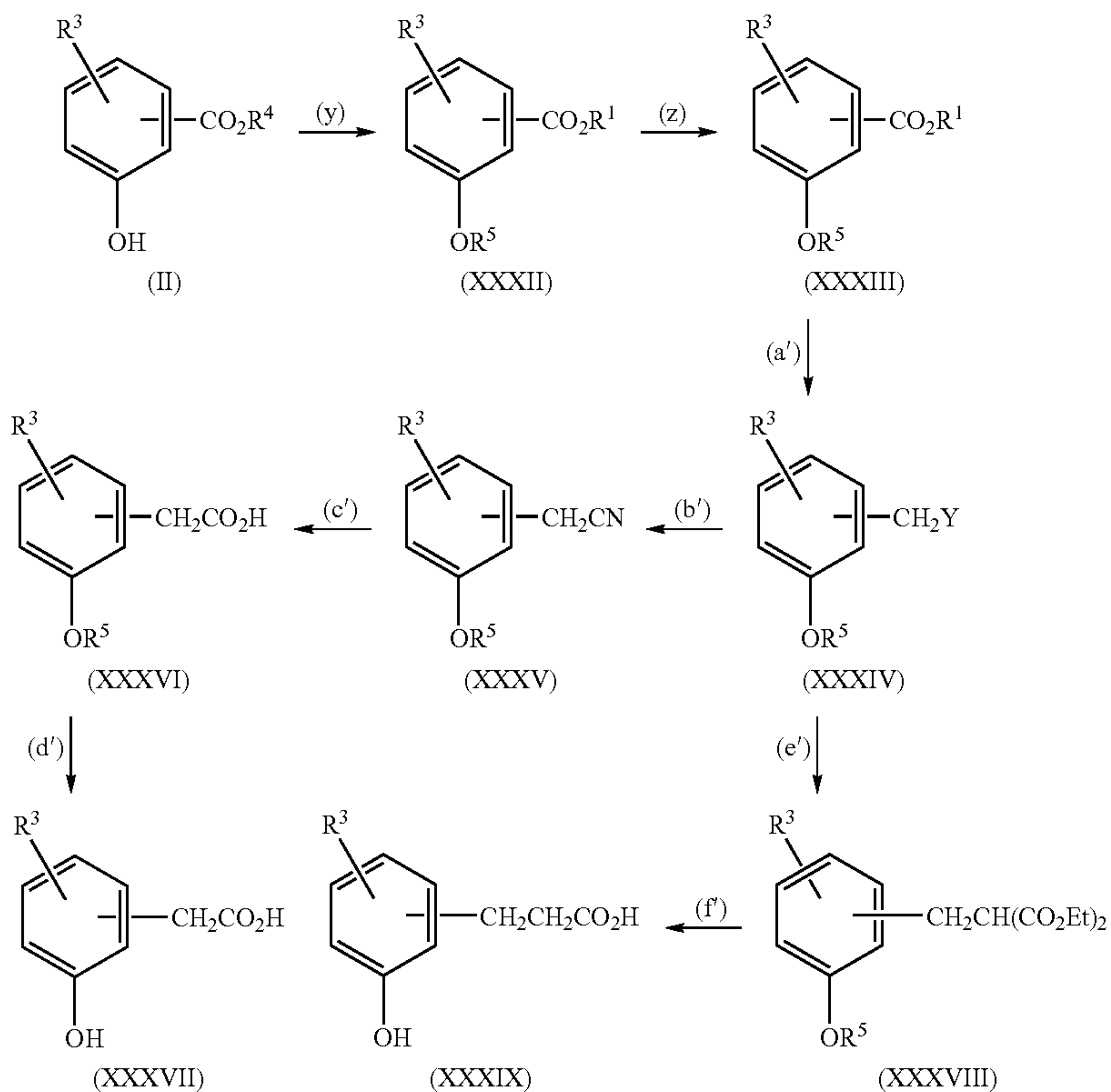
Reaction Scheme 8
