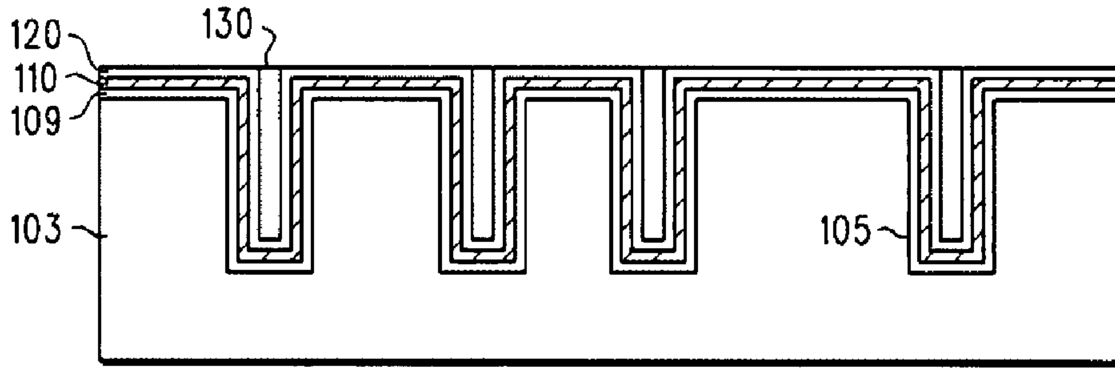
FIG. 5 -PRIOR ART-
