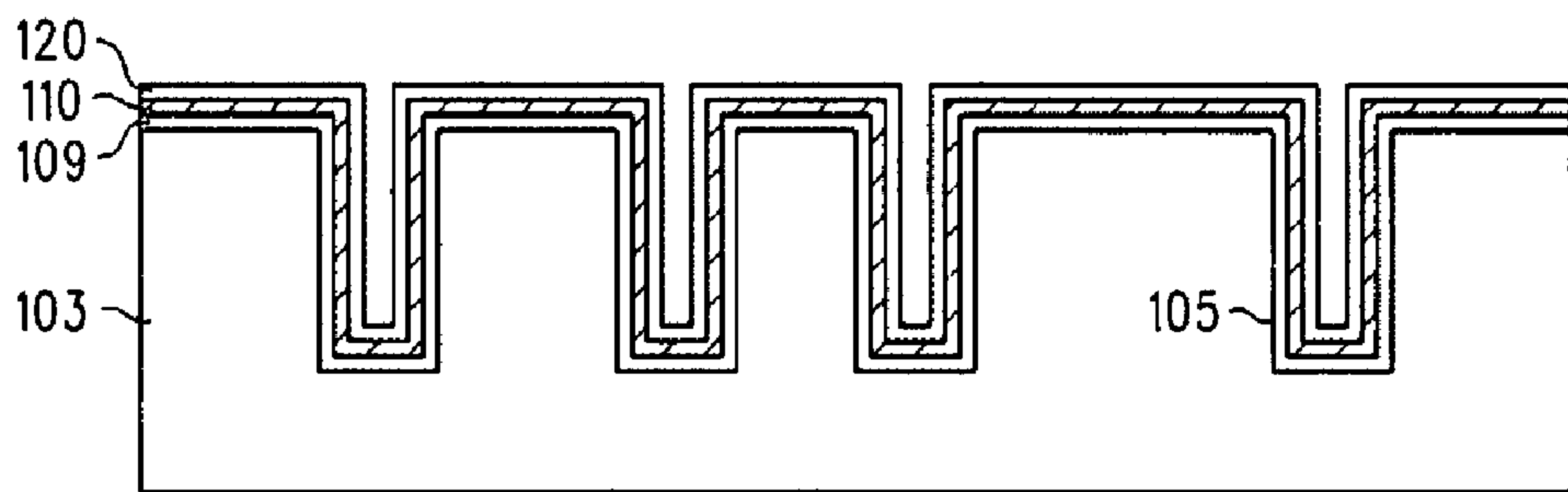
FIG. 2 -PRIOR ART-
