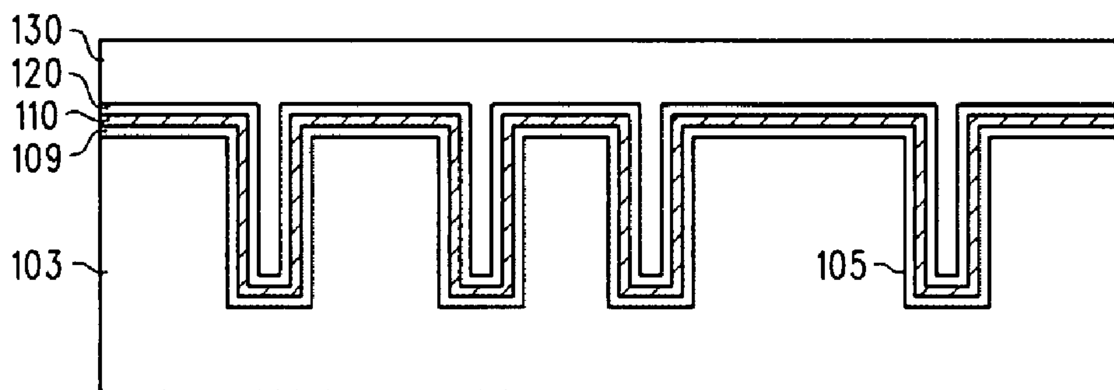
FIG. 4 -PRIOR ART-
