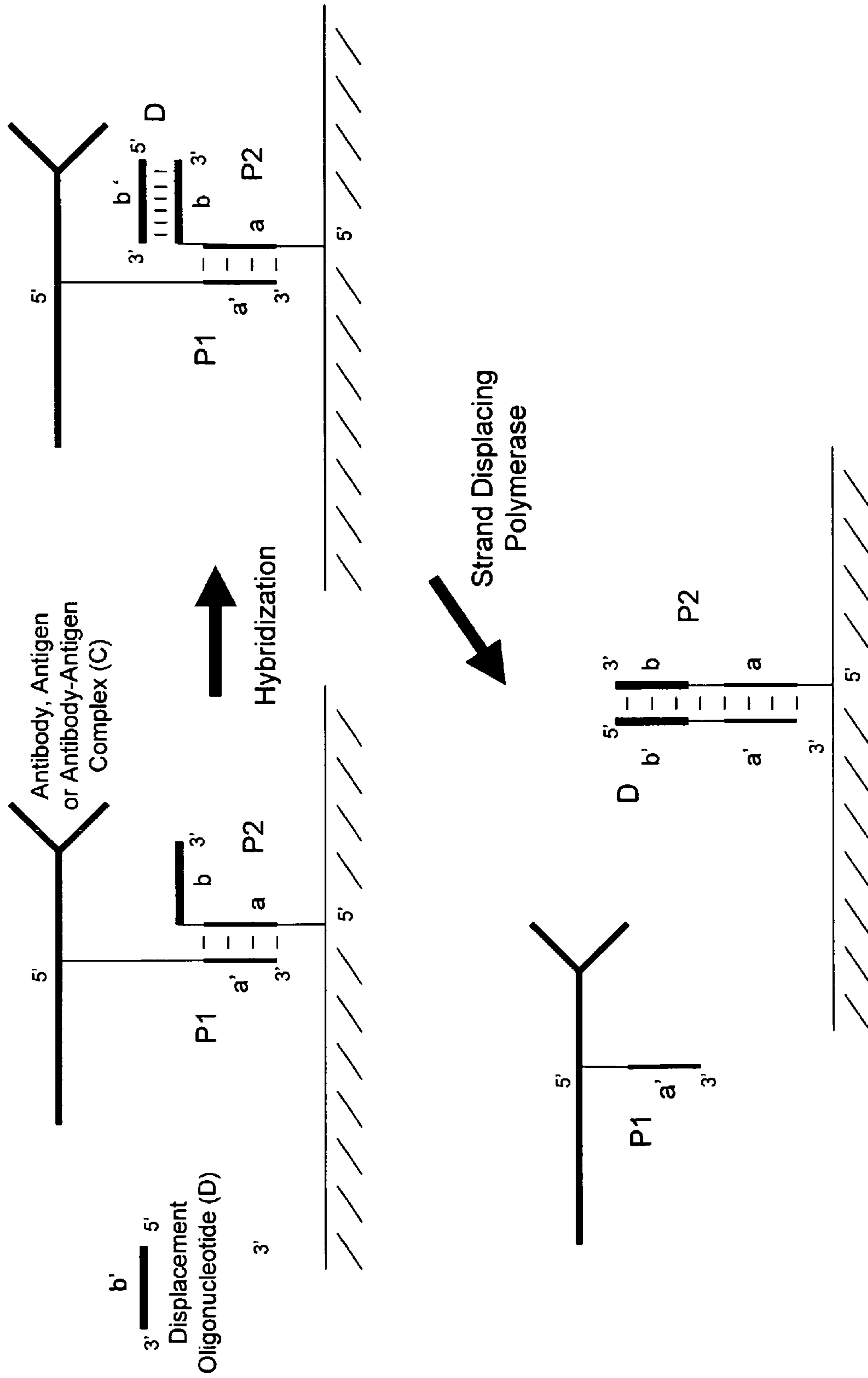
FIGURE 6I Oligonucleotide extension
