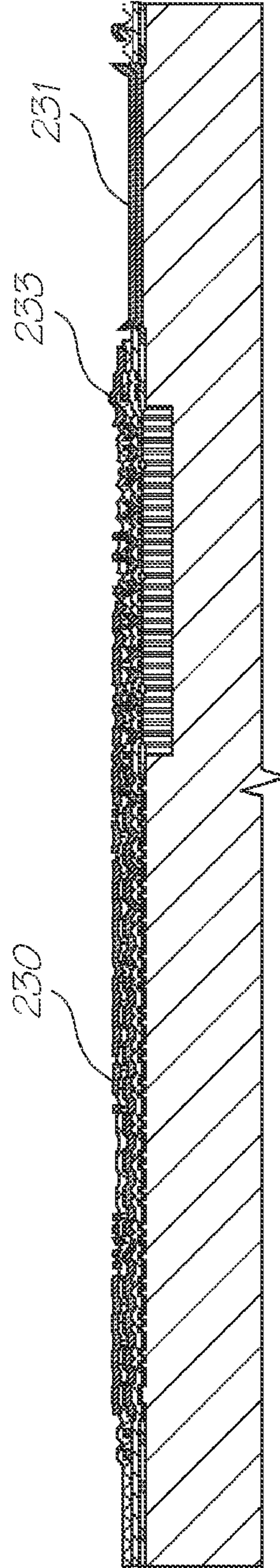
Deposit metal 2
