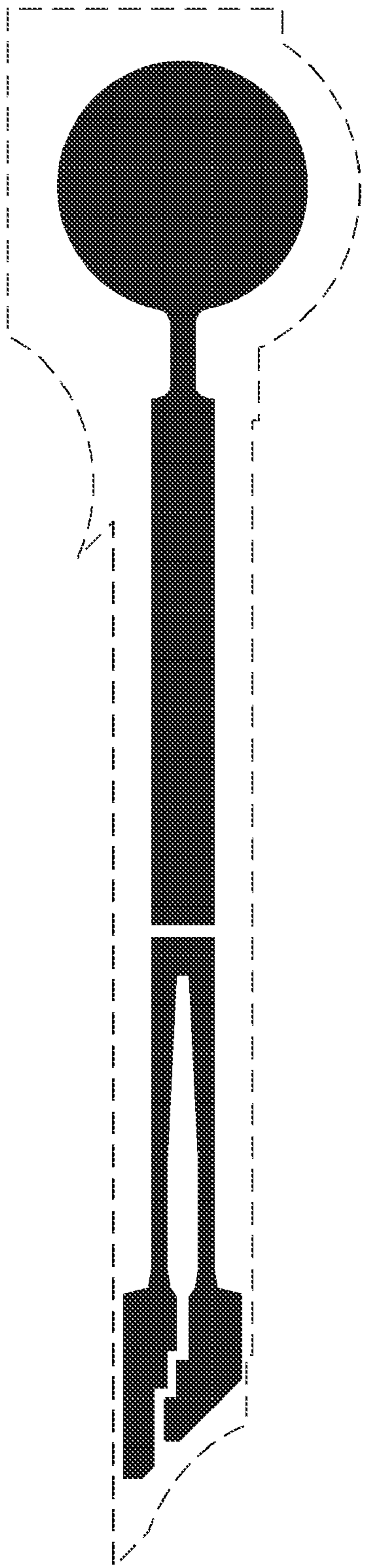
Heater mask
