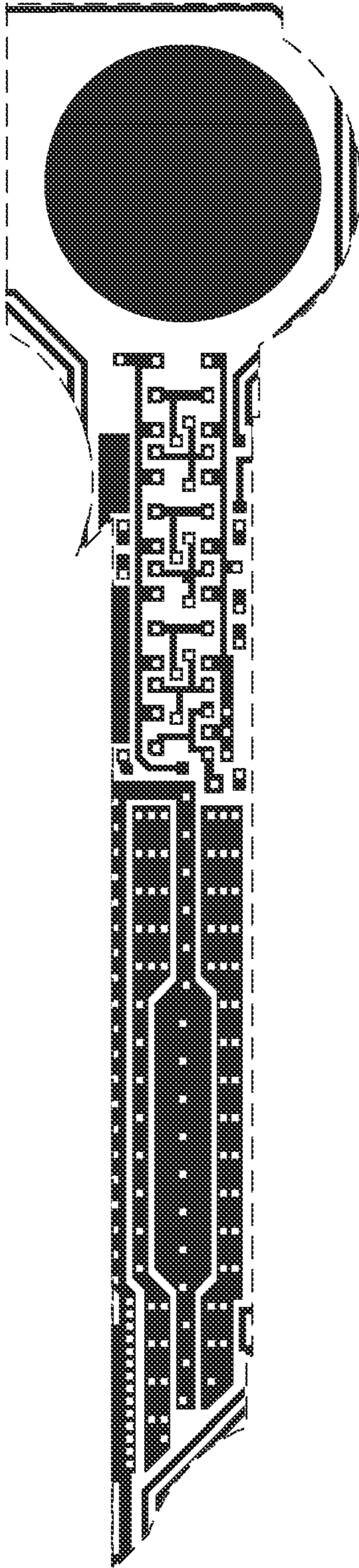
Metal 1 mask
