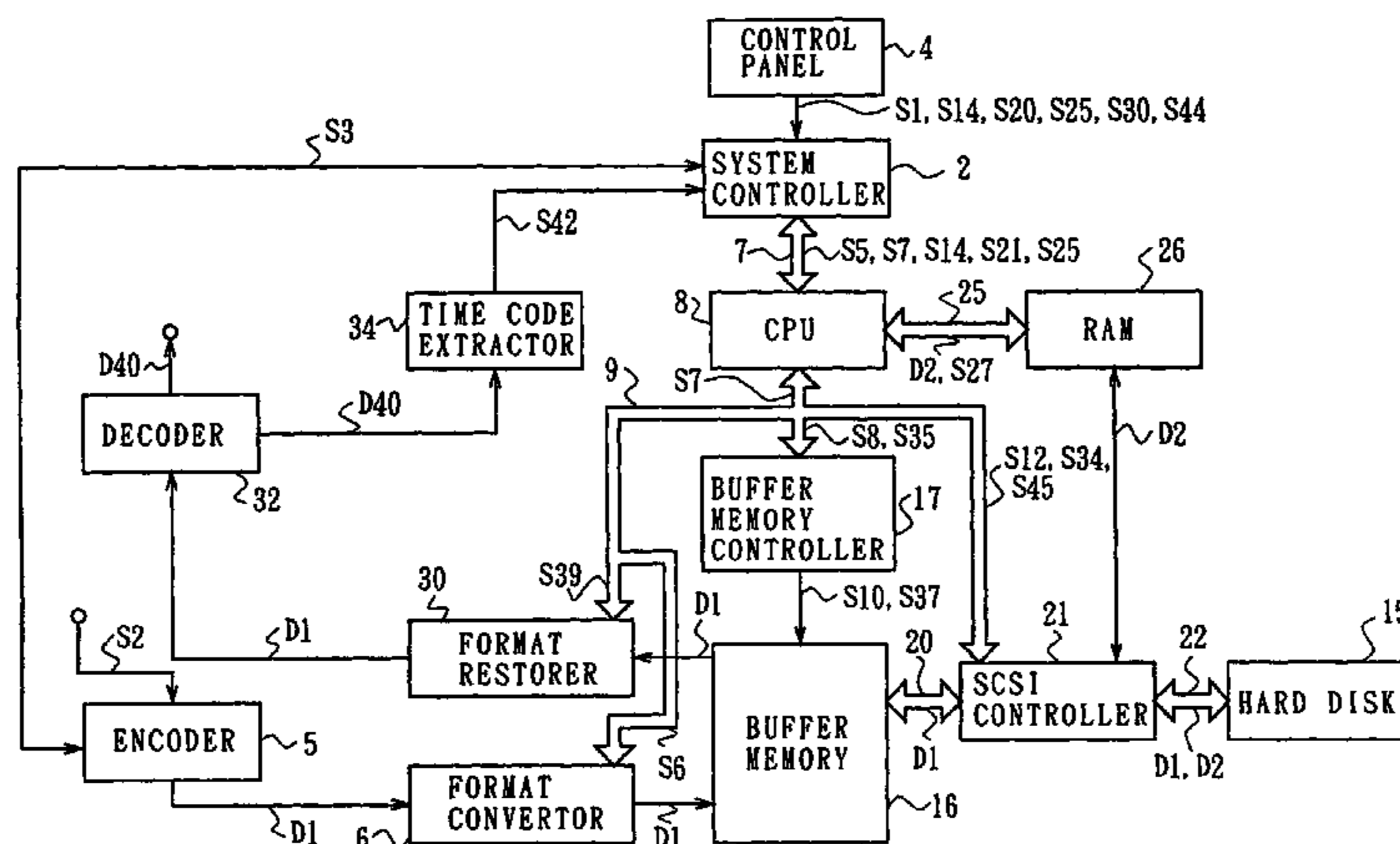
1 RECORDING/REPRODUCING APPARATUS
