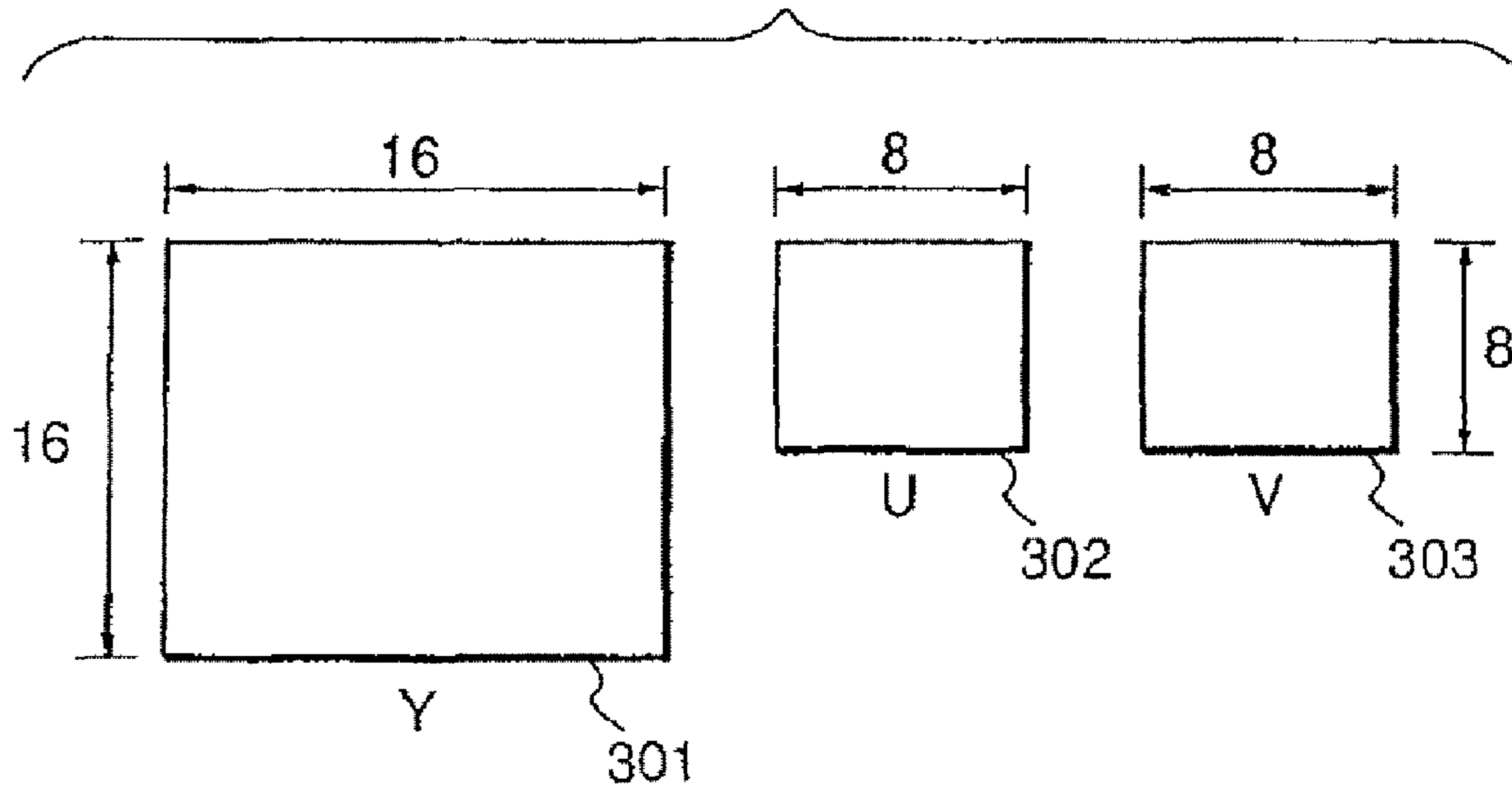
FIG. 3 (PRIOR ART)
